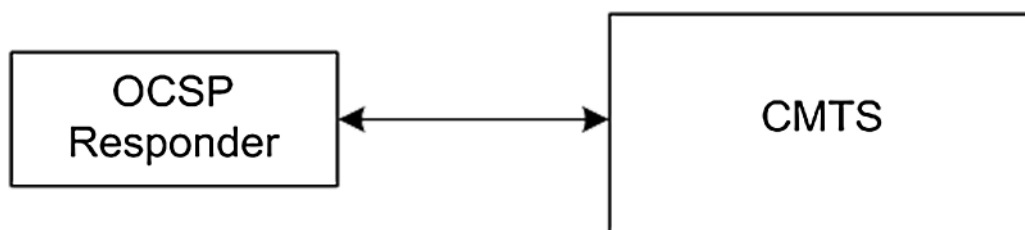
Figure 13-2 - OCSP Framework
