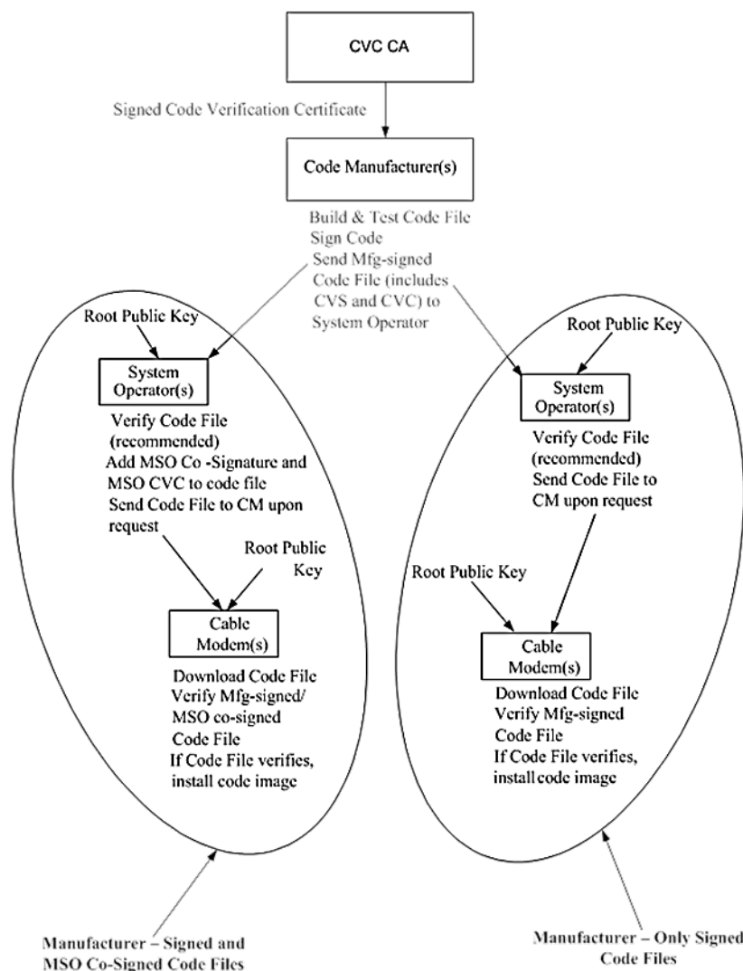
Figure 14-1 - Typical Code Validation Hierarchy
