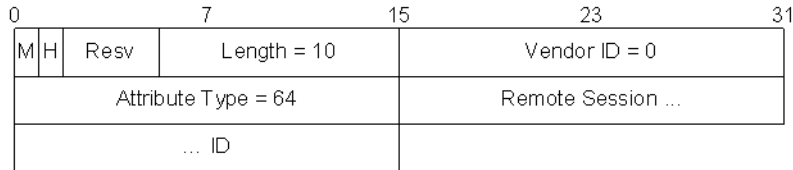
Figure 28 - Remote Session ID AVP
