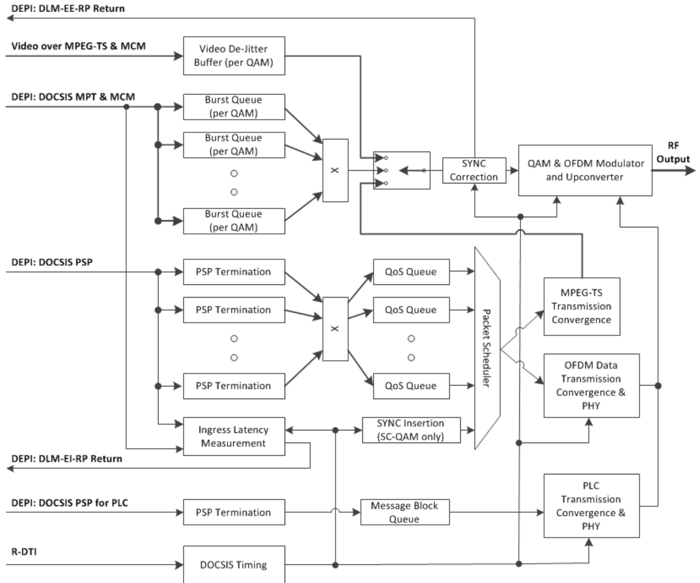
Figure 4 - Downstream DOCSIS and Video R-PHY Block Diagram
