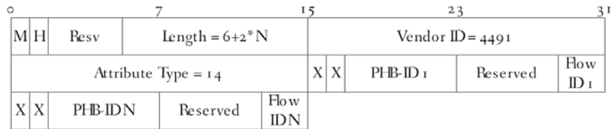
Figure 45 - Upstream Flow AVP
