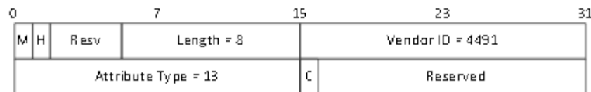
Figure 44 - DEPI Multicast Capability AVP
