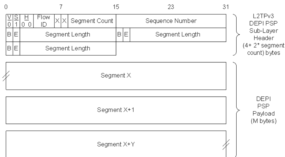
Figure 55 - DEPI Legacy PSP Sublayer Header and Payload
