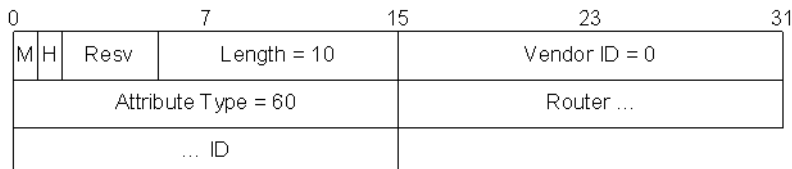
Figure 24 - Router ID AVP
