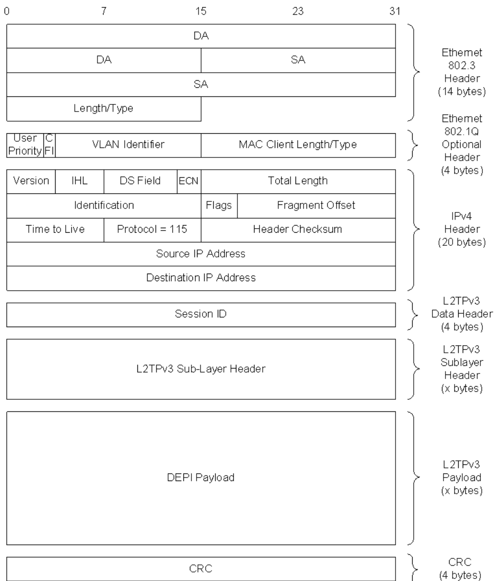
Figure 51 - L2TPv3 Data Packet Outer Encapsulation (without UDP)
