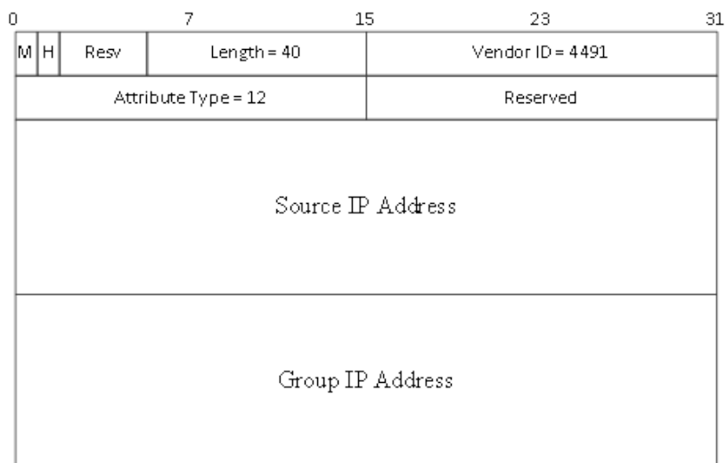
Figure 43 - DEPI Remote Multicast Leave AVP
