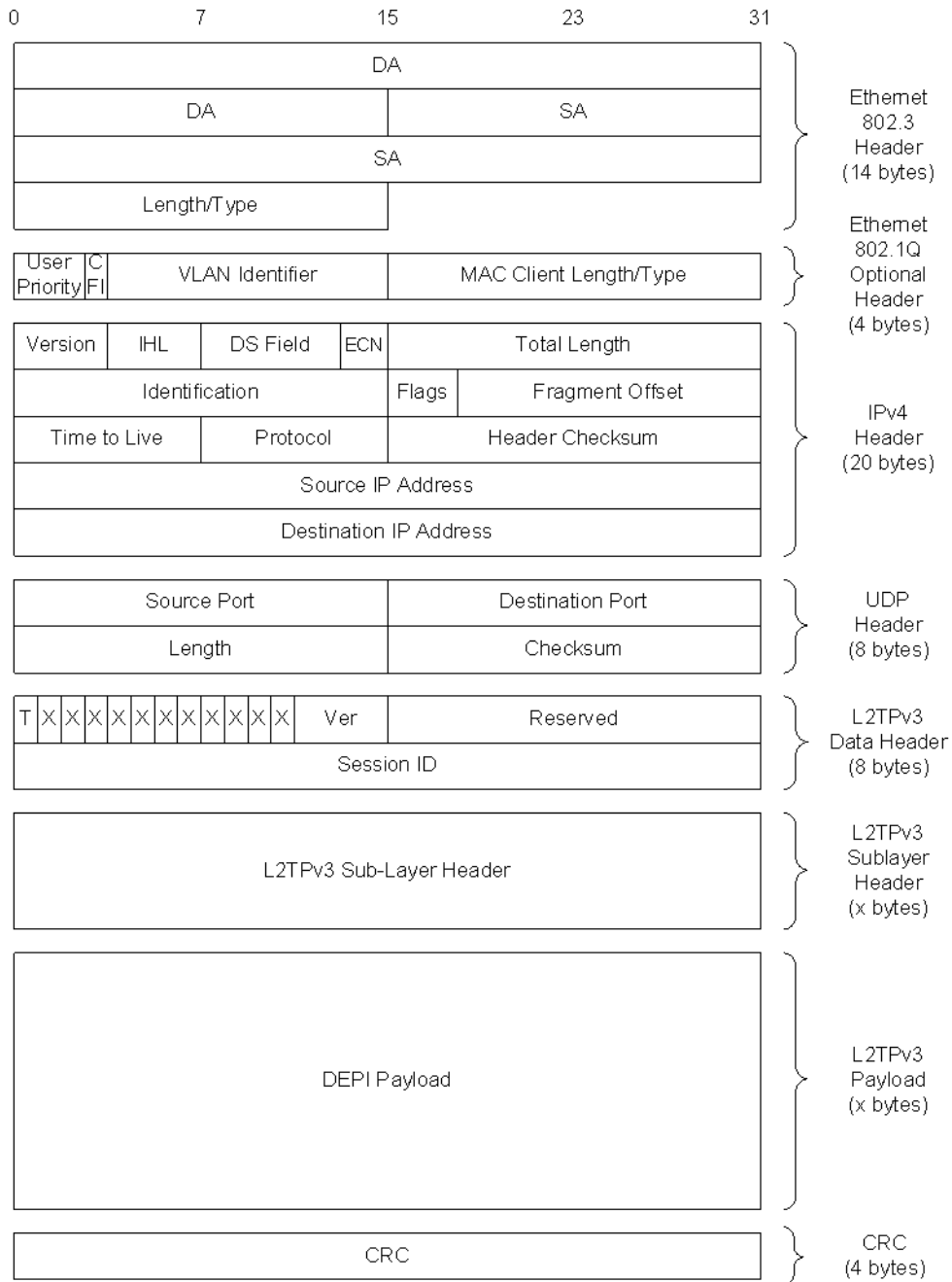
Figure 52 - L2TPv3 Data Packet Outer Encapsulation with UDP Header
