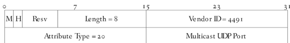
Figure 50 - DEPI Multicast UDP Port AVP
