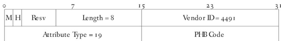
Figure 49 - DEPI S-BFD Return Path DSCP AVP
