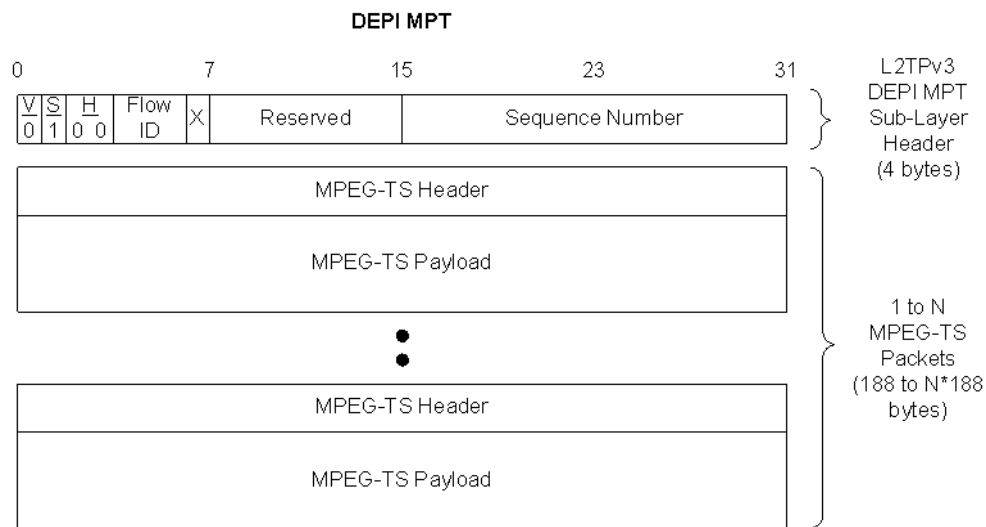
Figure 53 - DEPI MPT Sublayer Header and Payload
