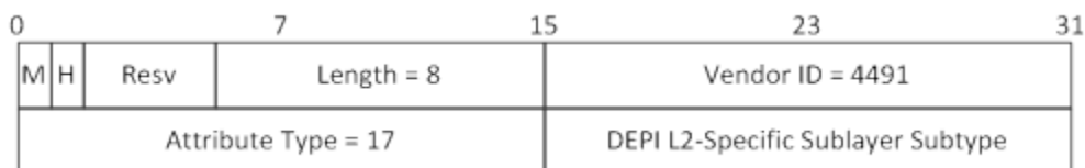
Figure 47 - DEPI L2-Specific Sublayer Subtype AVP
