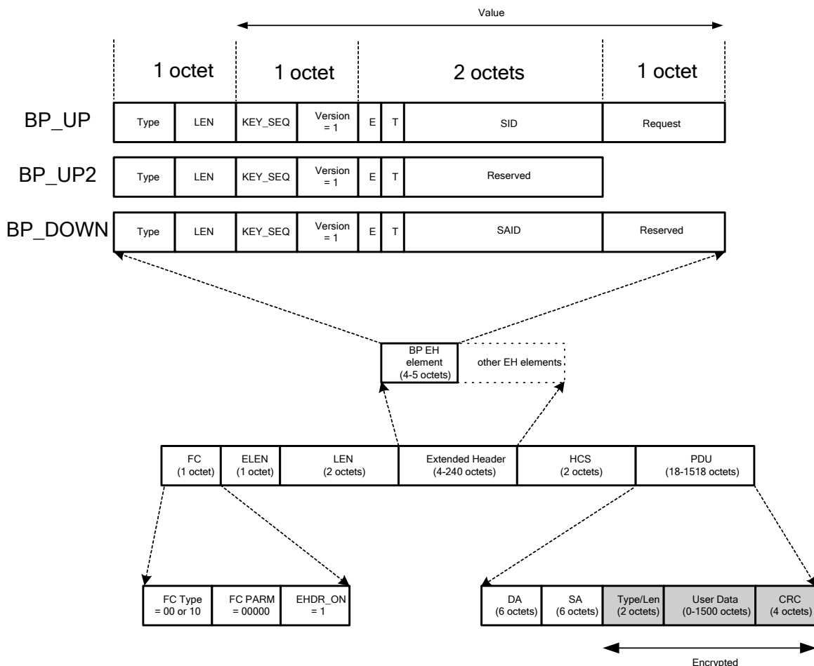
Figure 6-1 - Format of DOCSIS Variable-length PDU with Privacy EH Element 20
