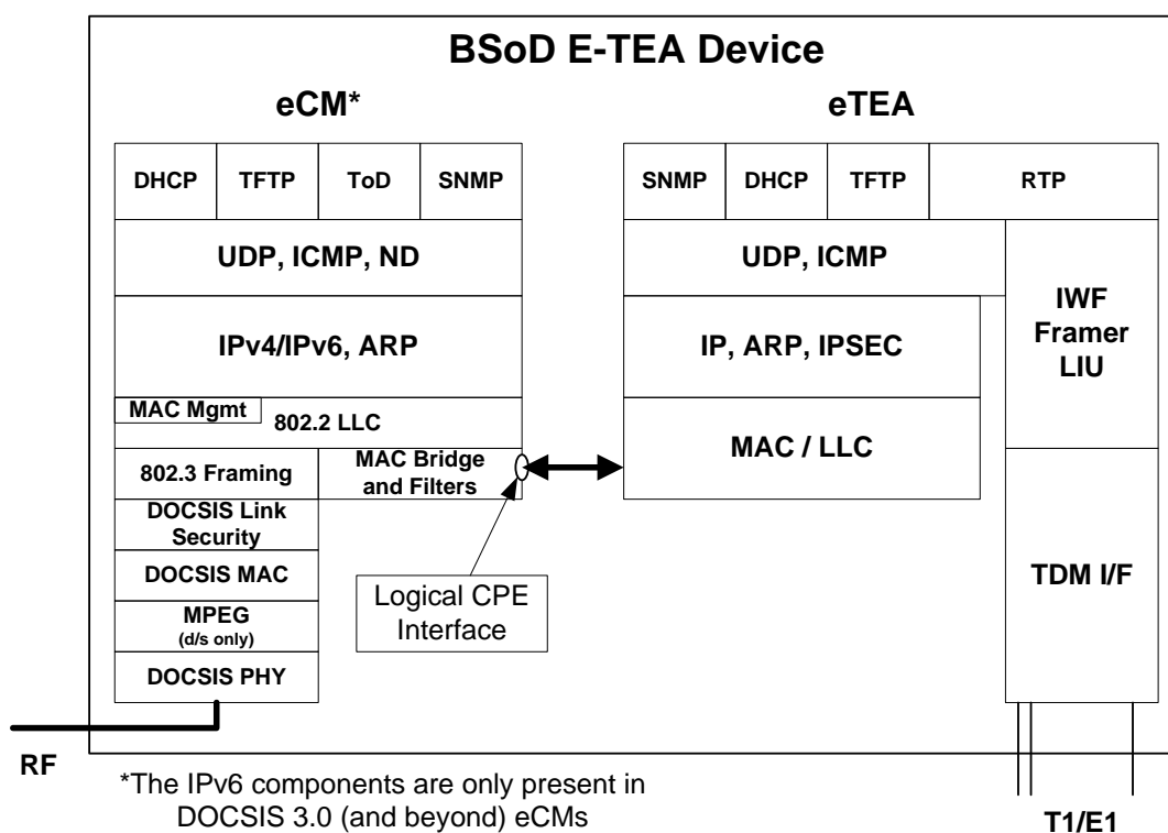
Figure 5–14 - eCM - eTEA Protocol Stacks 16
