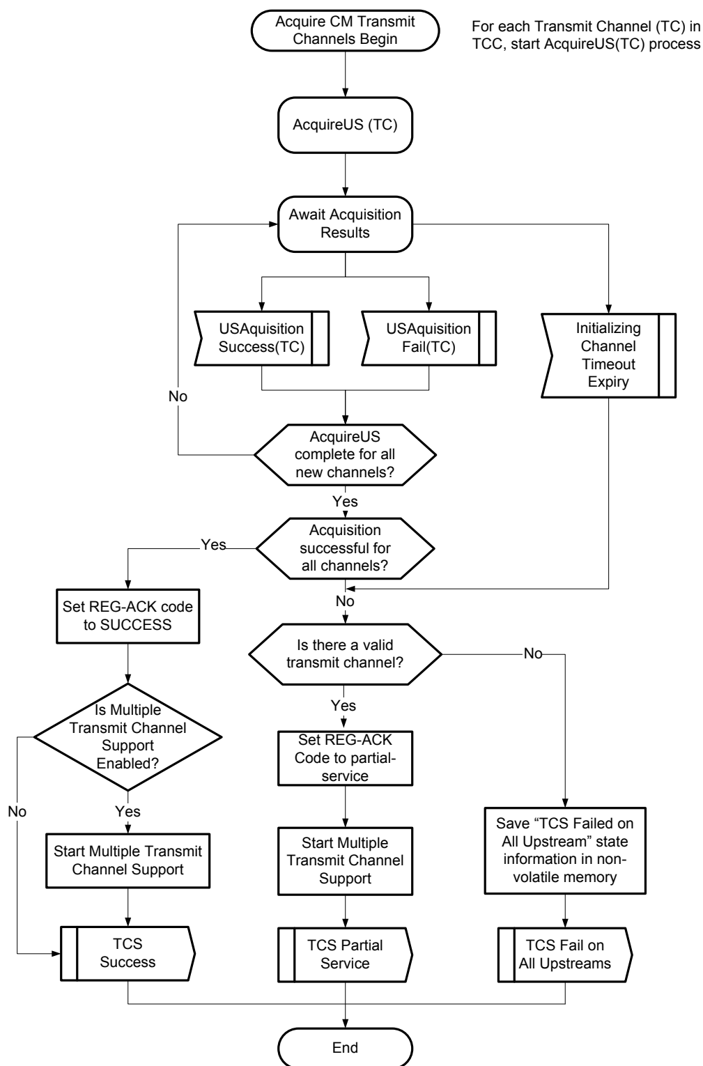
Figure 10–28 - CM Acquires Transmit Channels 324
