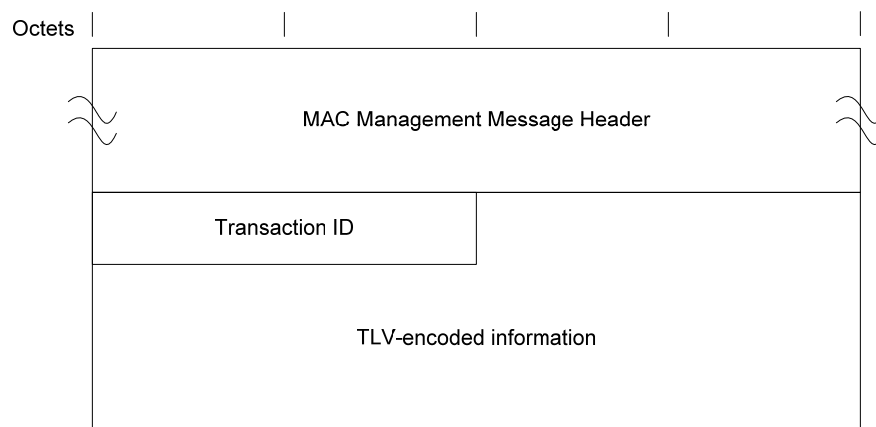
Figure 6–55 - CM-CTRL-REQ 160
