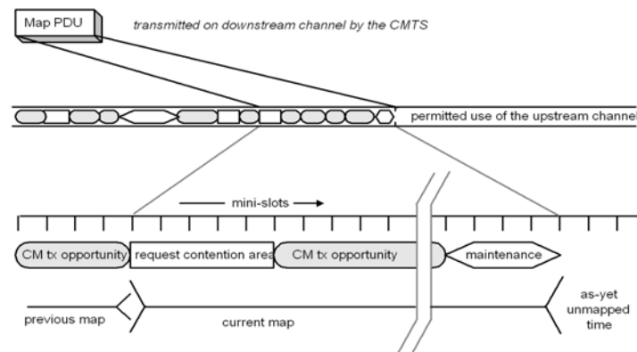
Figure 7–1 - Allocation Map
