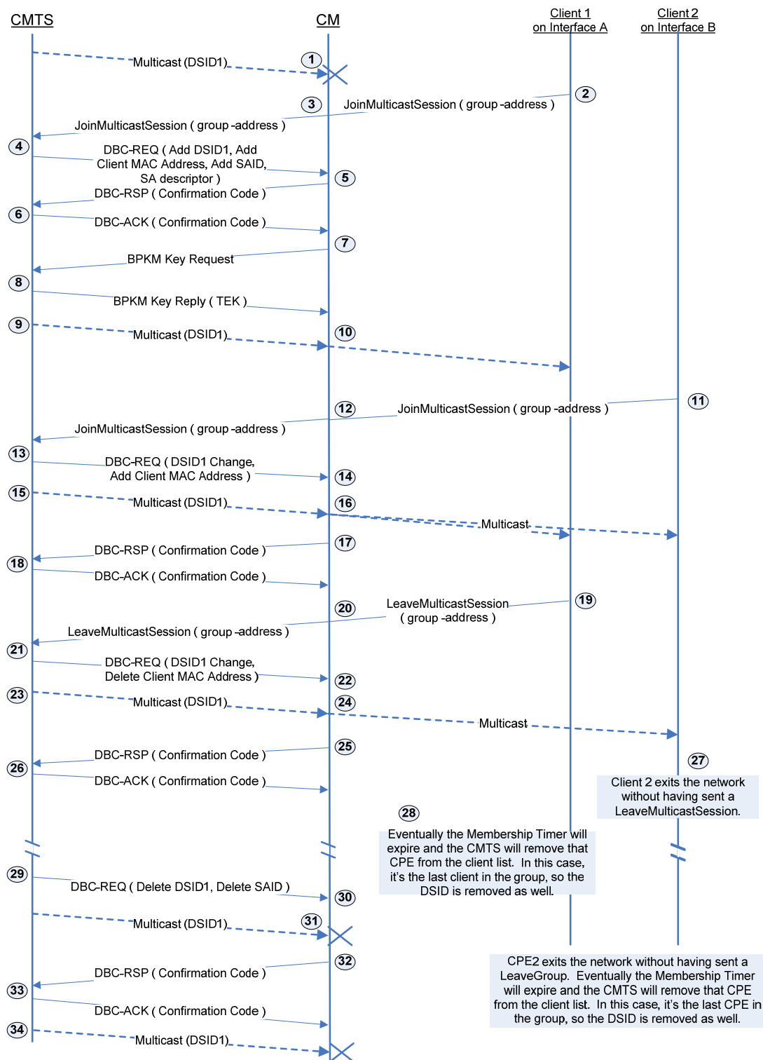
Figure 9-5 - Example: Encrypted Downstream Multicast Forwarding 272
