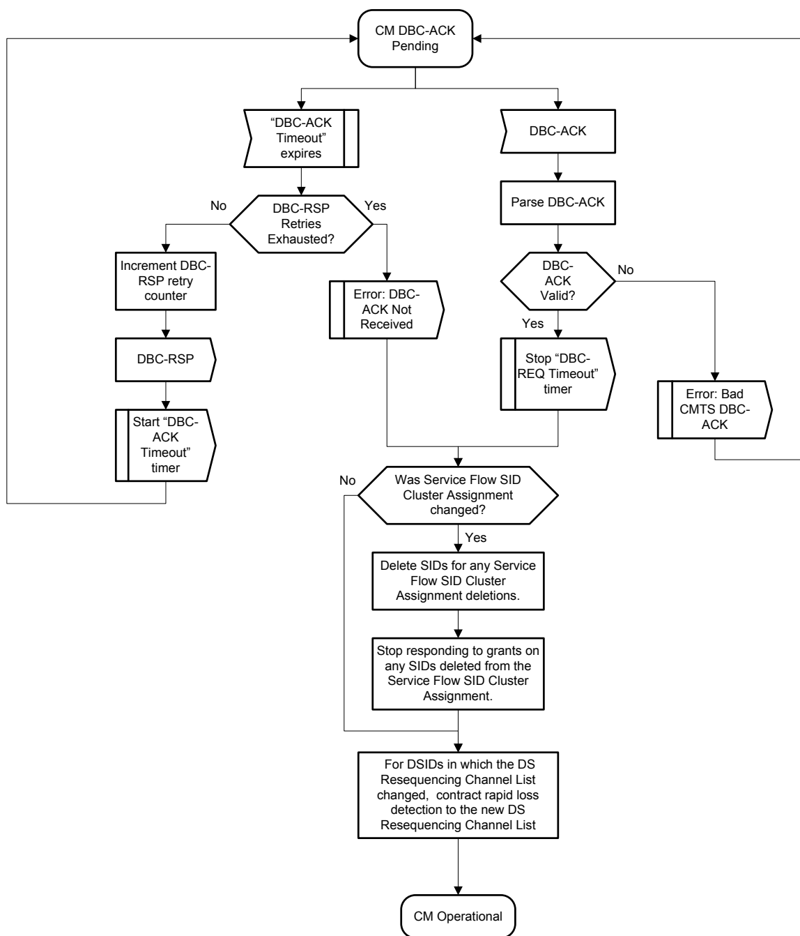
Figure 11–59 - CM DBC-ACK Pending 398
