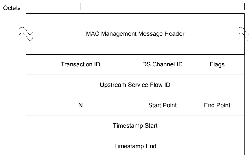
Figure 6–53 - DPV-RSP MAC Message 154
