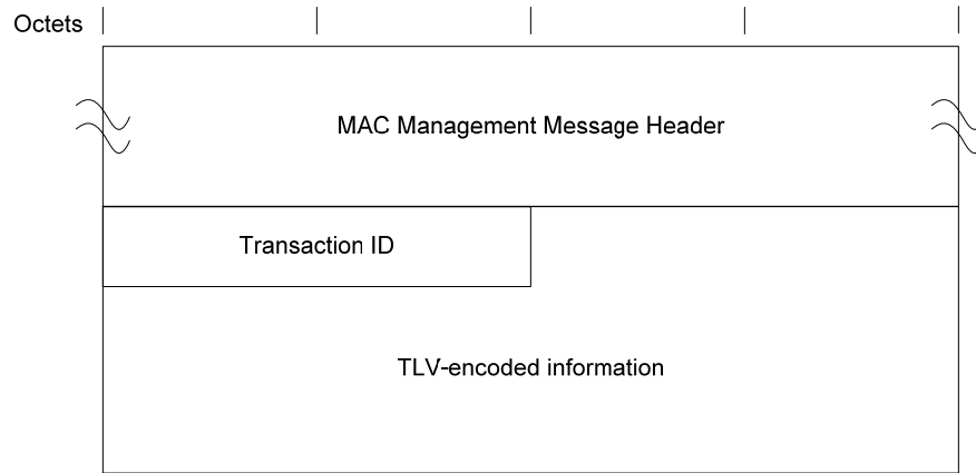
Figure 6–43 - Dynamic Channel Change Acknowledge 119
