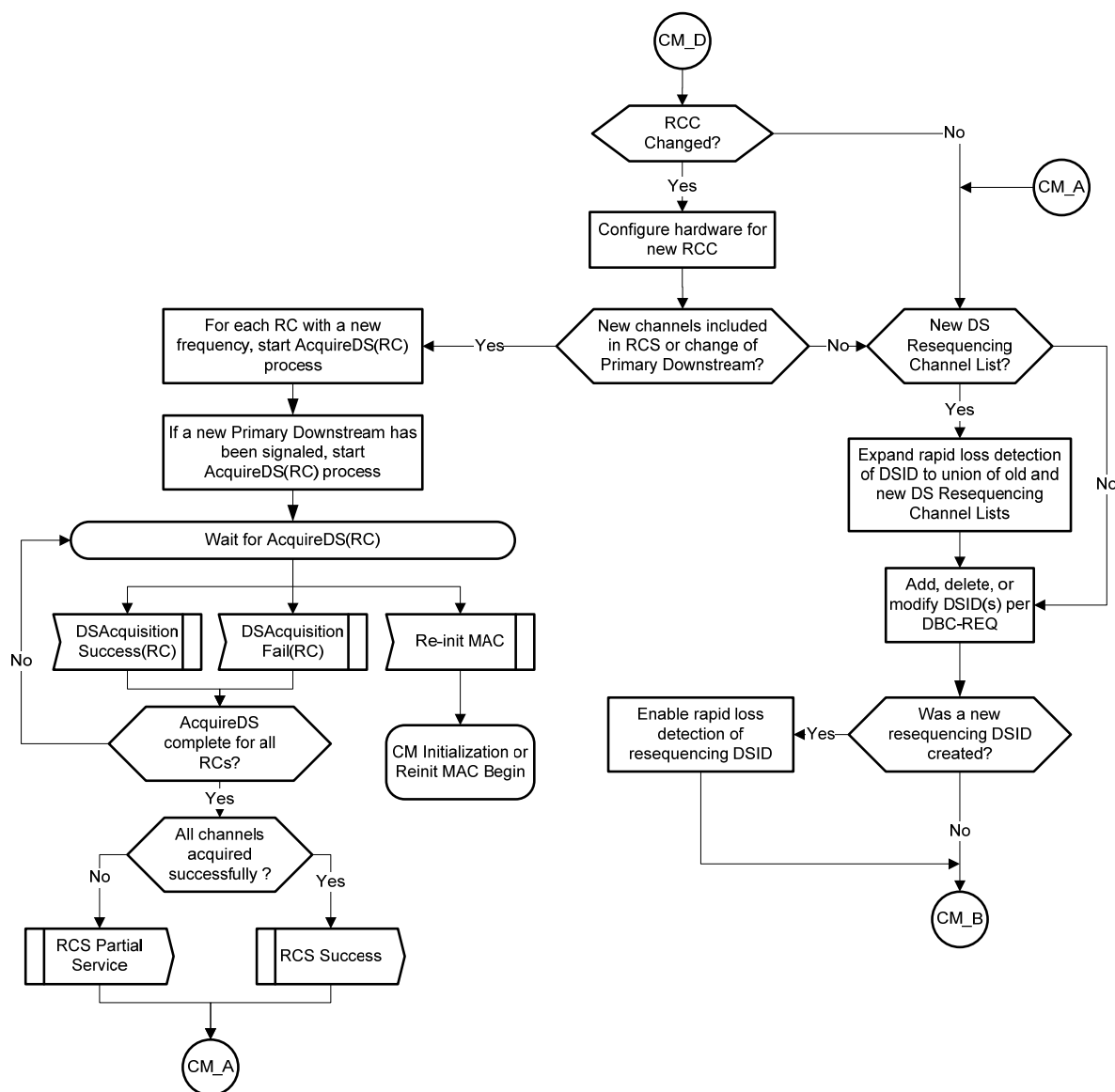
Figure 11-55 - CM DBC-RSP (part 2) 394
