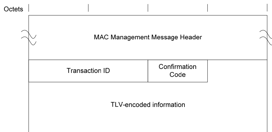
Figure 6–37 - Dynamic Service Change — Response 109
