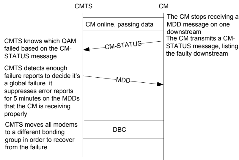
Figure V-2 - Example 2 - Option 4 637
