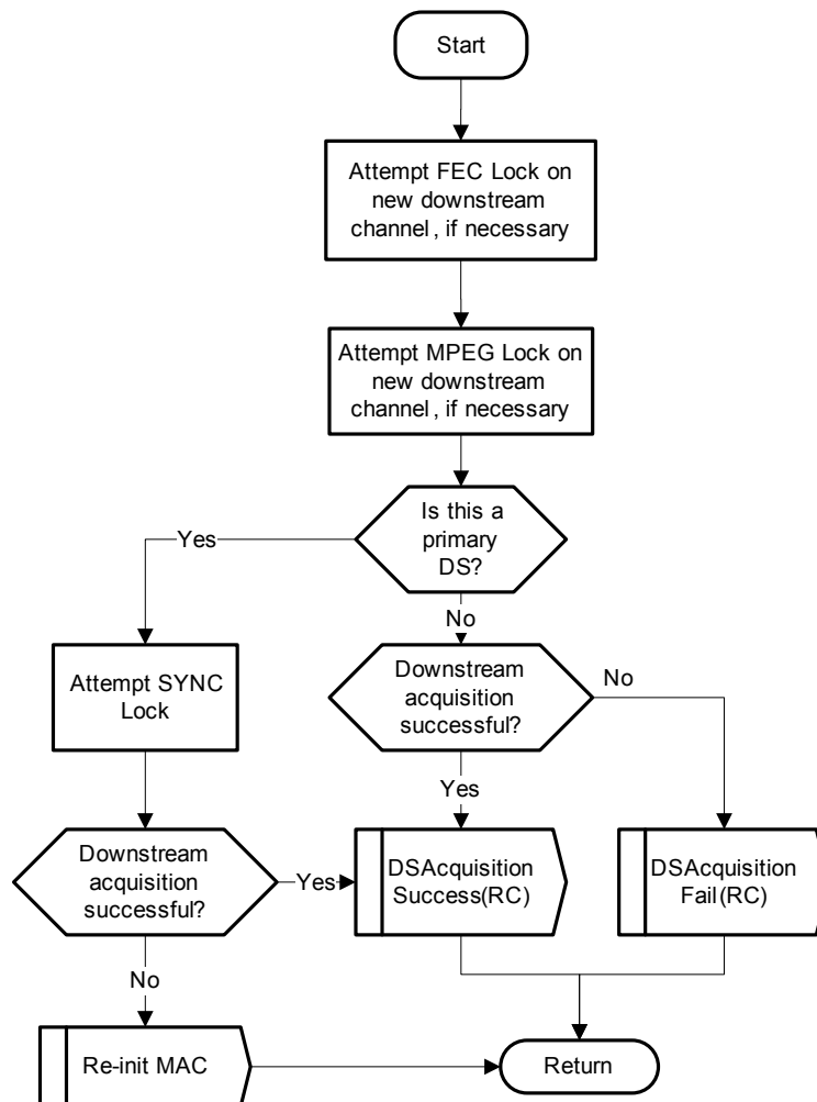
Figure 11-57 - CM AcquireDS Procedure 396
