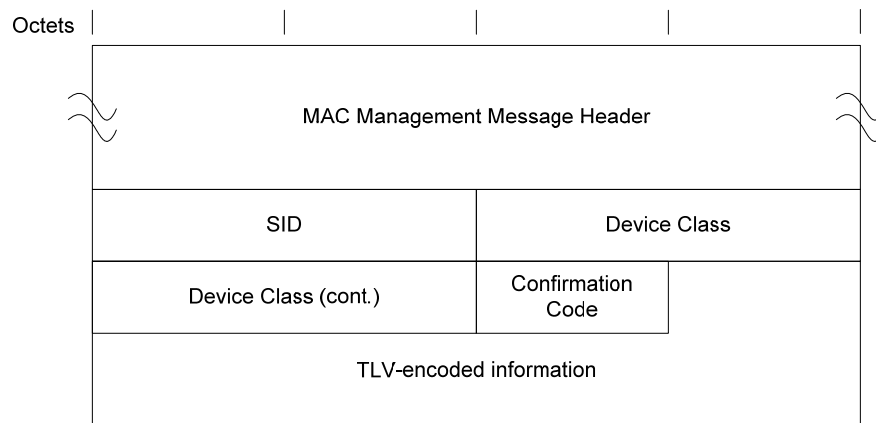
Figure 6-45 - Device Class Identification Response 121
