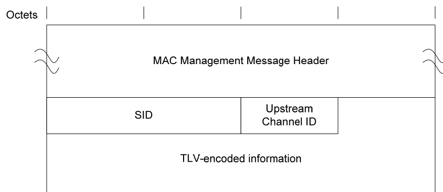
Figure 6–23 - Ranging Response 73
