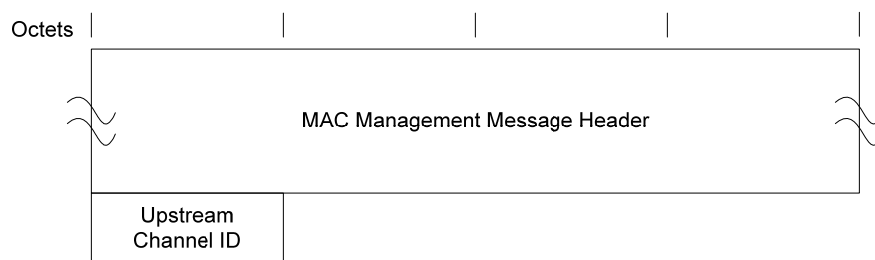
Figure 6–31 - Upstream Channel Change Request 100
