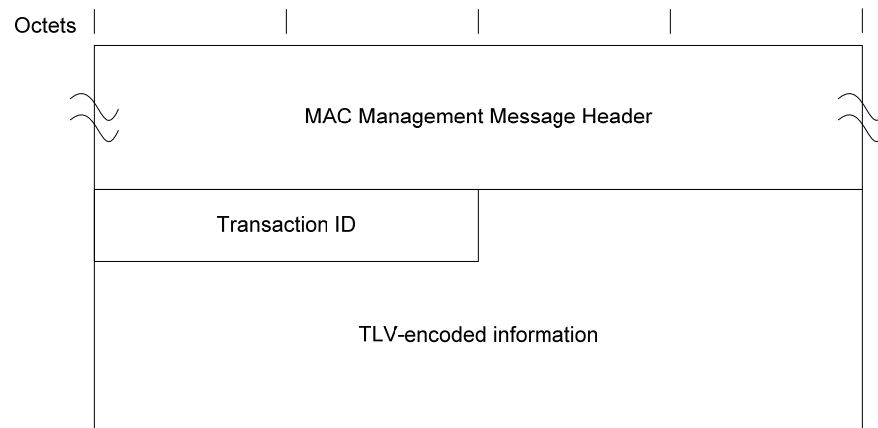
Figure 6-56 - CM-CTRL-RSP 163
