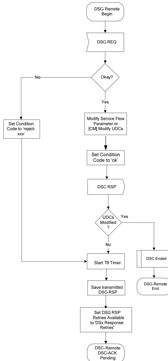
Figure 11–28 - DSC—Remotely Initiated Transaction Begin State Flow Diagram 362
