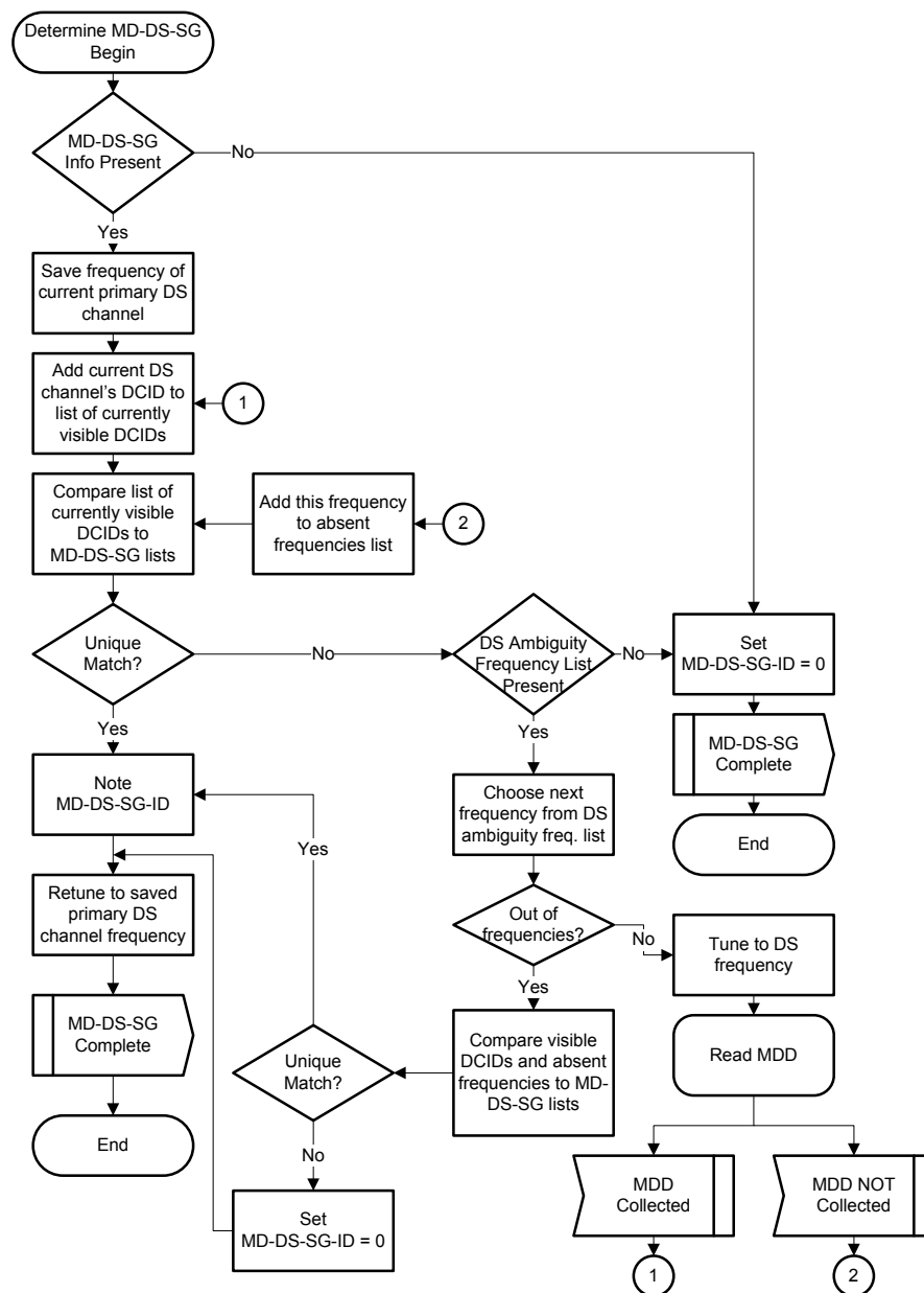
Figure 10–4 - Determine MD-DS-SG
