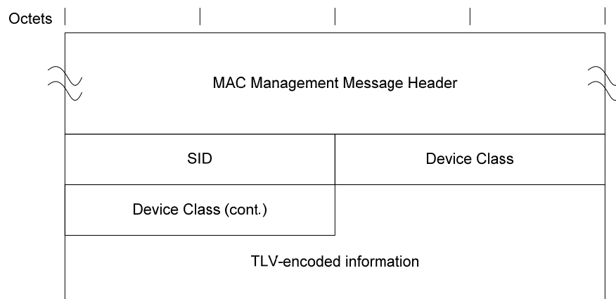
Figure 6-44 - Device Class Identification Request 120
