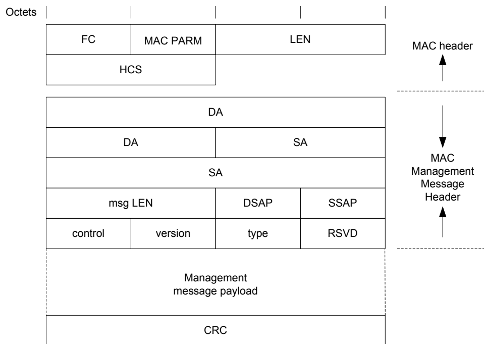
Figure 6–13 - MAC Header and MAC Management Message Header Fields 47
