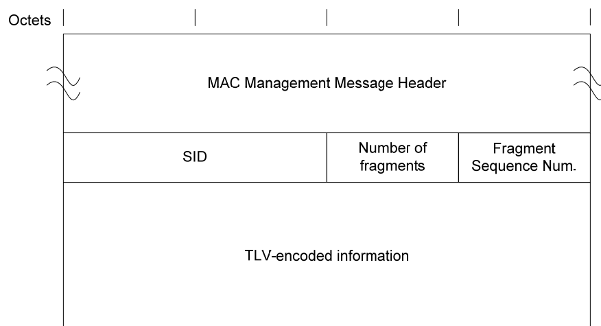
Figure 6–27 - Multipart Registration Request (REG-REQ-MP) 90
