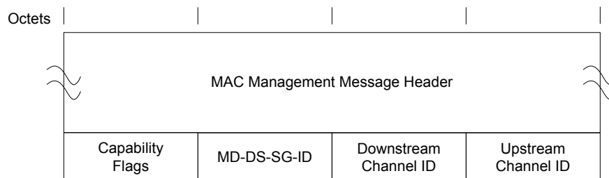
Figure 6–22 - B-INIT-RNG-REQ Format 72
