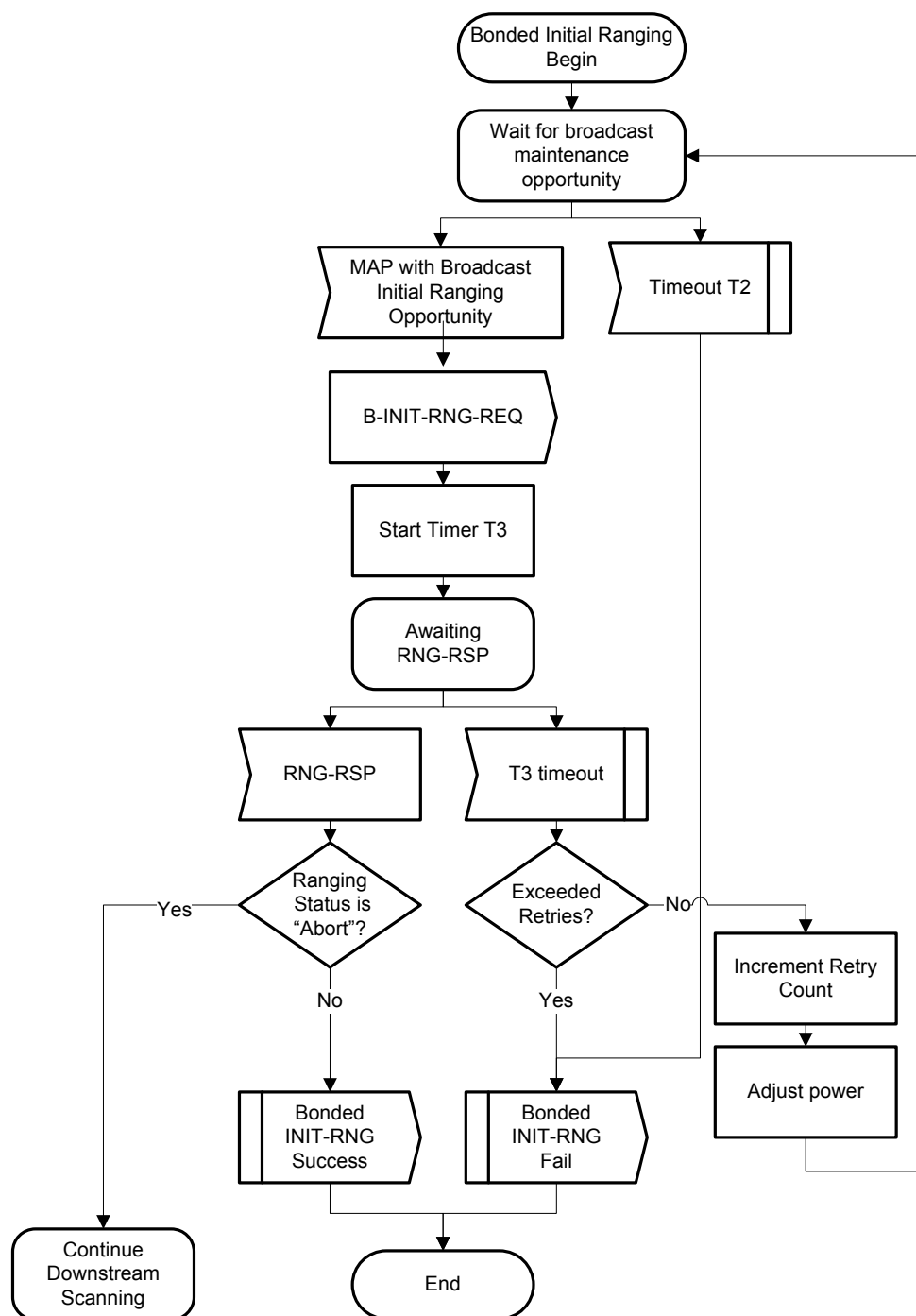
Figure 10–7 - Bonded Initial Ranging 288
