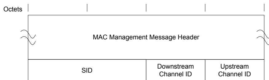
Figure 6–21 - INIT-RNG-REQ Format 69
