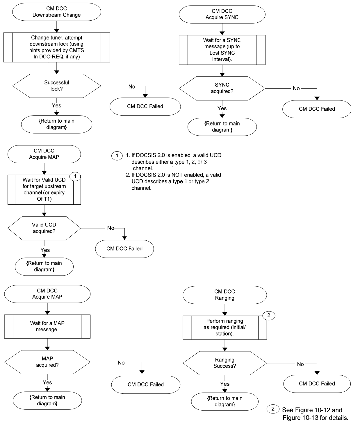
Figure 11–48 - Dynamically Changing Channels: CM View Part 3 372
