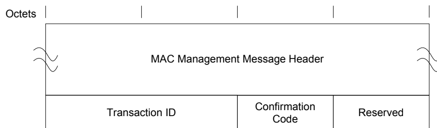
Figure 6–40 - Dynamic Service Deletion — Response 113
