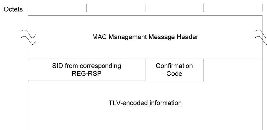
Figure 6–30 - Registration Acknowledgment 99
