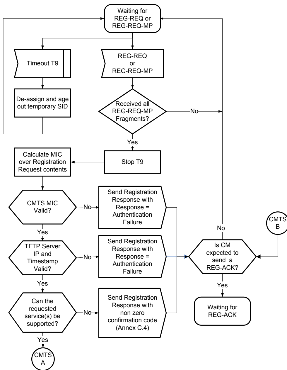
Figure 10–31 - CMTS Registration - Begin 334
