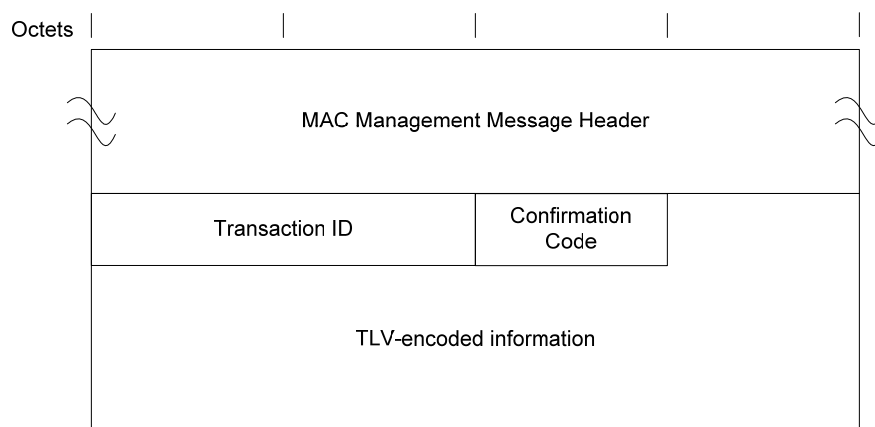
Figure 6–34 - Dynamic Service Addition — Response 103
