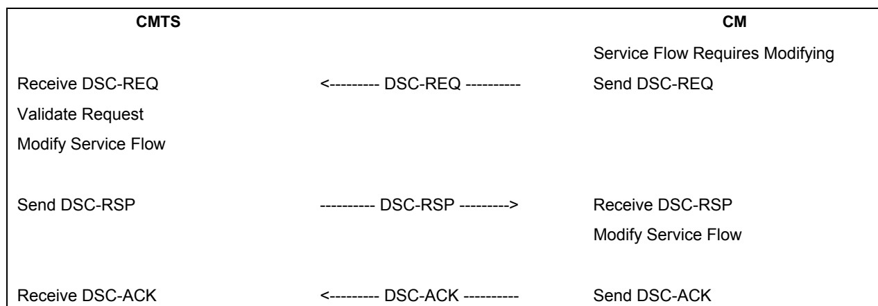
Figure 11–20 - CM-Initiated DSC
