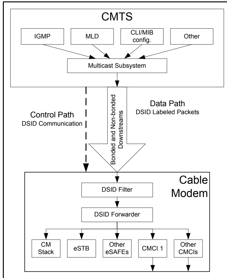
Figure 9-2 - Multicast Model
