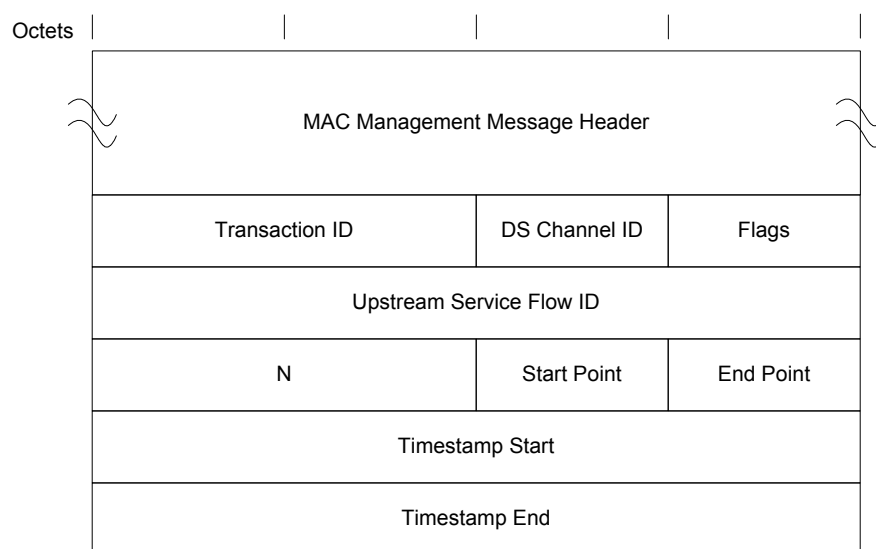
Figure 6–52 - DPV-REQ MAC Message 152
