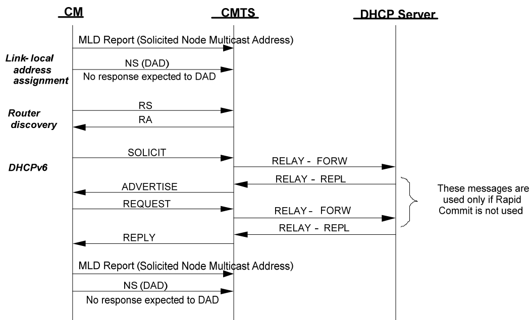
Figure 10–24 - IPv6 Provisioning Message Flow
