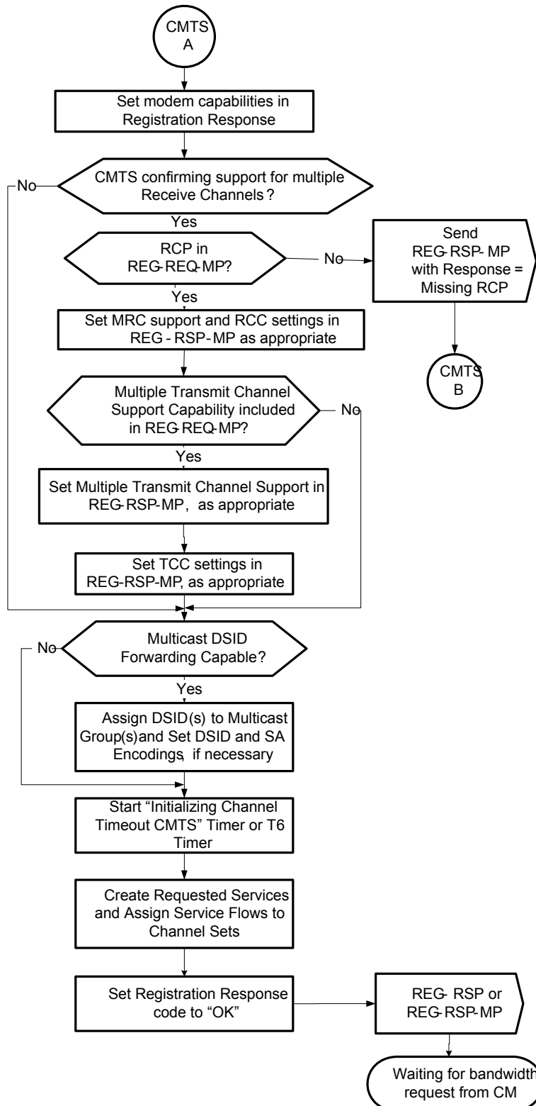
Figure 10–32 - CMTS Registration - Continued 335
