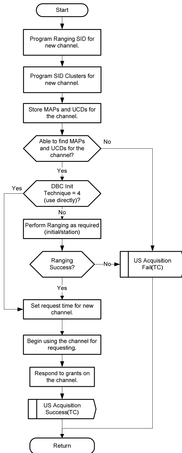
Figure 11–58 - CM AcquireUS Procedure 397
