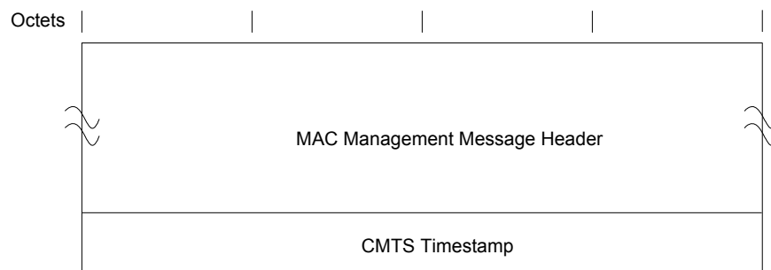
Figure 6–14 - Format of Packet PDU Following the Timing Header 49
