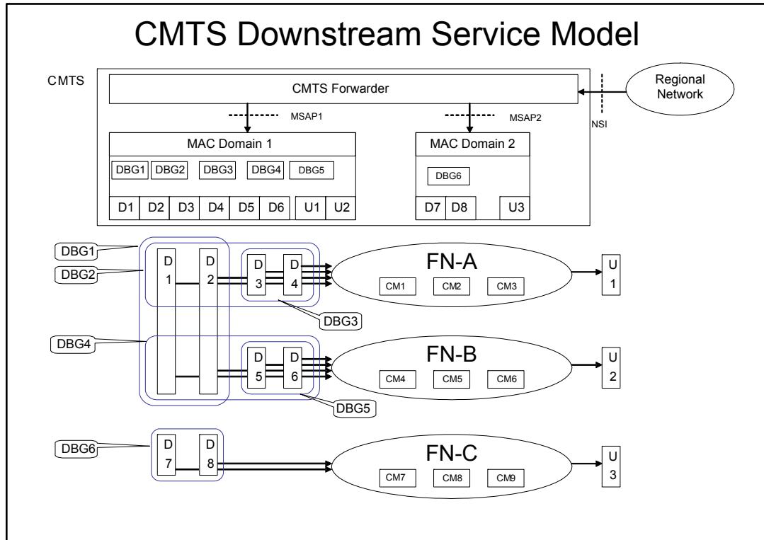
Figure 5–11 - CMTS Downstream Service Model
