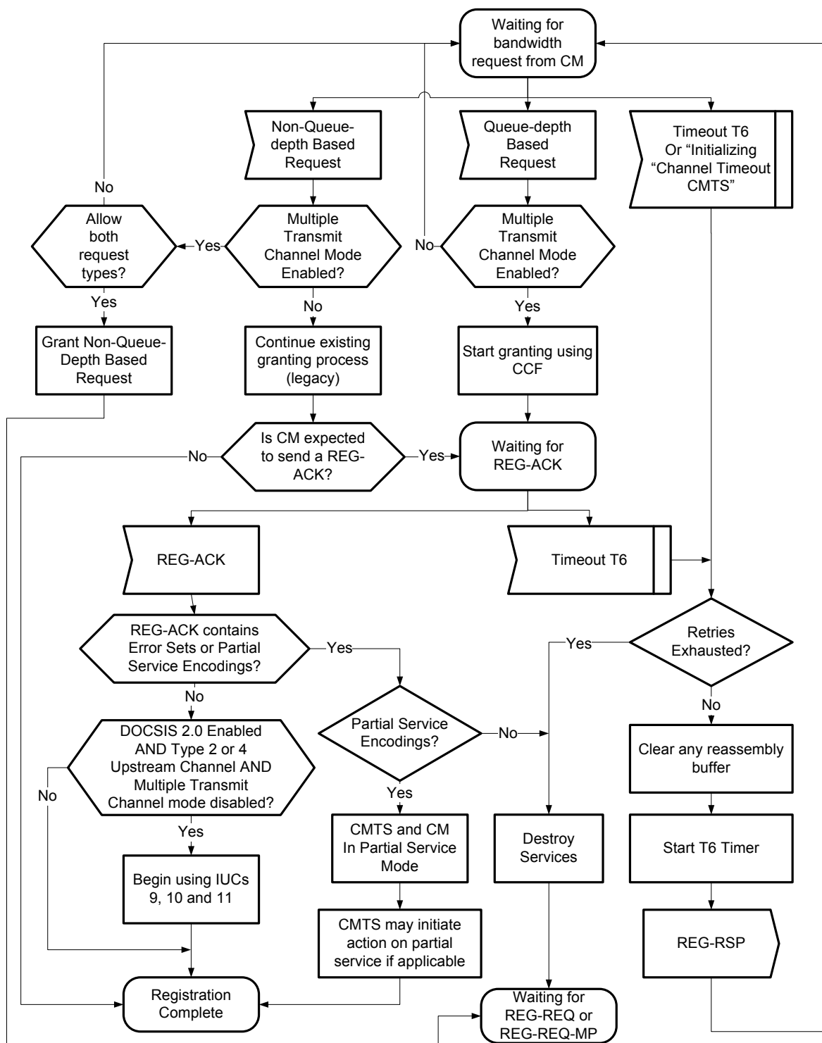
Figure 10-33 - CMTS Registration - End 336
