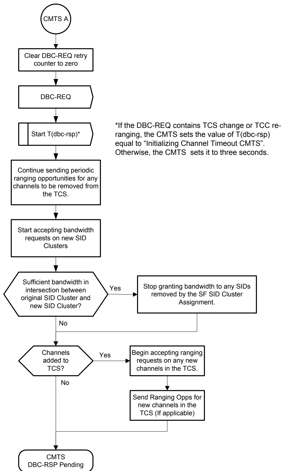
Figure 11-51 - CMTS DBC Request (part 2) 390
