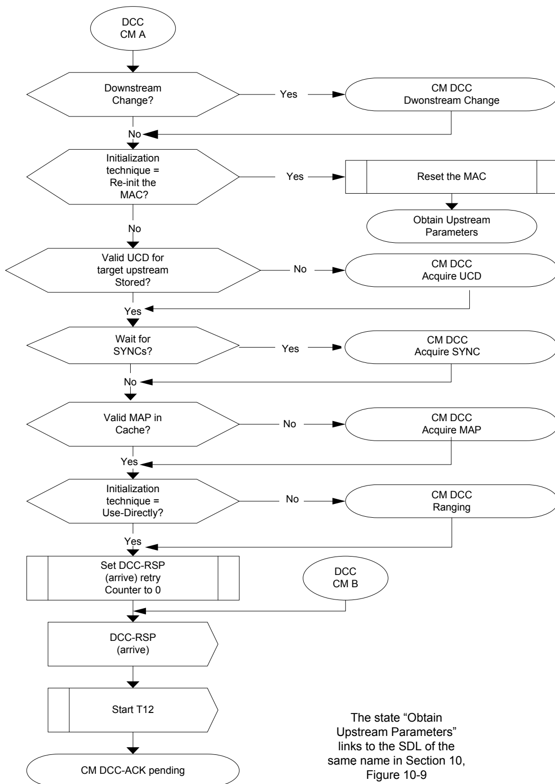
Figure 11–47 - Dynamically Changing Channels: CM View Part 2 371
