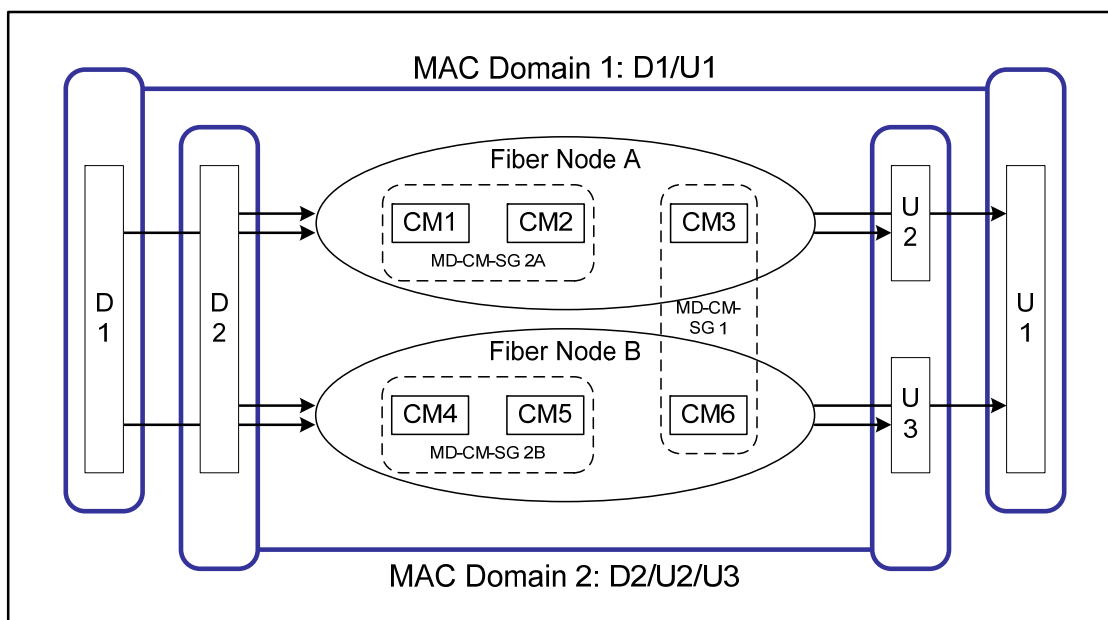
Figure 5–9 - Multiple MAC Domains per Fiber Node 22
