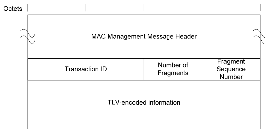
Figure 6–49 - Dynamic Bonding Change Request Message 145
