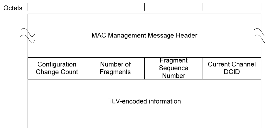
Figure 6–48 - MAC Domain Descriptor 125
