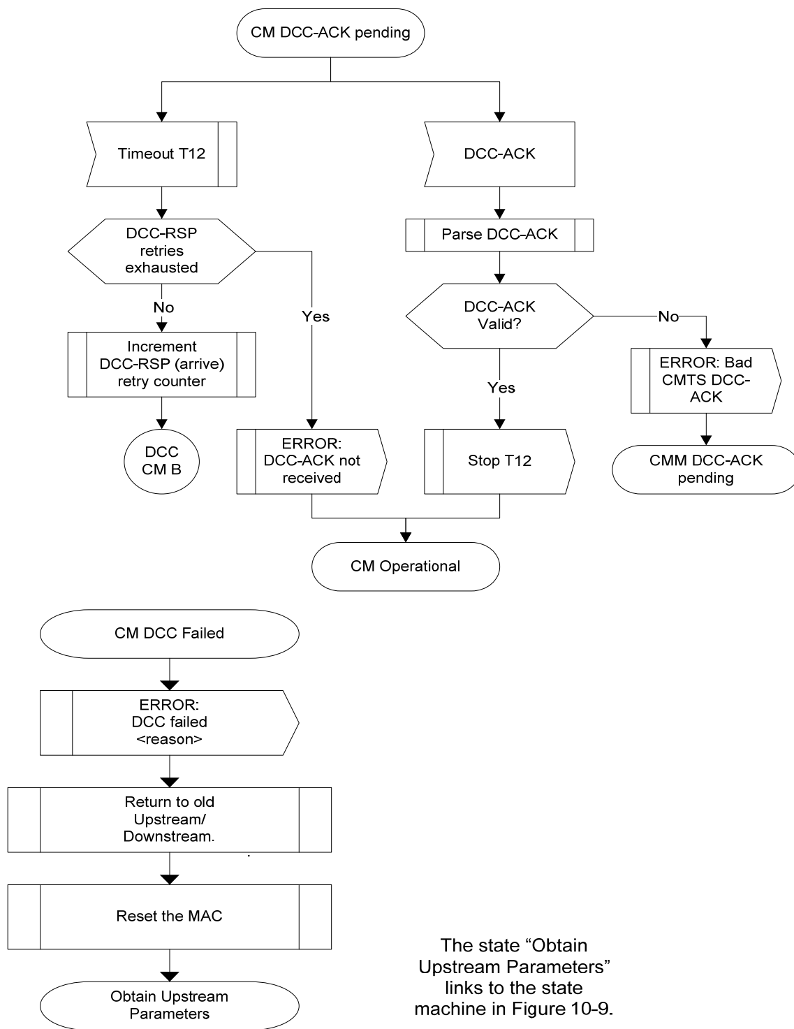
Figure 11–49 - Dynamically Changing Channels: CM View Part 4 373
