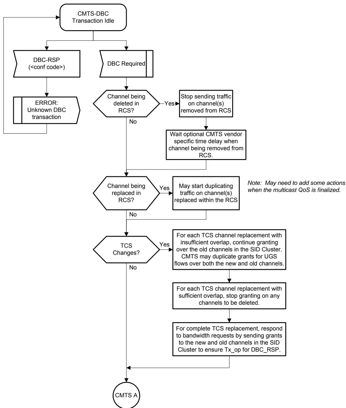
Figure 11–50 - CMTS DBC Request (part 1) 389
