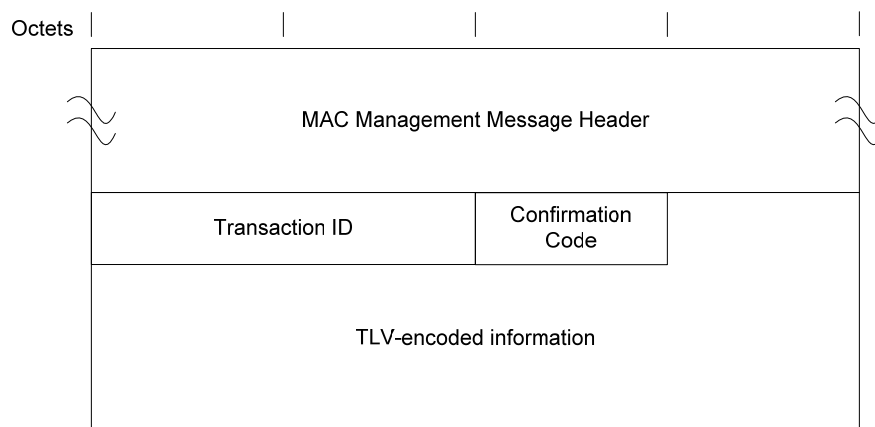
Figure 6–50 - Dynamic Bonding Change Response Message 149
