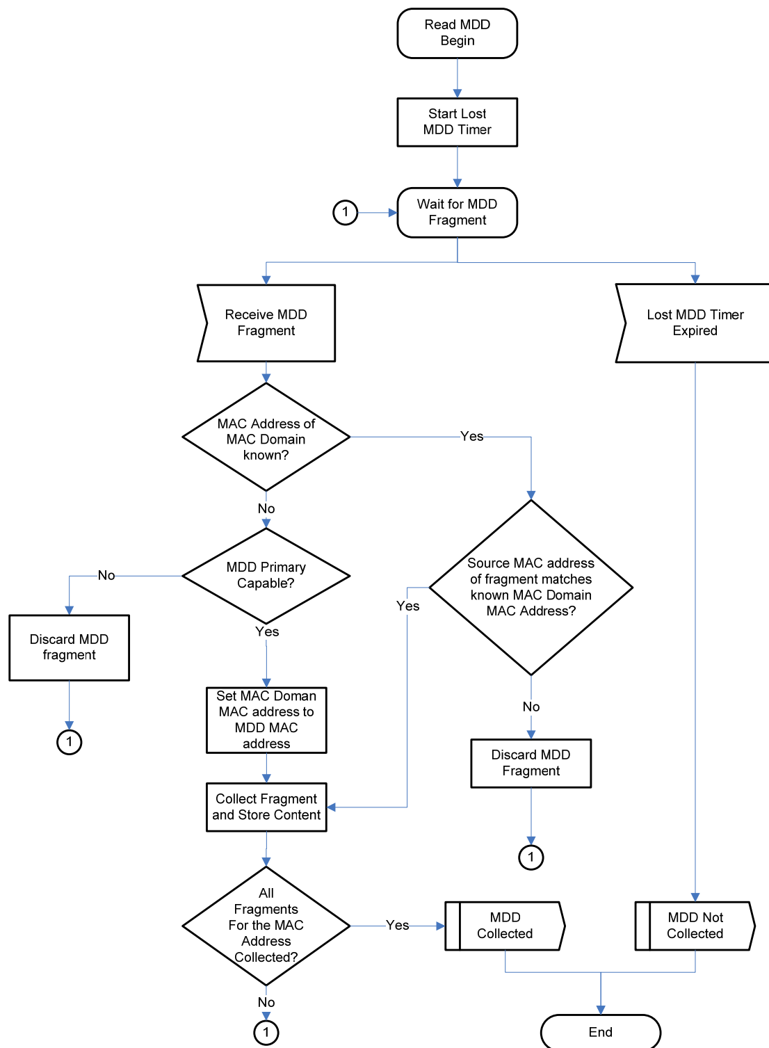
Figure 10–3 - Read MAC Domain Descriptor (MDD) 283
