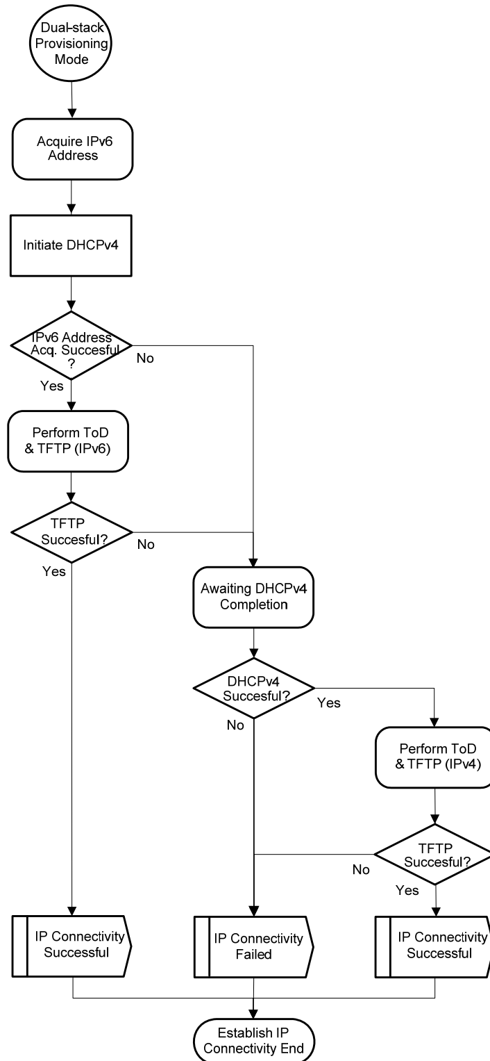
Figure 10–20 - Dual-stack Provisioning Mode 296
