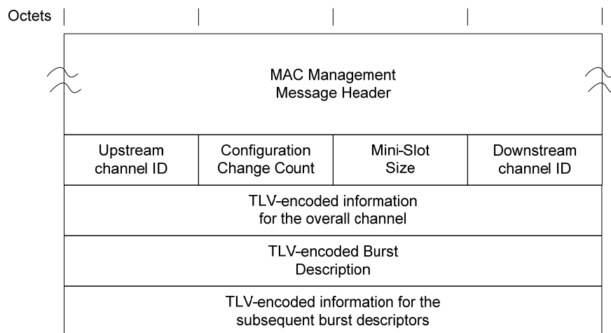
Figure 6–15 - Upstream Channel Descriptor 53
