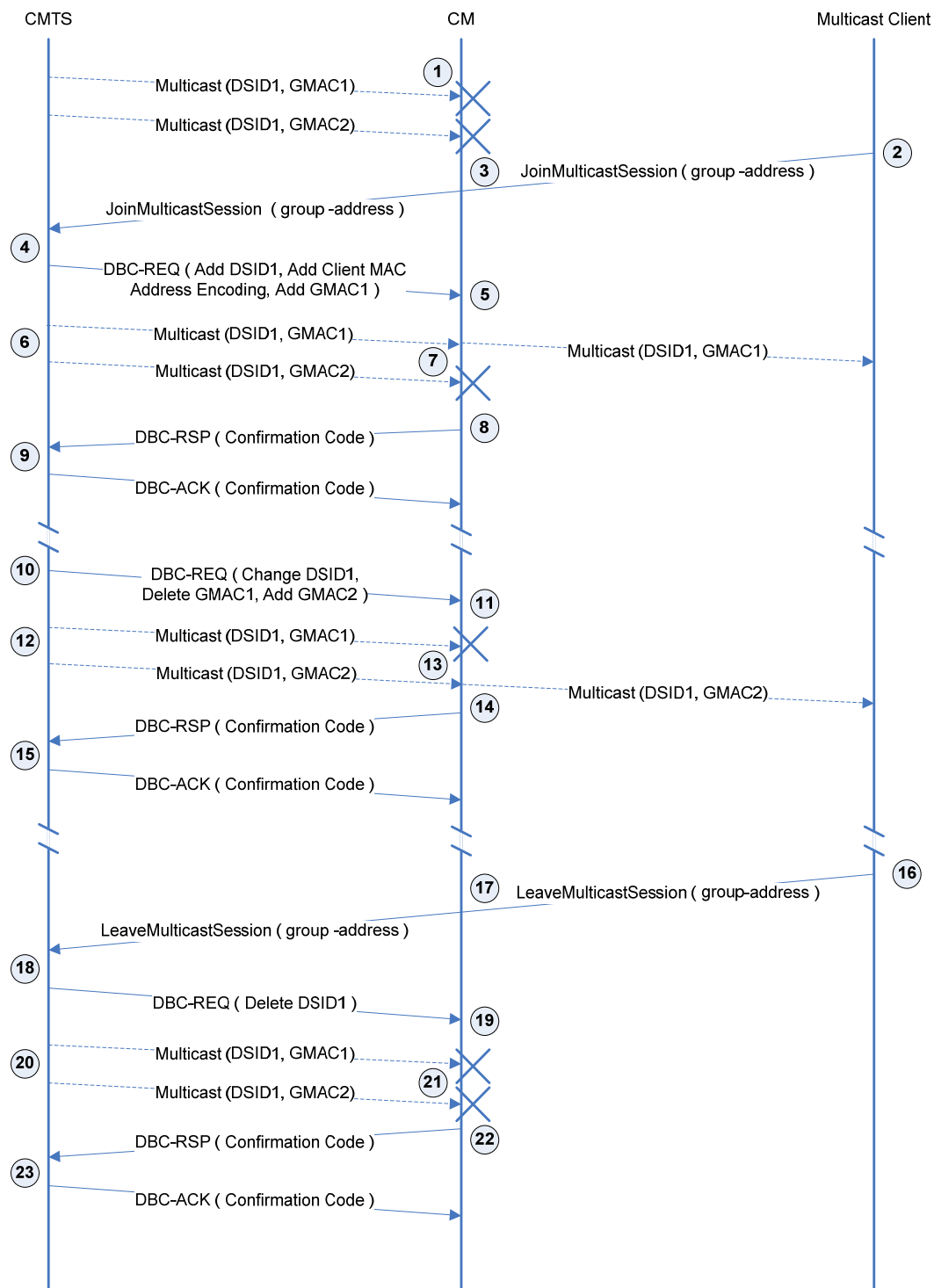
Figure G-1- Multicast Forwarding by a GMAC-Explicit CM 617
