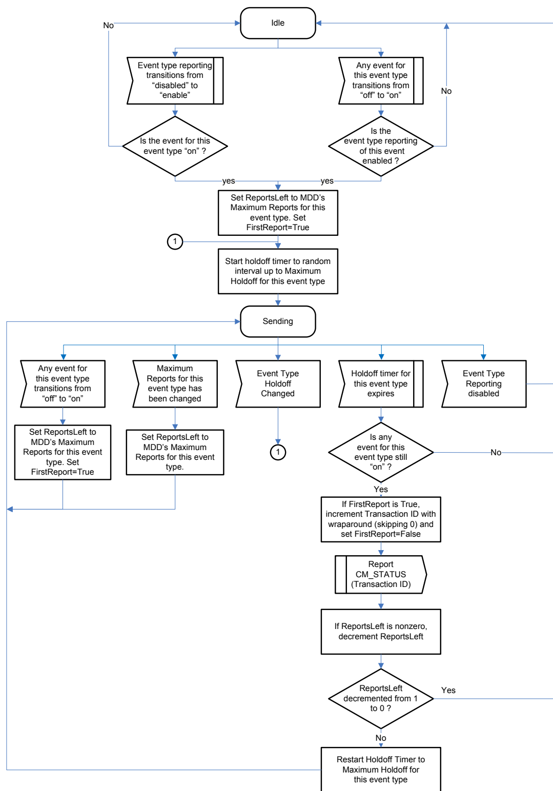
Figure 10-36 - CM-STATUS Event Type State Machine 350
