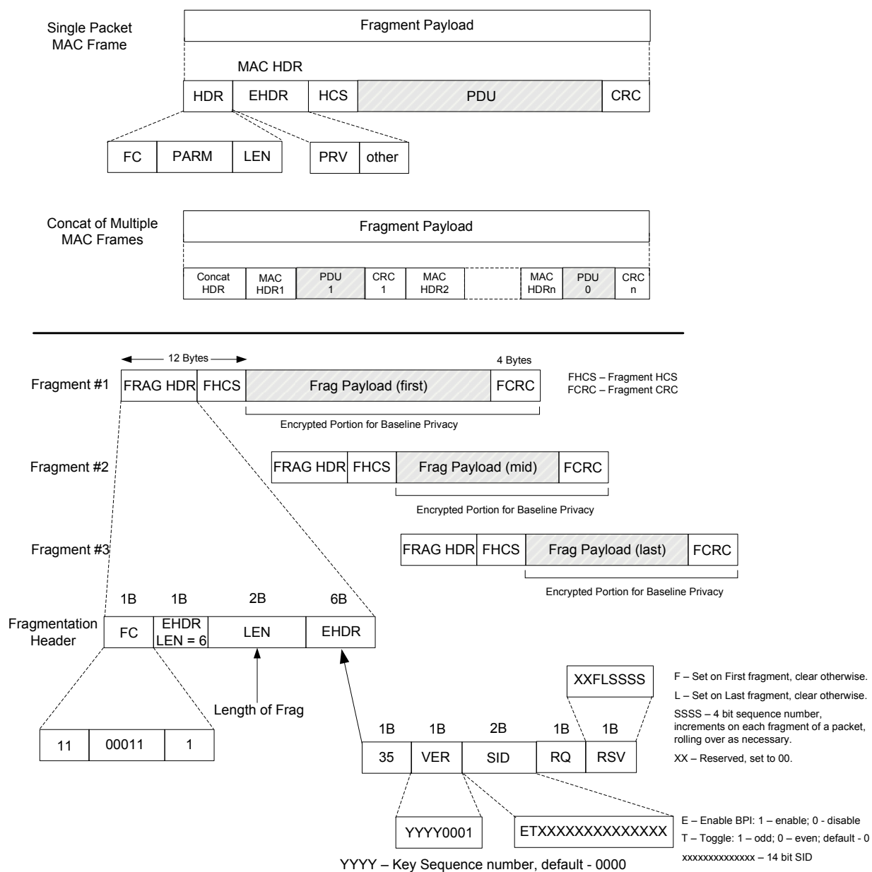
Figure 7-6 - Fragmentation Details 191
