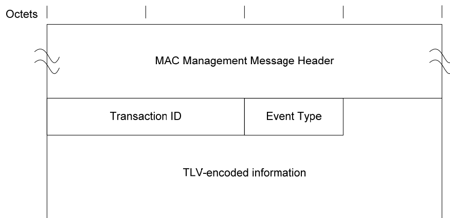
Figure 6–54 - CM-STATUS Report 156
