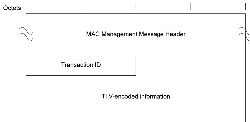
Figure 6–33 - Dynamic Service Addition — Request 102
