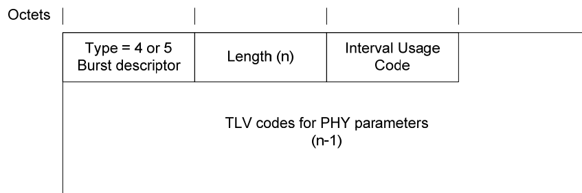
Figure 6–16 - Top-Level Encoding for Burst Descriptors 57
