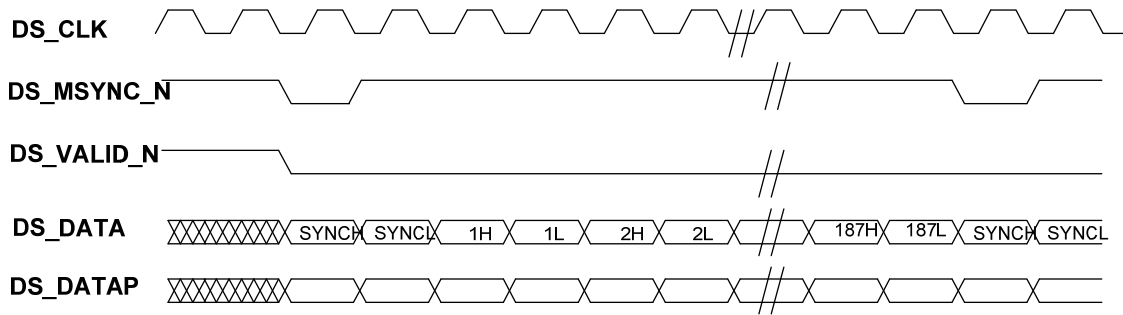
Figure F-3 - Downstream Data Signal Protocol for Annex B Operation
