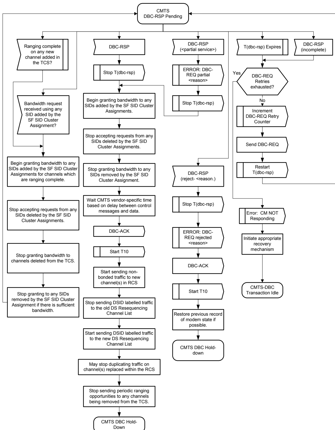
Figure 11-52 - CMTS DBC-RSP Pending 391
