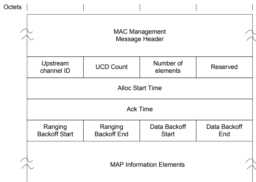
Figure 6–18 - MAP Format 59
