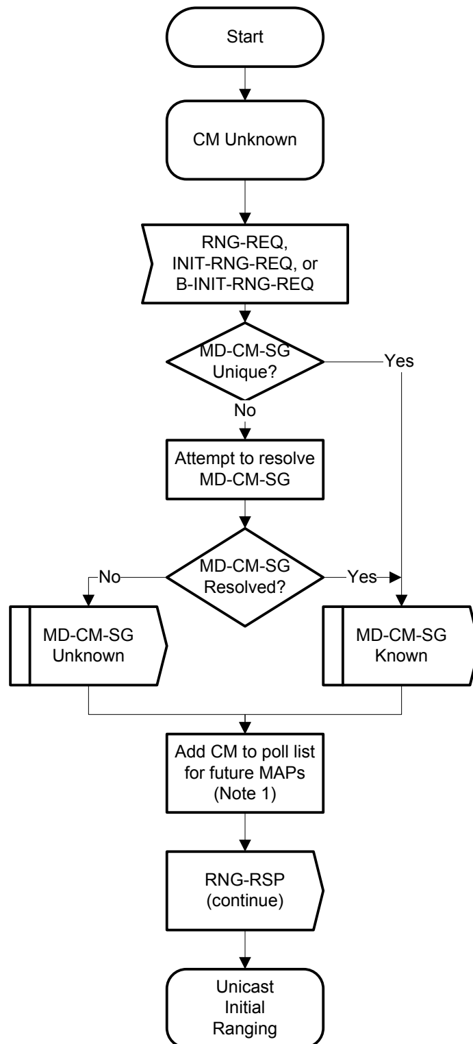
Figure 10–14 - CM-SG Determination - CMTS
