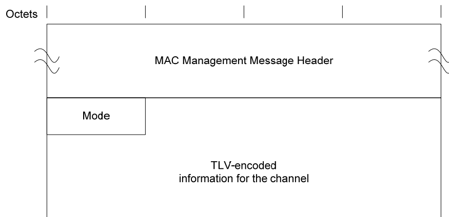
Figure 6–47 - Test Request 123
