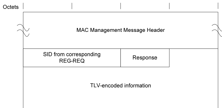
Figure 6–28 - Registration Response Format 92
