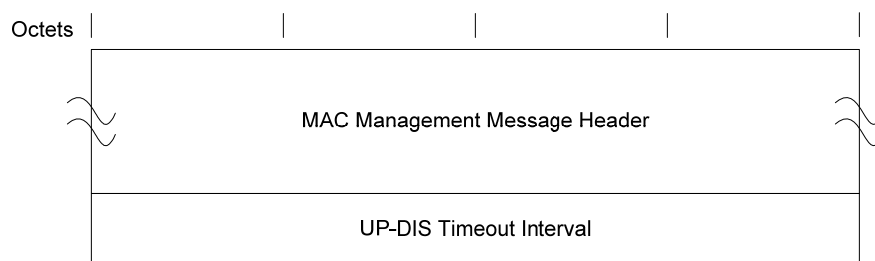
Figure 6–46 - UP-DIS message format 122
