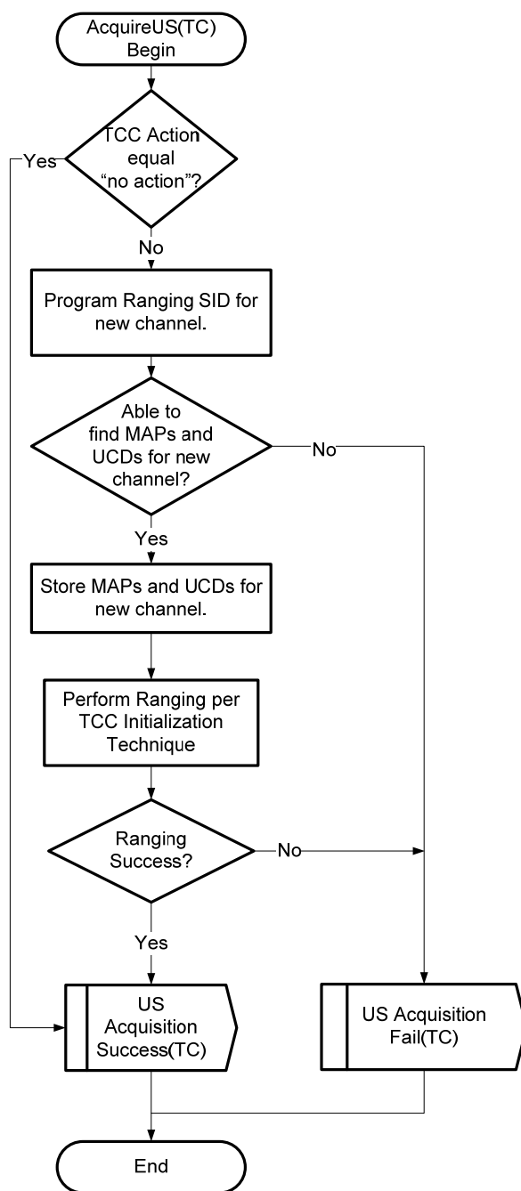
Figure 10-29 - CM Acquires Upstream Channels 325
