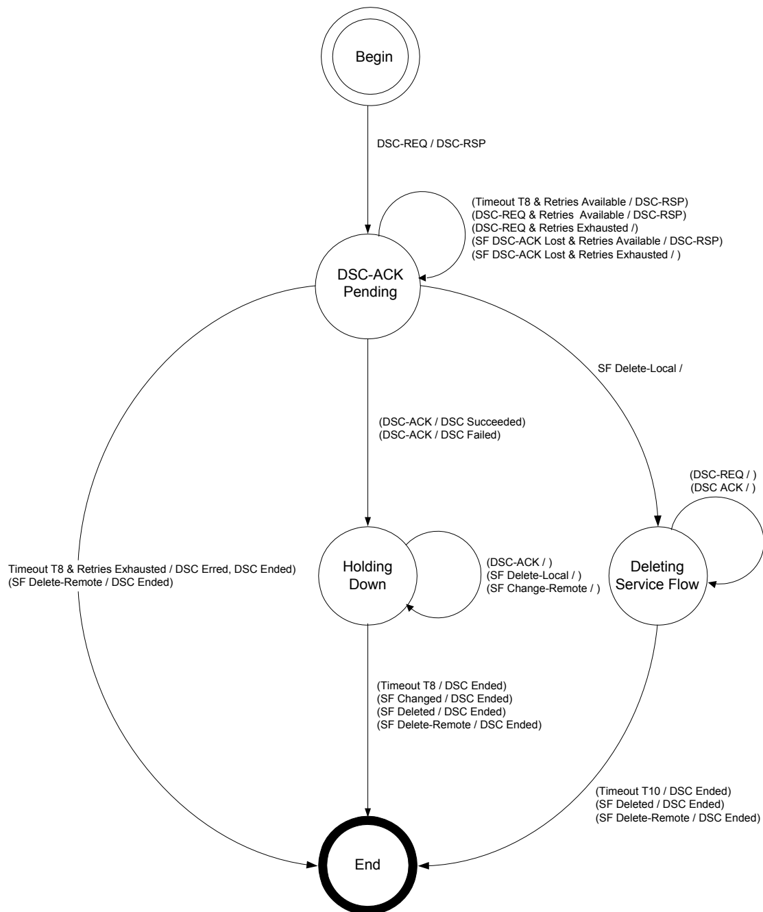
Figure 11–6 - DSC—Remotely Initiated Transaction State Transition Diagram
