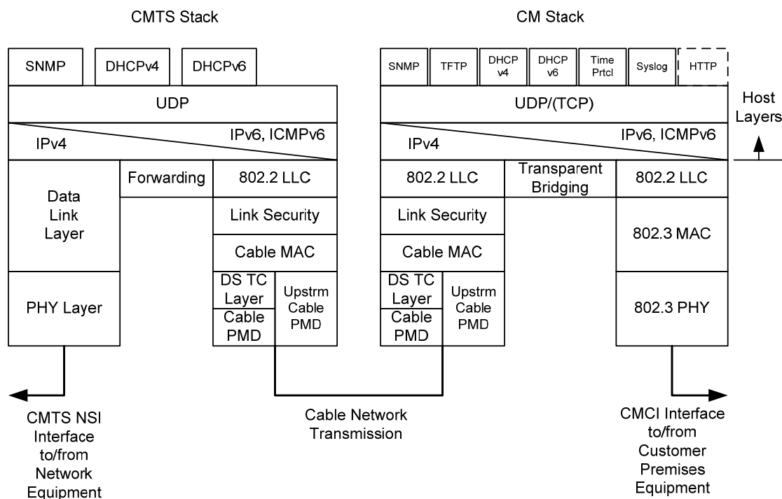
Figure 9–1 - DOCSIS Protocol Stacks 241
