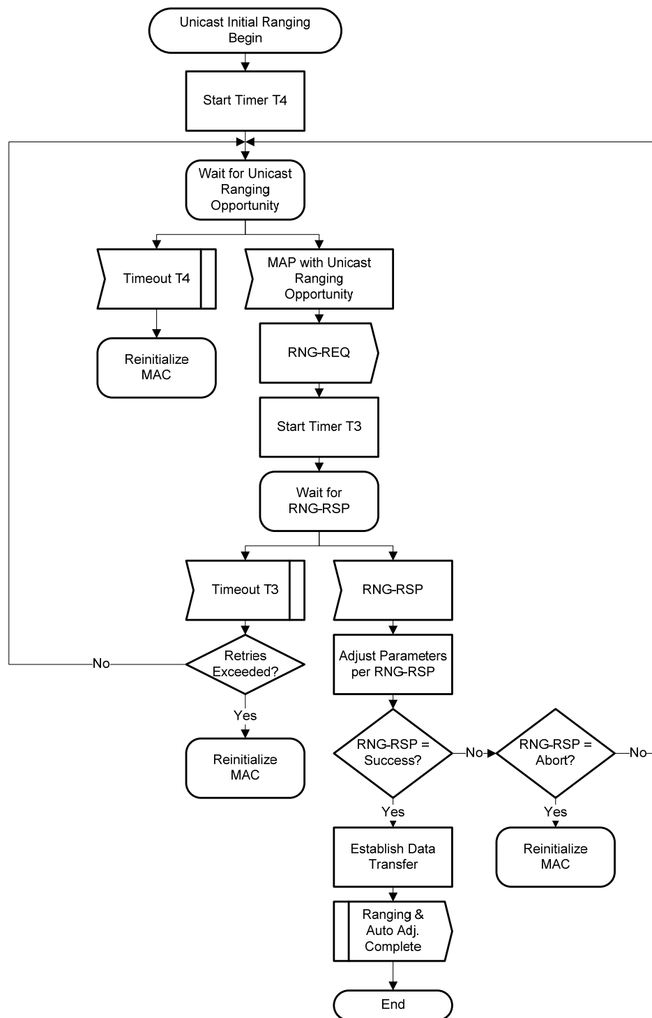
Figure 10–13 - Unicast Initial Ranging - CM 293
