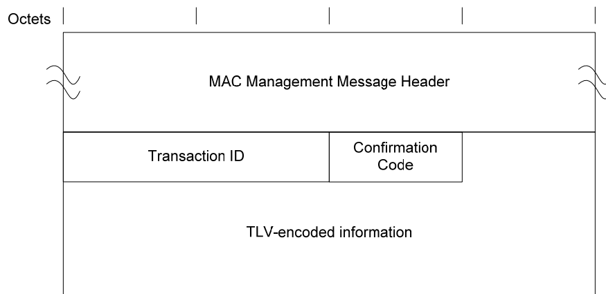
Figure 6–42 - Dynamic Channel Change Response 118
