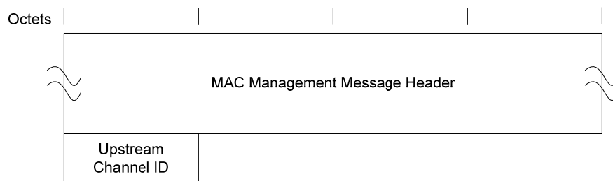
Figure 6–32 - Upstream Channel Change Response 101
