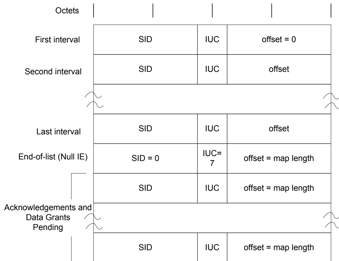
Figure 6–19 - MAP Information Element Structure 62
