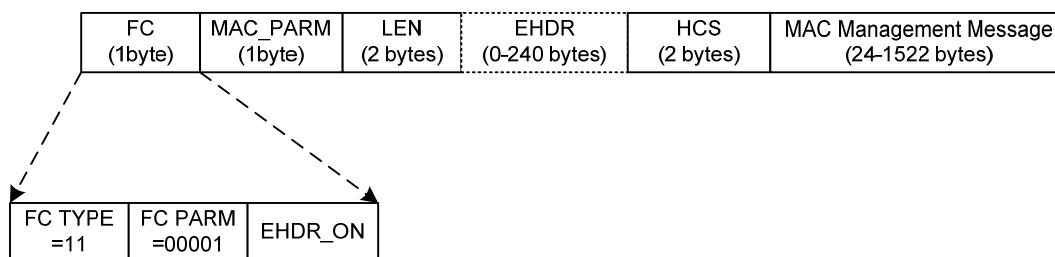
Figure 6–6 - Management MAC Header
