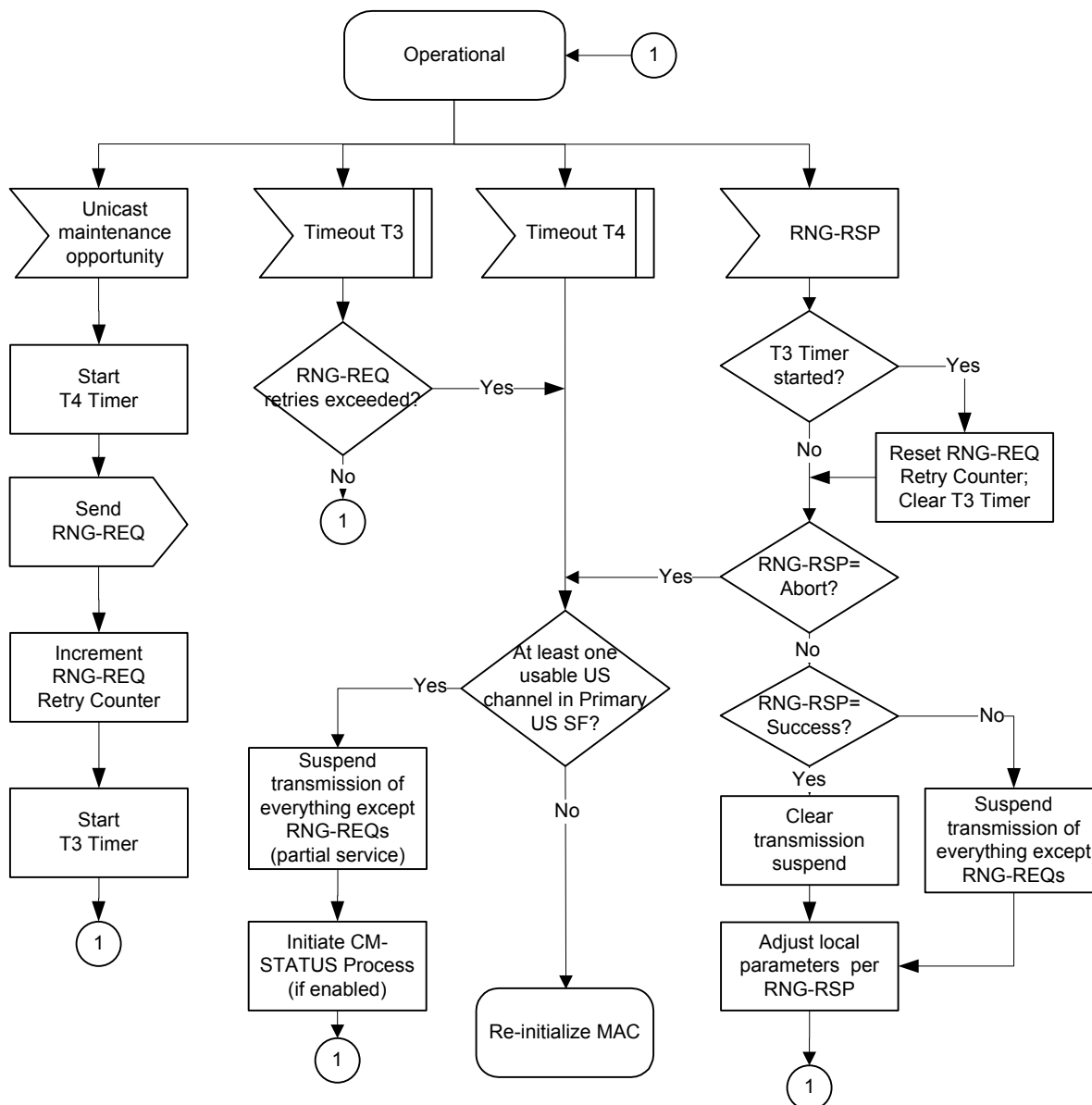
Figure 10-35 - Periodic Ranging - CM View 341
