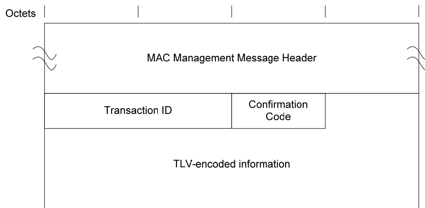
Figure 6–38 - Dynamic Service Change — Acknowledge 110
