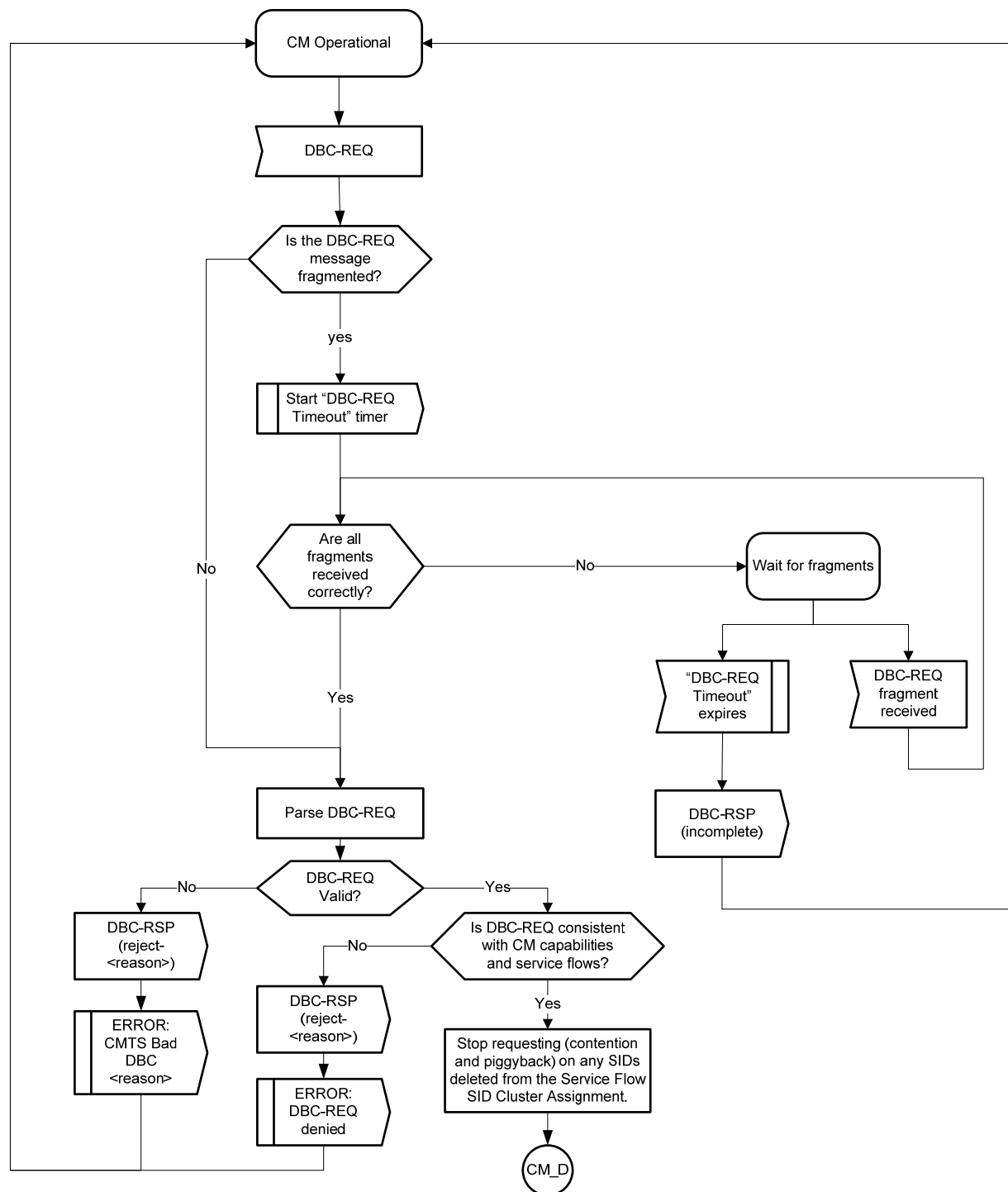
Figure 11-54 - CM DBC-RSP (part 1) 393
