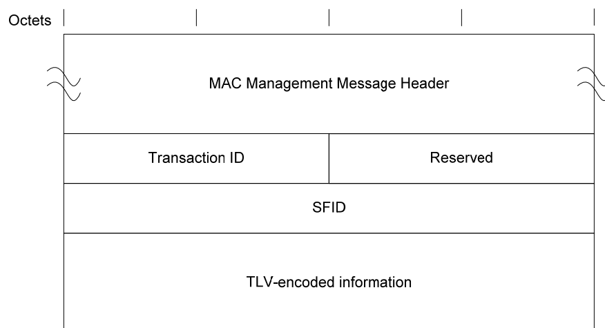
Figure 6–39 - Dynamic Service Deletion — Request 112
