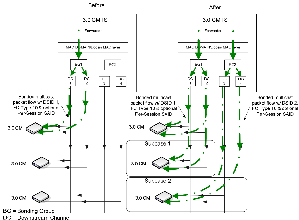
Figure VIII-8 - Multicast session replication to clients behind two 3.0 CMs 649
