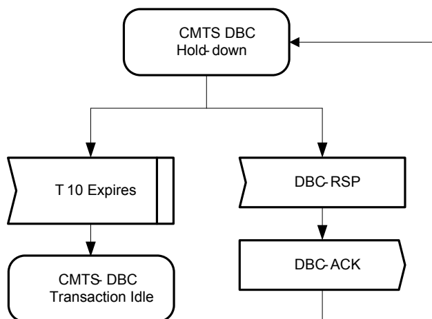
Figure 11–53 - CMTS DBC Hold-down 392
