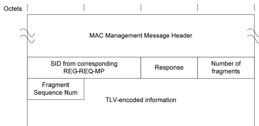
Figure 6–29 - Multipart Registration Response Format 93
