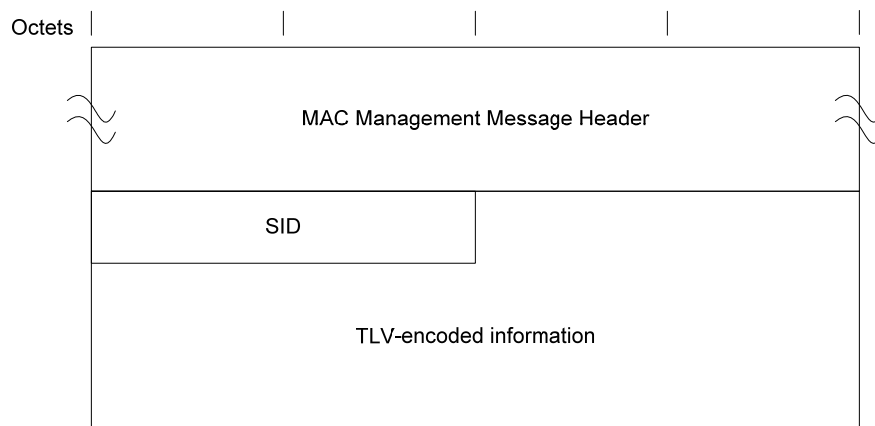
Figure 6–26 - Registration Request (REG-REQ) 88
