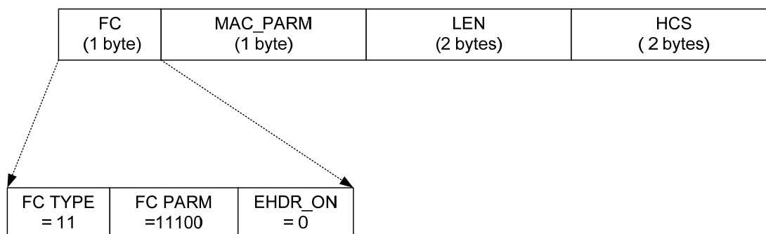
Figure 6–10 - Concatenation MAC Header Format 35
