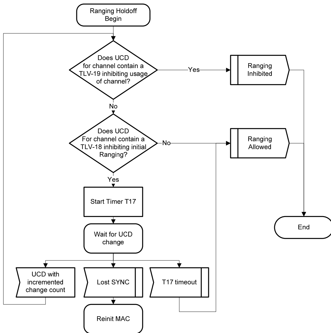
Figure 10–5 - Ranging Holdoff
