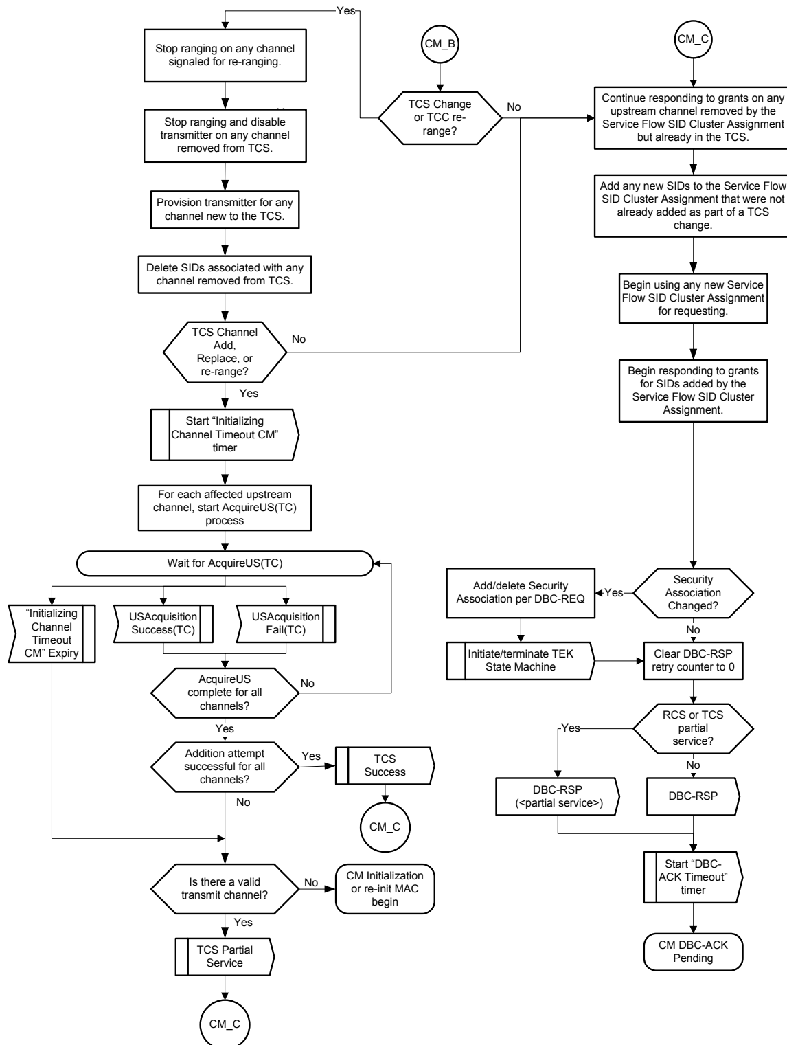
Figure 11-56 - CM DBC-RSP (part 3) 395
