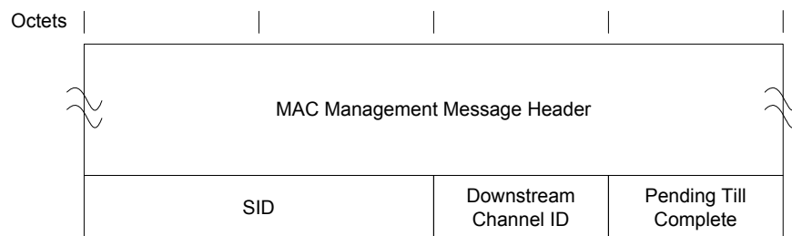
Figure 6–20 - RNG-REQ Format 67
