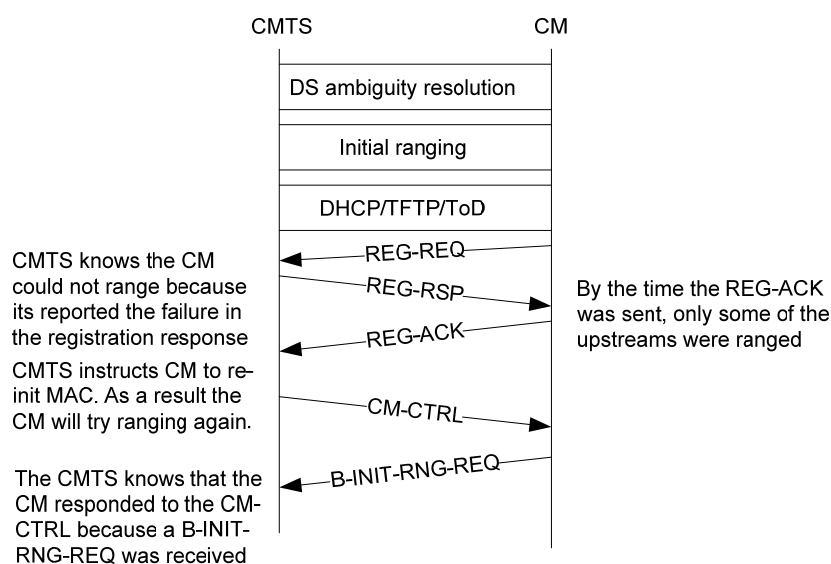
Figure V-1 - Example 1 - Modem can't range on all upstreams 636
