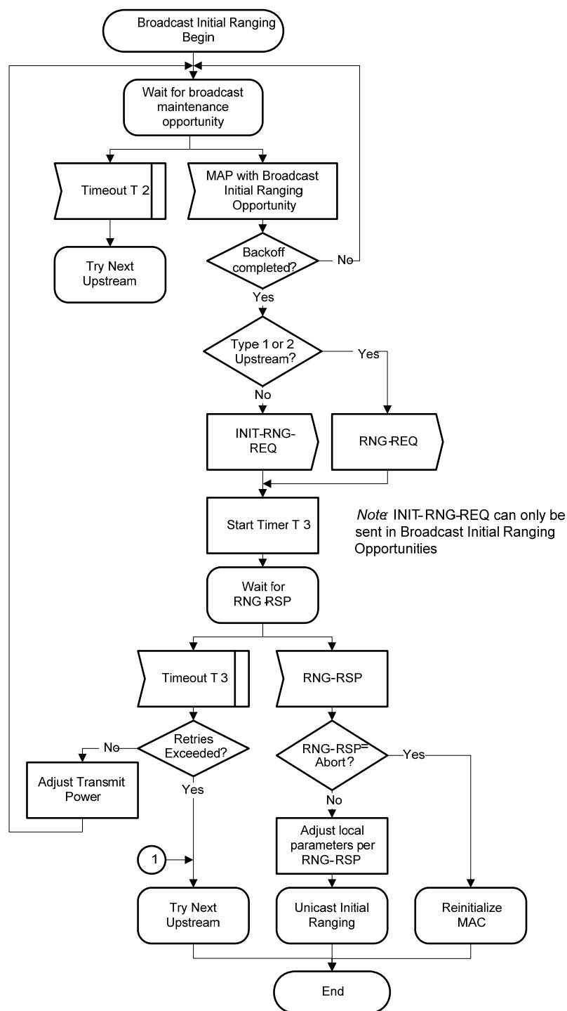
Figure 10-12 - Broadcast Initial Ranging – CM 292
