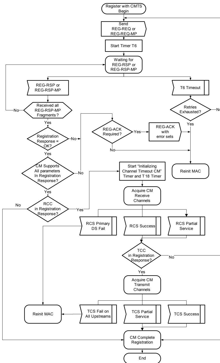
Figure 10-25 - CM Register with CMTS - Begin 323
