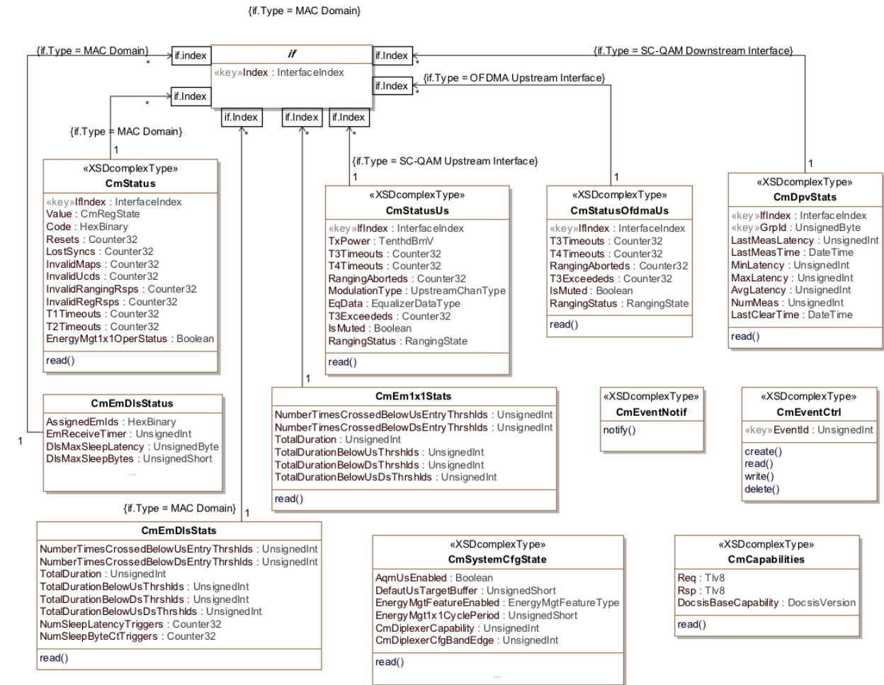
Figure F-1 - CM Operational Status Information Model Diagram 49
