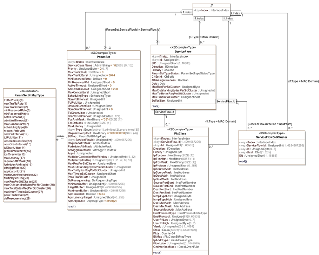
Figure G-2 - QoS Configuration Information Model Diagram 65
