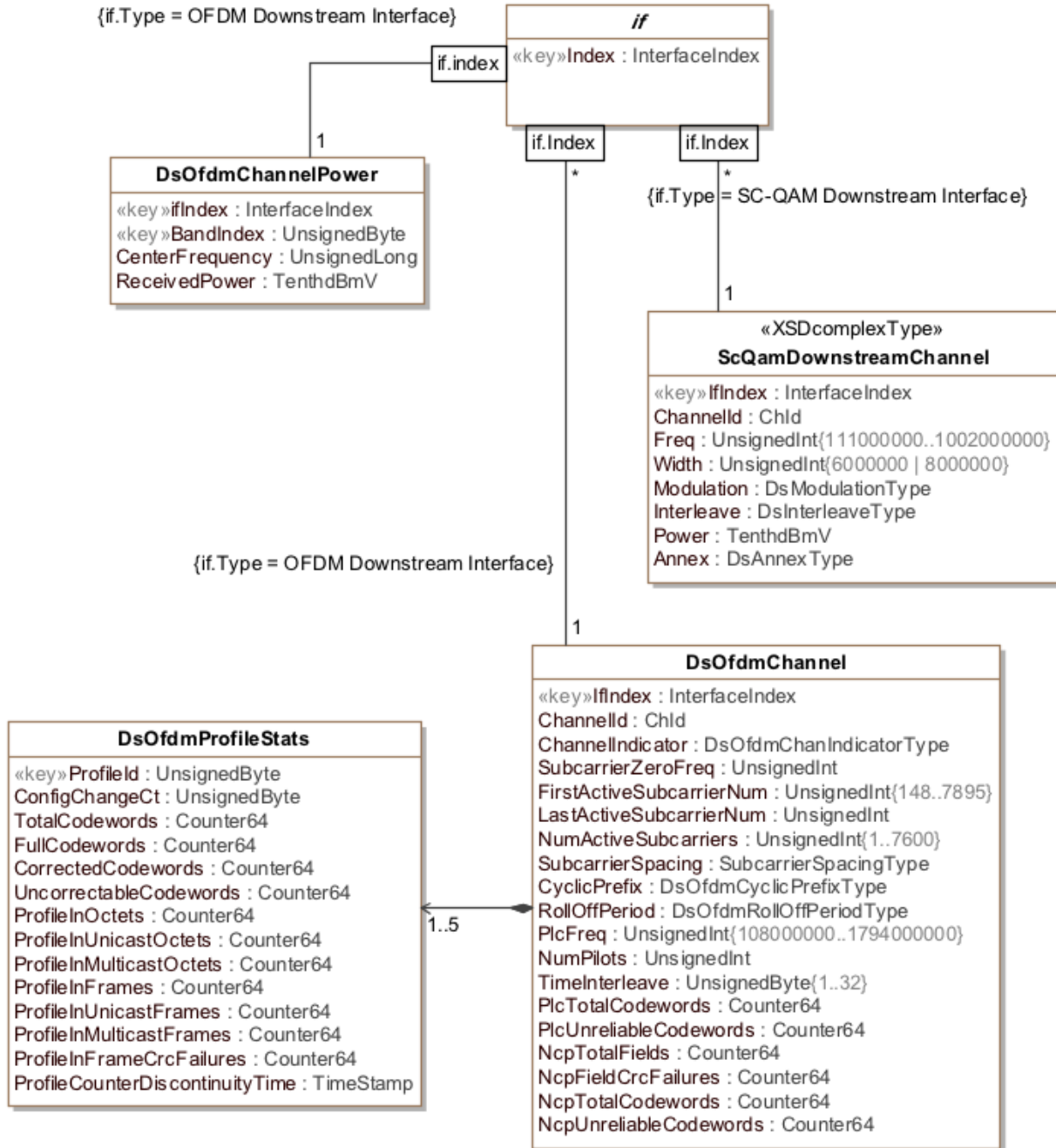
Figure F-2 - CM Downstream Information Model Diagram 56
