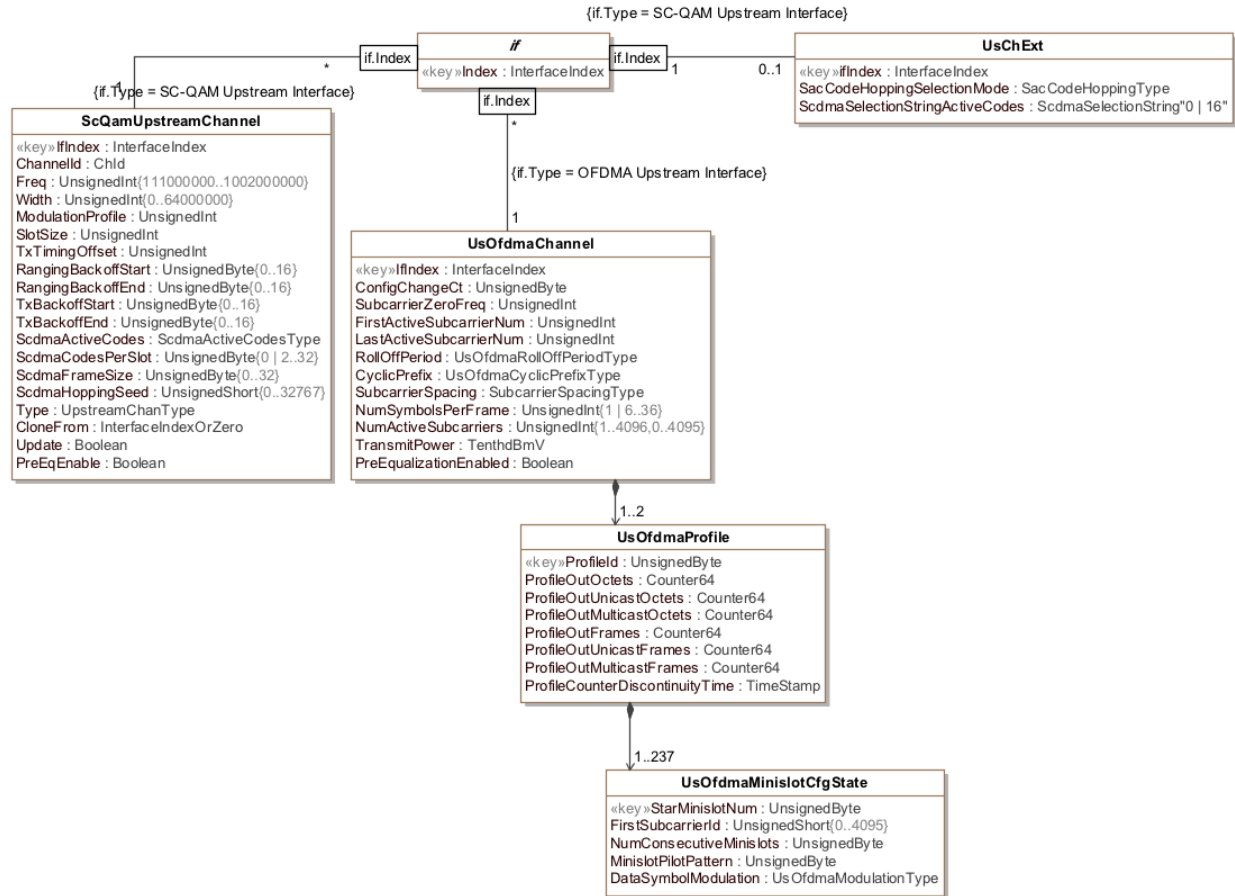
Figure F-3 - CM Upstream Information Model Diagram 62
