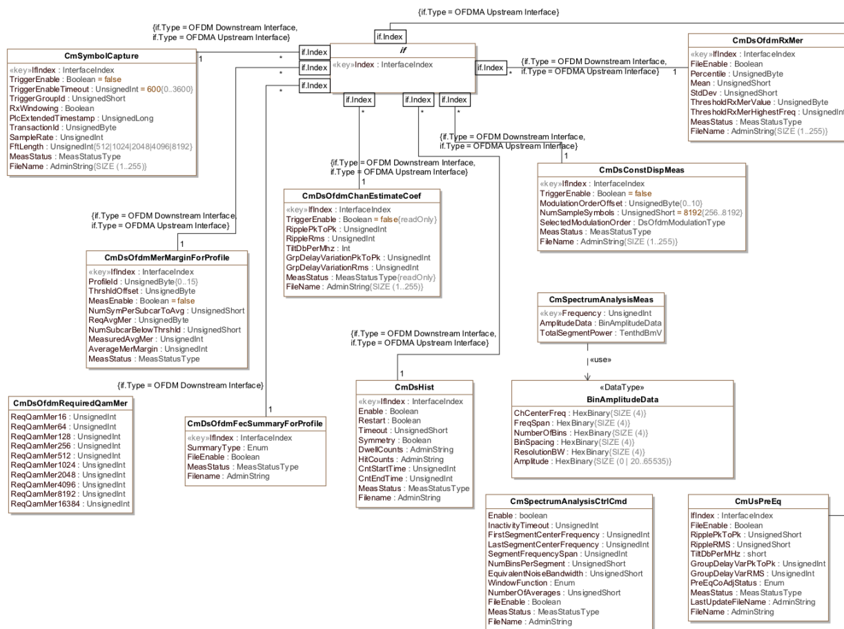
Figure D-1 - Proactive Network Maintenance Information Model Diagram 34
