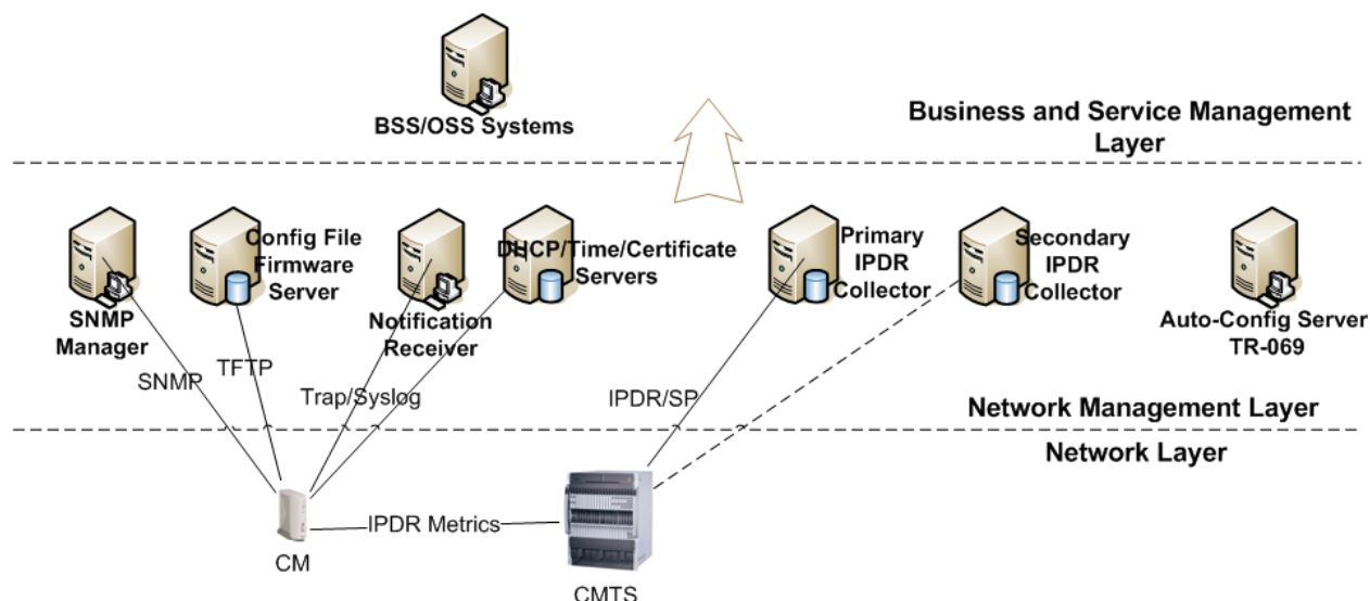
Figure 5-1 - CM Management Architecture
