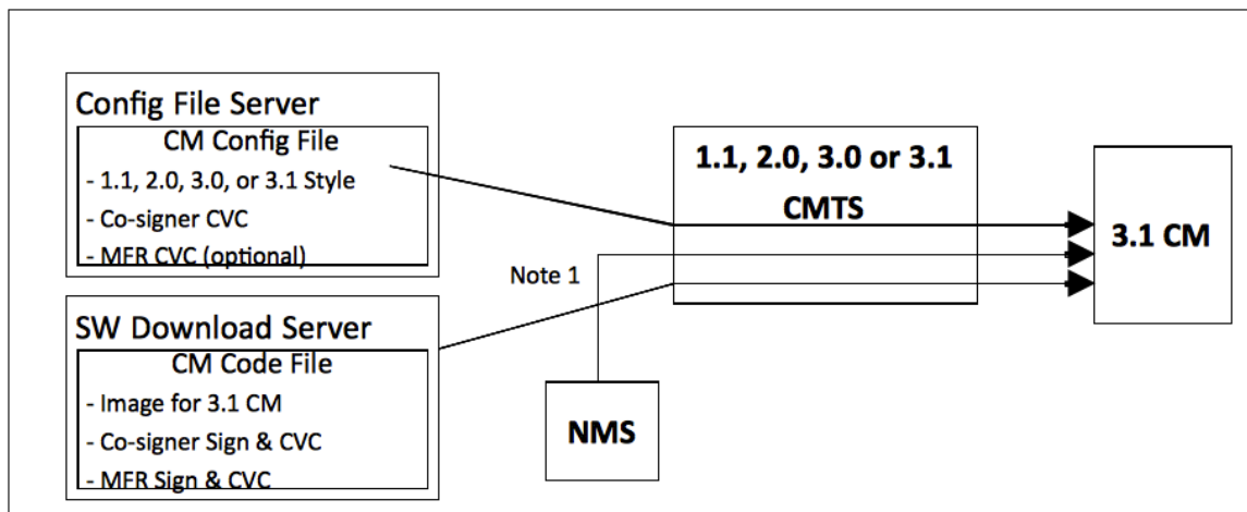
Figure 8-2 - Operator control scheme 20
