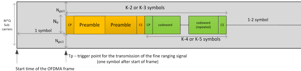
Figure 7-27 - Fine Ranging Signal Transmission 39
