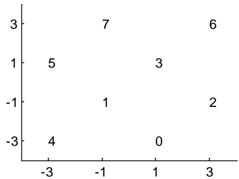
Figure A-3 - 8-QAM Constellation Mapping of \{y_0 y_1 y_2\}
