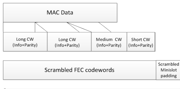
Figure 7-3 - Upstream Transmitter Block Diagram
