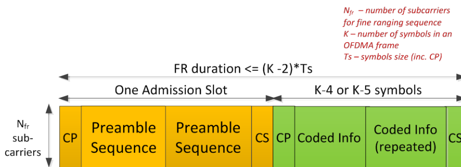
Figure 7-26 - Fine Ranging Signal 38
