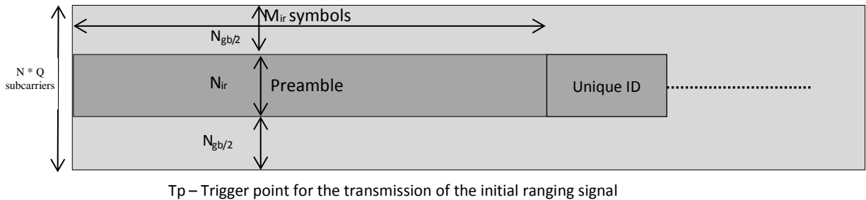
Figure 7-19 - Initial Ranging Signal
