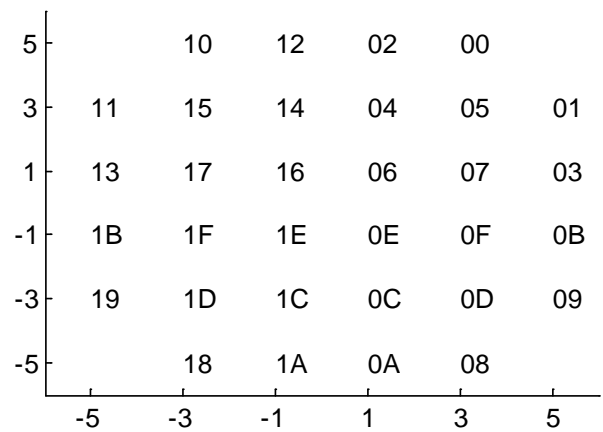
Figure A-5 - 32-QAM Constellation Mapping of \{y_0 y_1 y_2 y_3 y_4\}
