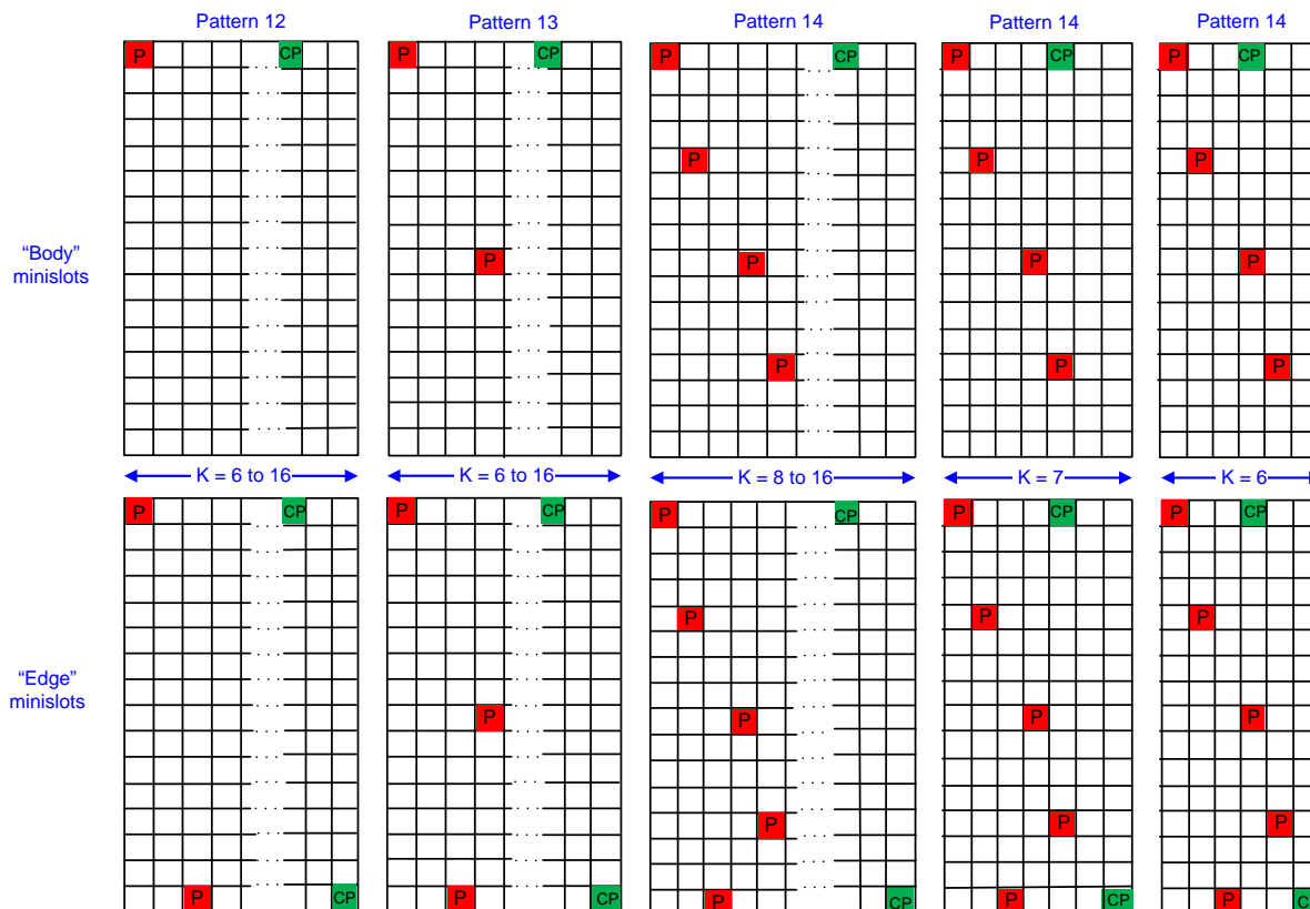
Figure 7-39 - Pilot Patterns 12-14 for Minislots with 16 Subcarriers
