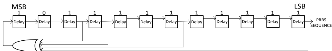
Figure 7-32 - Polynomial Sequence for Pseudorandom Binary Sequence Generation
