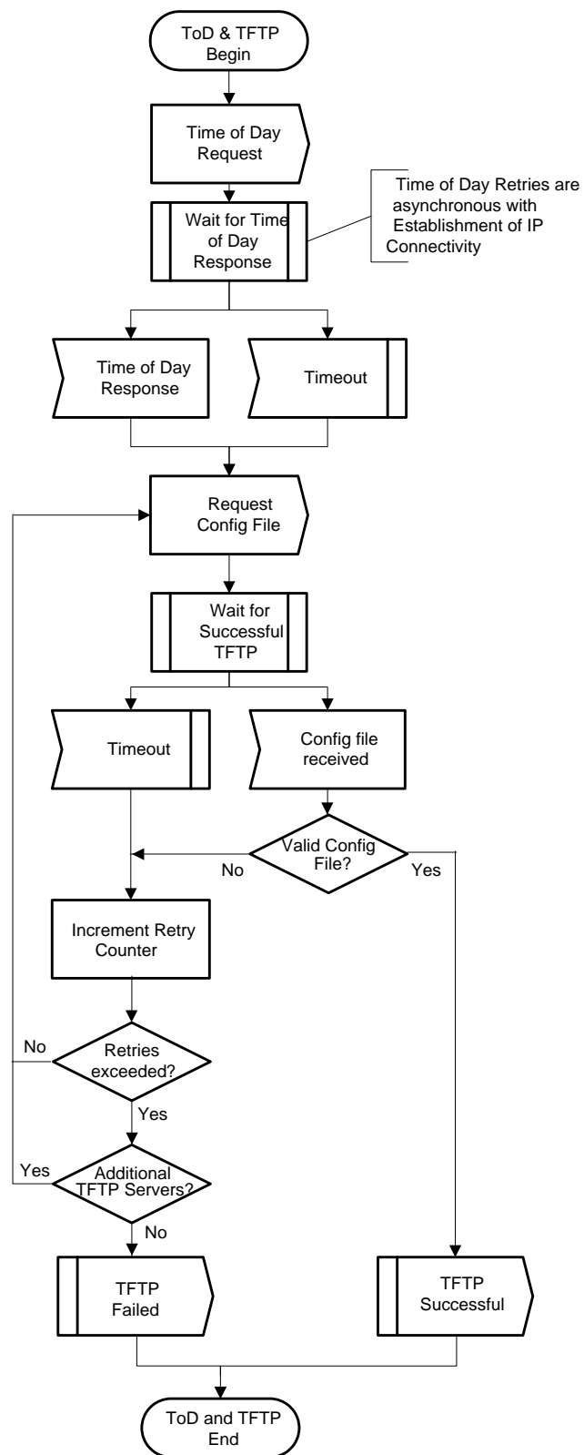
Figure 142 - ToD and TFTP
