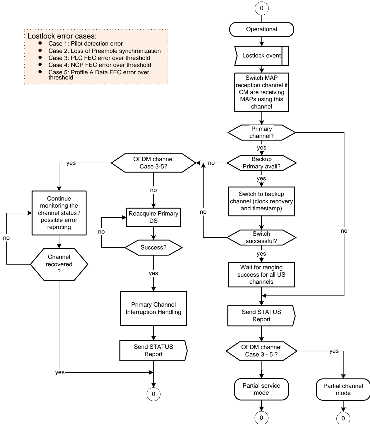
Figure 165 - Lost Lock on an OFDM Channel Procedure
