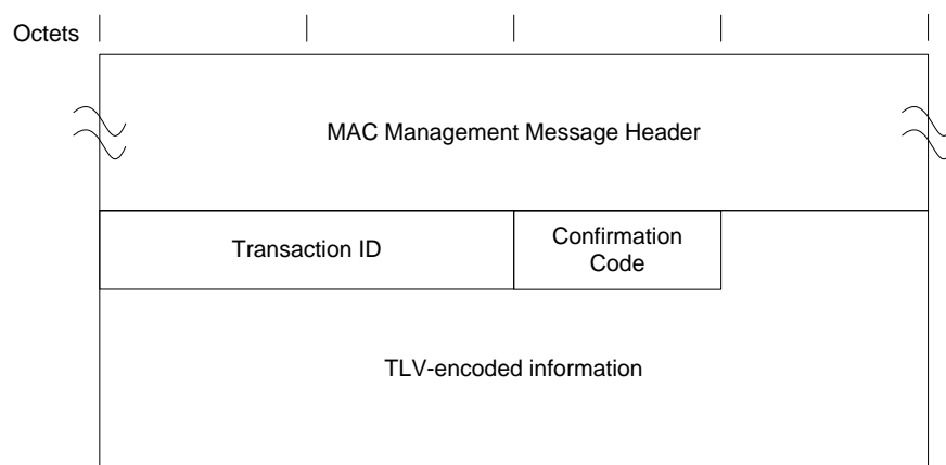
Figure 56 - Dynamic Service Addition - Response
