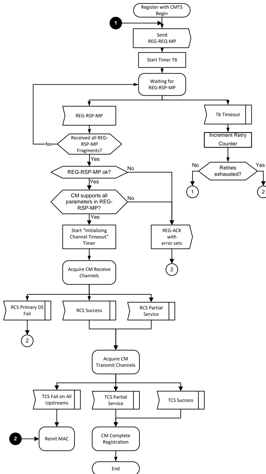
Figure 146 - CM Register with CMTS - Begin
