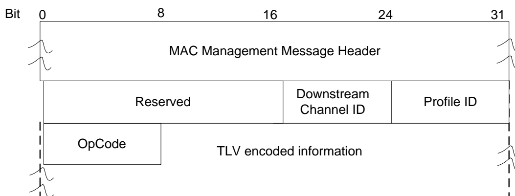
Figure 81 - The OFDM Downstream Profile Test Request (OPT-REQ) message
