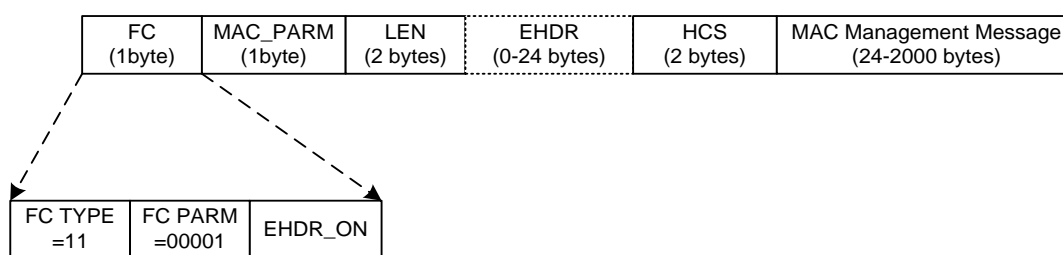
Figure 22 - Management MAC Header
