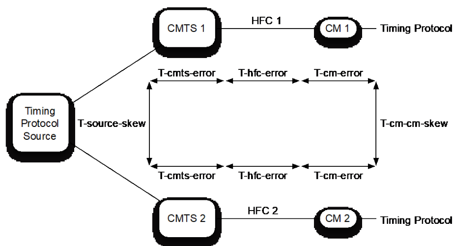
Figure 175 - DTP System Performance
