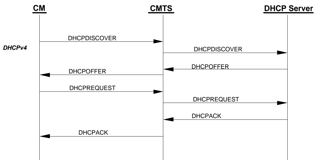
Figure 144 - IPv4 Provisioning Message Flow
