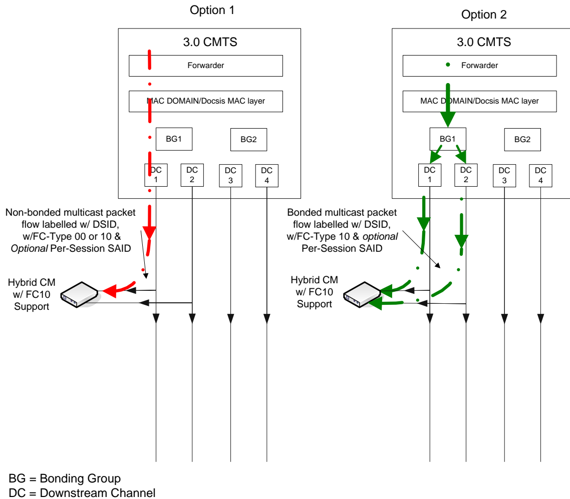
Figure 256 - Multicast Session Replication for a client behind a Hybrid CM capable of FC-Type 10
