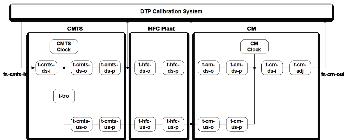
Figure 171 - DTP Math and Delays
