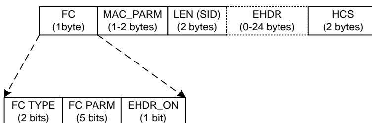
Figure 19 - MAC Header Format
