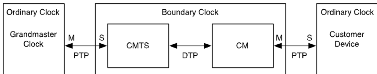
Figure 170 - DTP/PTP Reference Architecture
