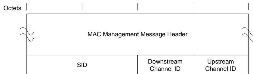
Figure 43 - INIT-RNG-REQ Format
