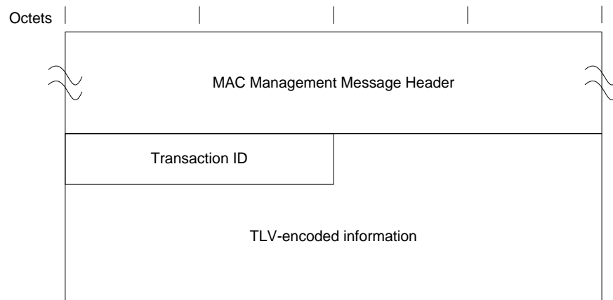
Figure 69 - Dynamic Bonding Change Acknowledge Message
