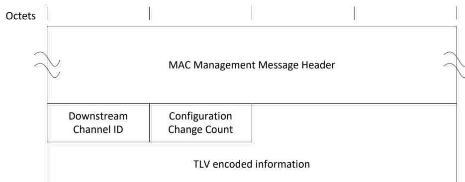
Figure 78 - OFDM Channel Descriptor
