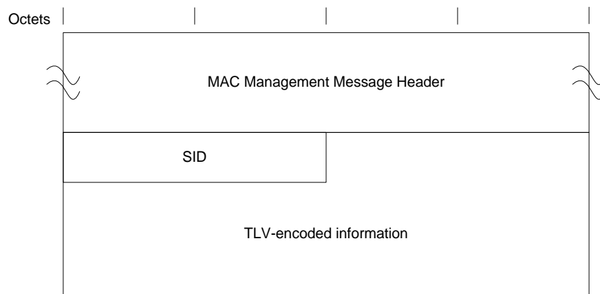
Figure 50 - Registration Request (REG-REQ)
