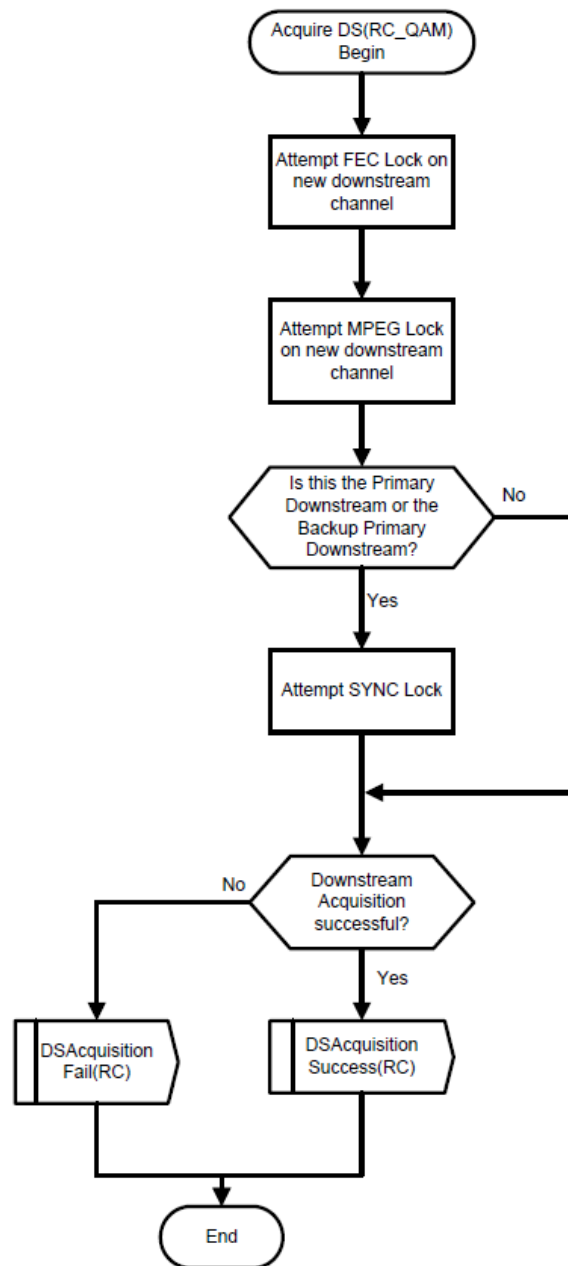
Figure 148 - CM Acquires SC-QAM Downstream Channel
