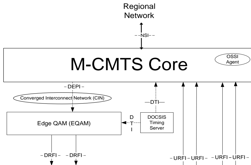
Figure 6 - Modular CMTS Network Diagram
