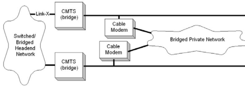
Figure 245 - Spanning Tree Across CMTSs
