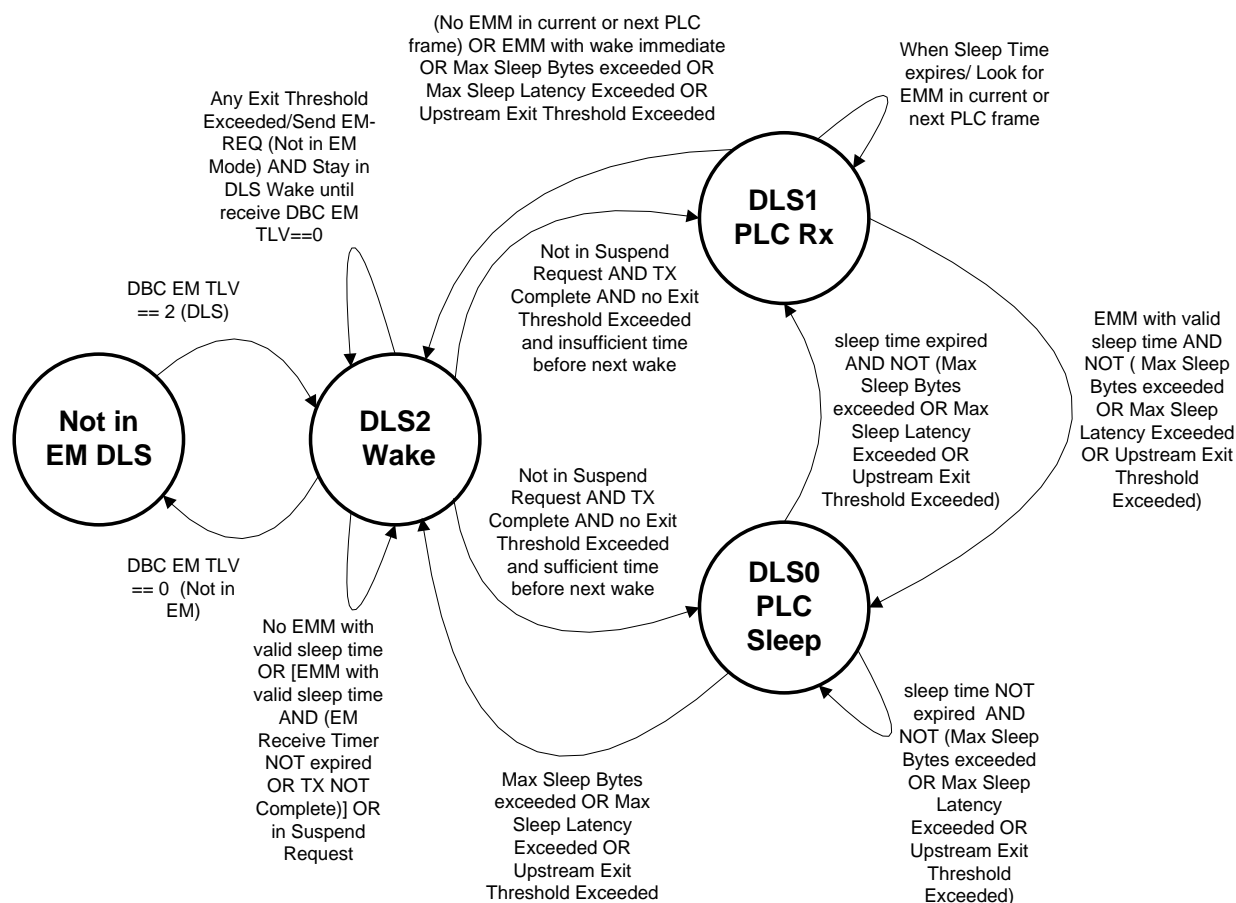
Figure 233 - CM DLS Substate Diagram
