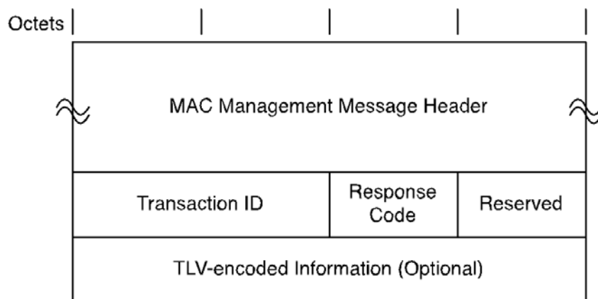
Figure 76 - Energy Management Response Message
