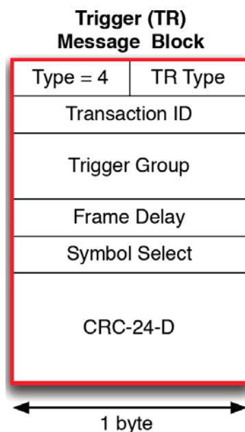
Figure 93 - Trigger Message Block
