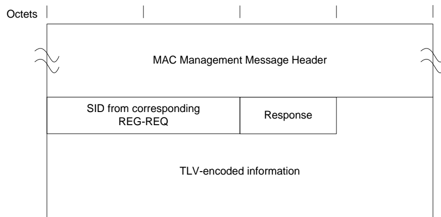
Figure 52 - Registration Response Format
