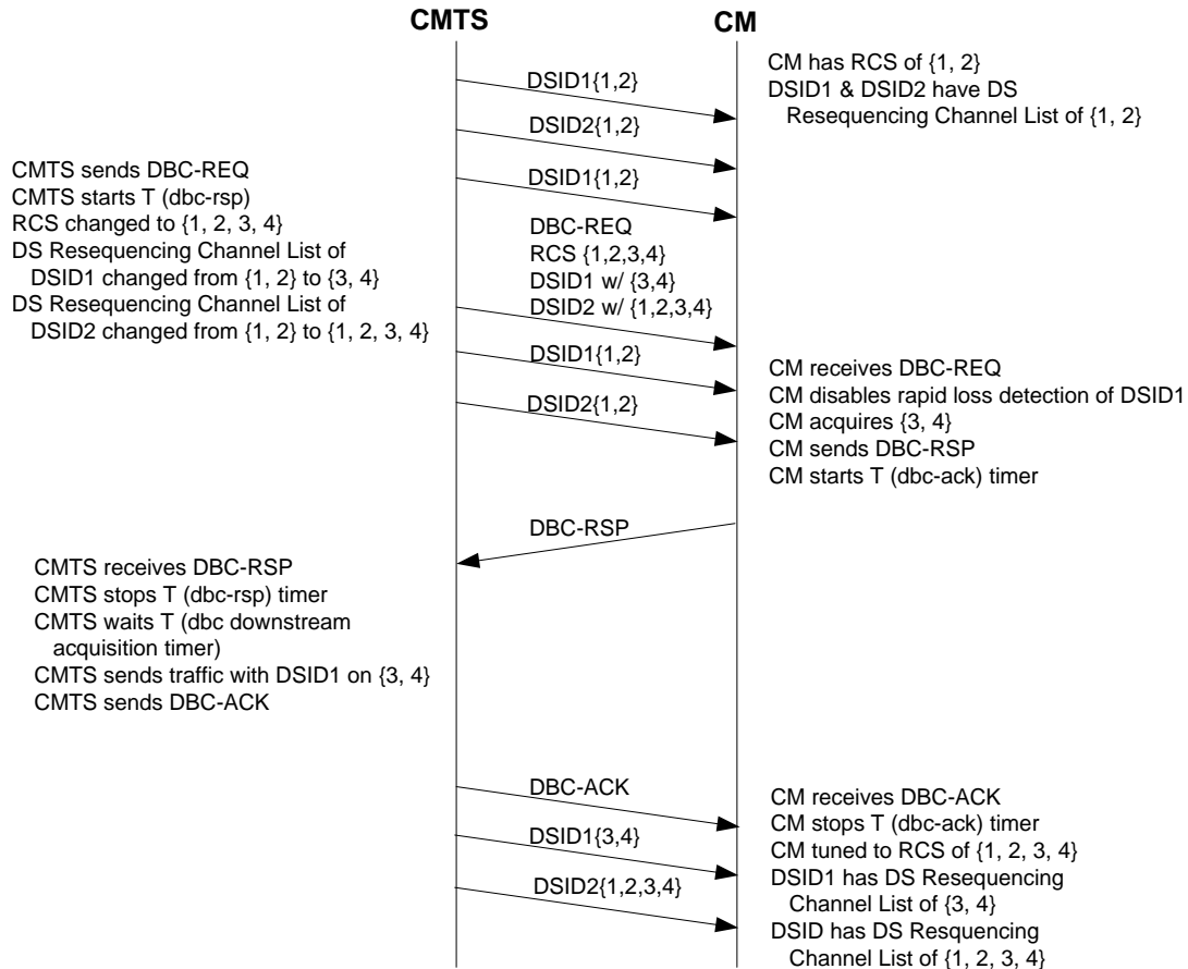
Figure 265 - Changing the RCS and Downstream Resequencing Channel List
