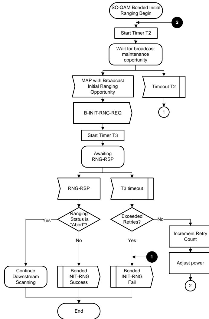
Figure 130 - SC-QAM Bonded Initial Ranging
