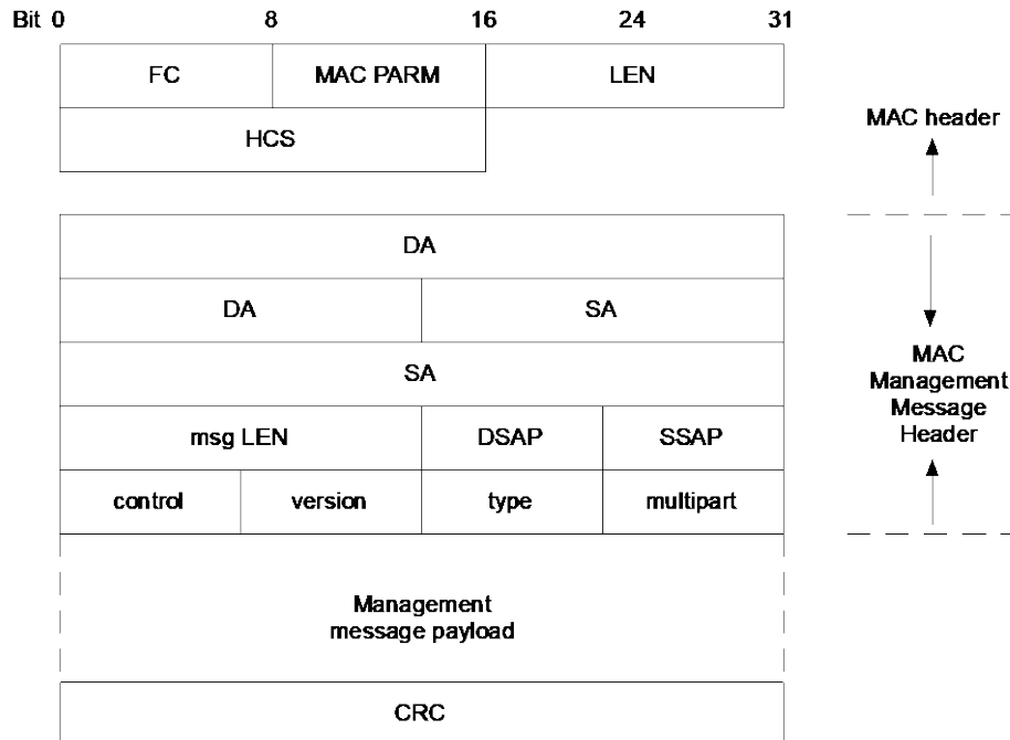
Figure 29 - MAC Header and MAC Management Message Header Fields
