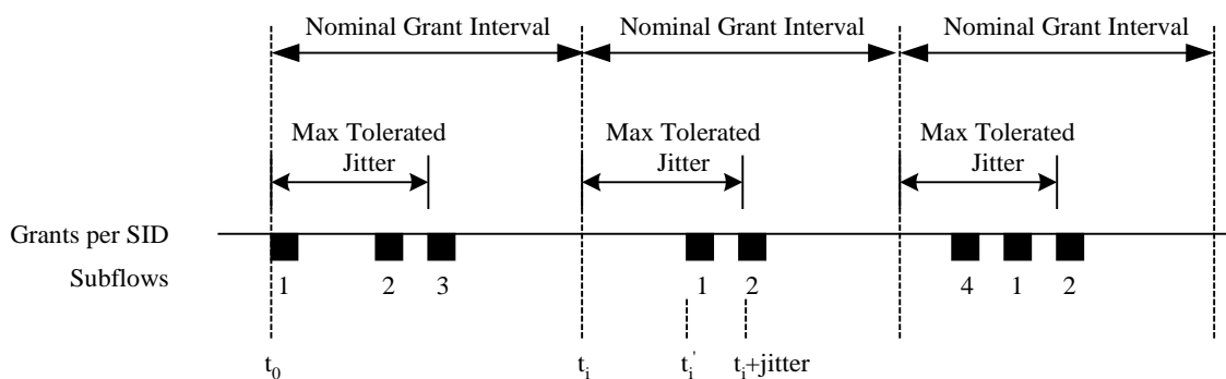
Figure 250 - Example Jitter with Multiple Grants per SID
