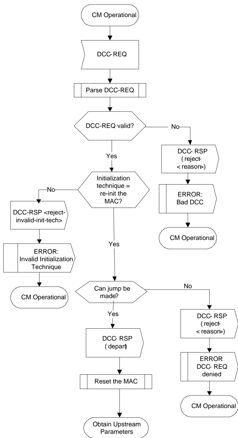
Figure 218 - Dynamically Changing Channels: CM View
