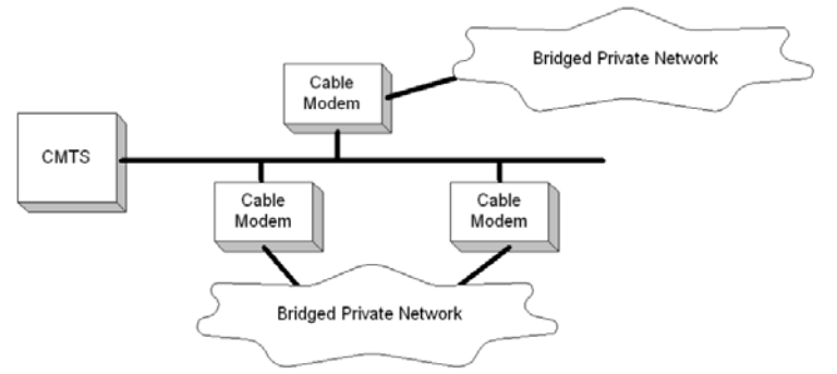
Figure 244 - Spanning Tree Topology
