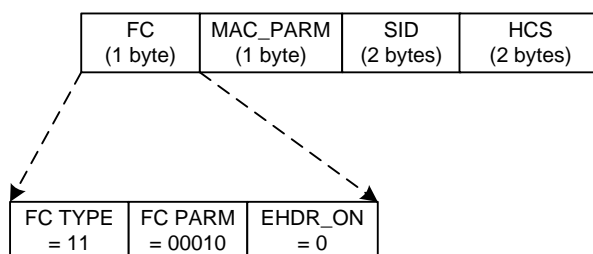
Figure 23 - Request Frame Format
