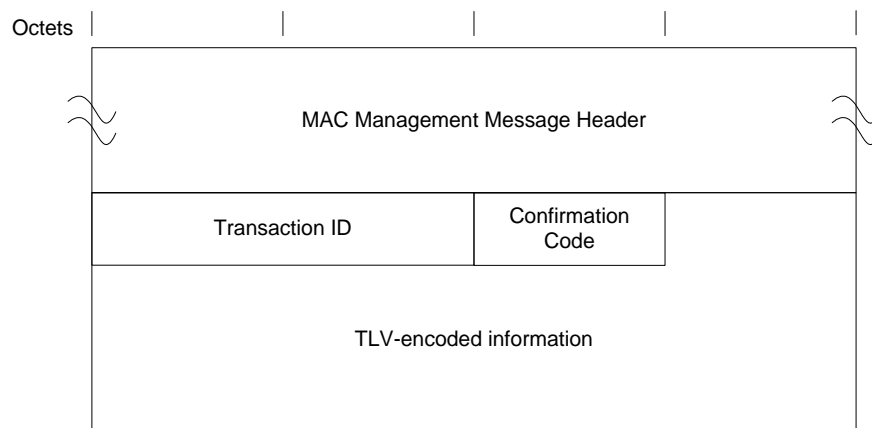
Figure 64 - Dynamic Channel Change Response
