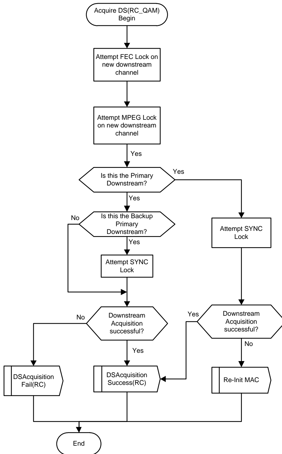
Figure 226 - CM AcquireDS Procedure for SC-QAM
