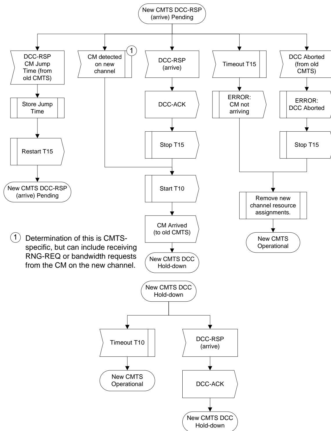
Figure 217 - Dynamically Changing Channels: CMTS View Part 4
