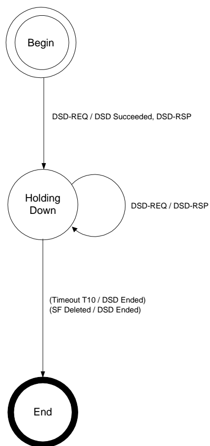
Figure 183 - Dynamic Deletion (DSD) - Remotely Initiated Transaction State Transition Diagram
