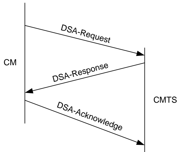
Figure 108 - Dynamic Service Addition Message Flow - CM Initiated
