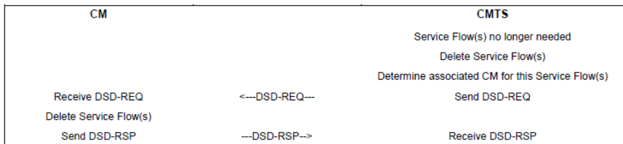
Figure 208 - Dynamic Service Deletion Initiated from CMTS
