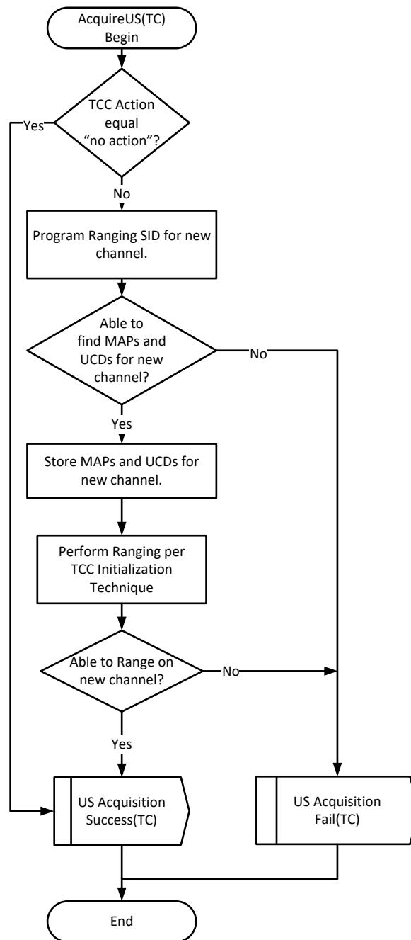
Figure 151 - CM Acquires Upstream Channel
