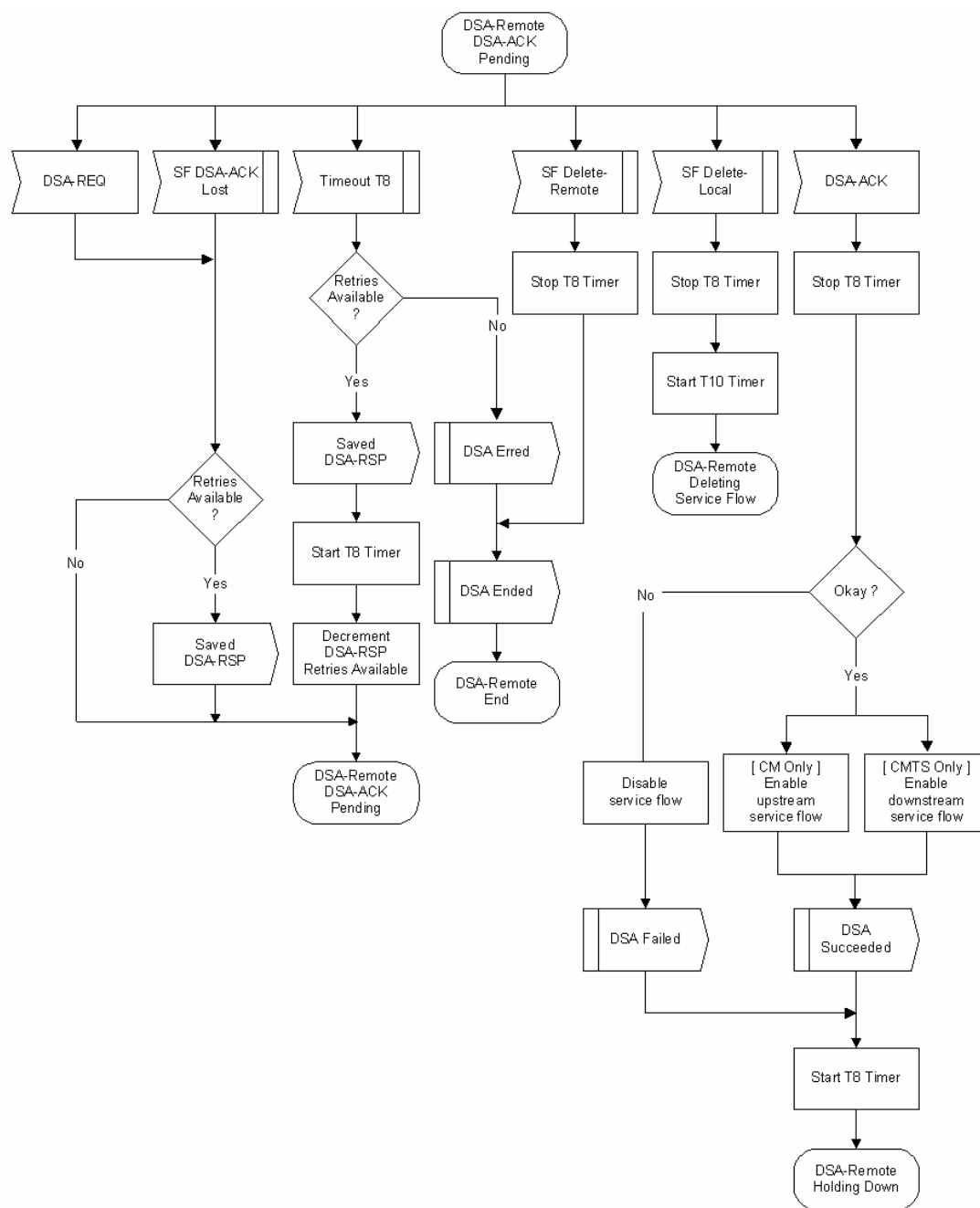
Figure 192 - DSA-Remotely Initiated Transaction DSA-ACK Pending State Flow Diagram
