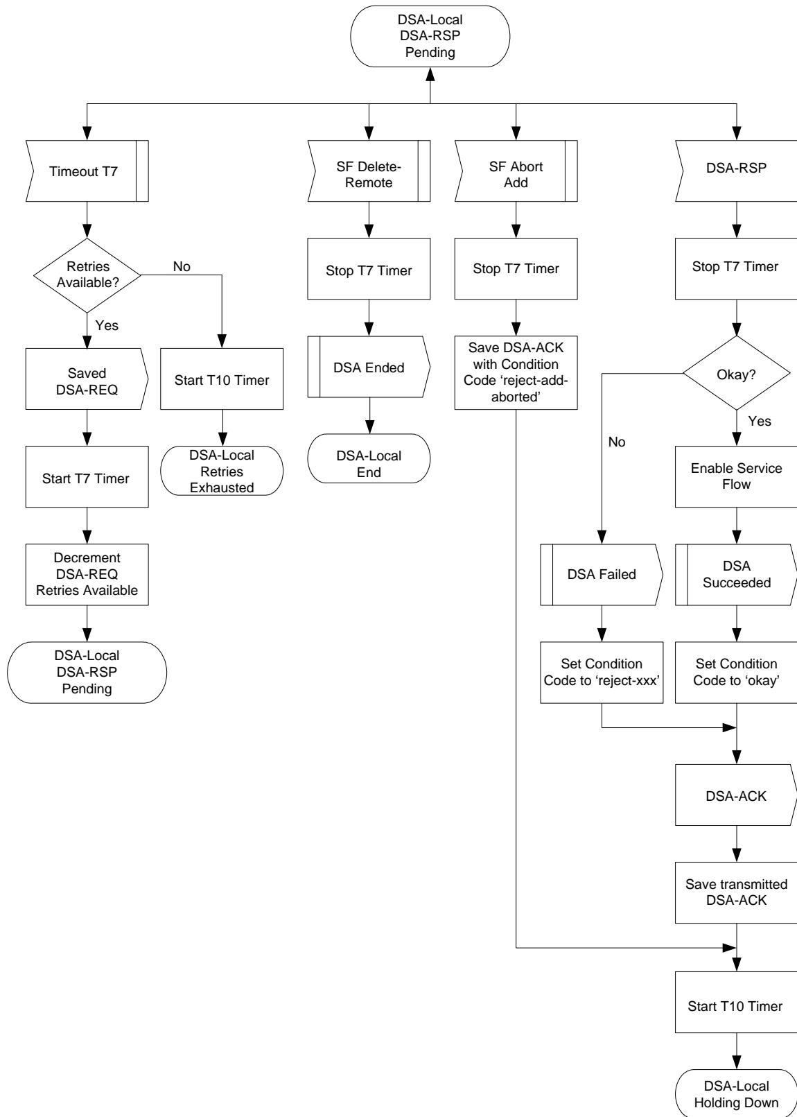
Figure 187 - DSA-Locally Initiated Transaction DSA-RSP Pending State Flow Diagram
