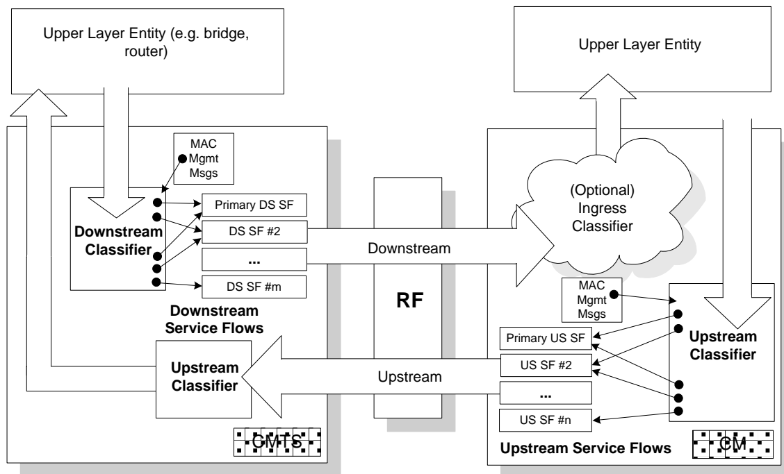
Figure 105 - Classification within the MAC Layer
