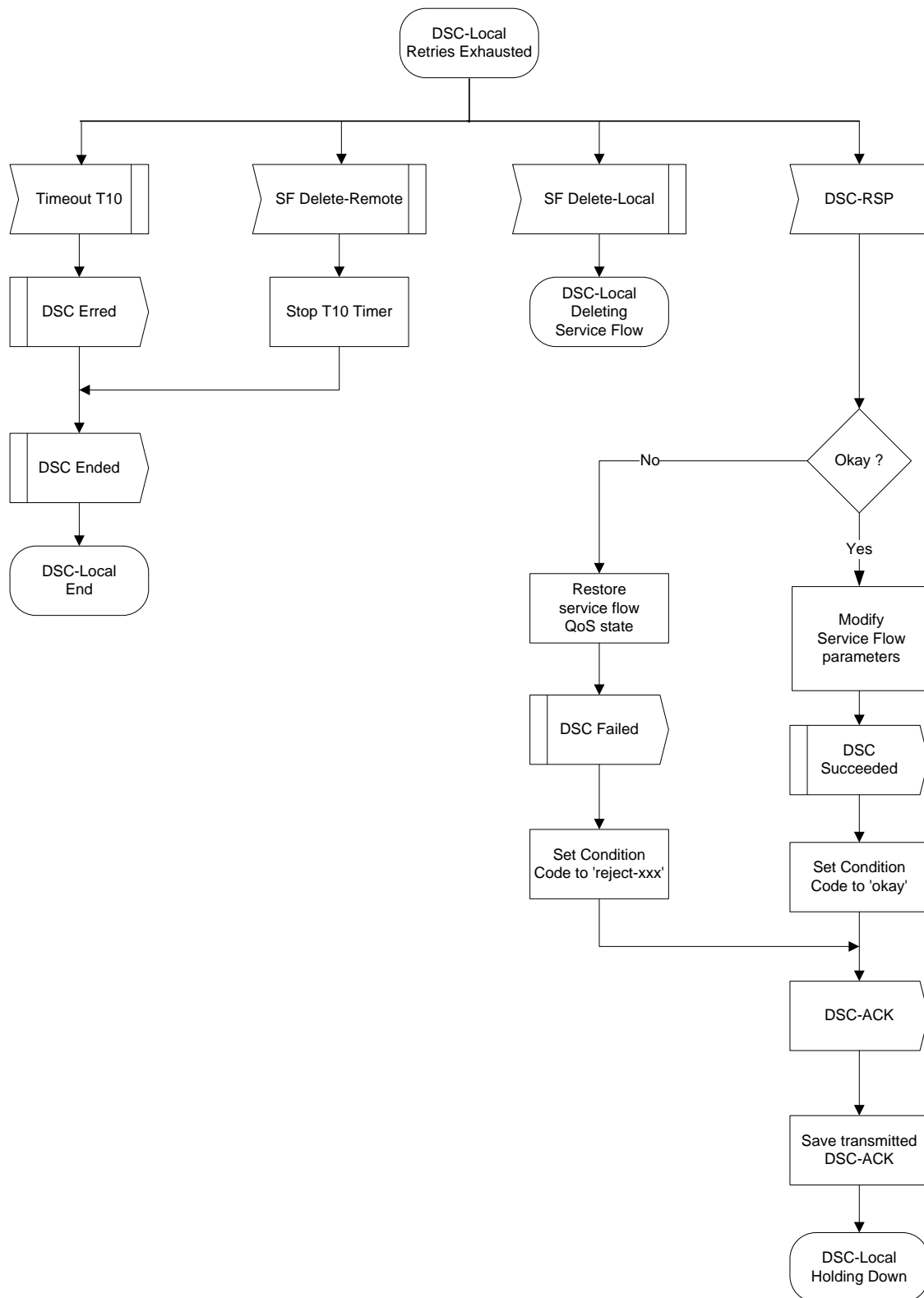
Figure 201 - DSC-Locally Initiated Transaction Retries Exhausted State Flow Diagram
