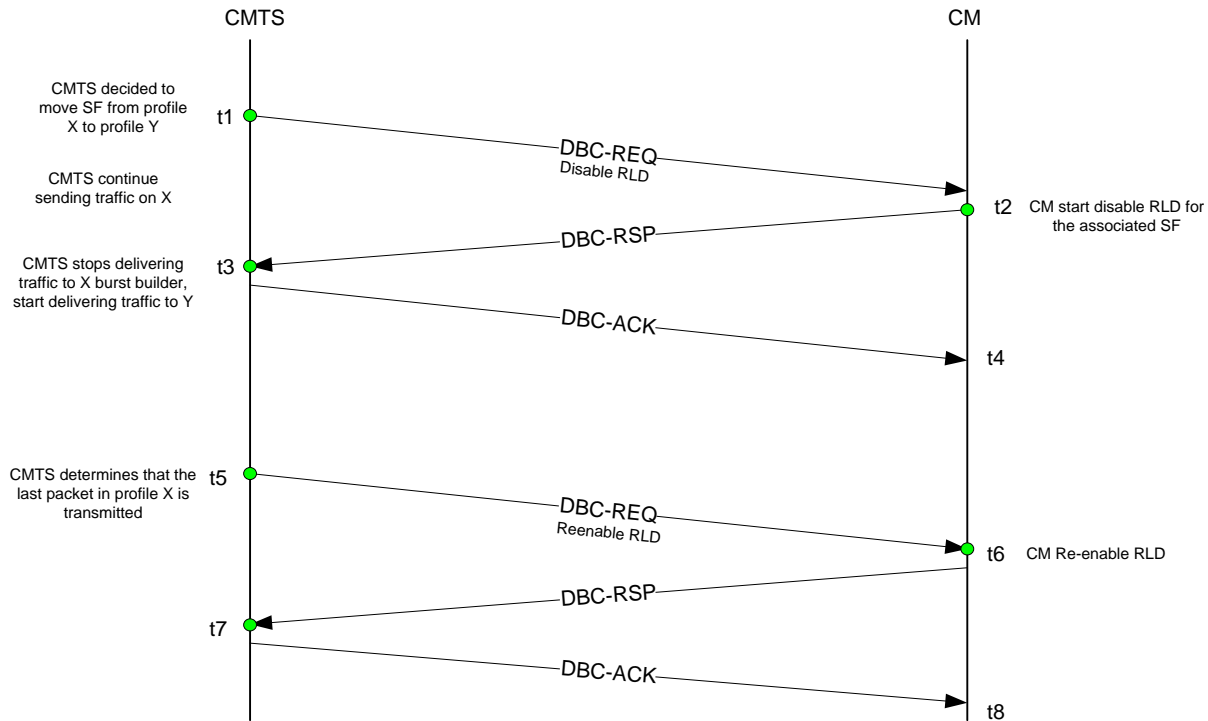
Figure 266 - DBC procedure for SF profile switch on OFDM channel
