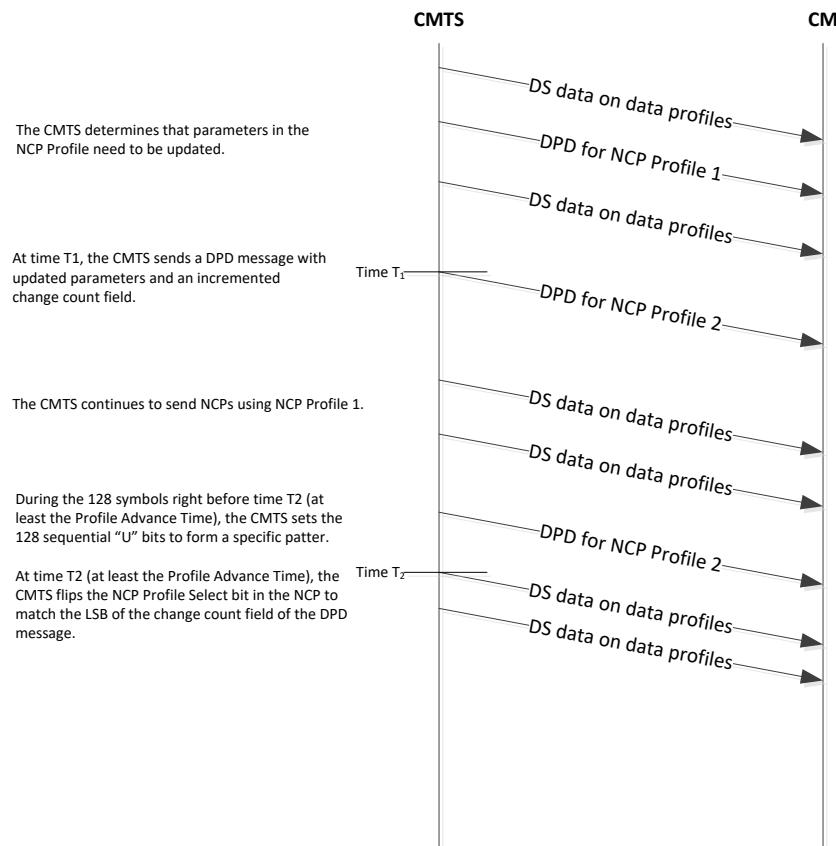
Figure 270 - DPD Change to the NCP Profile
