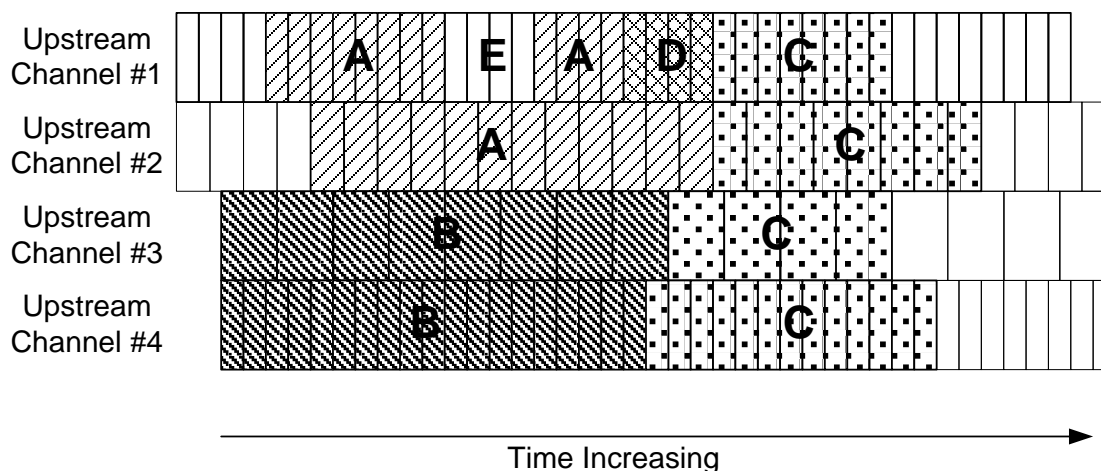
Figure 9 - Segmentation Example
