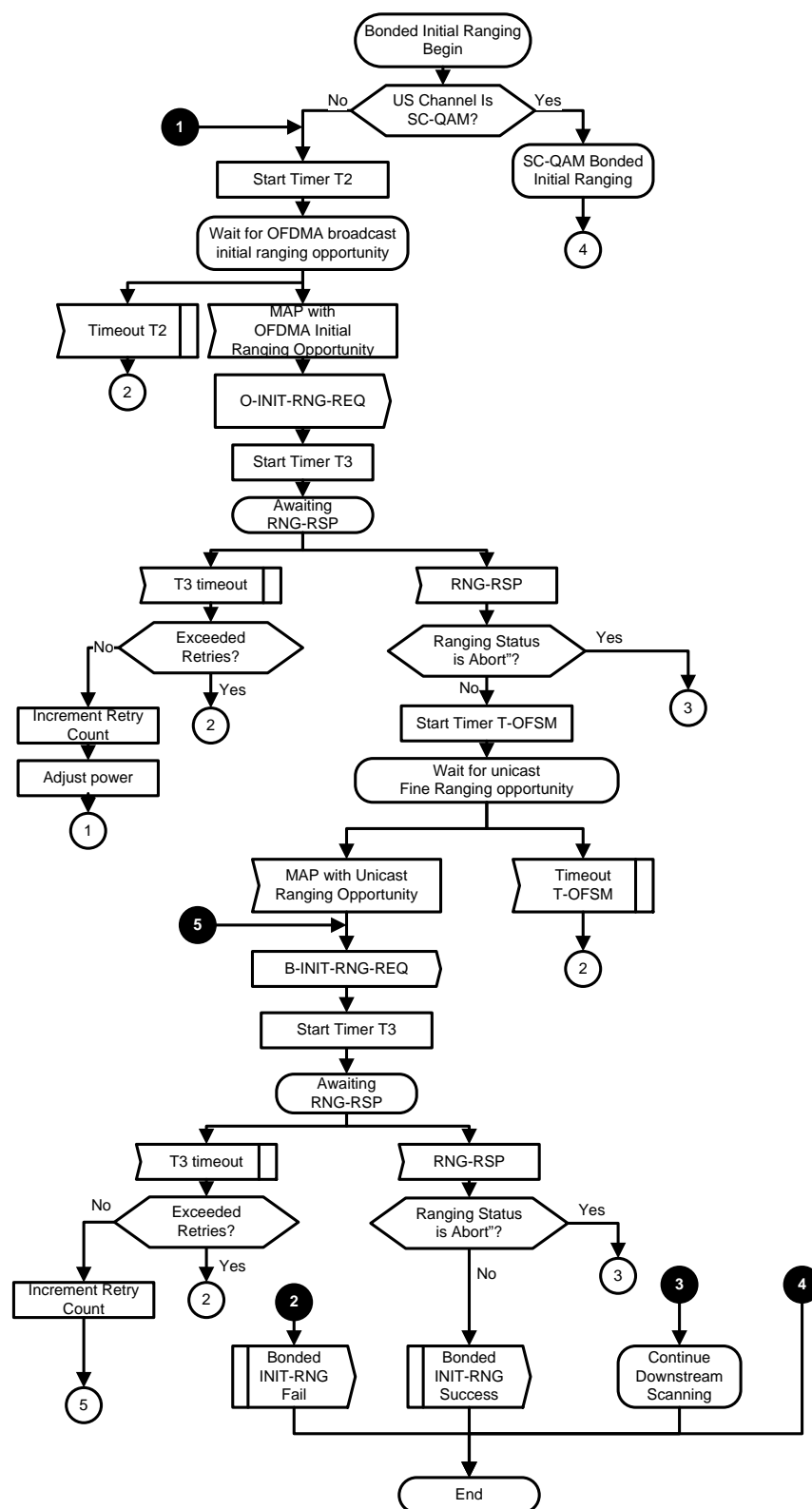
Figure 129 - Bonded Initial Ranging
