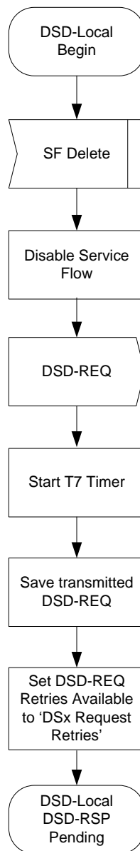
Figure 209 - DSD-Locally Initiated Transaction Begin State Flow Diagram
