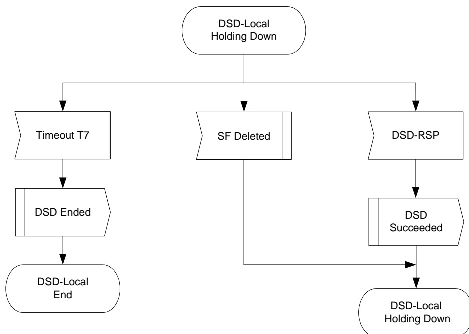
Figure 211 - DSD-Locally Initiated Transaction Holding Down State Flow Diagram
