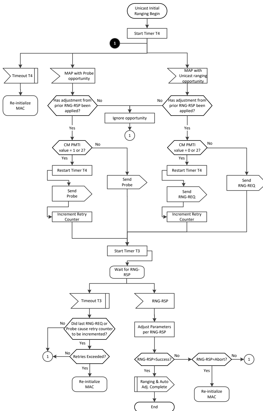
Figure 134 - Unicast Initial Ranging - CM
