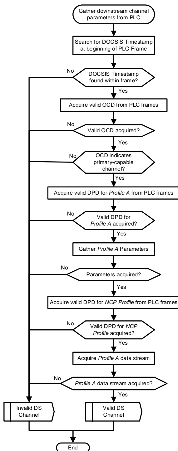
Figure 123 - Gather Downstream Channel Parameters from PLC
