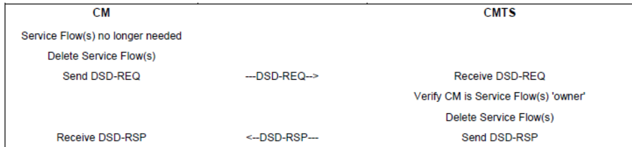
Figure 207 - Dynamic Service Deletion Initiated from CM
