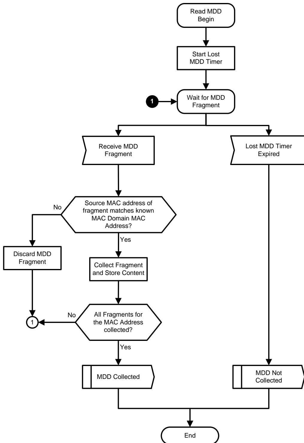
Figure 125 - Read MAC Domain Descriptor (MDD)
