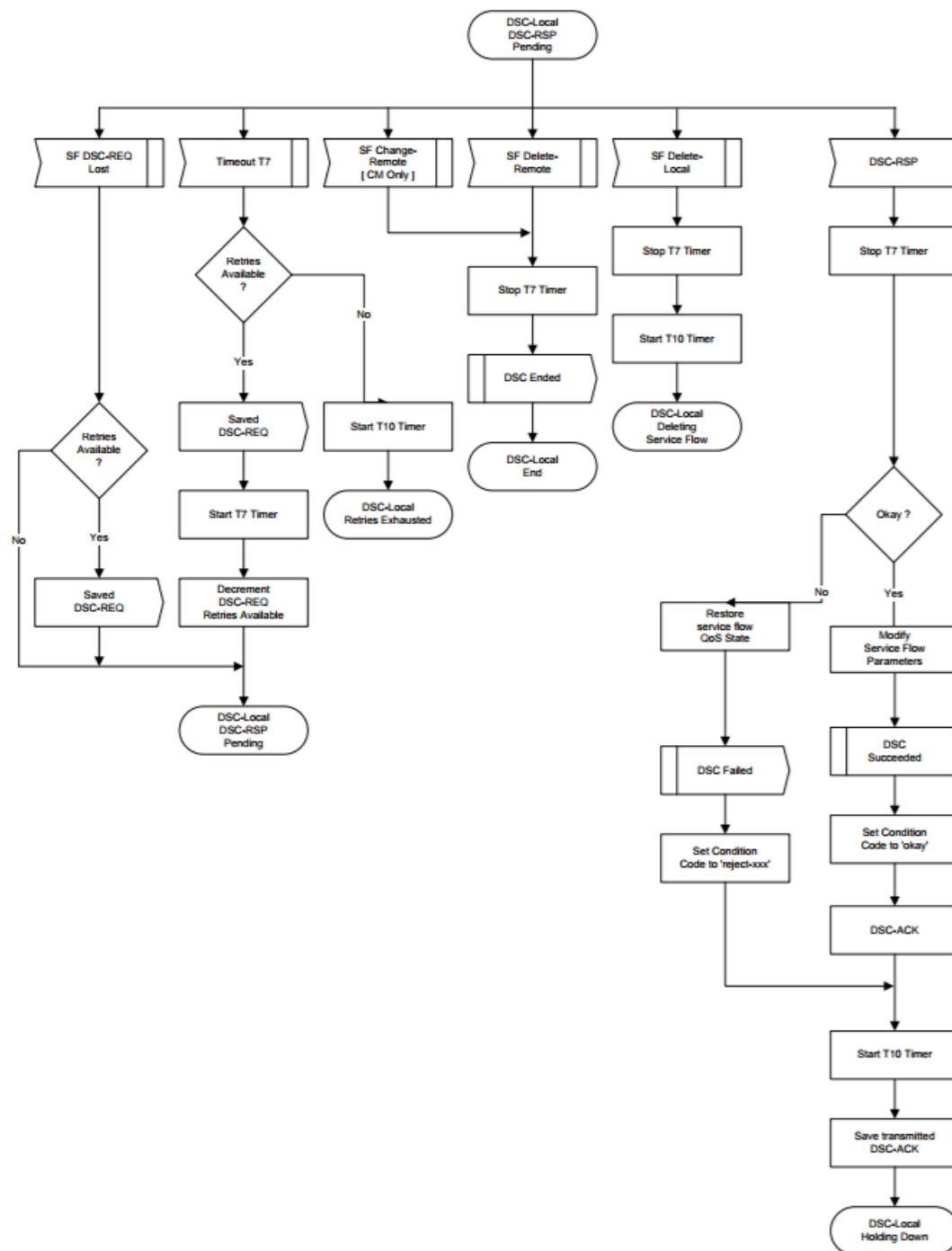
Figure 199 - DSC-Locally Initiated Transaction DSC-RSP Pending State Flow Diagram
