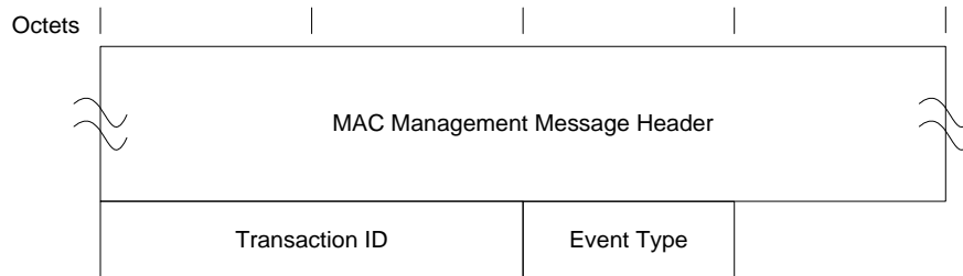
Figure 77 - CM STATUS-ACK message
