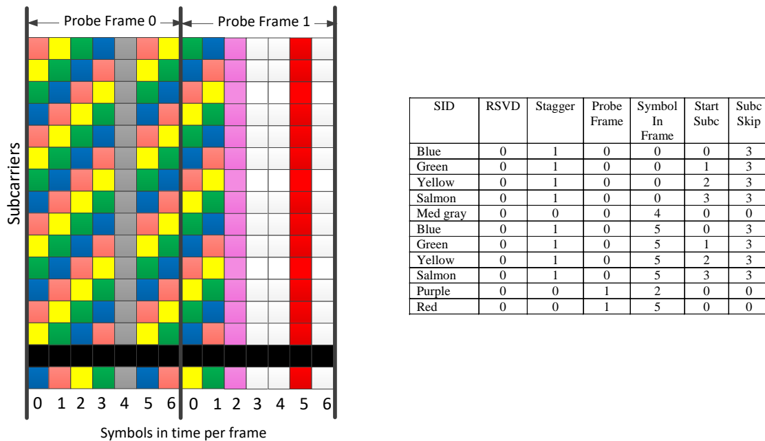
Figure 41 - Sample Probe Frame and P-IEs
