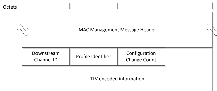
Figure 79 - Downstream Profile Descriptor
