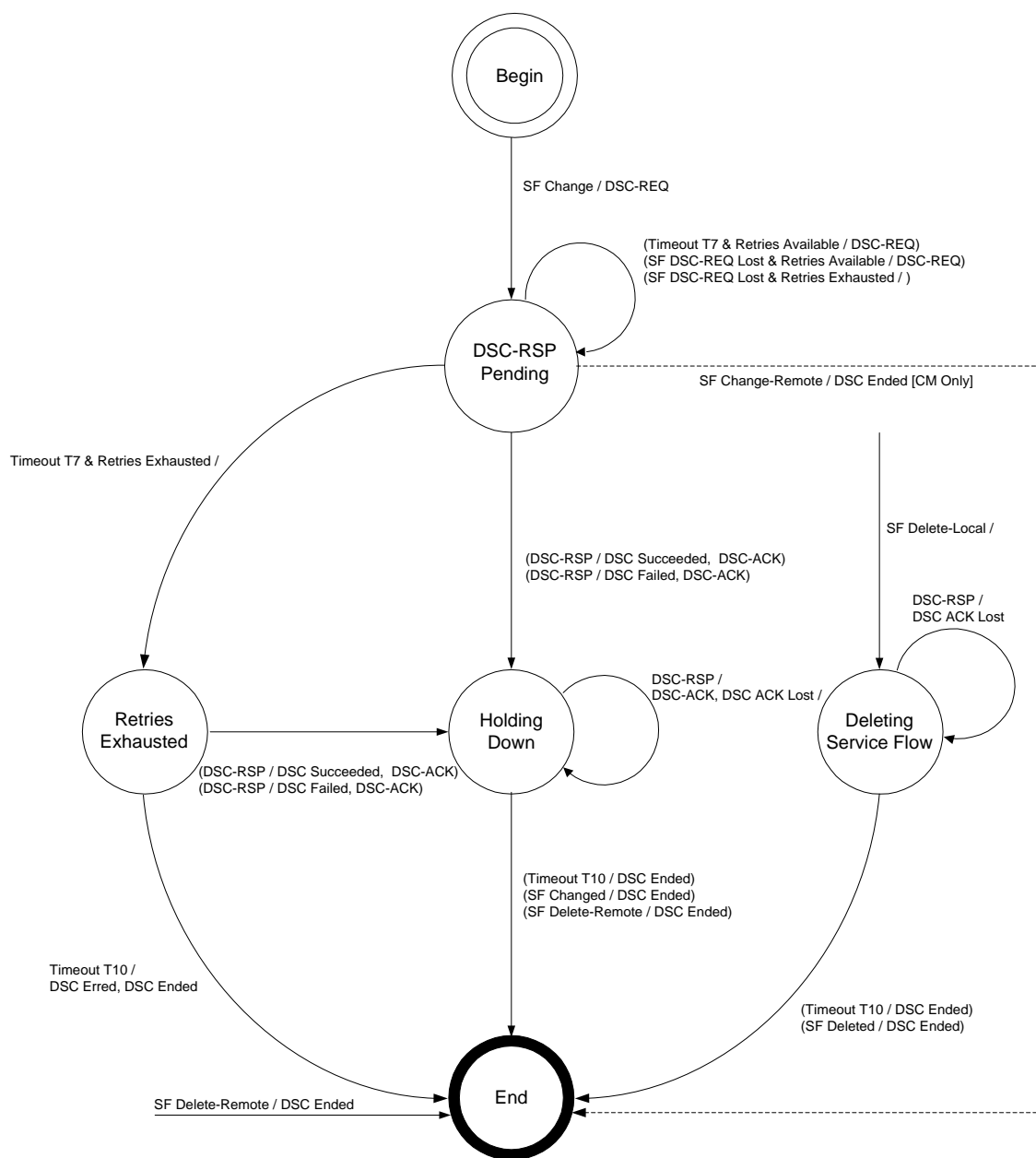
Figure 180 - DSC-Locally Initiated Transaction State Transition Diagram
