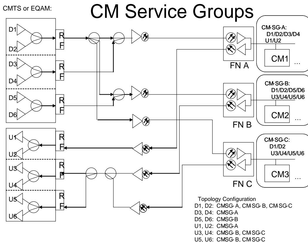
Figure 11 - CM Topology Configuration Example
