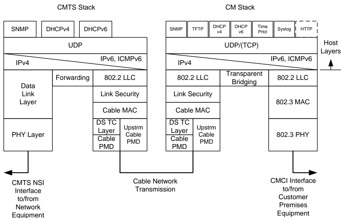
Figure 116 - DOCSIS Protocol Stacks
