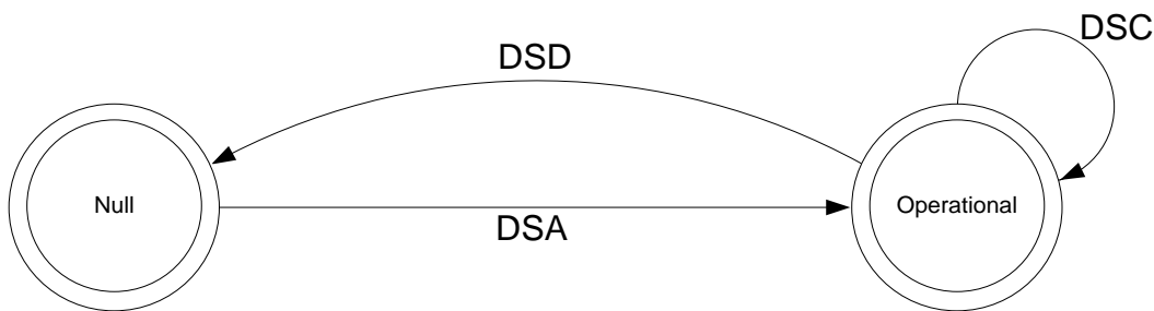
Figure 176 - Dynamic Service Flow Overview
