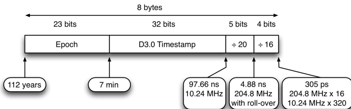
Figure 95 - Extended Timestamp Structure
