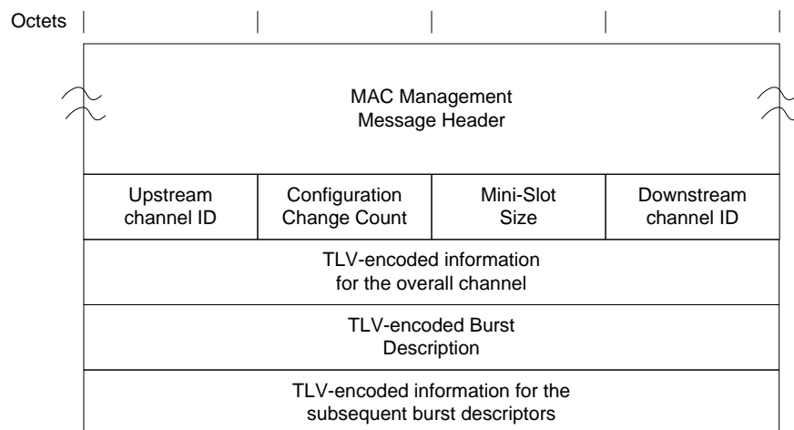
Figure 31 - Upstream Channel Descriptor
