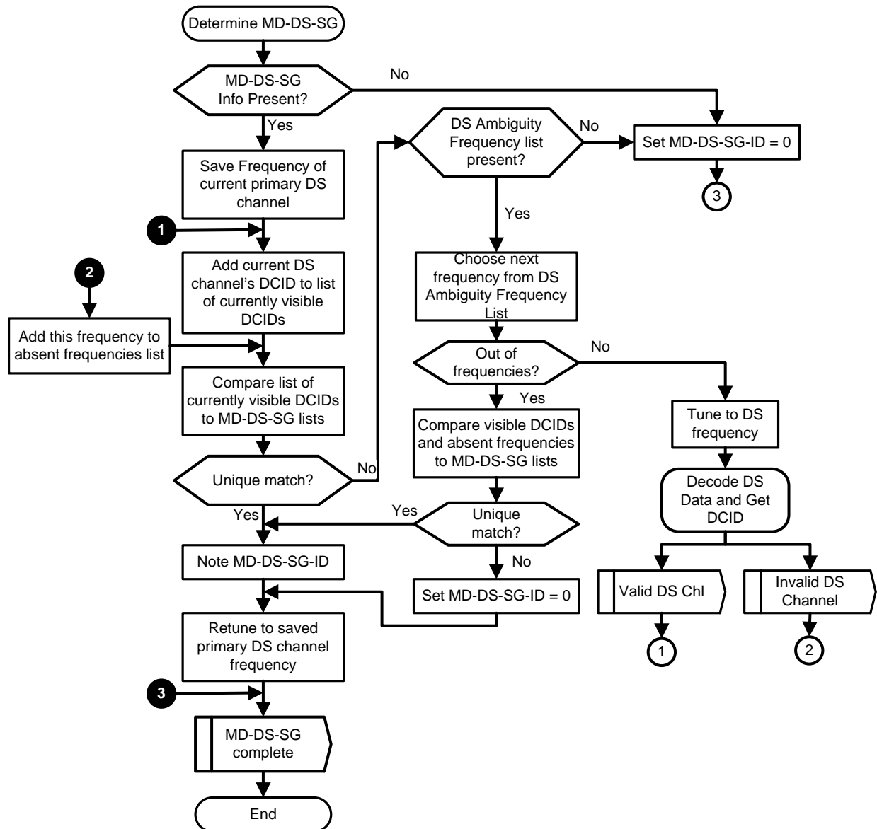
Figure 126 - Determine MD-DS-SG
