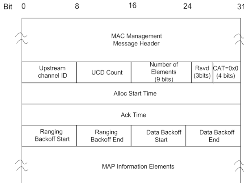
Figure 37 - Version 5 MAP Format for Non-Probe Frames
