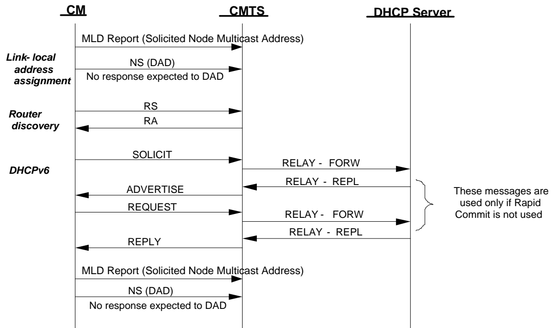
Figure 145 - IPv6 Provisioning Message Flow
