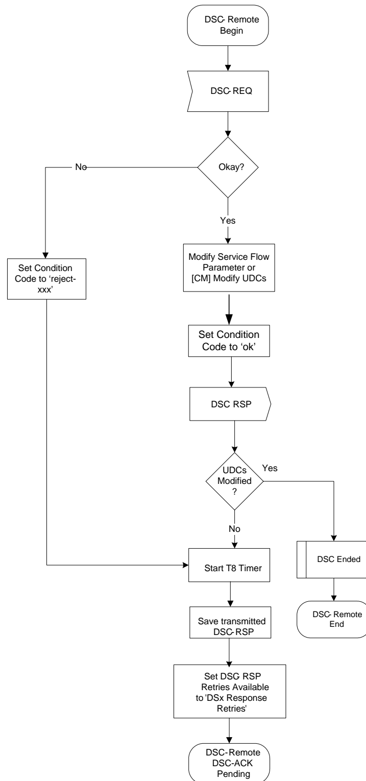
Figure 203 - DSC-Remotely Initiated Transaction Begin State Flow Diagram
