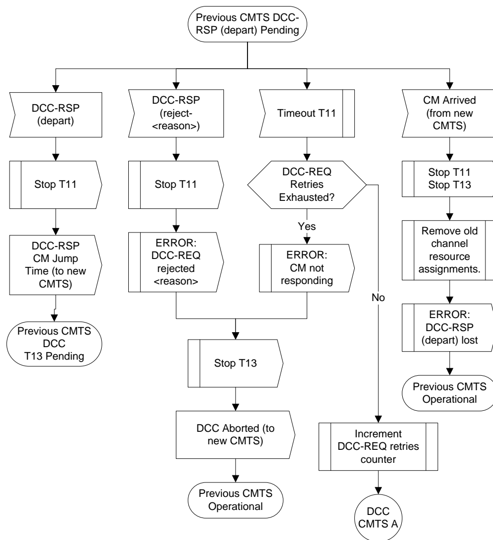
Figure 215 - Dynamically Changing Channels: CMTS View Part 2
