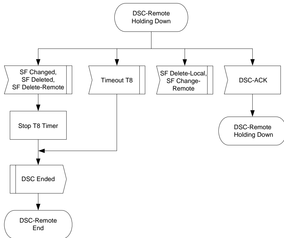
Figure 205 - DSC-Remotely Initiated Transaction Holding Down State Flow Diagram
