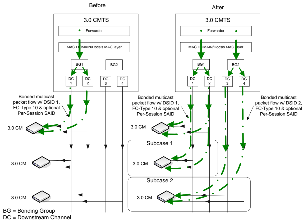
Figure 262 - Multicast Session Replication to Clients Behind Two 3.0 CMs
