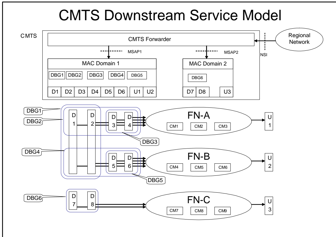
Figure 17 - CMTS Downstream Service Model
