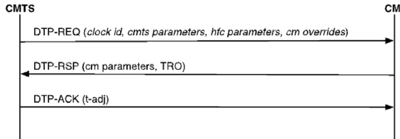
Figure 173 - CMTS is DTP Master
