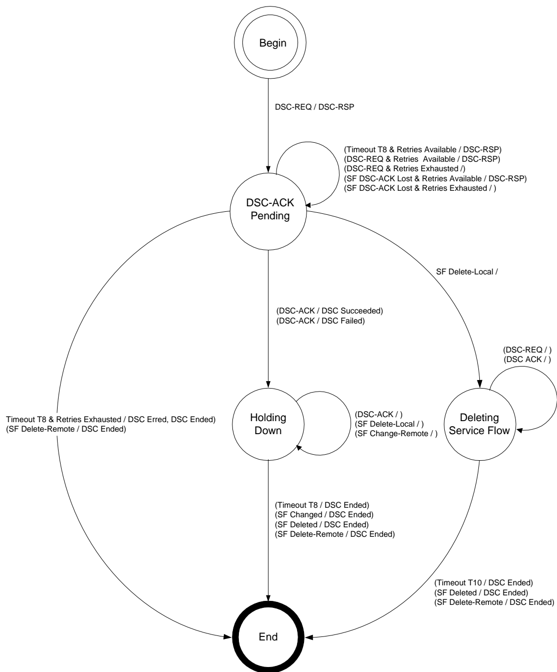
Figure 181 - DSC-Remotely Initiated Transaction State Transition Diagram
