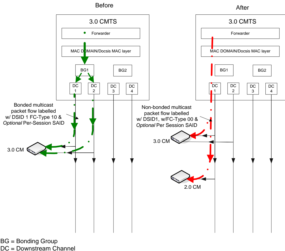
Figure 258 - Multicast Session Replication to Clients Behind Both a 3.0 CM and a 2.0 CM on the Same Downstream Channel (Subcase 1)
