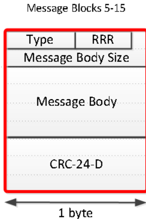
Figure 94 - Generic Format for Message Blocks 5-15
