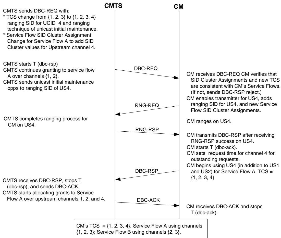
Figure 264 - Adding a Channel to the TCS and making a Service Flow SID Cluster Assignment
