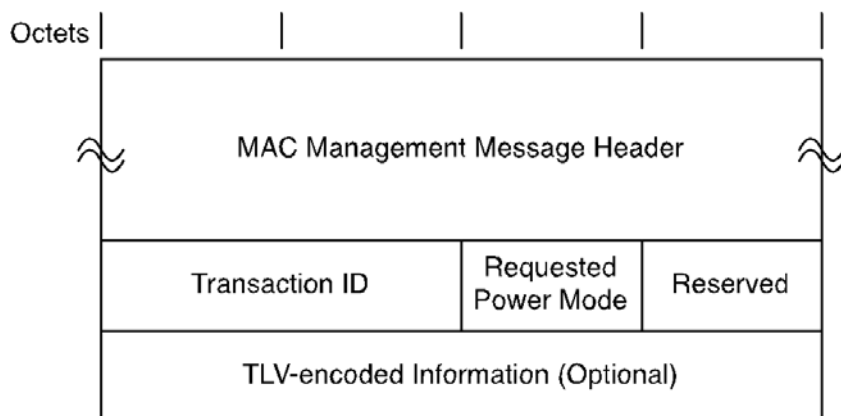
Figure 75 - Energy Management Request Message
