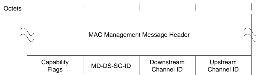
Figure 44 - B-INIT-RNG-REQ Format
