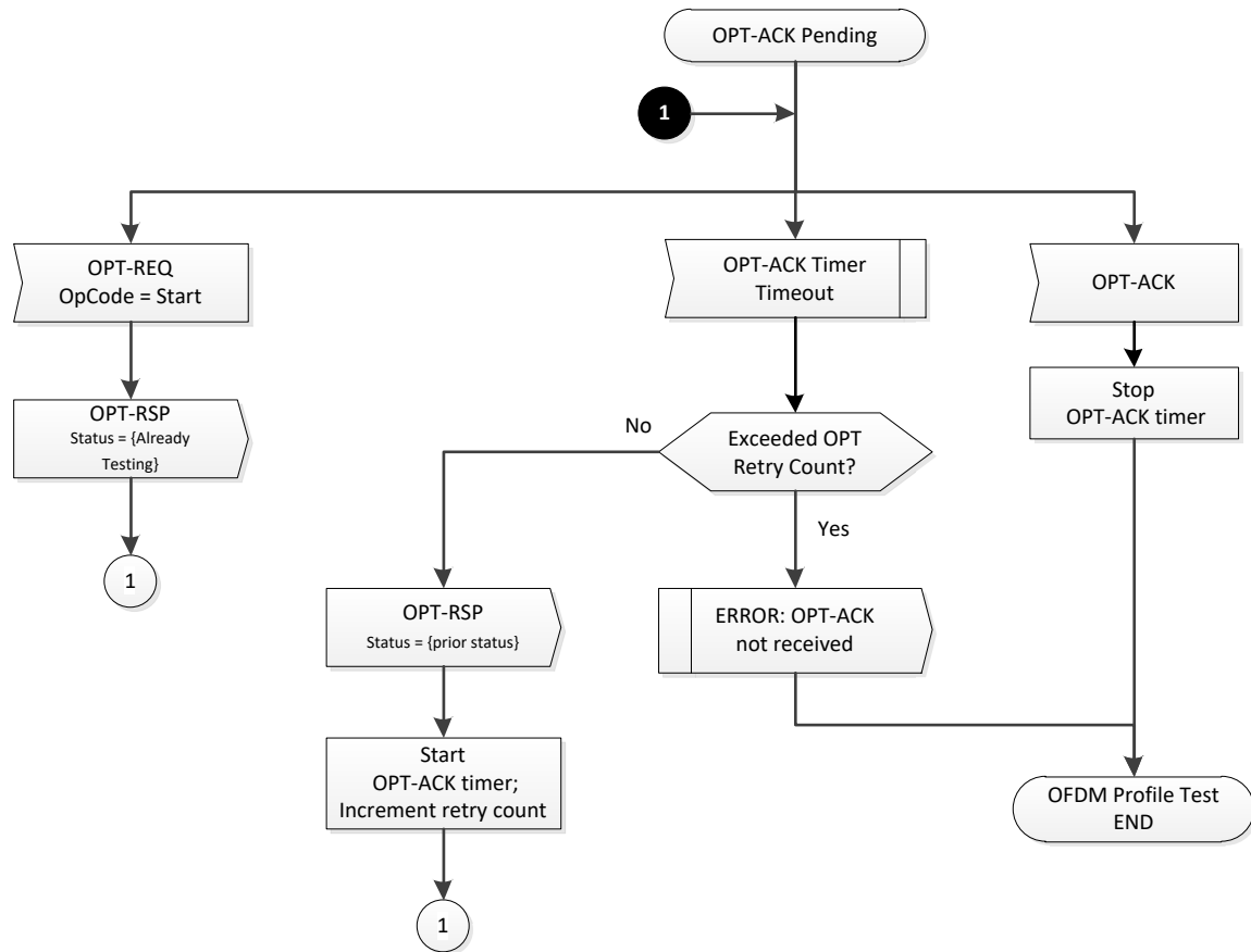
Figure 162 - CM OPT State Machine - OPT-ACK Pending
