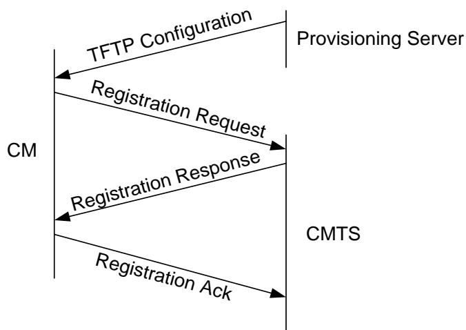
Figure 107 - Registration Message Flow
