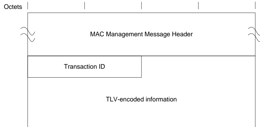
Figure 73 - CM-CTRL-REQ
