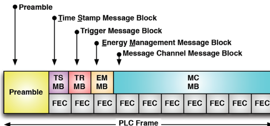
Figure 89 - PLC Frame
