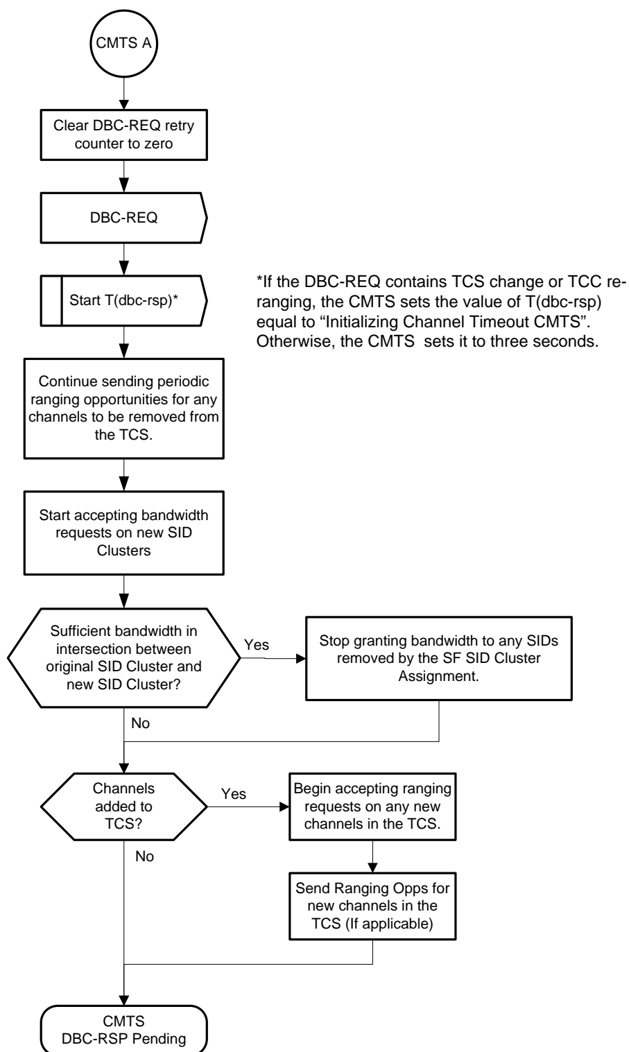
Figure 220 - CMTS DBC Request (part 2)
