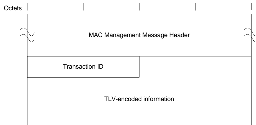
Figure 84 - DTP Request Message
