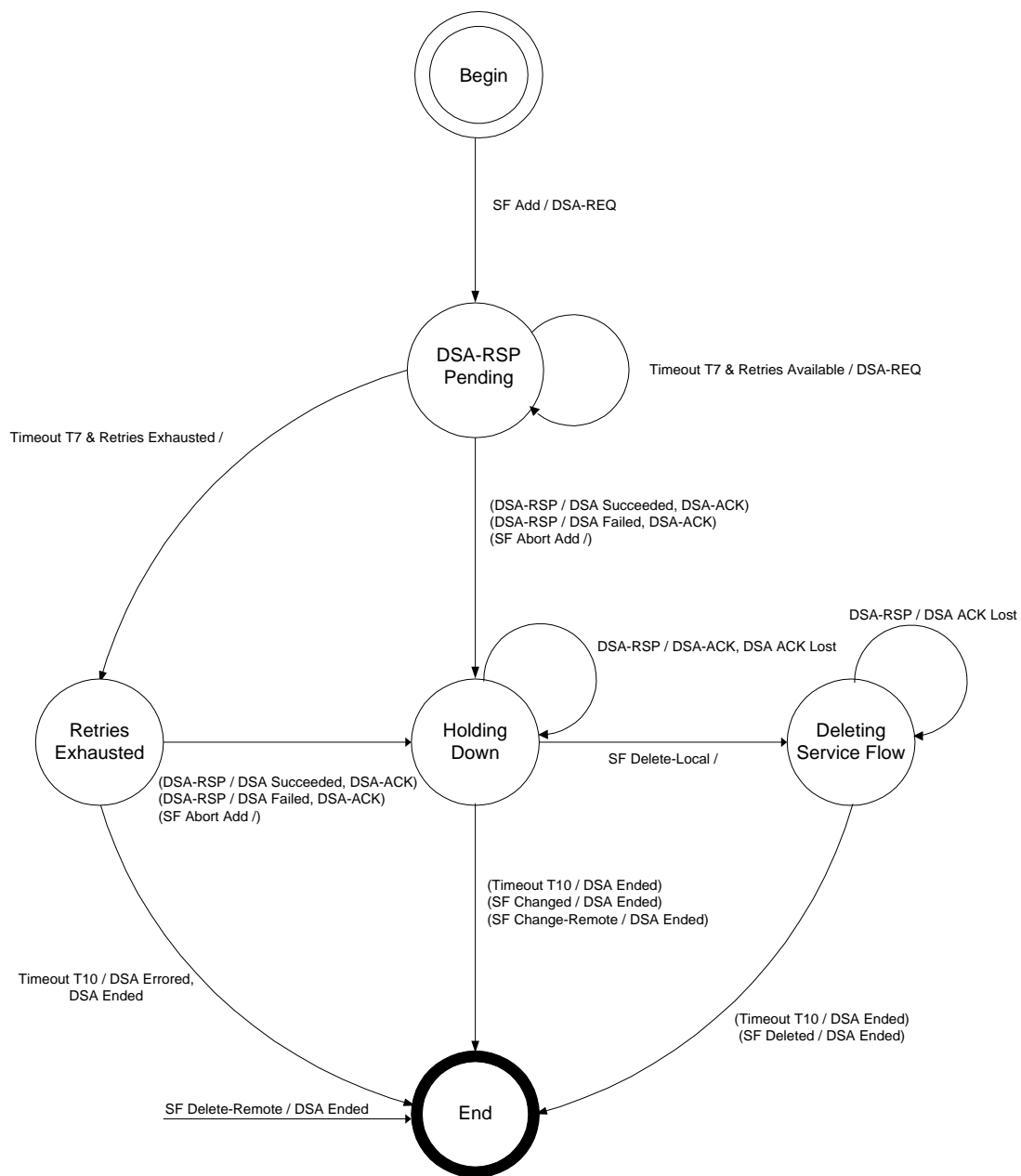
Figure 178 - DSA-Locally Initiated Transaction State Transition Diagram
