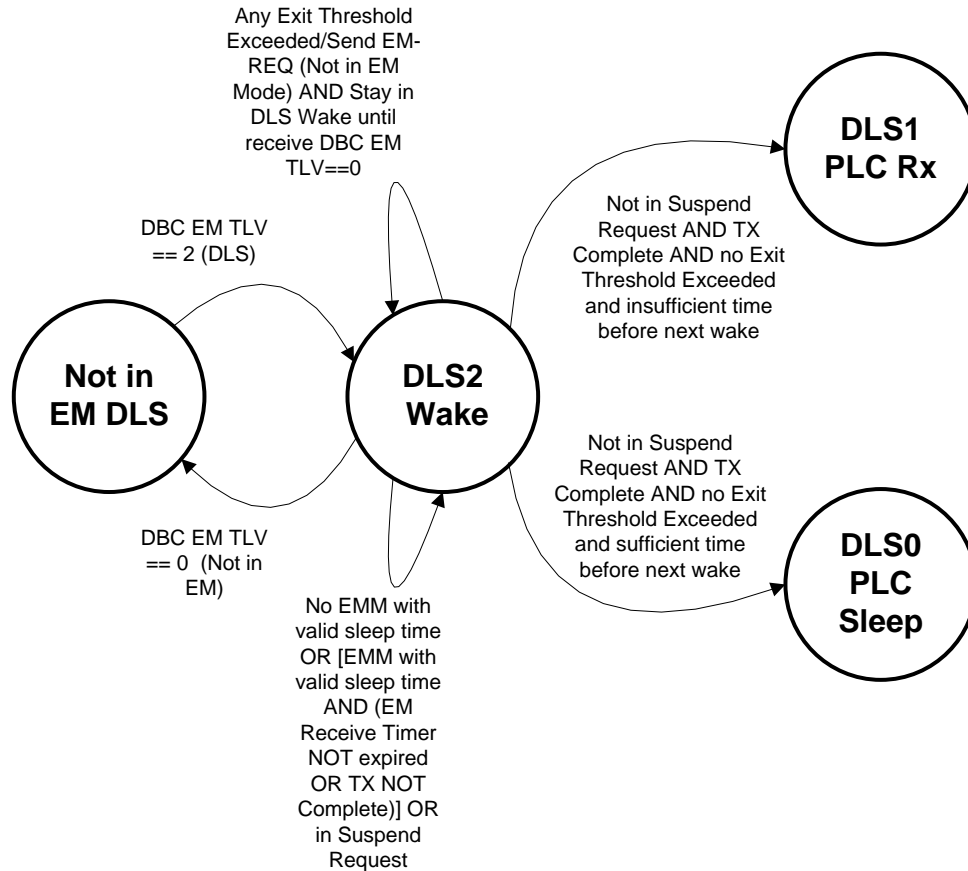
Figure 234 - Wake Substate transitions for DLS Mode
