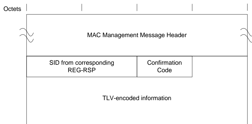
Figure 54 - Registration Acknowledgment
