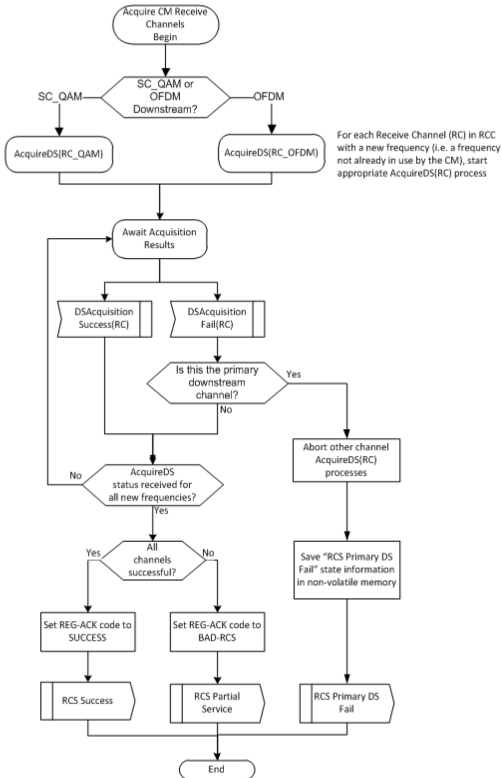
Figure 147 - CM Acquires Receive Channels
