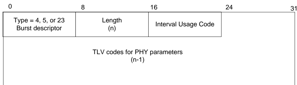
Figure 33 - Top-Level Encoding for Burst Descriptors
