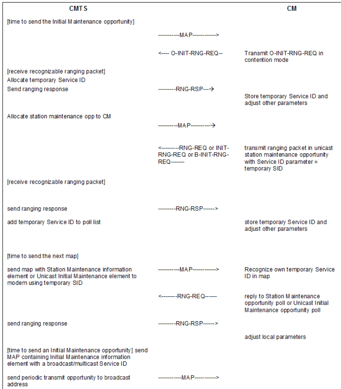
Figure 133 - Ranging and Automatic Adjustments Procedure for OFDMA Upstreams
