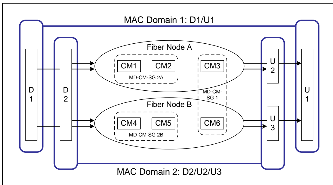
Figure 15 - Multiple MAC Domains per Fiber Node
