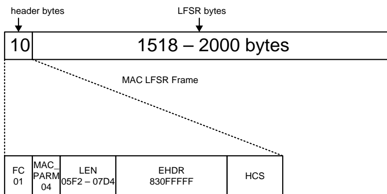
Figure 164 - MAC LFSR Frame
