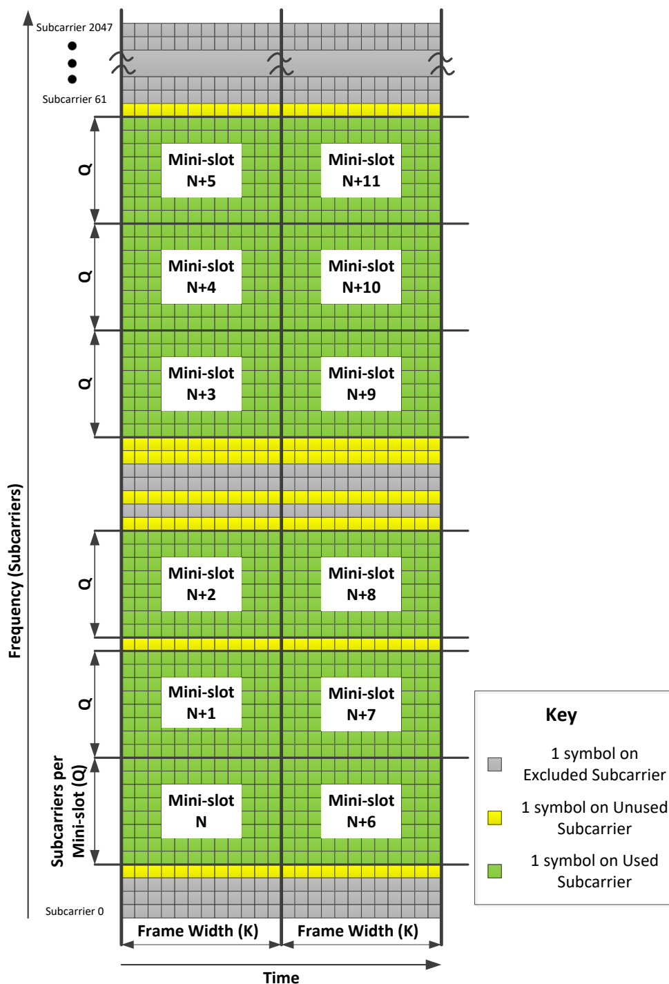
Figure 35 - Example Minislot Mapping for OFDMA
