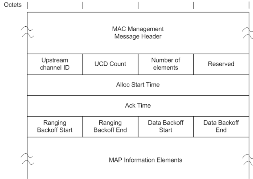
Figure 36 - Version 1 MAP Format
