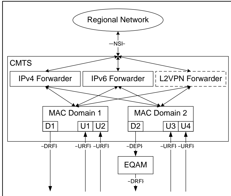
Figure 7 - CMTS Internal Forwarding Model
