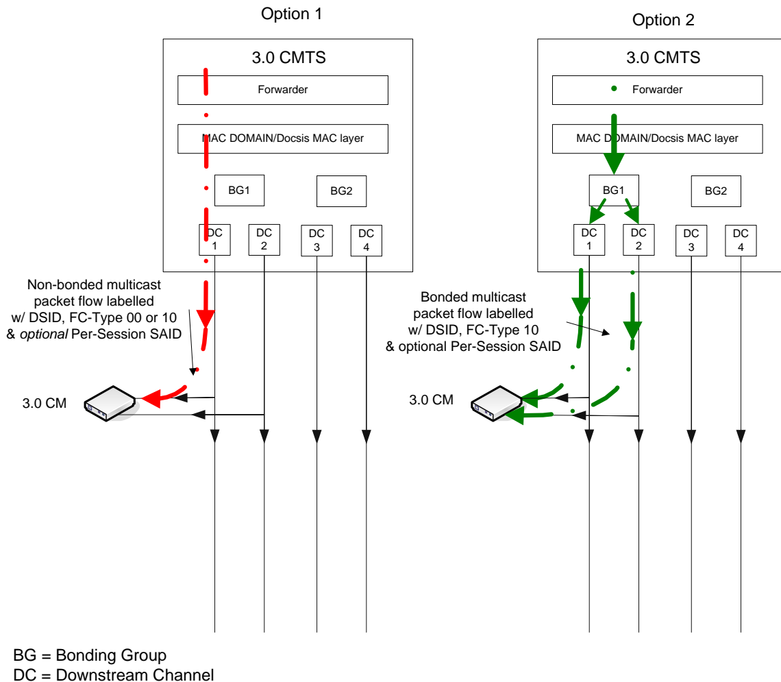
Figure 257 - Multicast Session Replication for a client behind a 3.0 CM
