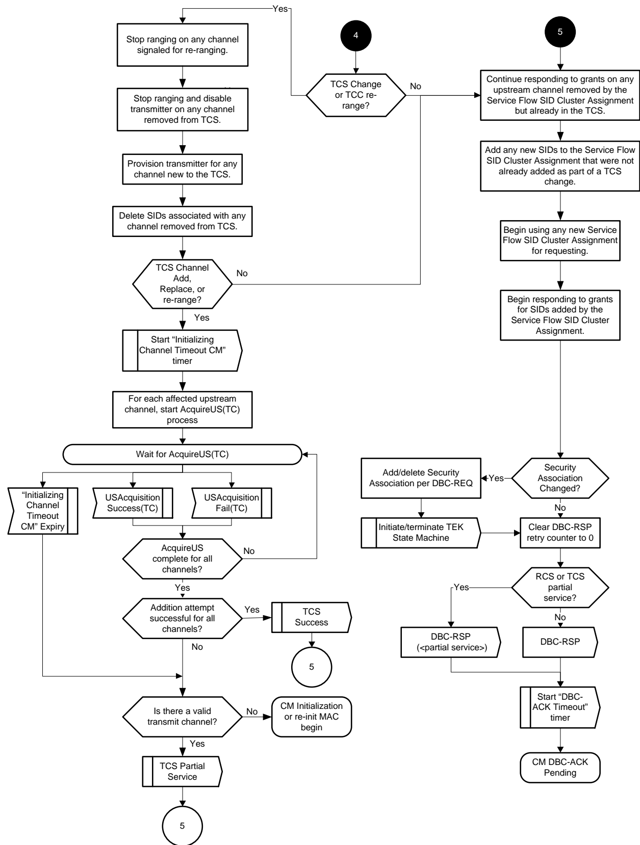
Figure 224 - CM DBC-RSP (part 2)
