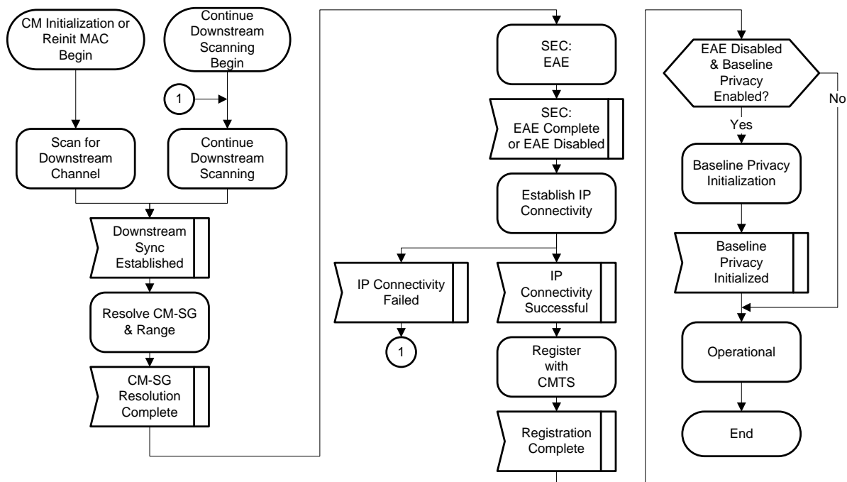
Figure 121 - Cable Modem Initialization Overview
