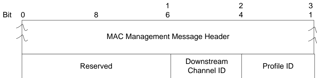
Figure 83 - The OFDM Profile Test Acknowledge (OPT-ACK) message
