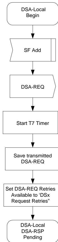
Figure 186 - DSA-Locally Initiated Transaction Begin State Flow Diagram
