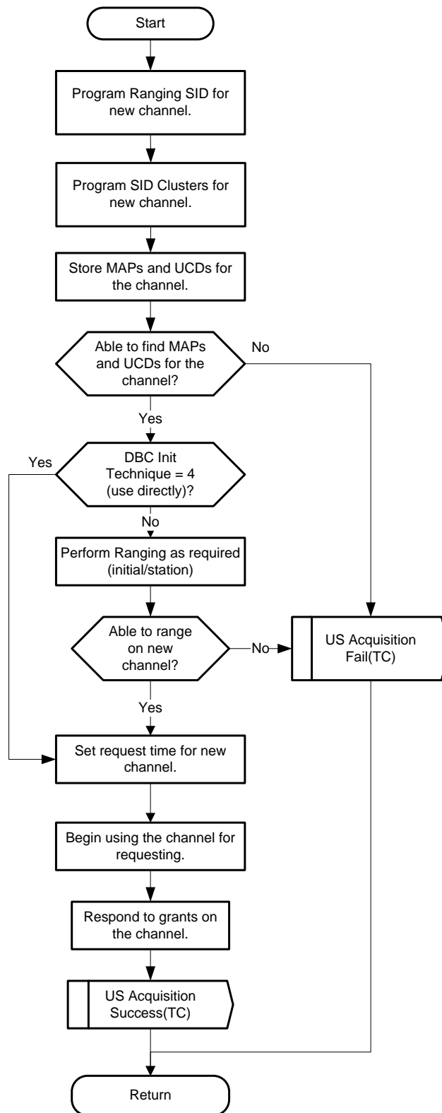
Figure 228 - CM AcquireUS Procedure
