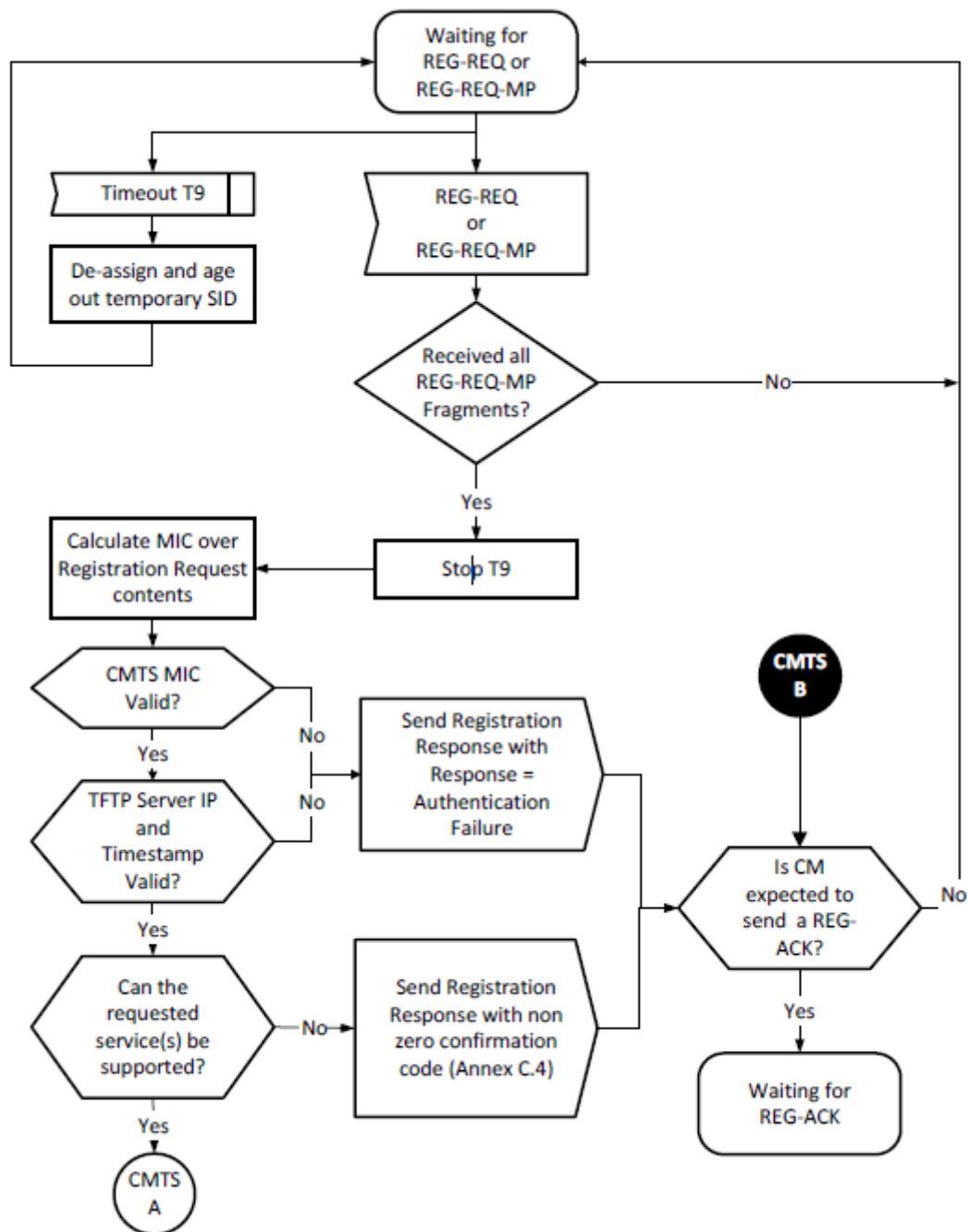
Figure 153 - CMTS Registration - Begin
