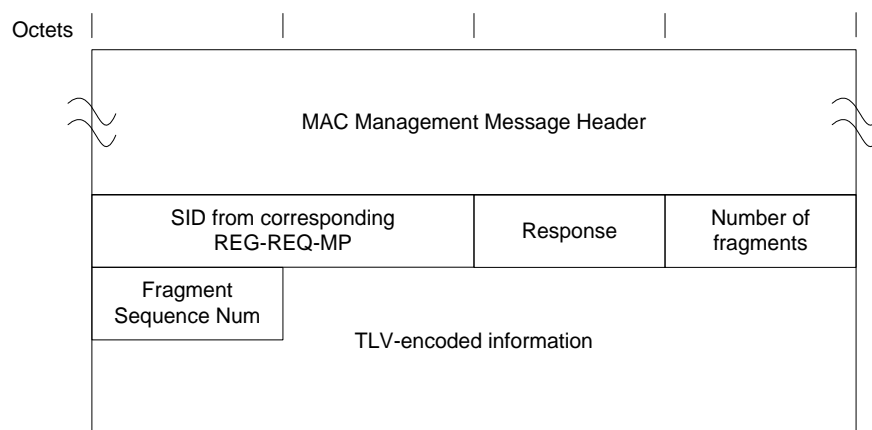
Figure 53 - Multipart Registration Response Format
