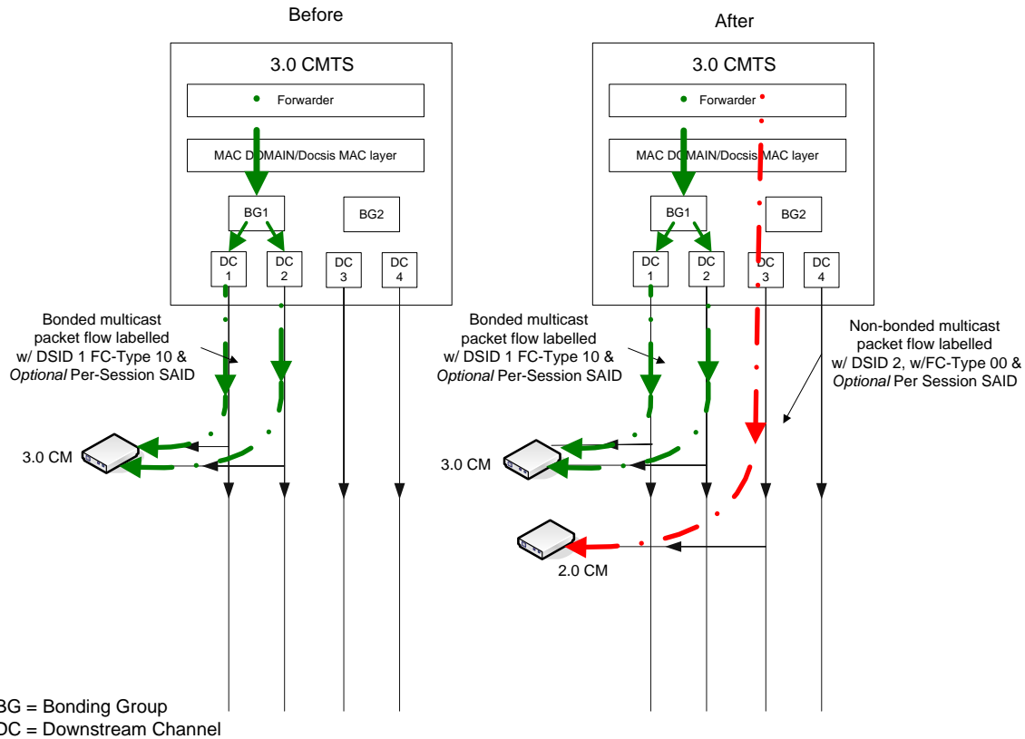
Figure 260 - Multicast Session Replications to Clients Behind Both a 3.0 CM and a 2.0 CM on Different Downstream Channel (Subcase 3)
