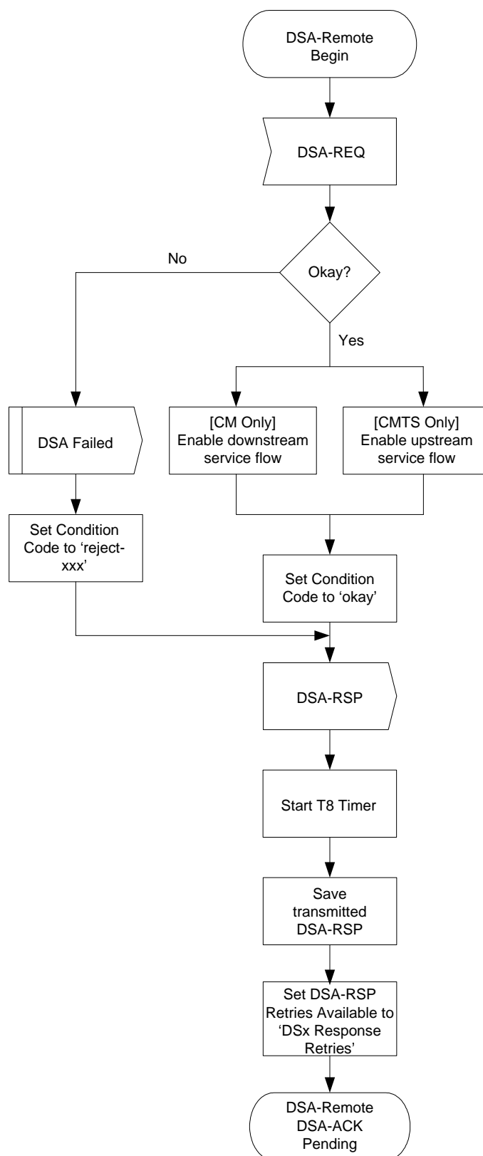
Figure 191 - DSA-Remotely Initiated Transaction Begin State Flow Diagram
