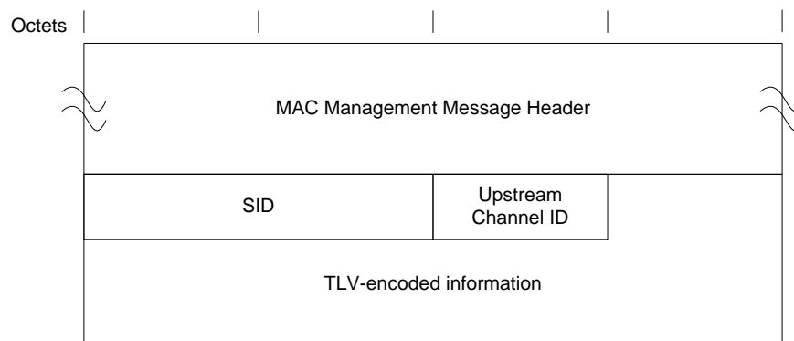
Figure 46 - Ranging Response
