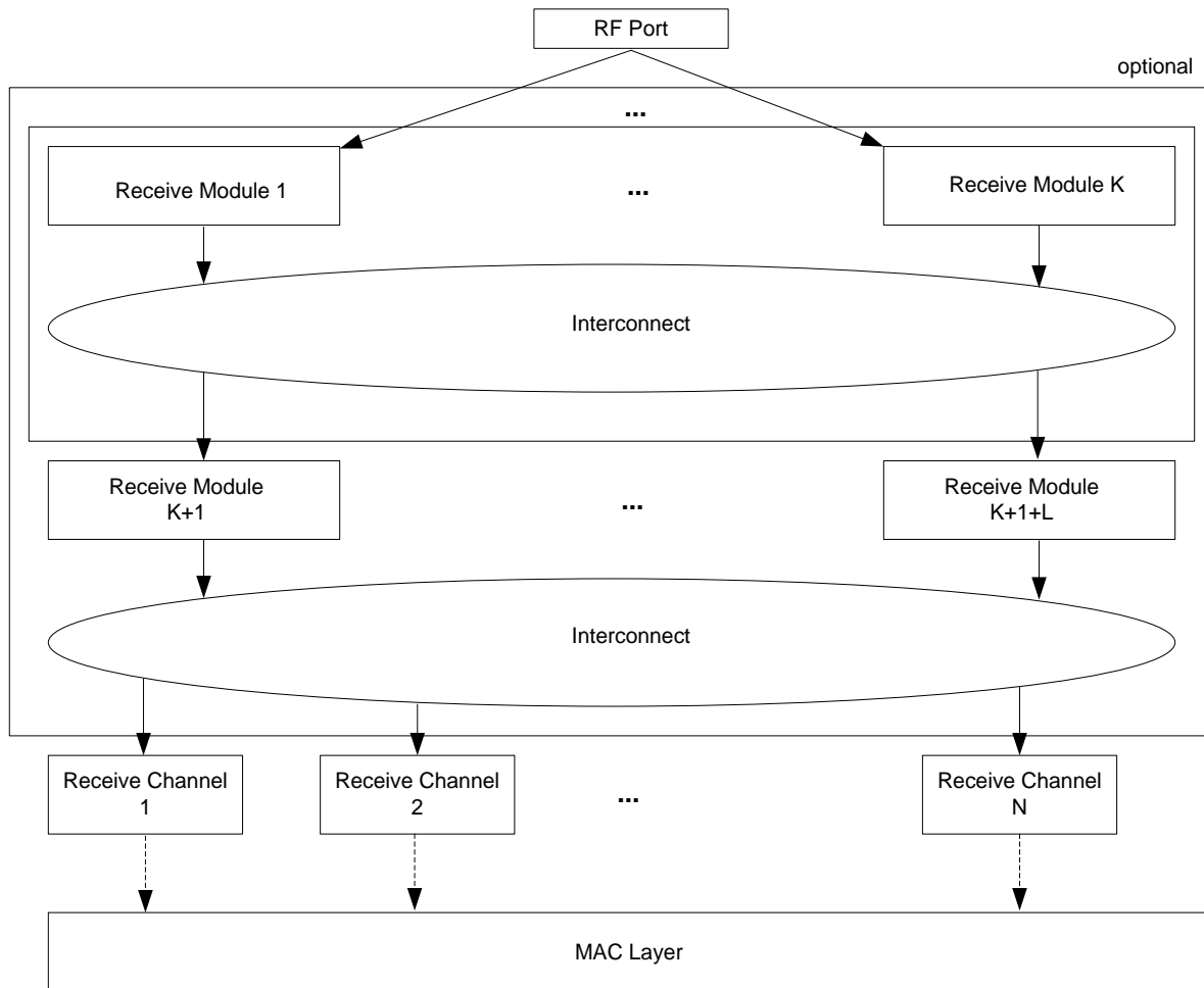
Figure 114 - Interconnection between Receive Channels and Receive Modules
