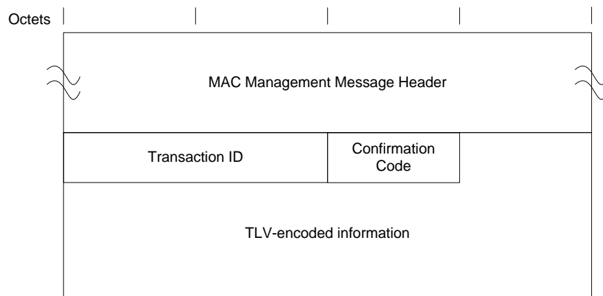
Figure 59 - Dynamic Service Change - Response
