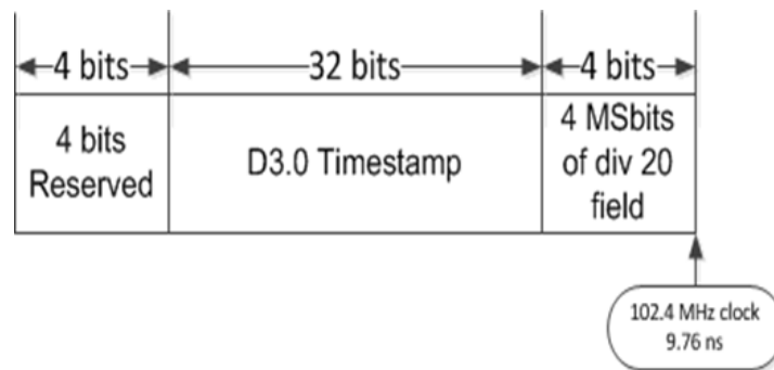
Figure 32 - OFDMA Timestamp Snapshot subTLV relationship to the Extended Timestamp
