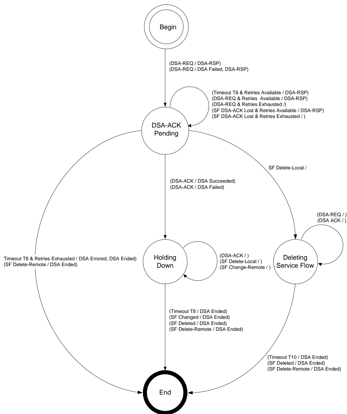
Figure 179 - DSA-Remotely Initiated Transaction State Transition Diagram
