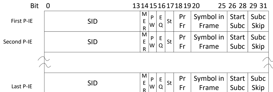
Figure 40 - Probe Information Element Structure
