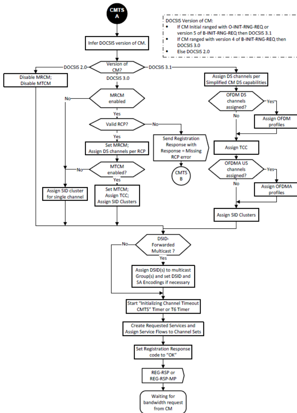
Figure 154 - CMTS Registration - Continued
