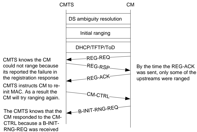
Figure 252 - Example 1 - Modem can't range on all upstreams
