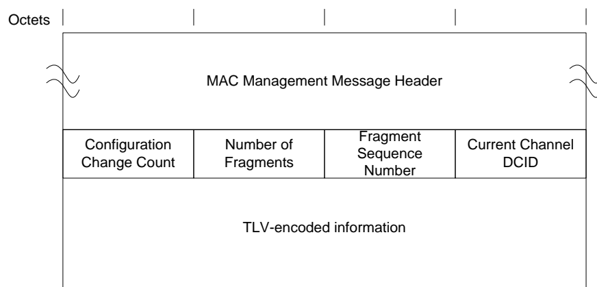
Figure 66 - MAC Domain Descriptor
