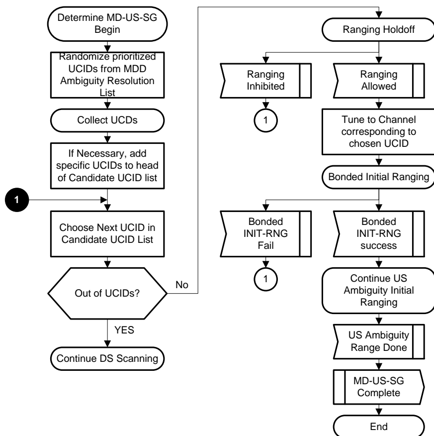
Figure 127 - Determine MD-US-SG
