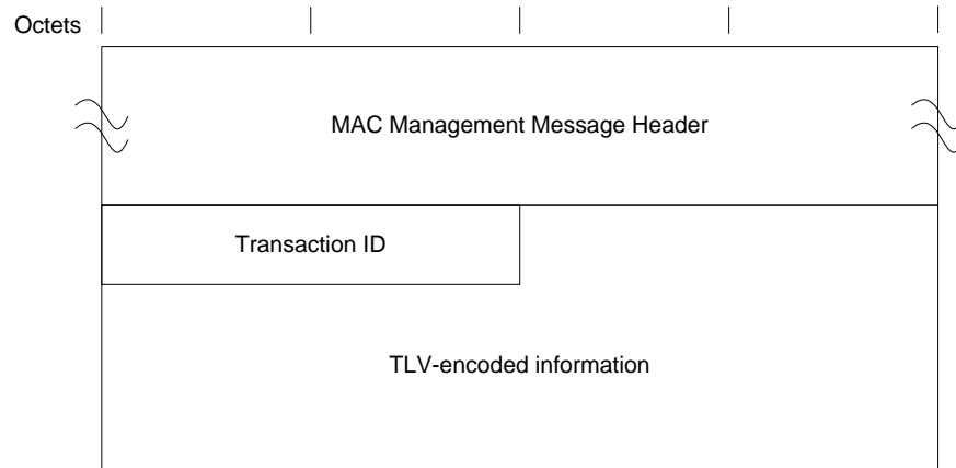
Figure 58 - Dynamic Service Change - Request
