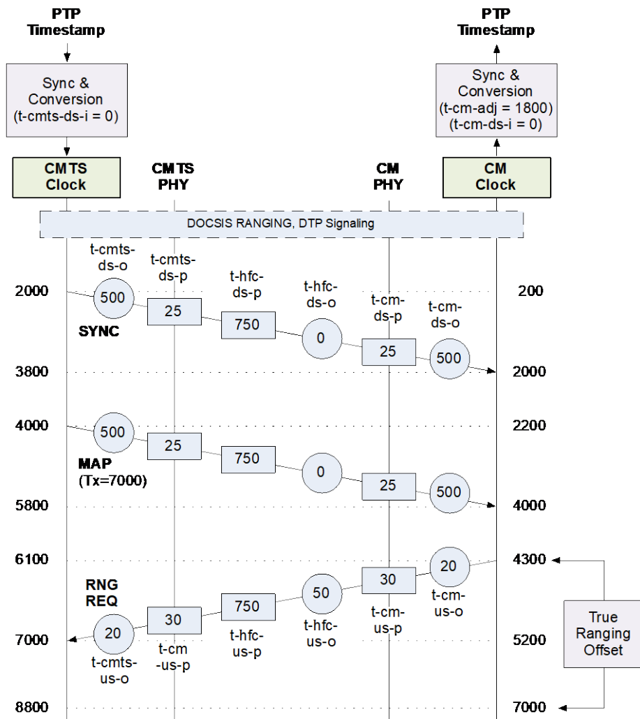
Figure 172 - True Ranging Offset Example
