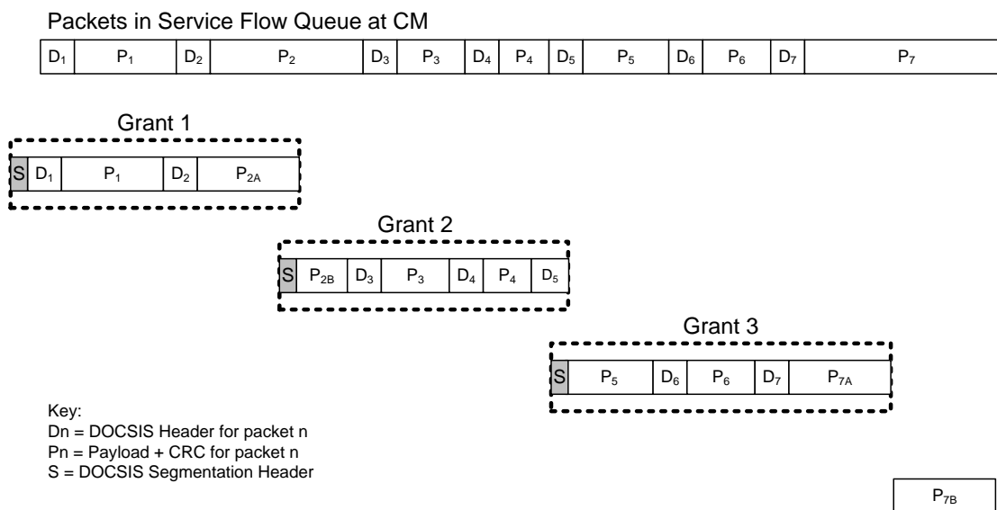
Figure 102 - CCF Using Segment Headers
