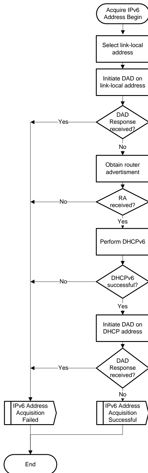
Figure 143 - IPv6 Address Acquisition
