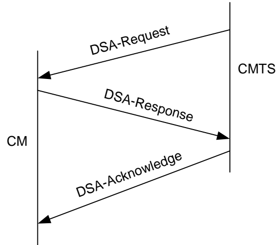
Figure 109 - Dynamic Service Addition Message Flow - CMTS Initiated
