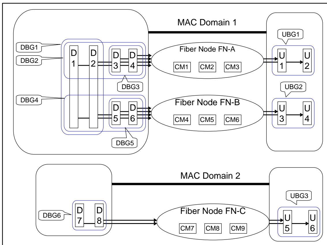
Figure 16 - Bonding Group Example
