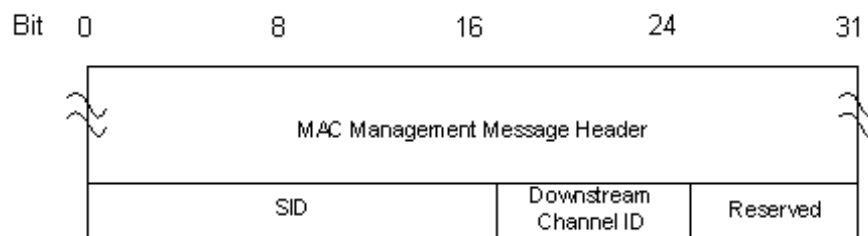
Figure 42 - RNG-REQ Format
