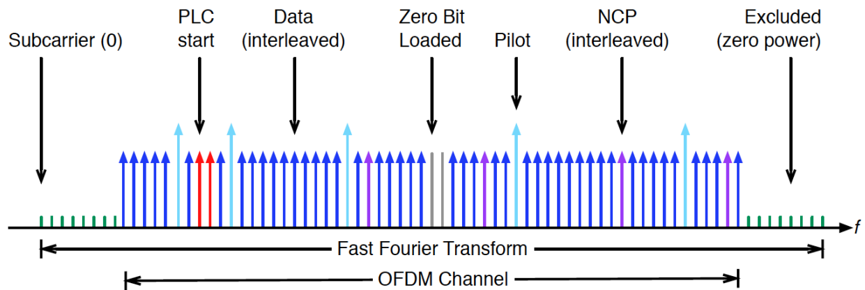
Figure 80 - OFDM Channel with PLC After Interleaving
