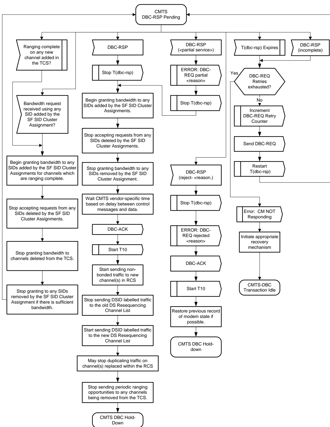
Figure 221 - CMTS DBC-RSP Pending
