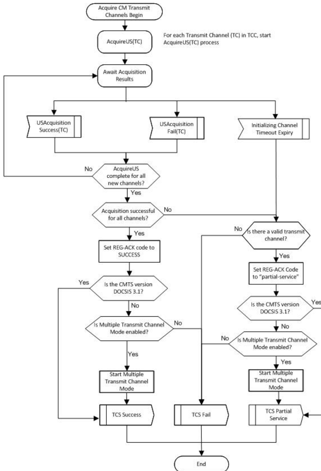
Figure 150 - CM Acquires Transmit Channels
