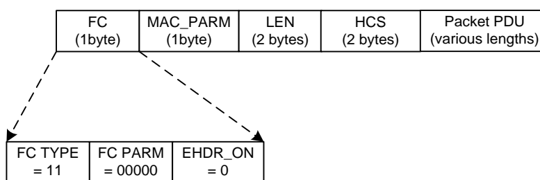
Figure 21 - Timing MAC Header
