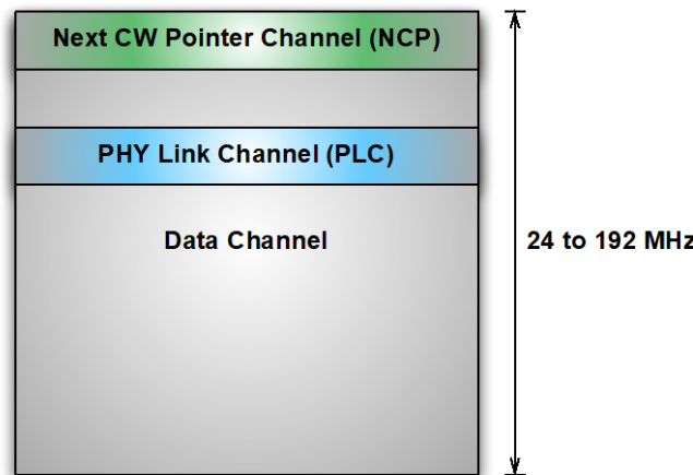
Figure 88 - OFDM Channel with PLC Prior to Interleaving
