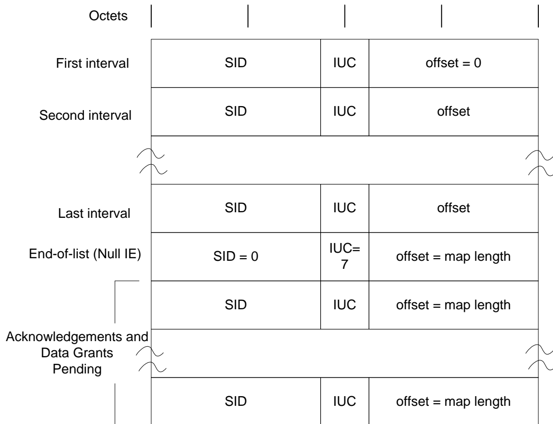
Figure 38 - MAP Information Element Structure
