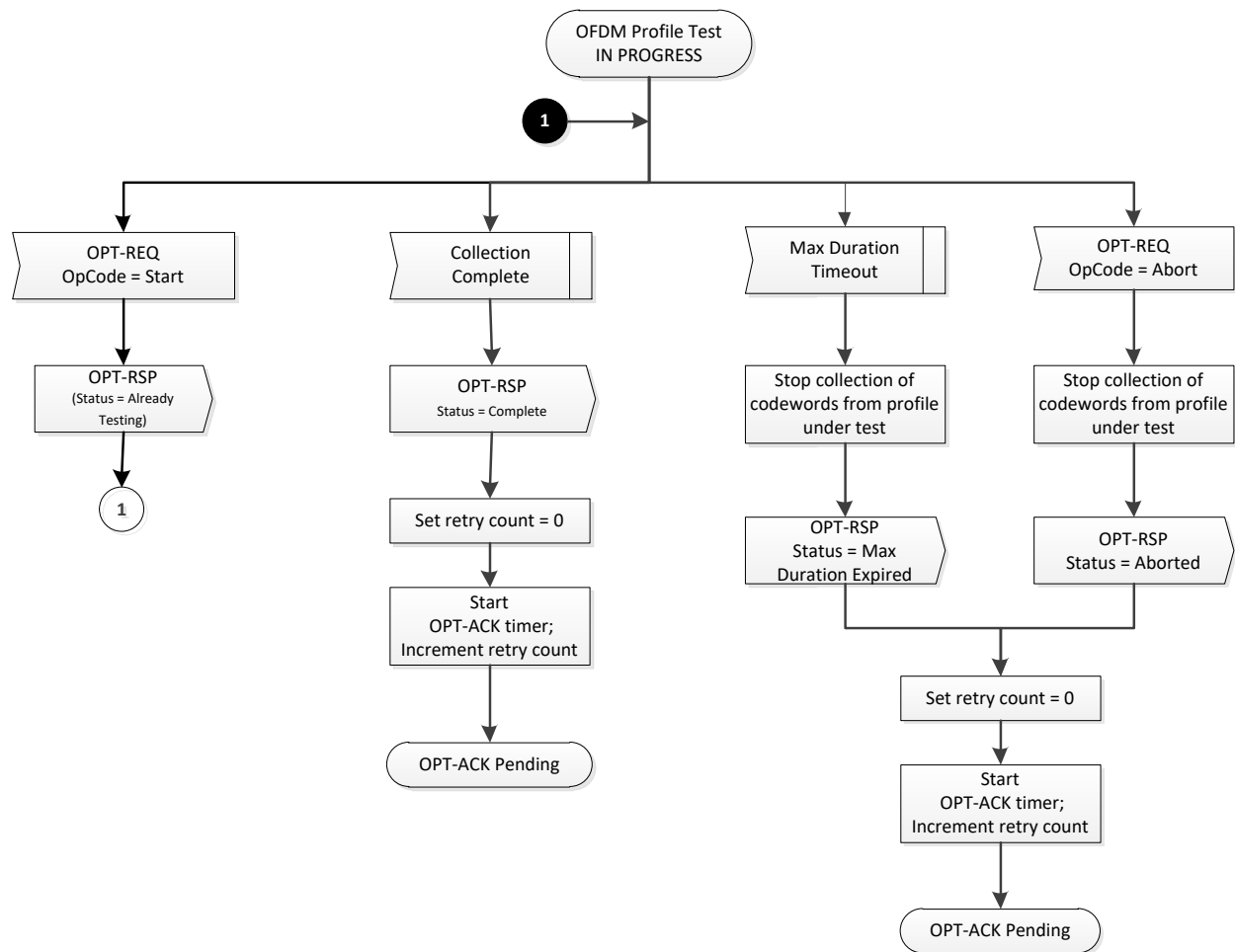
Figure 161 - CM OPT State Machine - OFDM Profile Test in Progress
