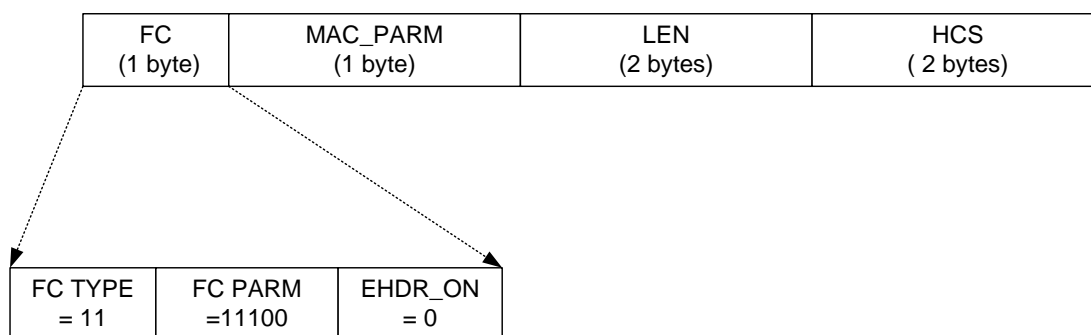
Figure 26 - Concatenation MAC Header Format
