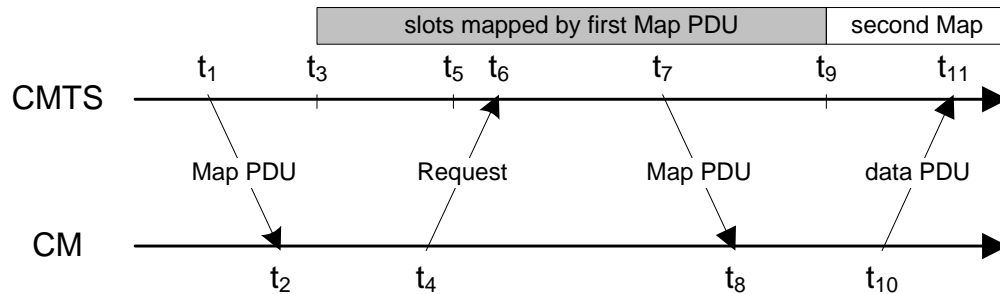
Figure 97 - Protocol Example
