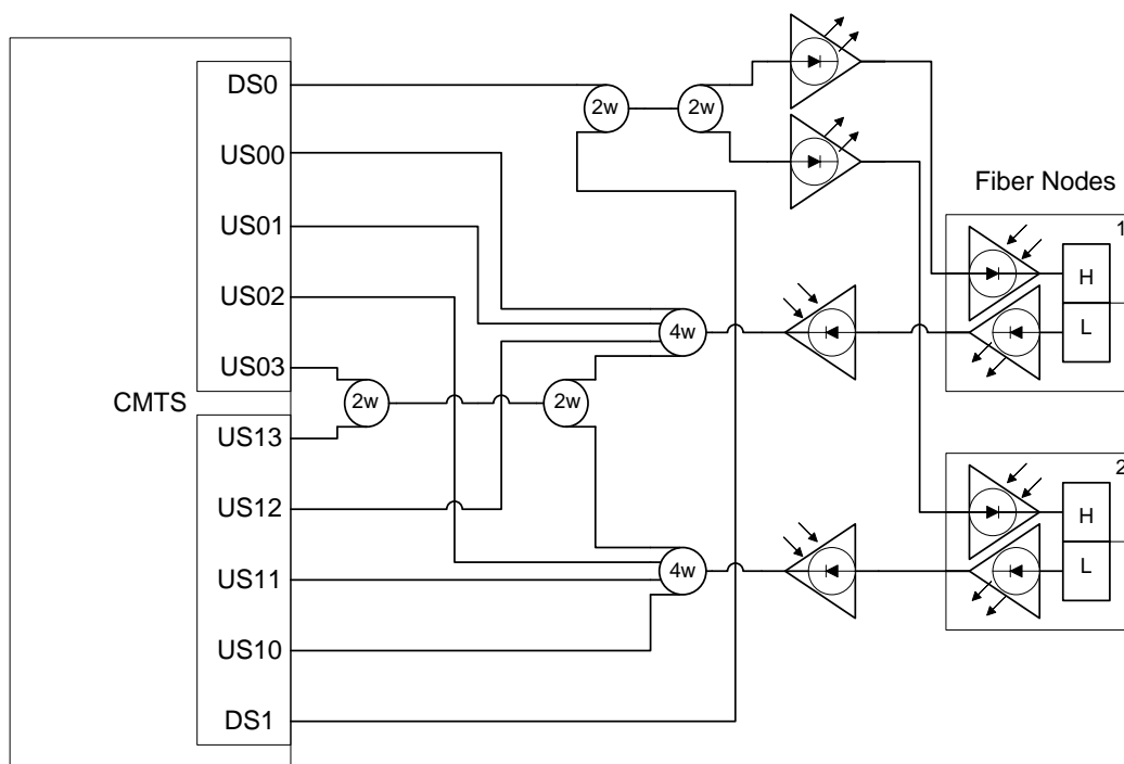
Figure 268 - Example Combining Network 2
