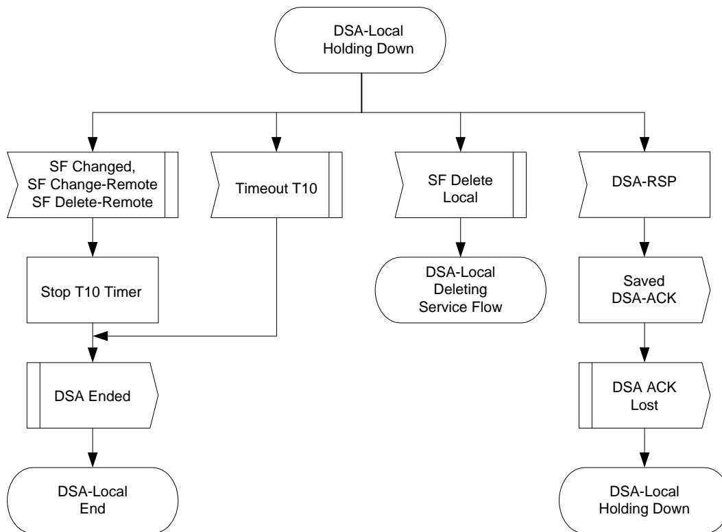
Figure 188 - DSA-Locally Initiated Transaction Holding State Flow Diagram
