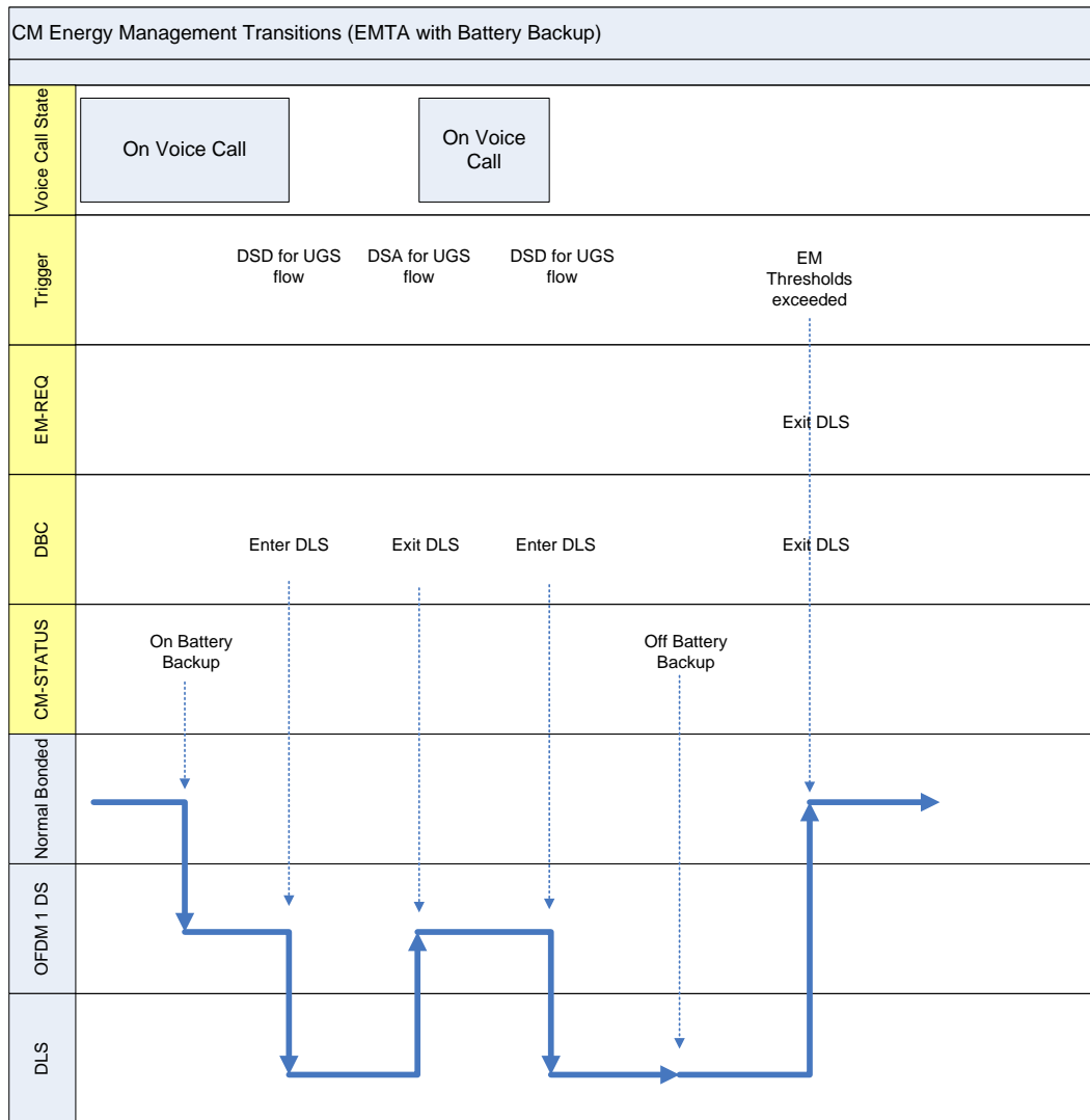
Figure 236 - Example Interaction between Battery Backup and DLS mode
