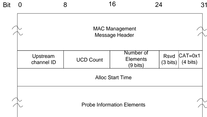
Figure 39 - Version 5 MAP Format for probe frames (P-MAPs)
