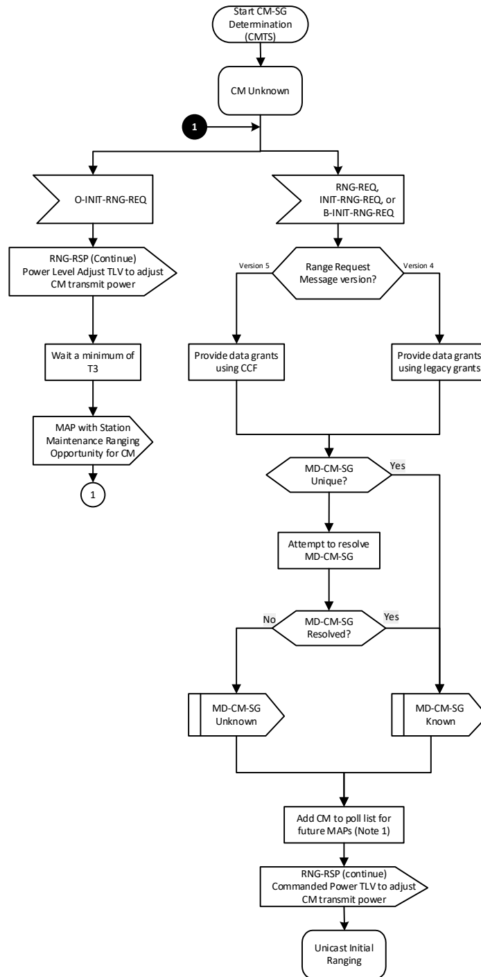
Figure 135 - CM-SG Determination - CMTS
