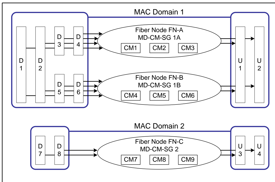
Figure 14 - Example MAC Domain Channel Assignment
