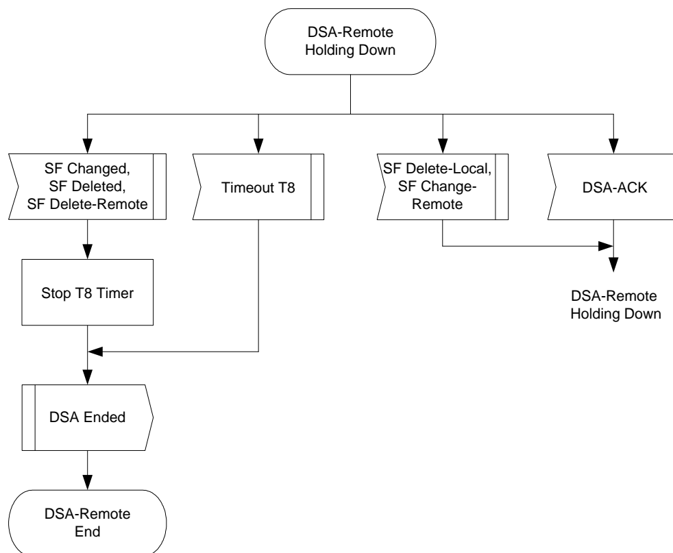
Figure 193 - DSA-Remotely Initiated Transaction Holding Down State Flow Diagram
