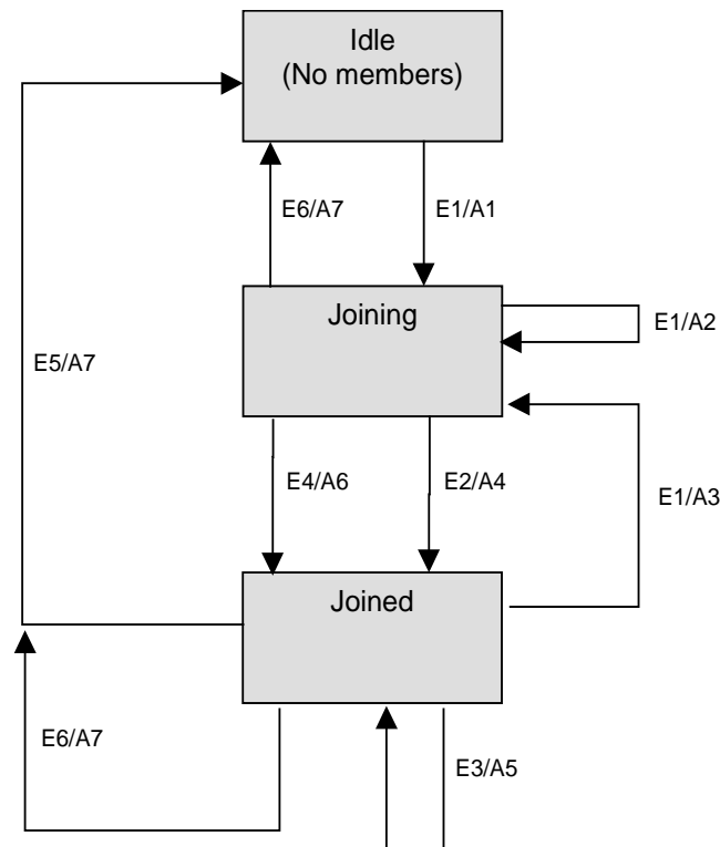
Figure 263 - IGMP Support - CM Passive Mode
