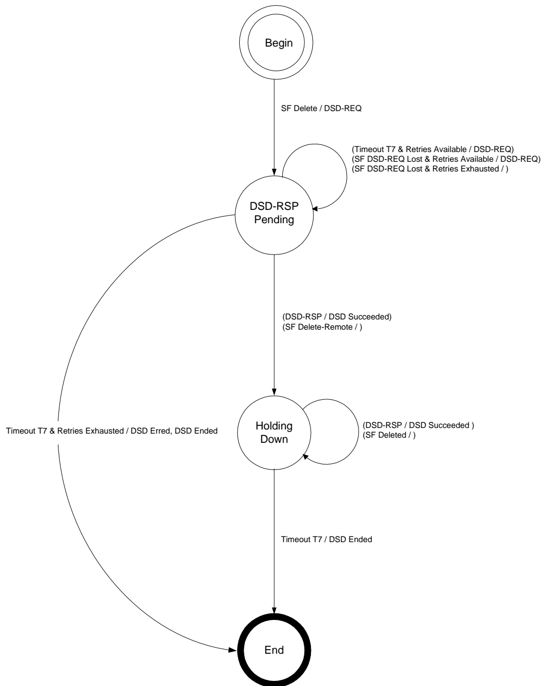
Figure 182 - DSD-Locally Initiated Transaction State Transition Diagram
