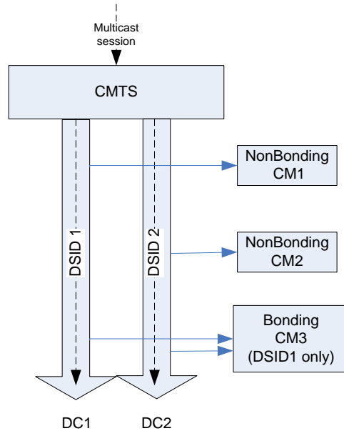
Figure 118 - DSIDs prevent duplication of non-bonded replications
