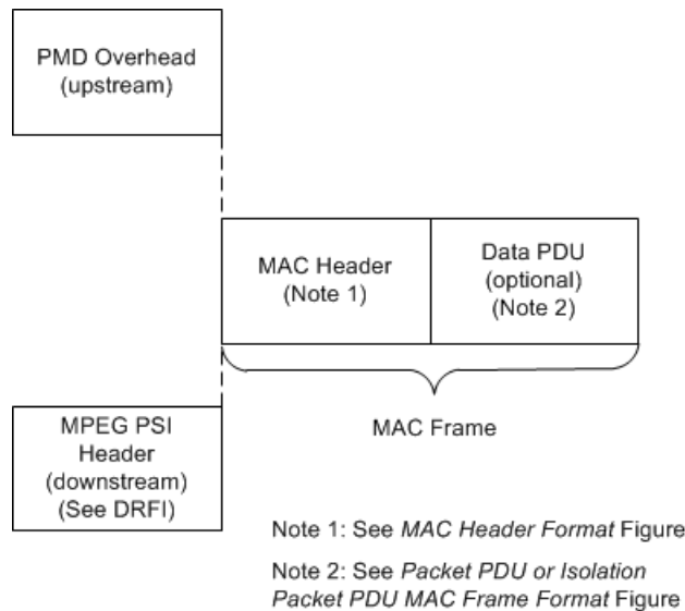
Figure 18 - Generic MAC Frame Format
