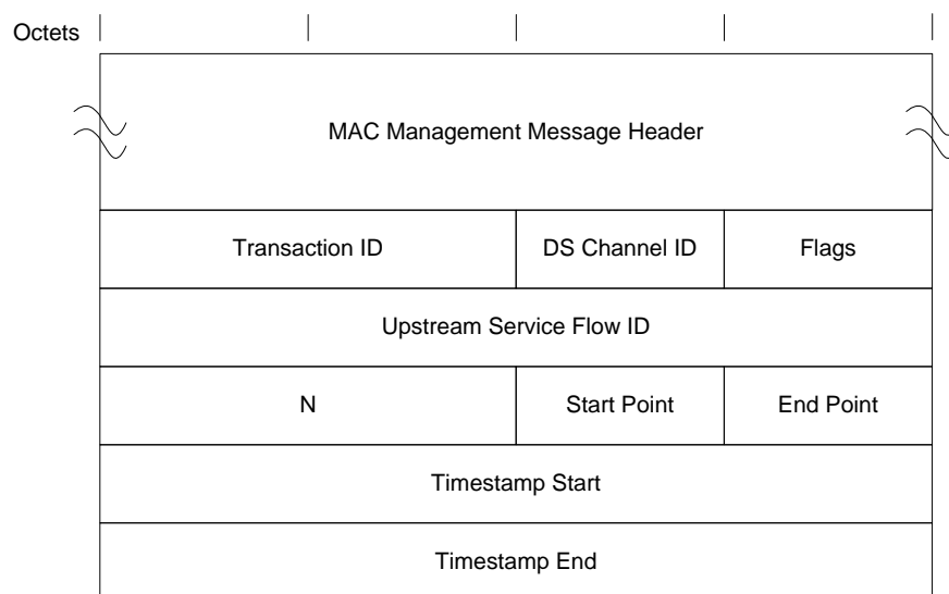
Figure 70 - DPV-REQ MAC Message
