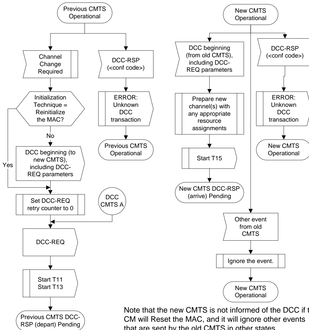
Figure 214 - Dynamically Changing Channels: CMTS View Part 1
