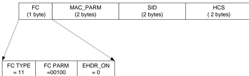
Figure 25 - Queue-depth Based Request Frame Format
