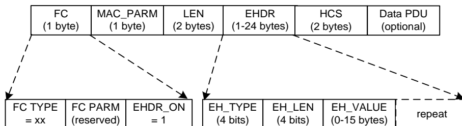
Figure 27 - Extended MAC Format
