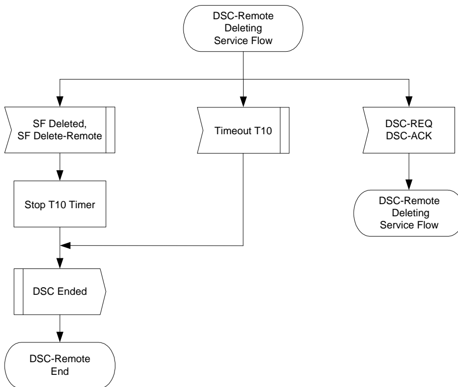
Figure 206 - DSC-Remotely Initiated Transaction Deleting Service Flow State Flow Diagram
