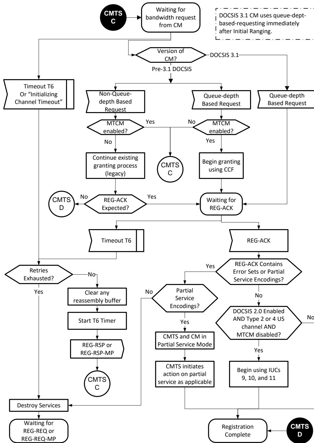
Figure 155 - CMTS Registration - End
