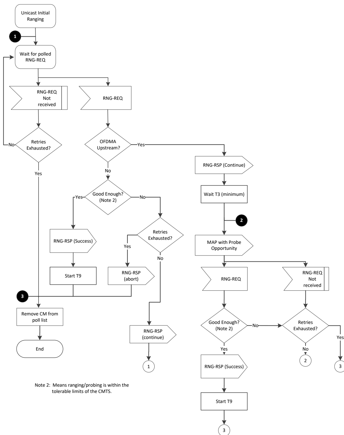
Figure 136 - Unicast Initial Ranging - CMTS
