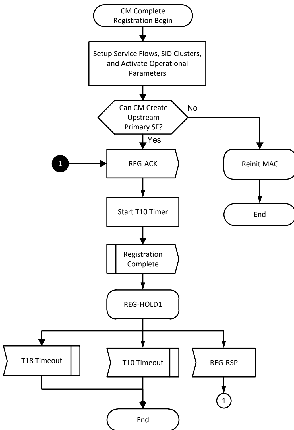
Figure 152 - CM Completes Registration
