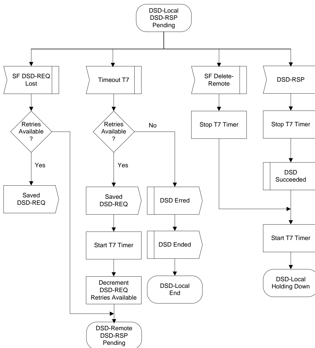
Figure 210 - DSD-Locally Initiated Transaction DSD-RSP Pending State Flow Diagram
