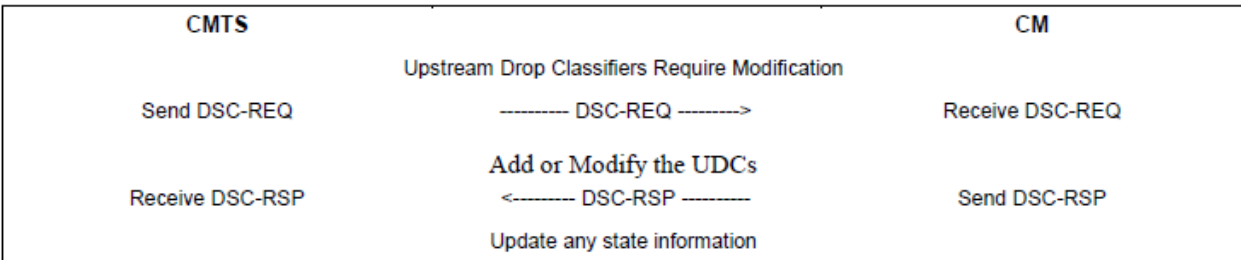
Figure 197 - CMTS-Initiated DSC Modifying an Upstream Drop Classifier
