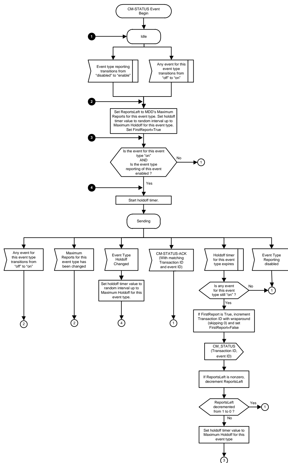
Figure 166 - CM-STATUS Event Type State Machine
