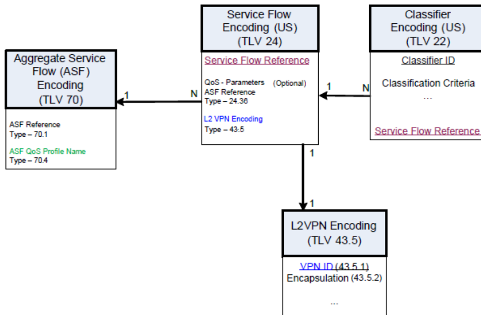
Figure 111 - Relationship of Upstream Classifiers, Service Flows, ASFs and L2VPN
