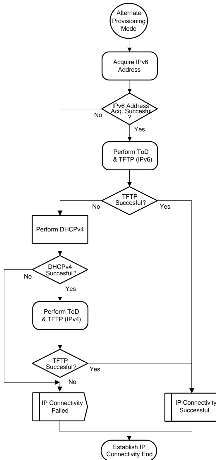
Figure 140 - Alternate Provisioning Mode
