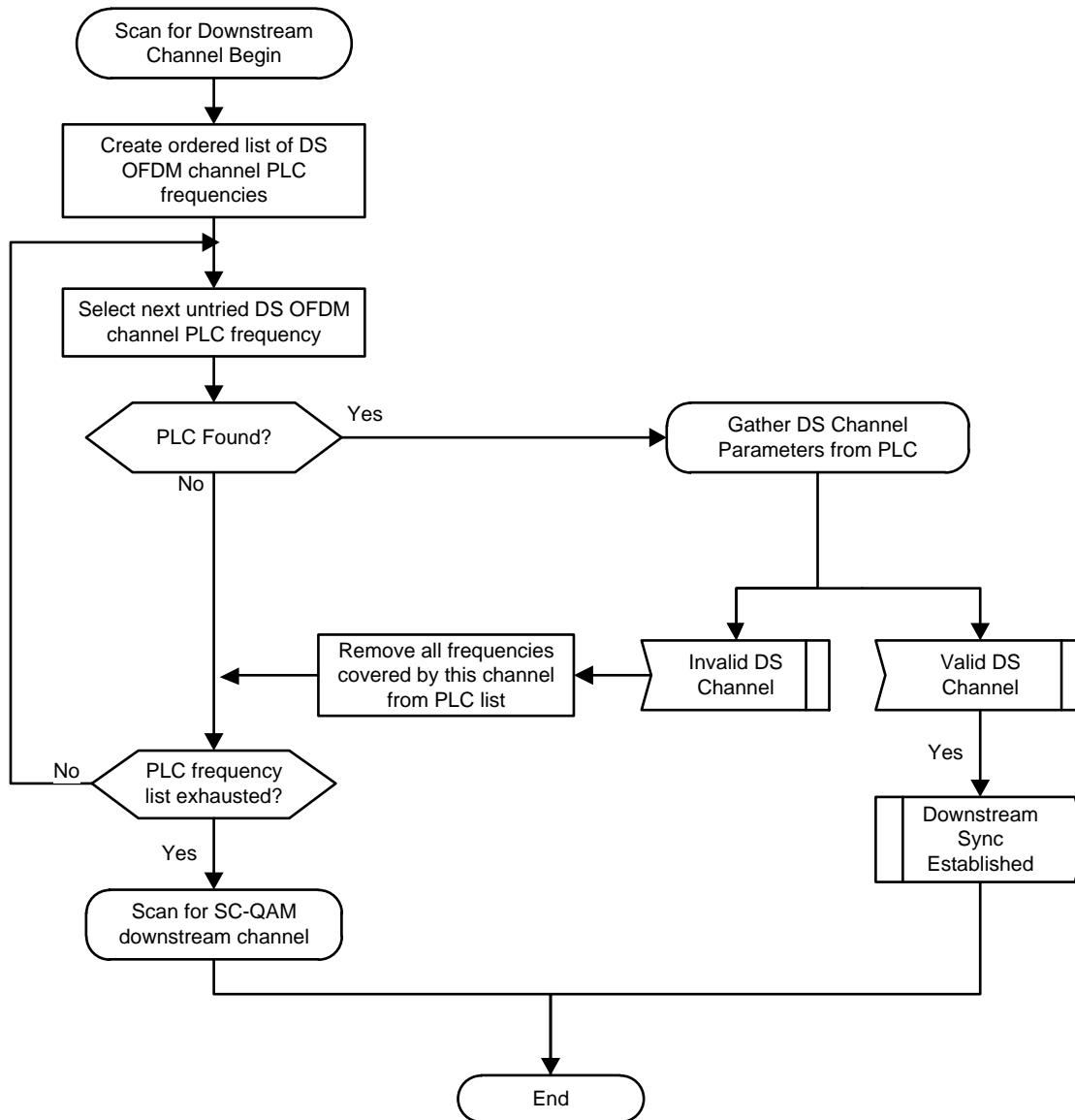
Figure 122 - Scan for Downstream Channel
