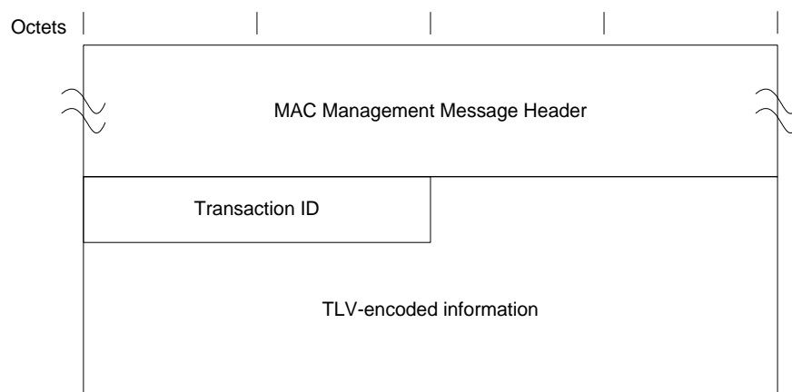
Figure 86 - DTP-INFO Message
