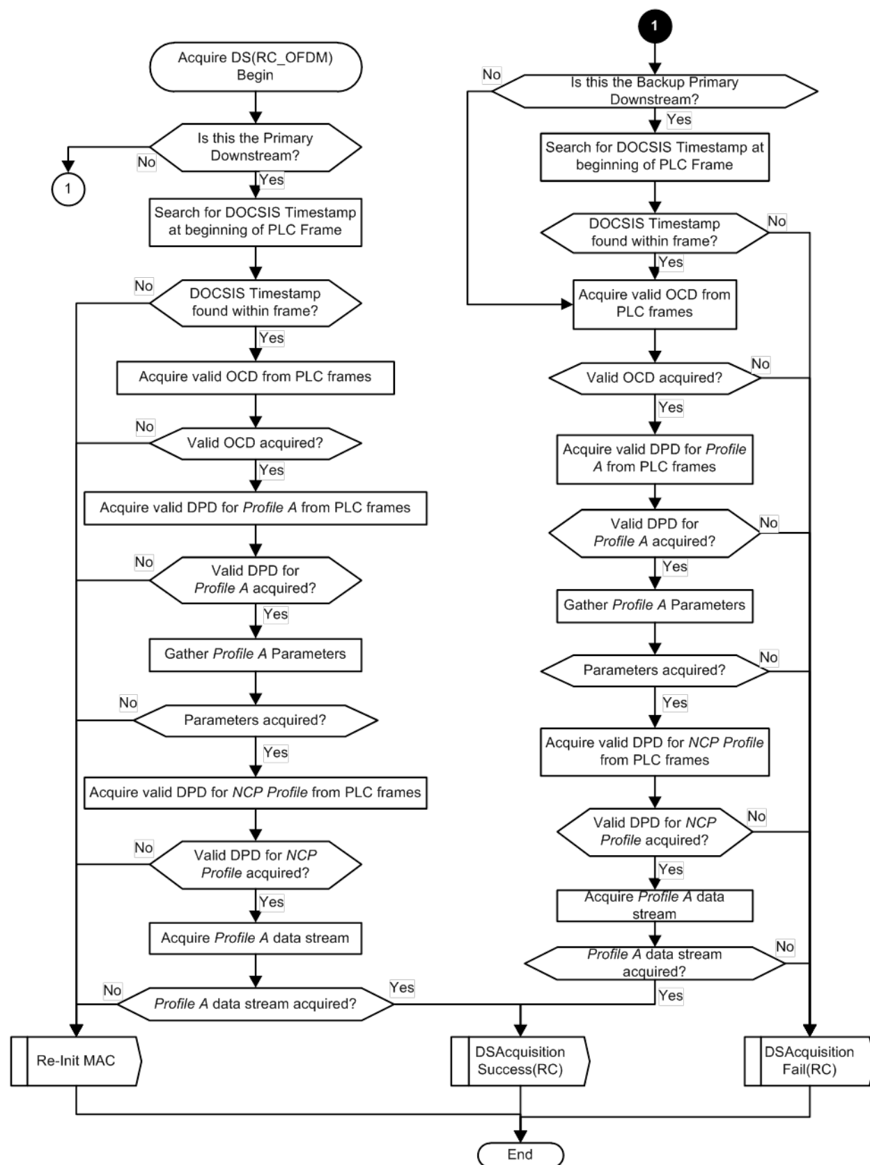
Figure 227 - CM AcquireDS Procedure for OFDM
