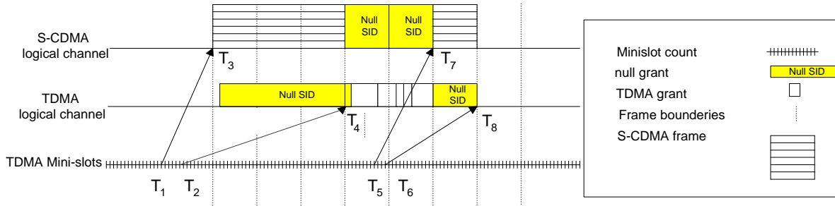
Figure 98 - Logical S-CDMA and TDMA channels
