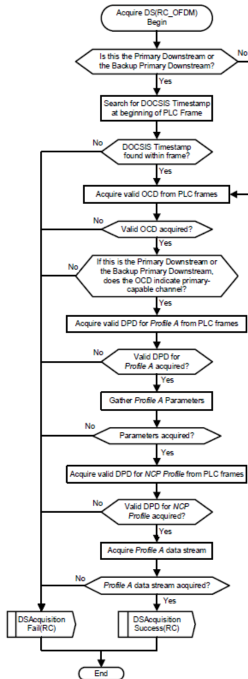
Figure 149 - CM Acquires OFDM Downstream Channel
