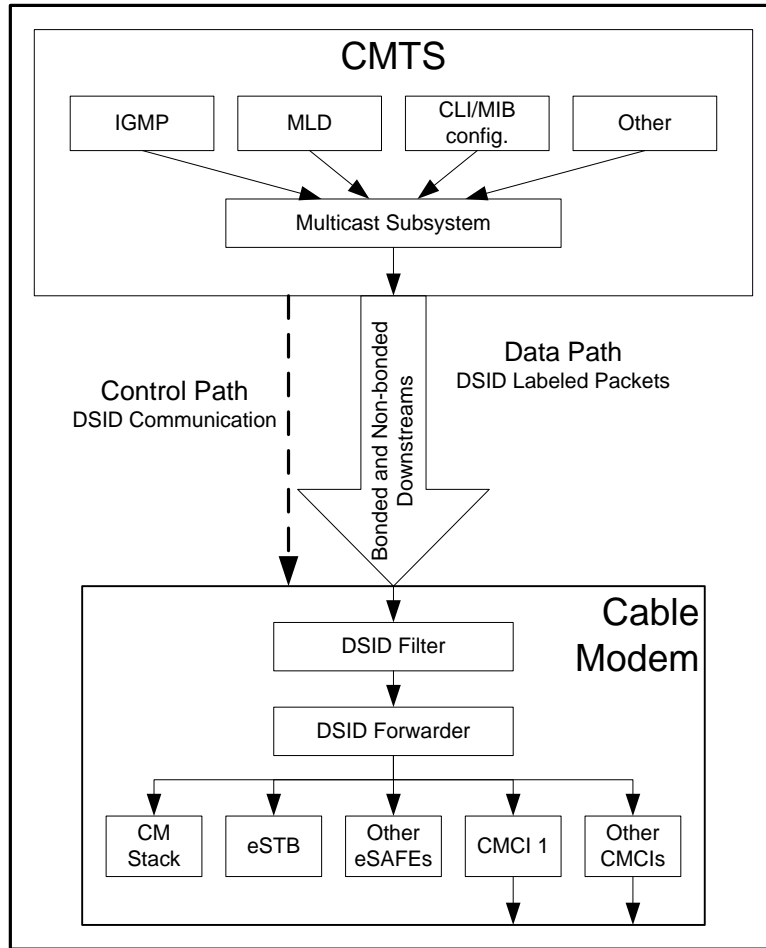
Figure 117 - Multicast Model
