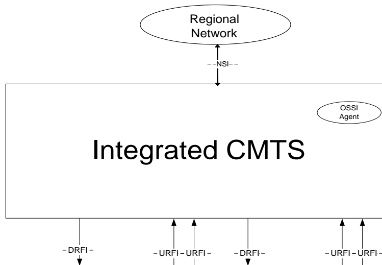
Figure 5 - Integrated CMTS Network Diagram
