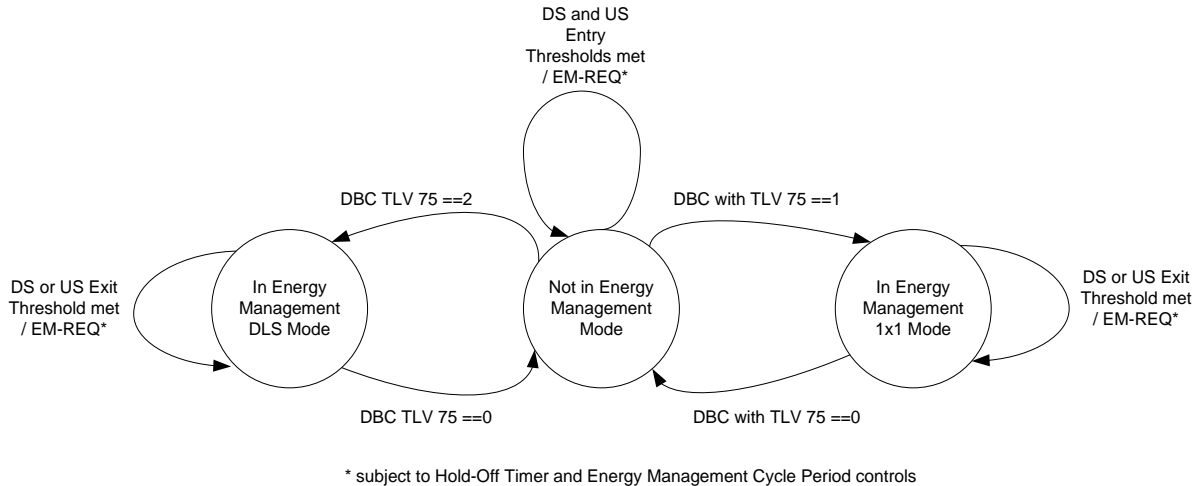
Figure 230 - Energy Management Modes State Diagram
