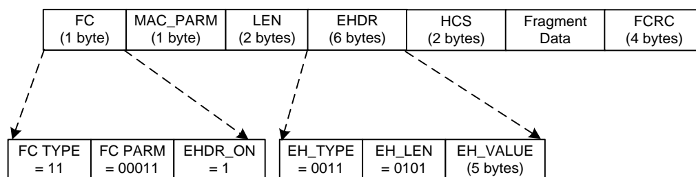
Figure 24 - Fragmentation MAC Header Format
