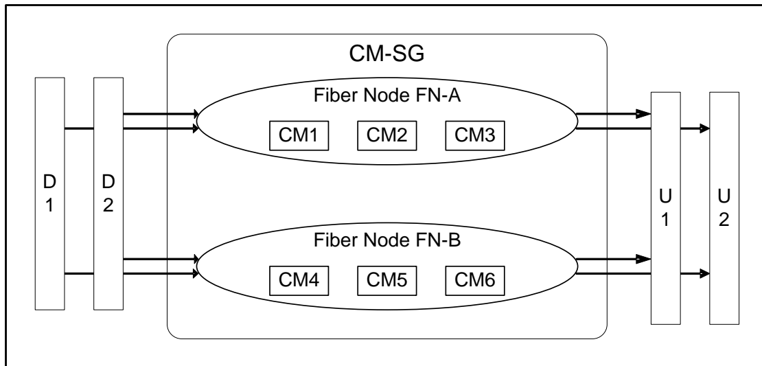
Figure 13 - Multiple Fiber Nodes per CM-SG
