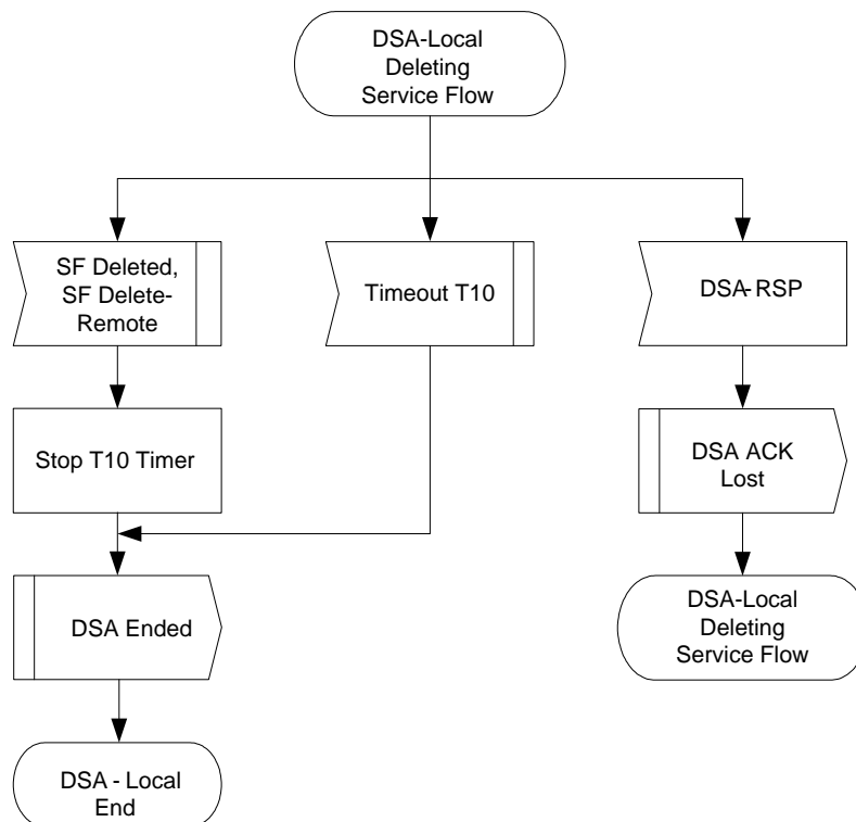
Figure 190 - DSA-Locally Initiated Transaction Deleting Service Flow State Flow Diagram
