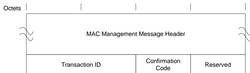
Figure 62 - Dynamic Service Deletion - Response
