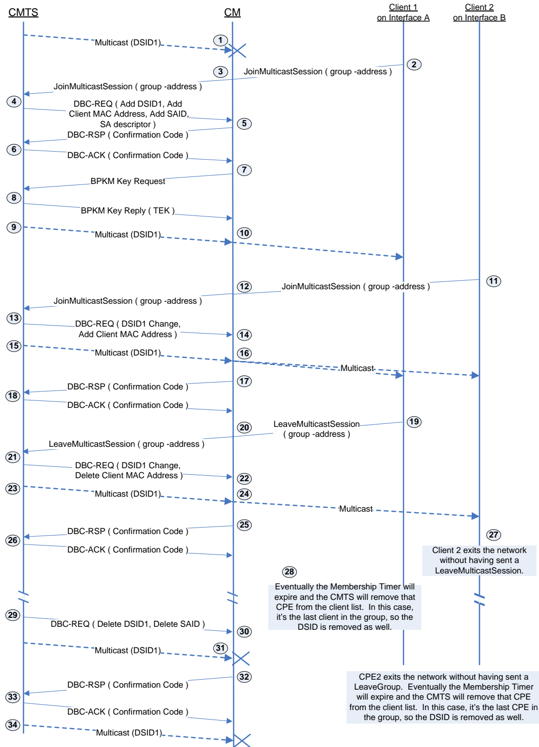
Figure 120 - Example - Encrypted Downstream Multicast Forwarding
