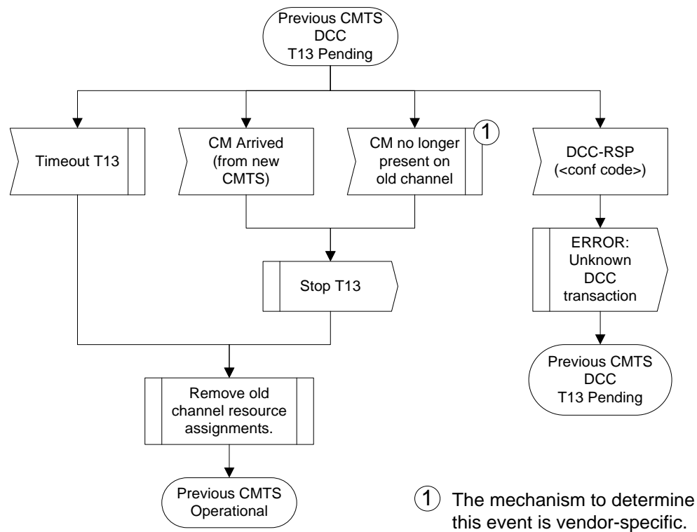
Figure 216 - Dynamically Changing Channels: CMTS View Part 3
