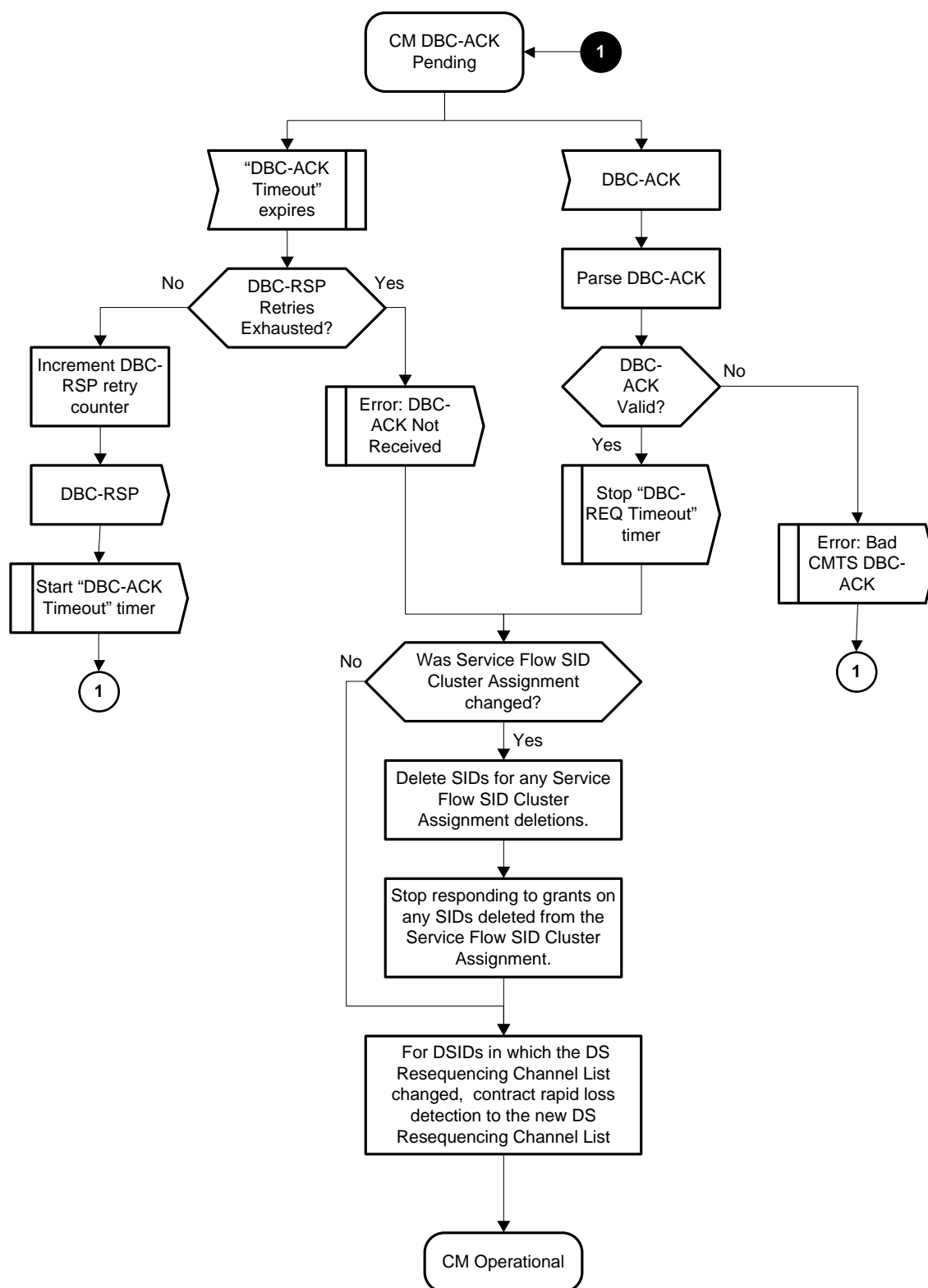
Figure 229 - CM DBC-ACK Pending
