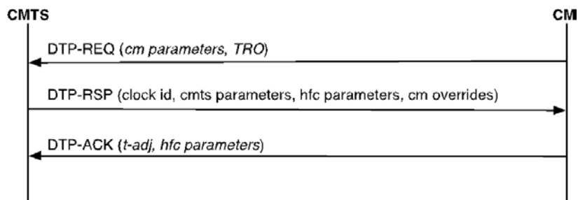
Figure 174 - CM is DTP Master
