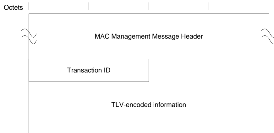
Figure 55 - Dynamic Service Addition - Request
