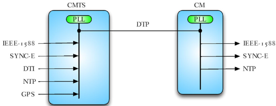
Figure 168 - DOCSIS Time Protocol System Overview
