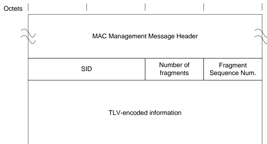
Figure 51 - Multipart Registration Request (REG-REQ-MP)
