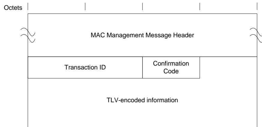
Figure 60 - Dynamic Service Change - Acknowledge
