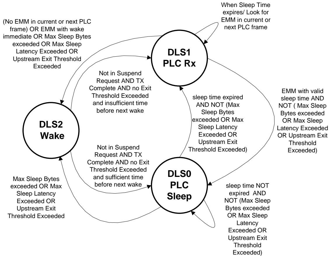
Figure 235 - PLC Rx and PLC Sleep Substate transitions for DLS Mode
