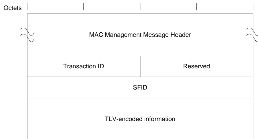
Figure 61 - Dynamic Service Deletion - Request
