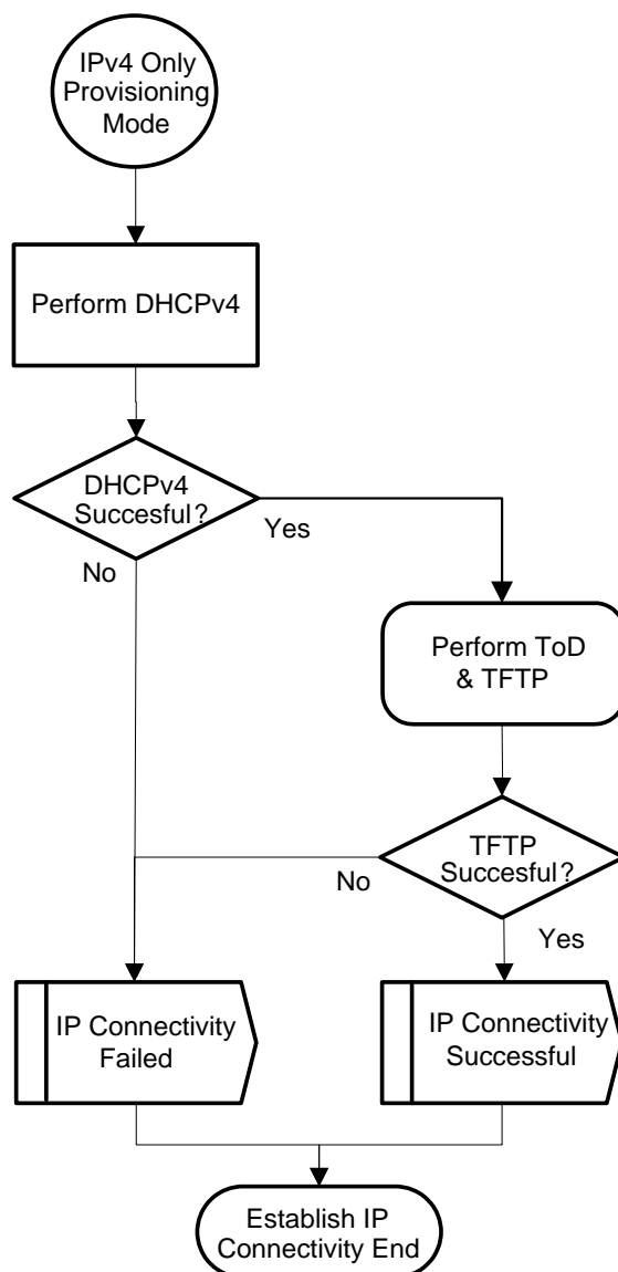
Figure 138 - IPv4 Only Provisioning Mode
