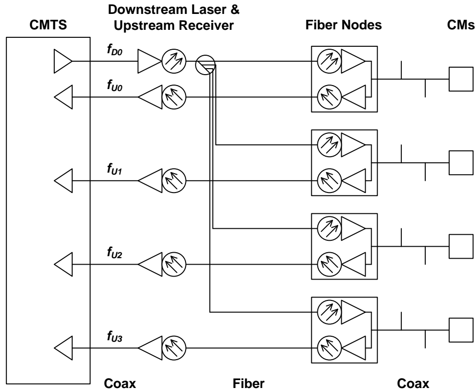
Figure 246 - Single Downstream and Single Upstream Channels per CM
