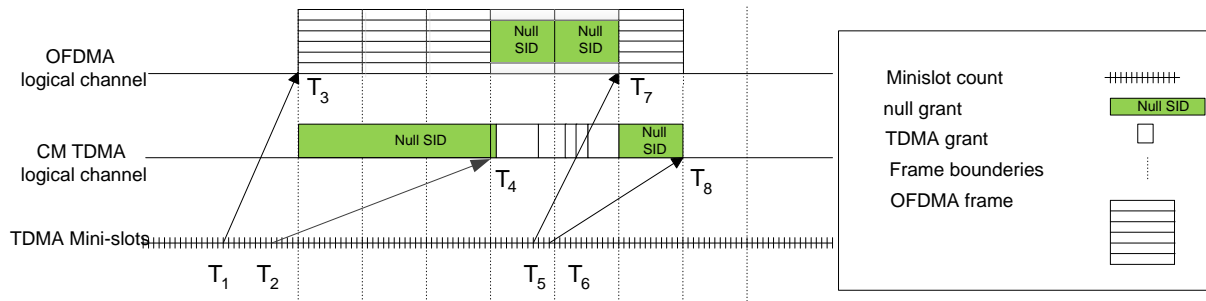
Figure 99 - Logical OFDMA and TDMA channels
