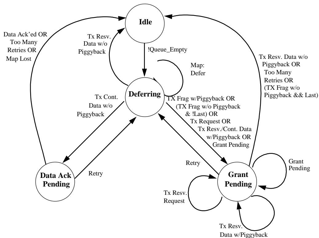
Figure 249 - Transmission and Deference State Transition Diagram
