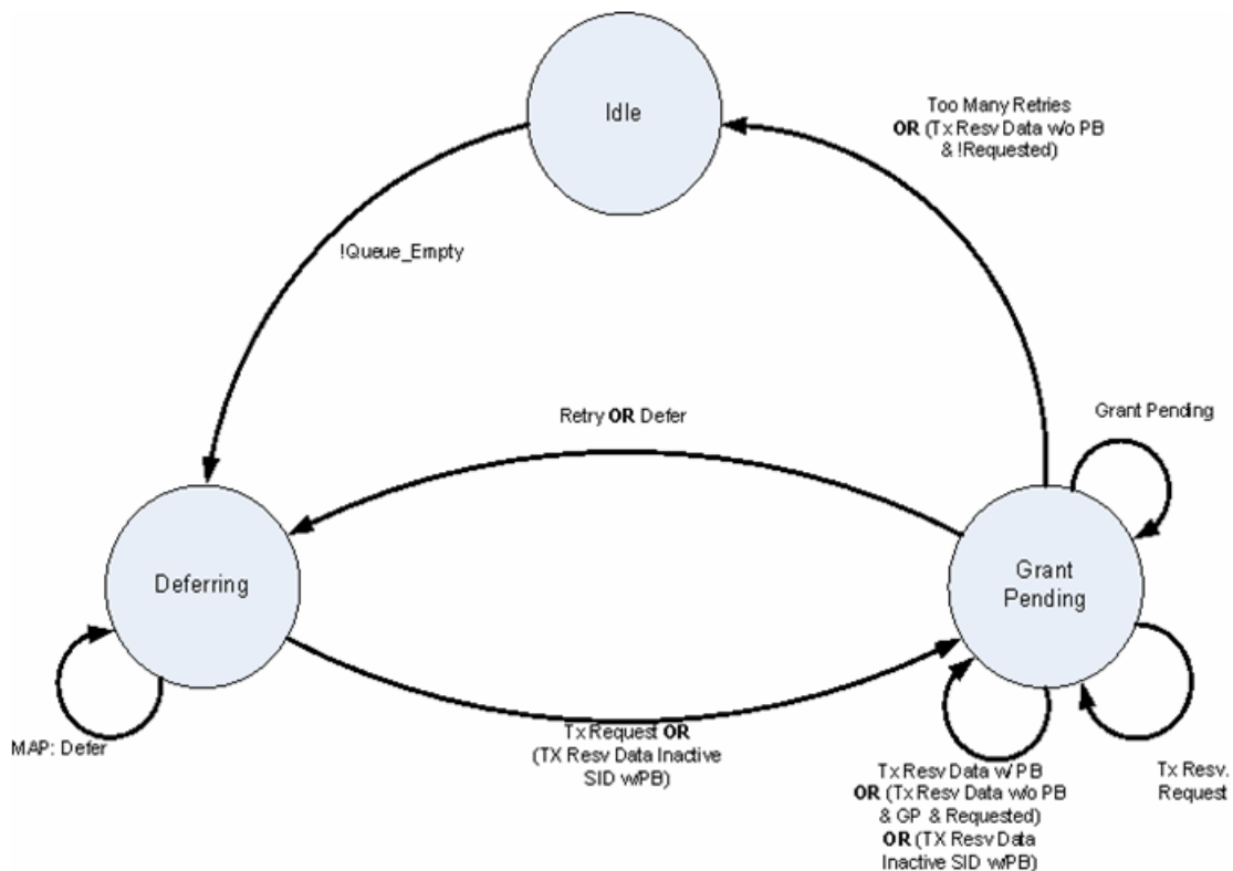
Figure 248 - Transmission and Deference State Transition Diagram (Multiple Transmit Channel Mode)
