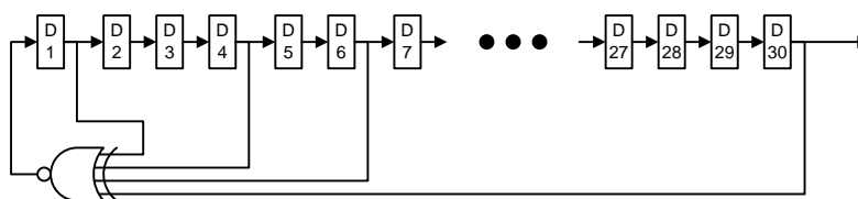
Figure 163 - Linear Feedback Shift Register for Synthetic Data Generation
