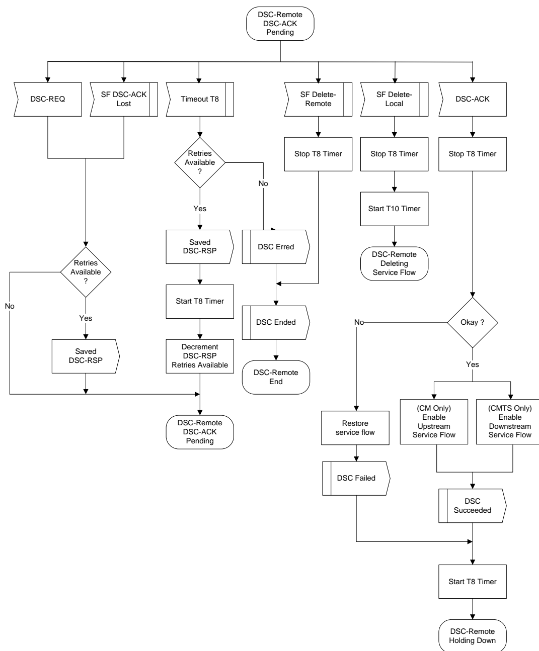
Figure 204 - DSC-Remotely Initiated Transaction DSC-ACK Pending State Flow Diagram
