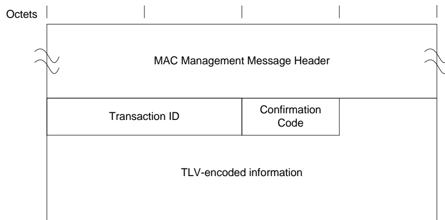
Figure 68 - Dynamic Bonding Change Response Message
