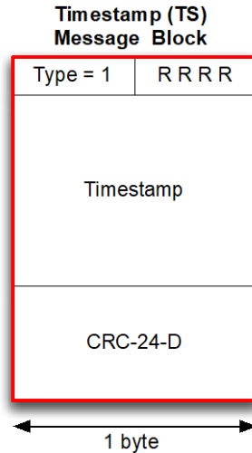
Figure 90 - Timestamp Message Block
