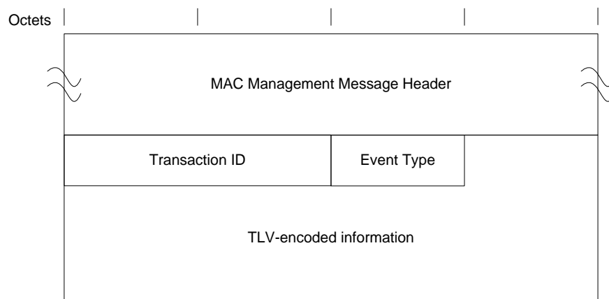
Figure 72 - CM-STATUS Report
