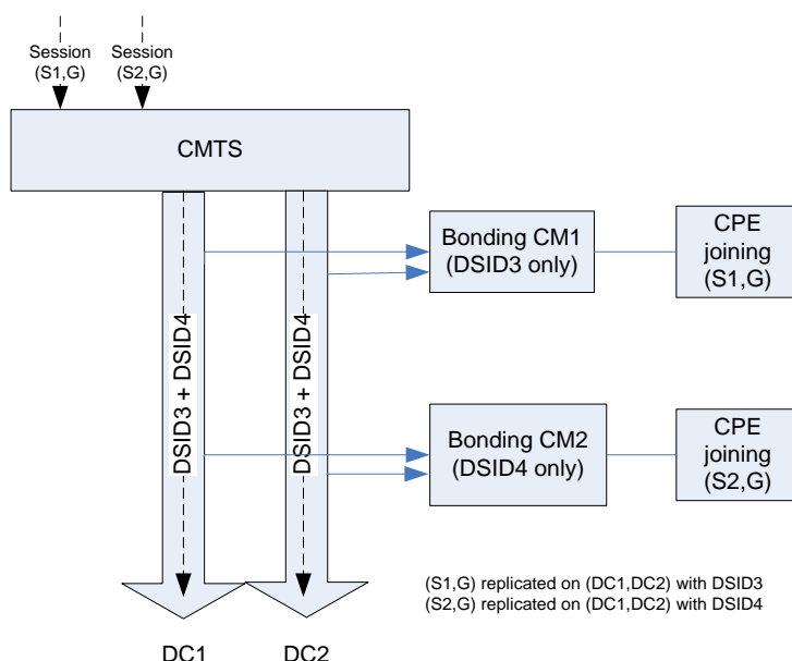
Figure 119 - DSIDs separate Source-Specific Multicast Sessions
