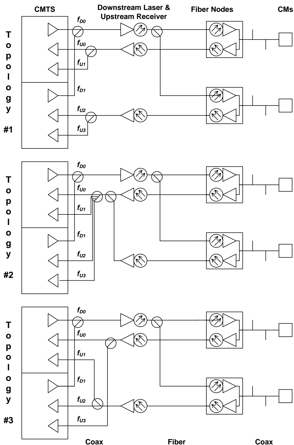
Figure 247 - Bonding Group Example
