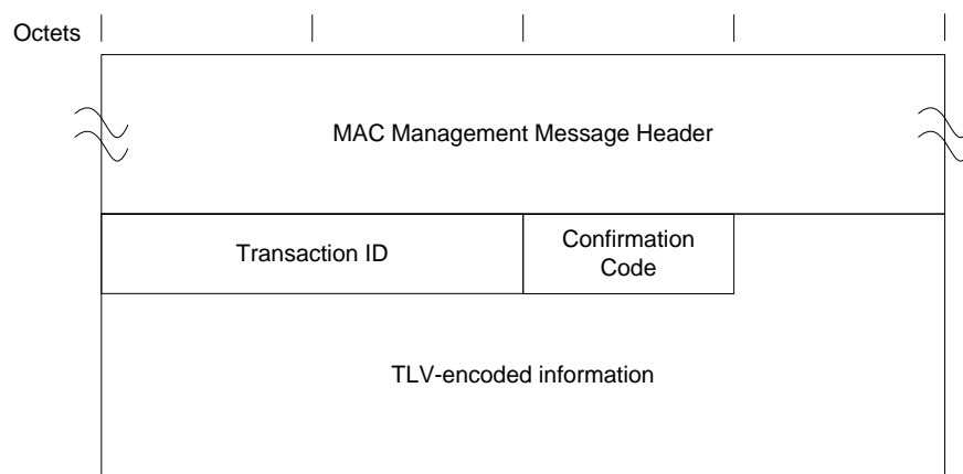
Figure 57 - Dynamic Service Addition - Acknowledge
