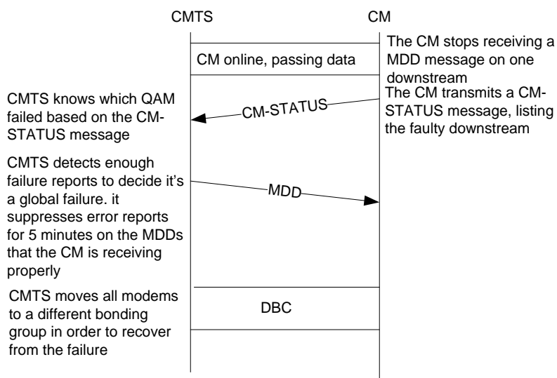
Figure 253 - Example 2 - Option 4
