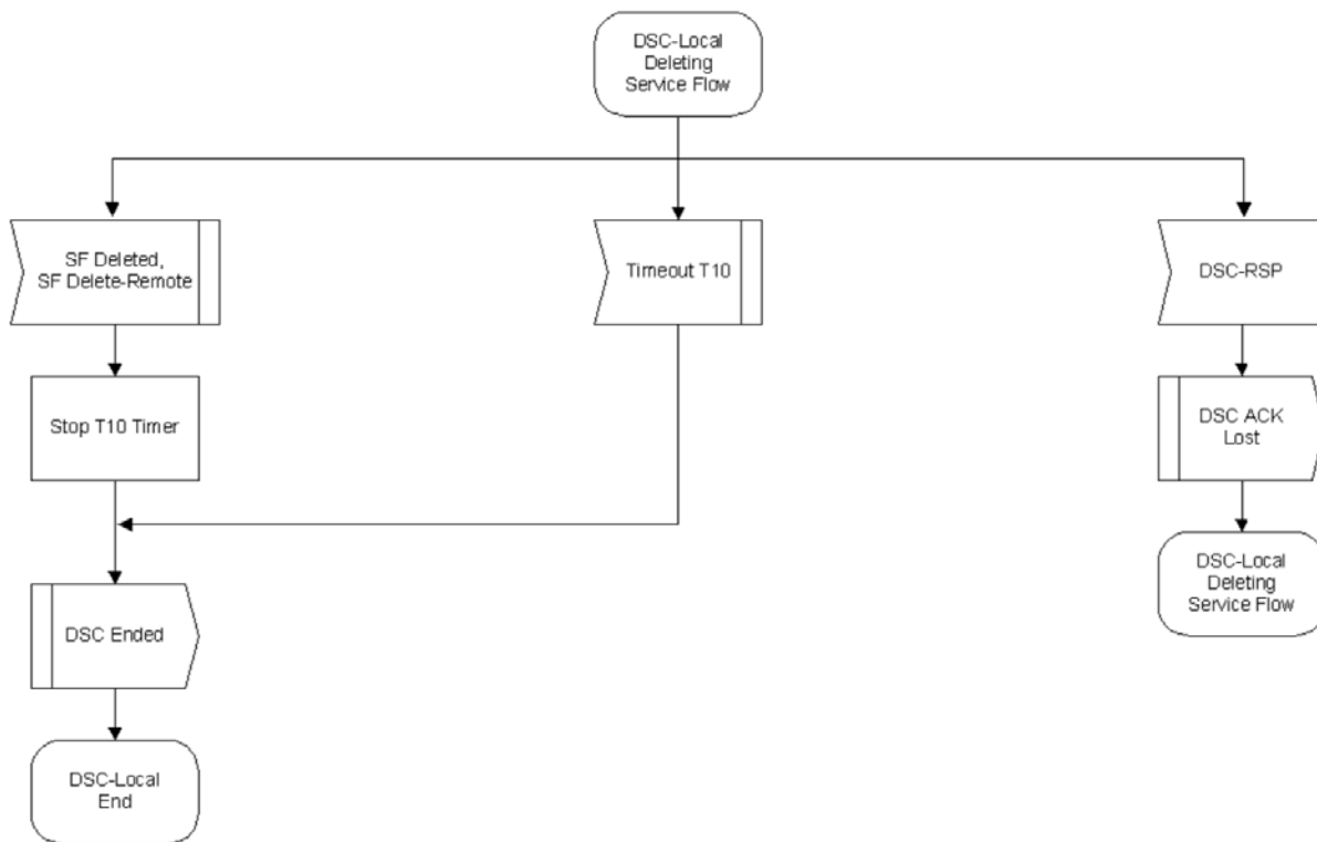
Figure 202 - DSC-Locally Initiated Transaction Deleting Service Flow State Flow Diagram
