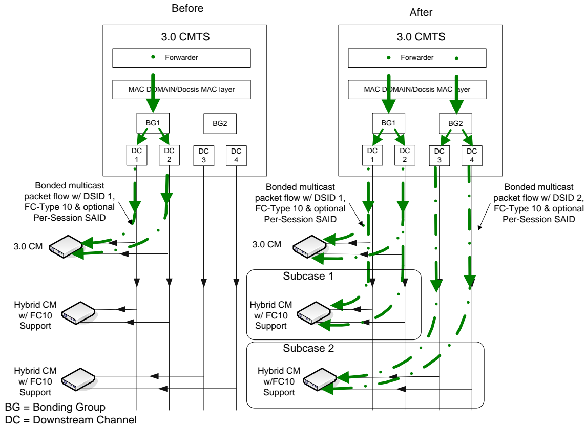
Figure 261 - Multicast Session Replication to Clients Behind Both a 3.0 CM and a Hybrid CM w/ FC-Type 10 Support
