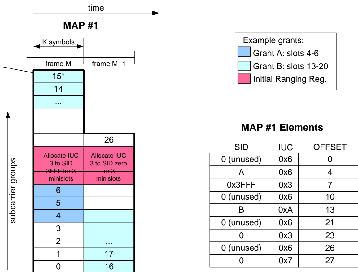
Figure 101 - Example MAP for Initial Ranging Region on an OFDMA Channel
