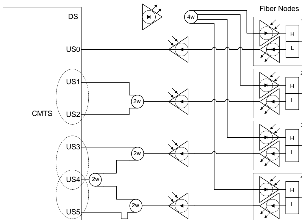
Figure 267 - Example Combining Network 1
