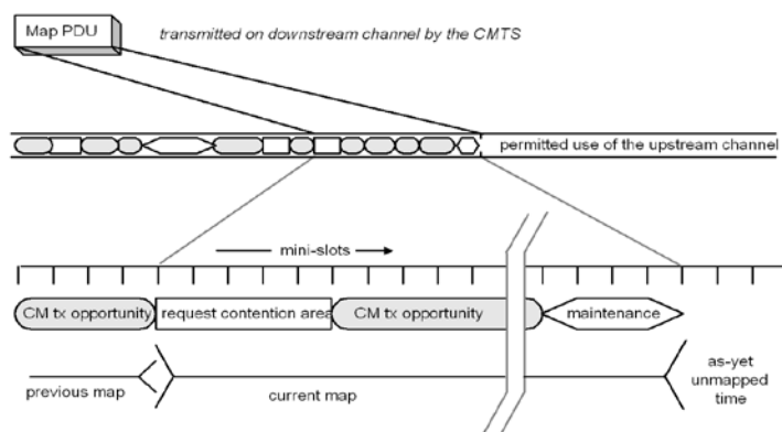
Figure 96 - Allocation Map
