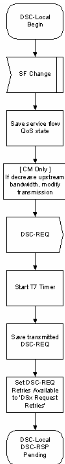
Figure 198 - DSC-Locally Initiated Transaction Begin State Flow Diagram
