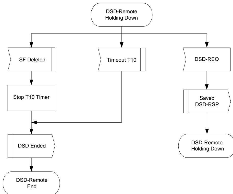
Figure 213 - DSD-Remotely Initiated Transaction Holding Down State Flow Diagram
