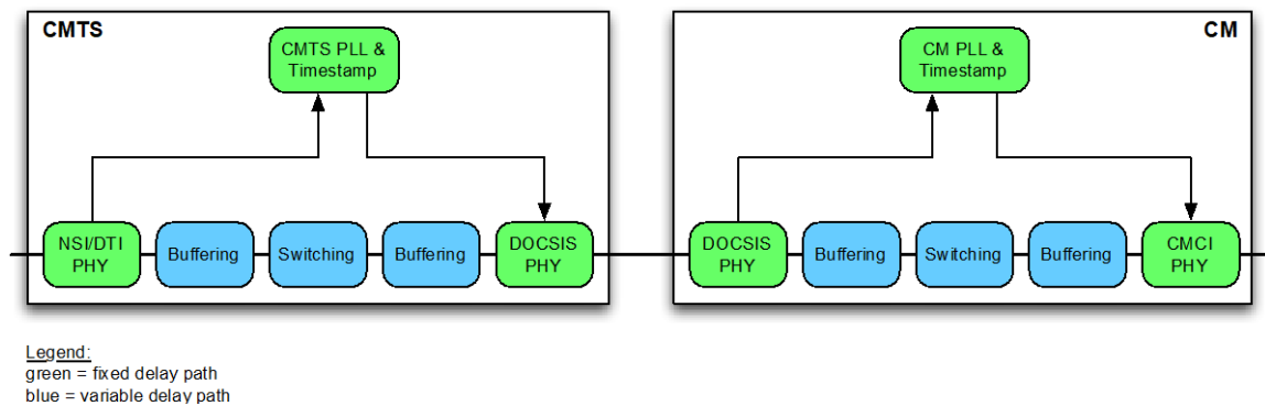
Figure 169 - DOCSIS Time Protocol Fixed Latency Path Example
