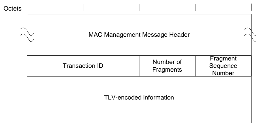
Figure 67 - Dynamic Bonding Change Request Message
