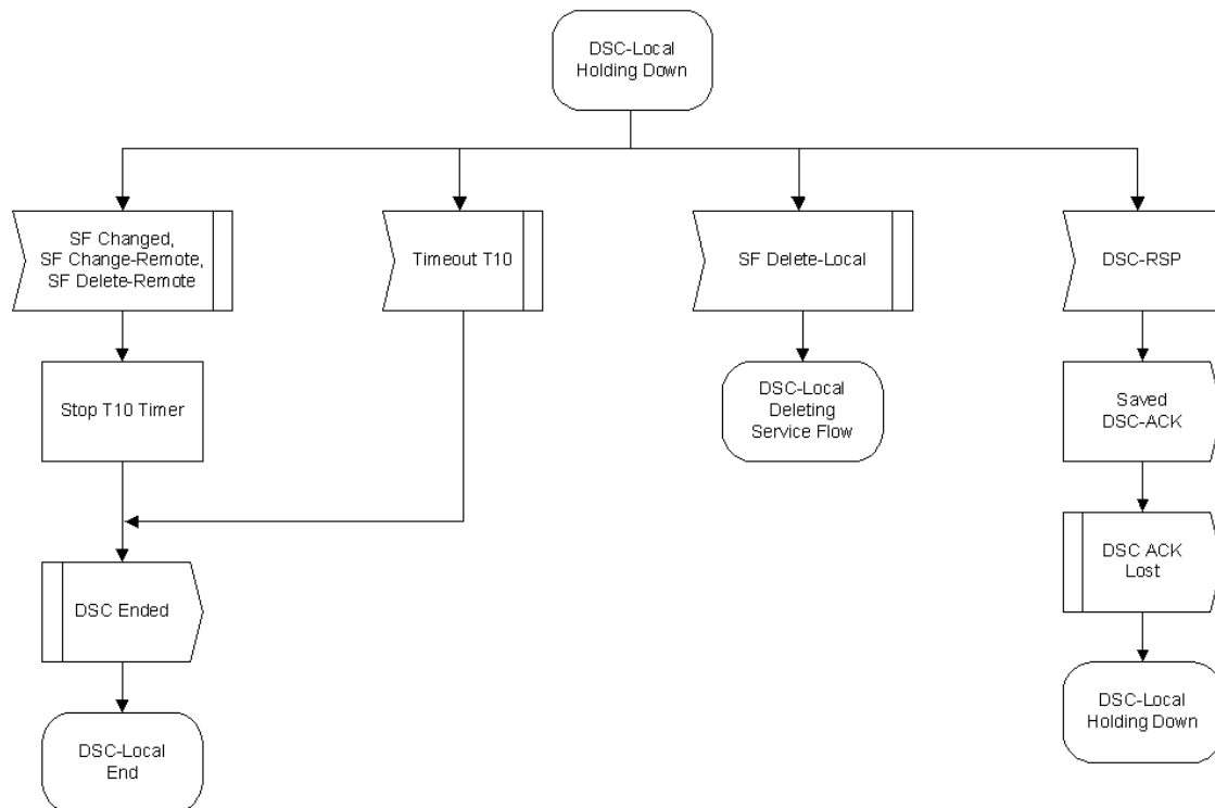
Figure 200 - DSC-Locally Initiated Transaction Holding Down State Flow Diagram
