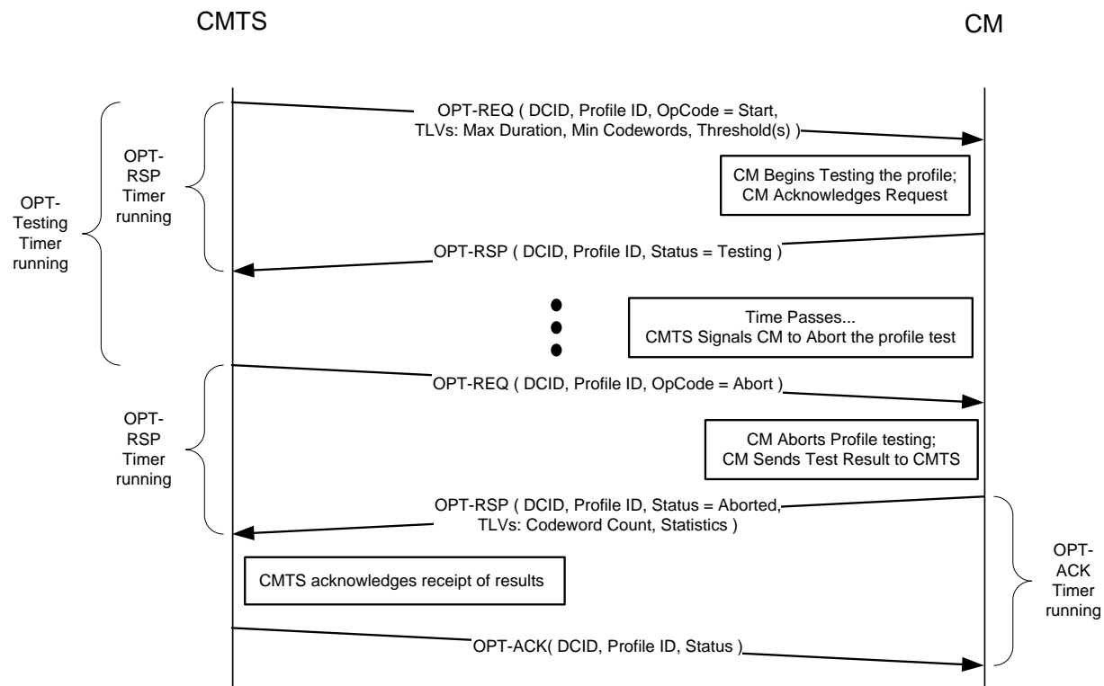
Figure 159 - Aborted OFDM Profile Test Transaction
