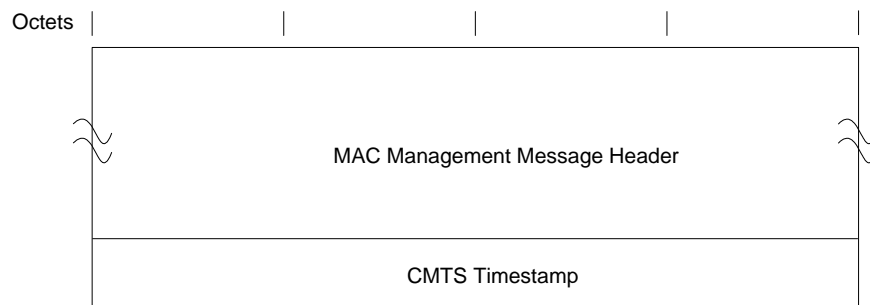
Figure 30 - Format of Packet PDU Following the Timing Header
