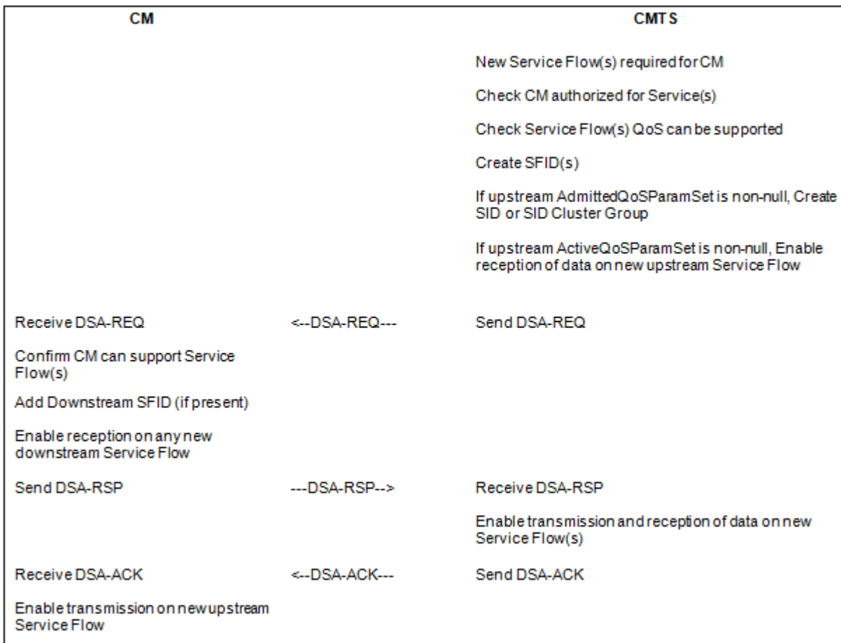
Figure 185 - Dynamic Service Addition Initiated from CMTS
