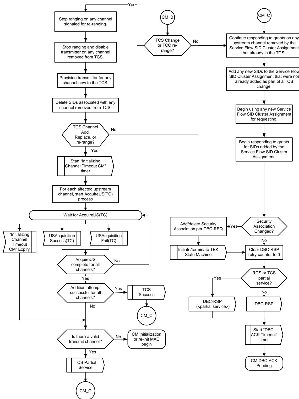
Figure 225 - CM DBC-RSP (part 3)
