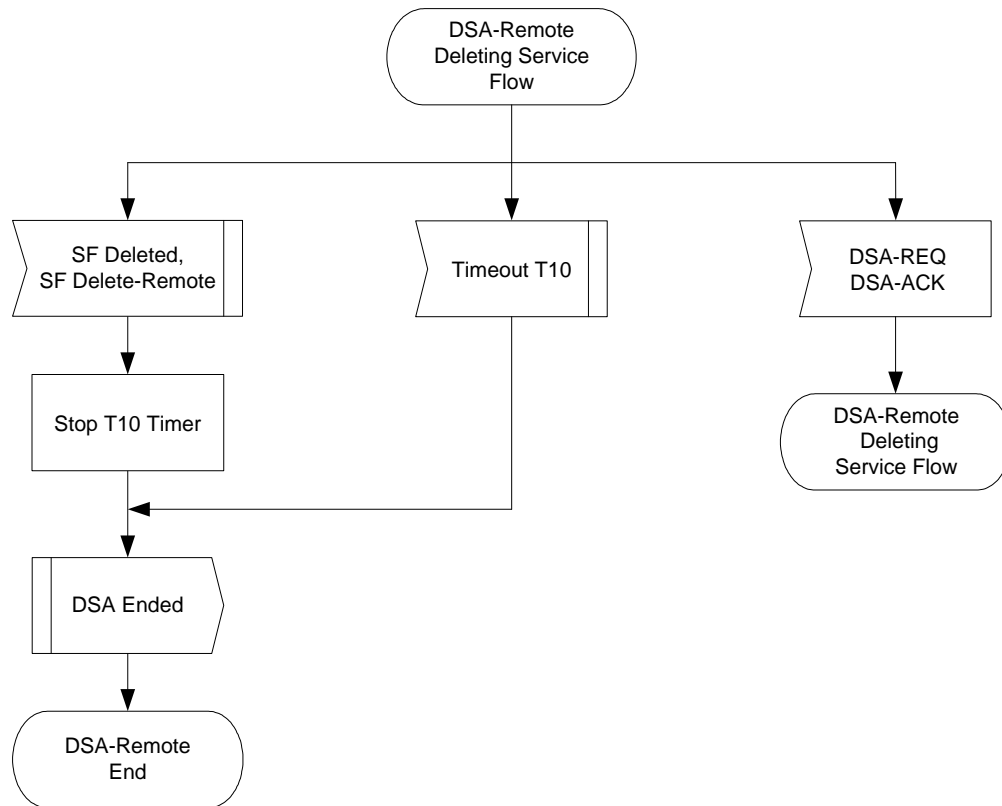
Figure 194 - DSA-Remotely Initiated Transaction Deleting Service State Flow Diagram
