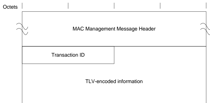
Figure 85 - DTP Response Message
