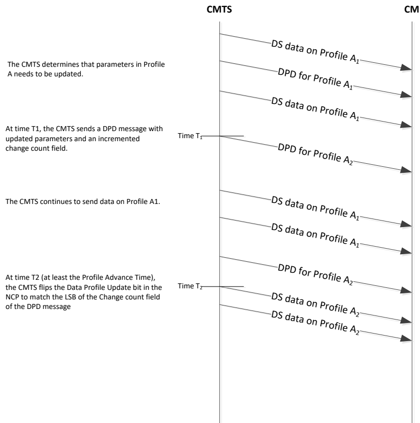
Figure 269 - DPD Change to Profile A
