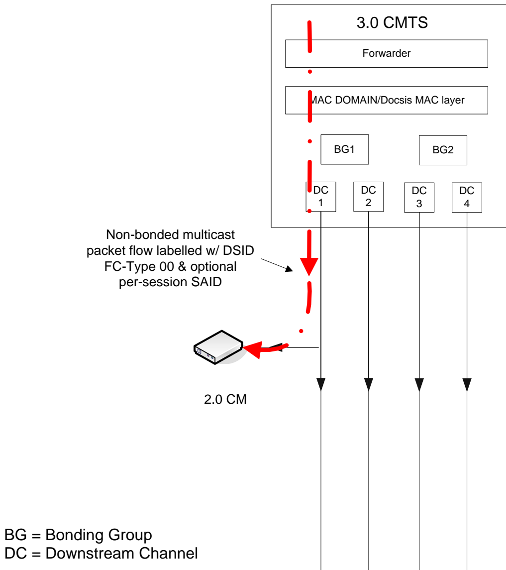
Figure 255 - Multicast Session Replication for a client behind a 2.0 CM
