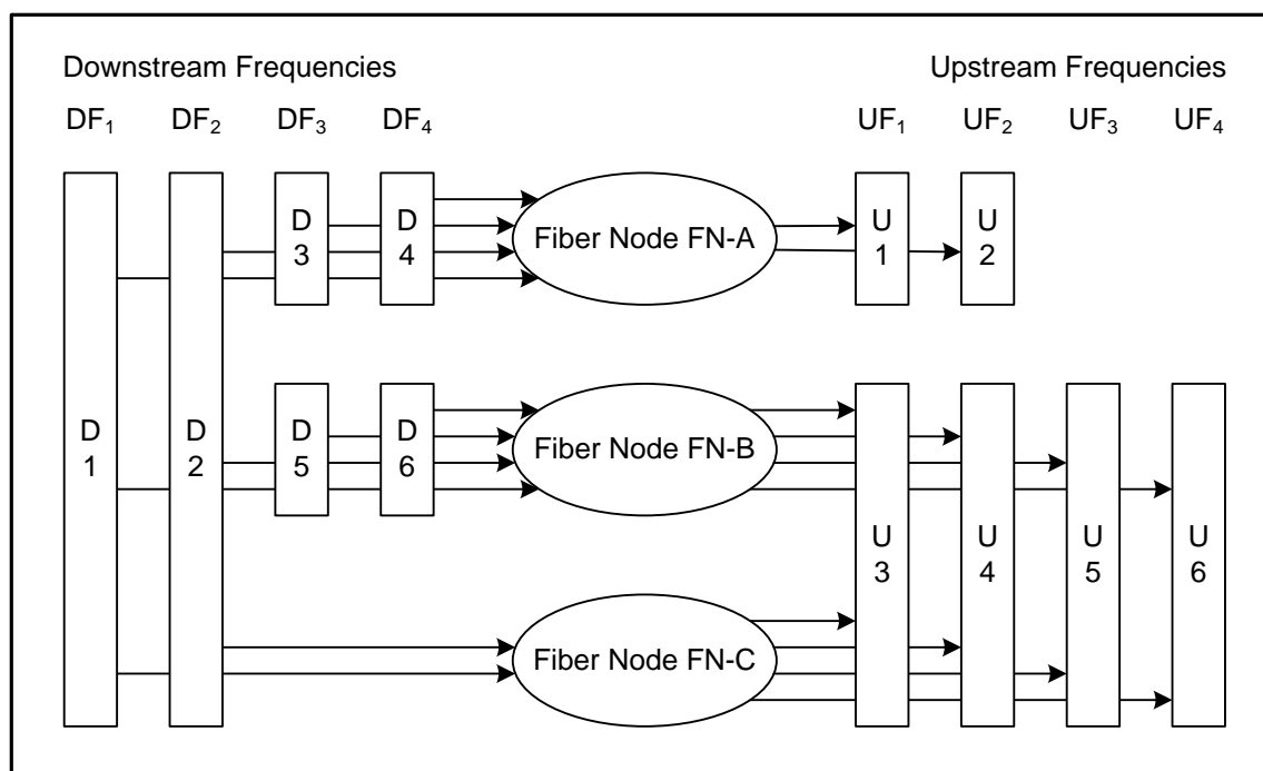
Figure 12 - Frequency Space Diagram
