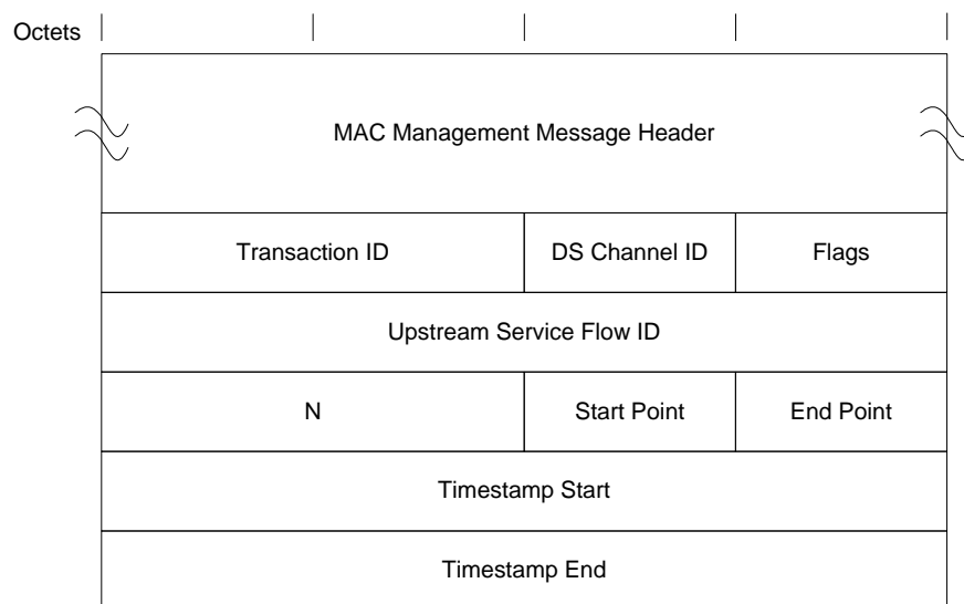
Figure 71 - DPV-RSP MAC Message
