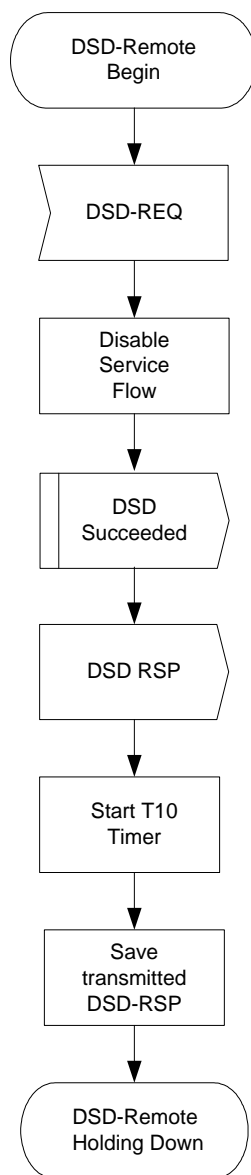
Figure 212 - - DSD-Remotely Initiated Transaction Begin State Flow Diagram
