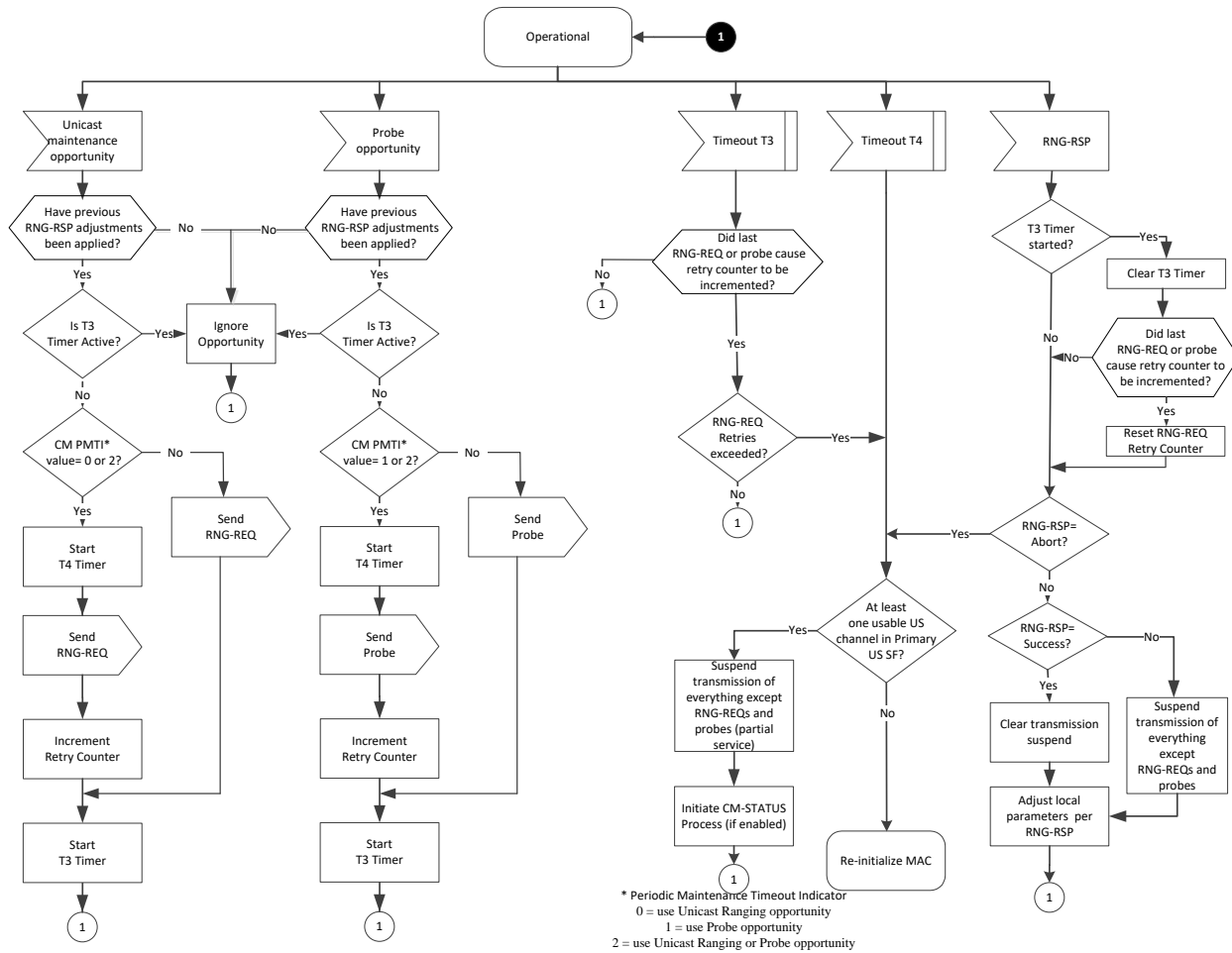
Figure 157 - Periodic Ranging - CM View
