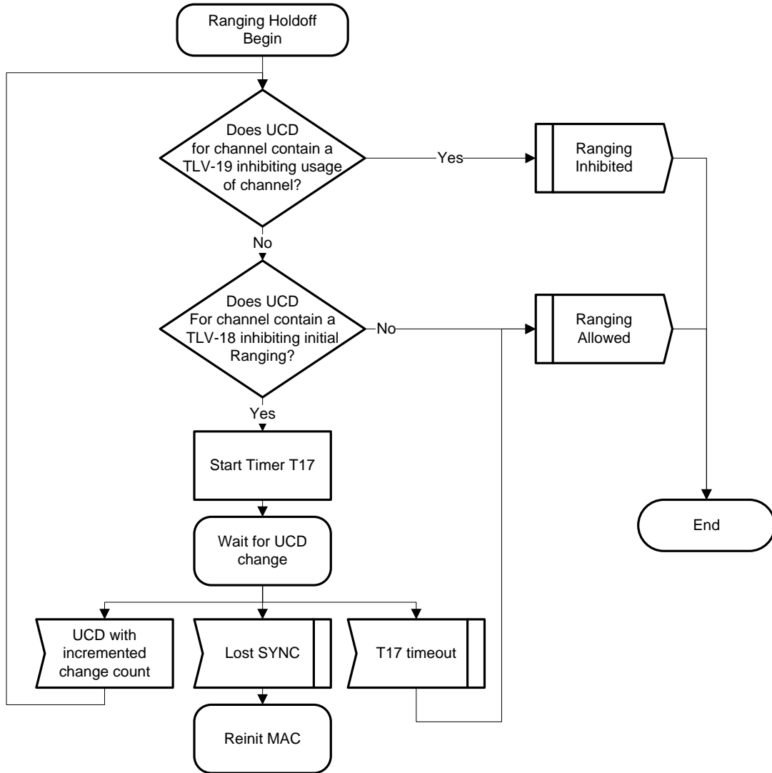
Figure 128 - Ranging Holdoff
