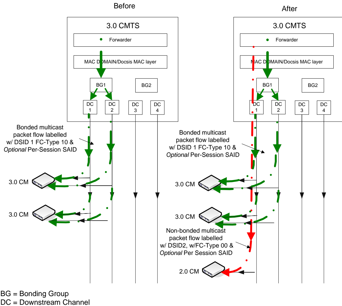
Figure 259 - Bonded and Non-bonded Replications of a Multicast Session on an Overlapping Downstream Channel Using FC 10 Isolation Technique (Subcase 2)
