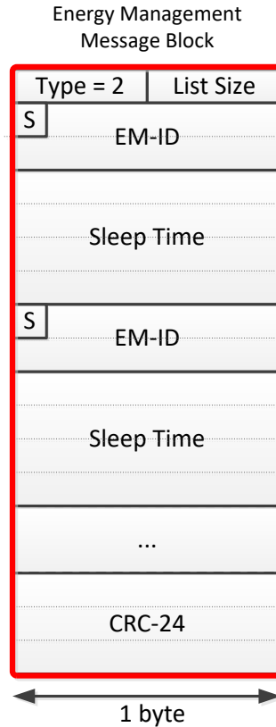
Figure 91 - Energy Management Message Block
