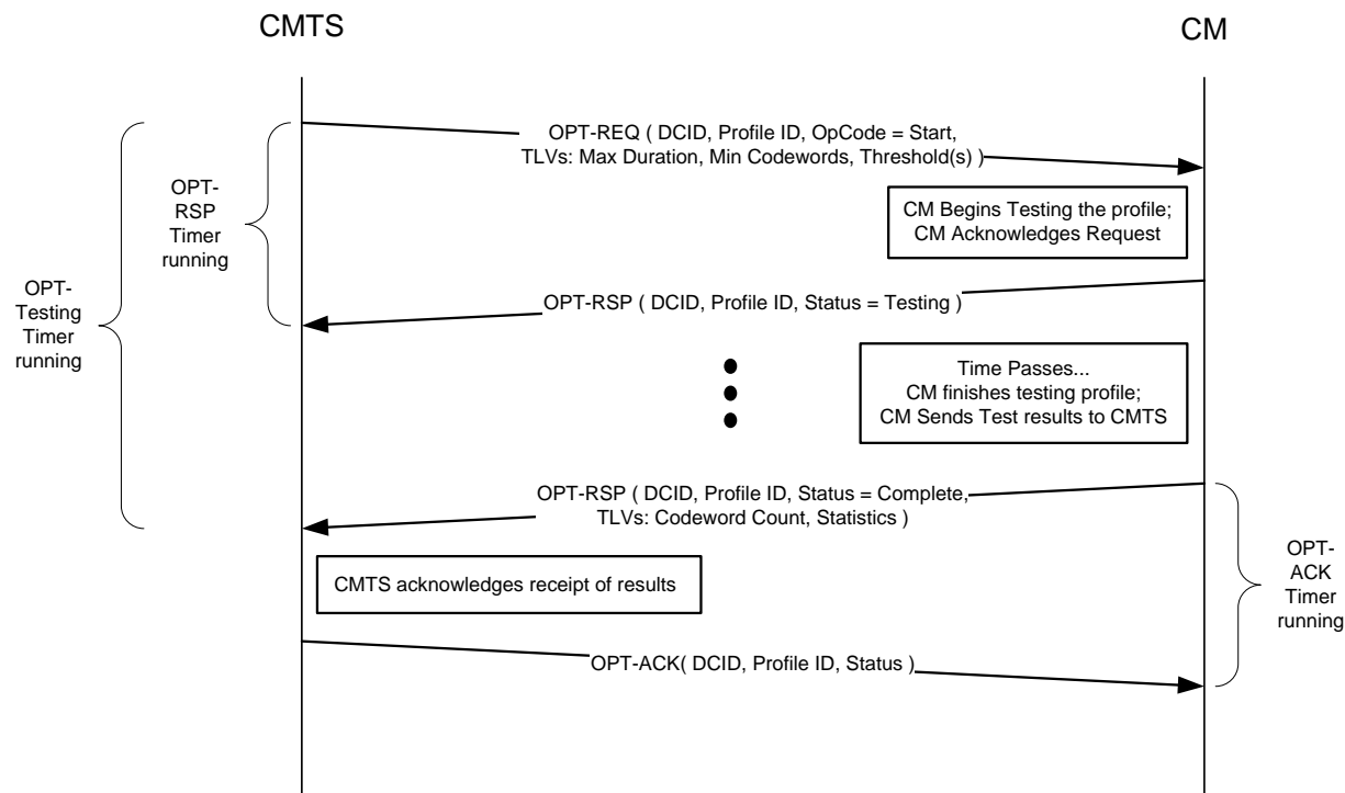
Figure 158 - Typical OFDM Profile Test Transaction
