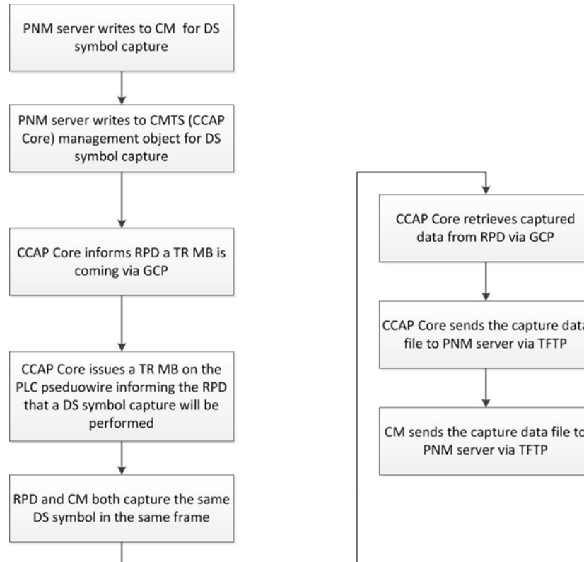
Figure 28 - DS Symbol Capture Flow in R-PHY Architecture
