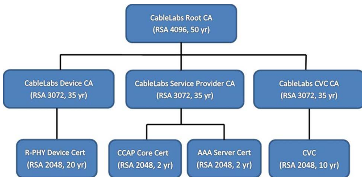
Figure 49 - Certificate Hierarchy
