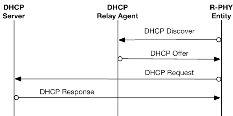
Figure 14 - DHCP Signaling
