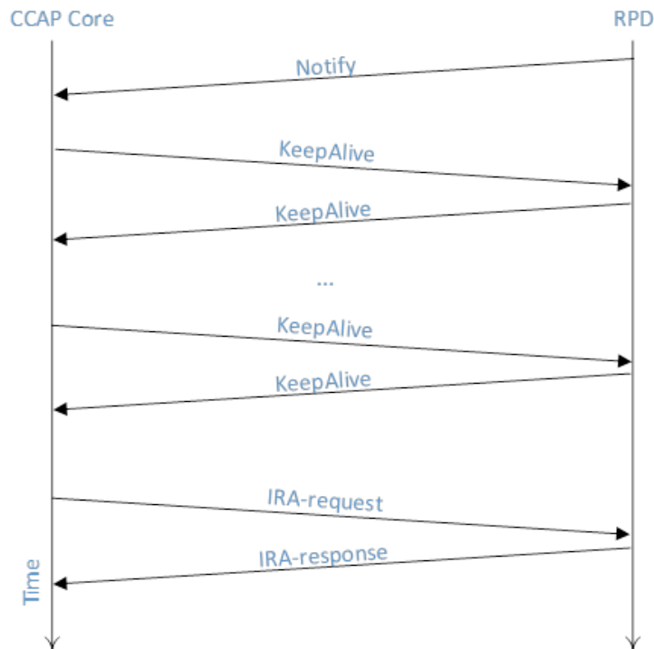
Figure 33 - RCP Initialization Sequence
