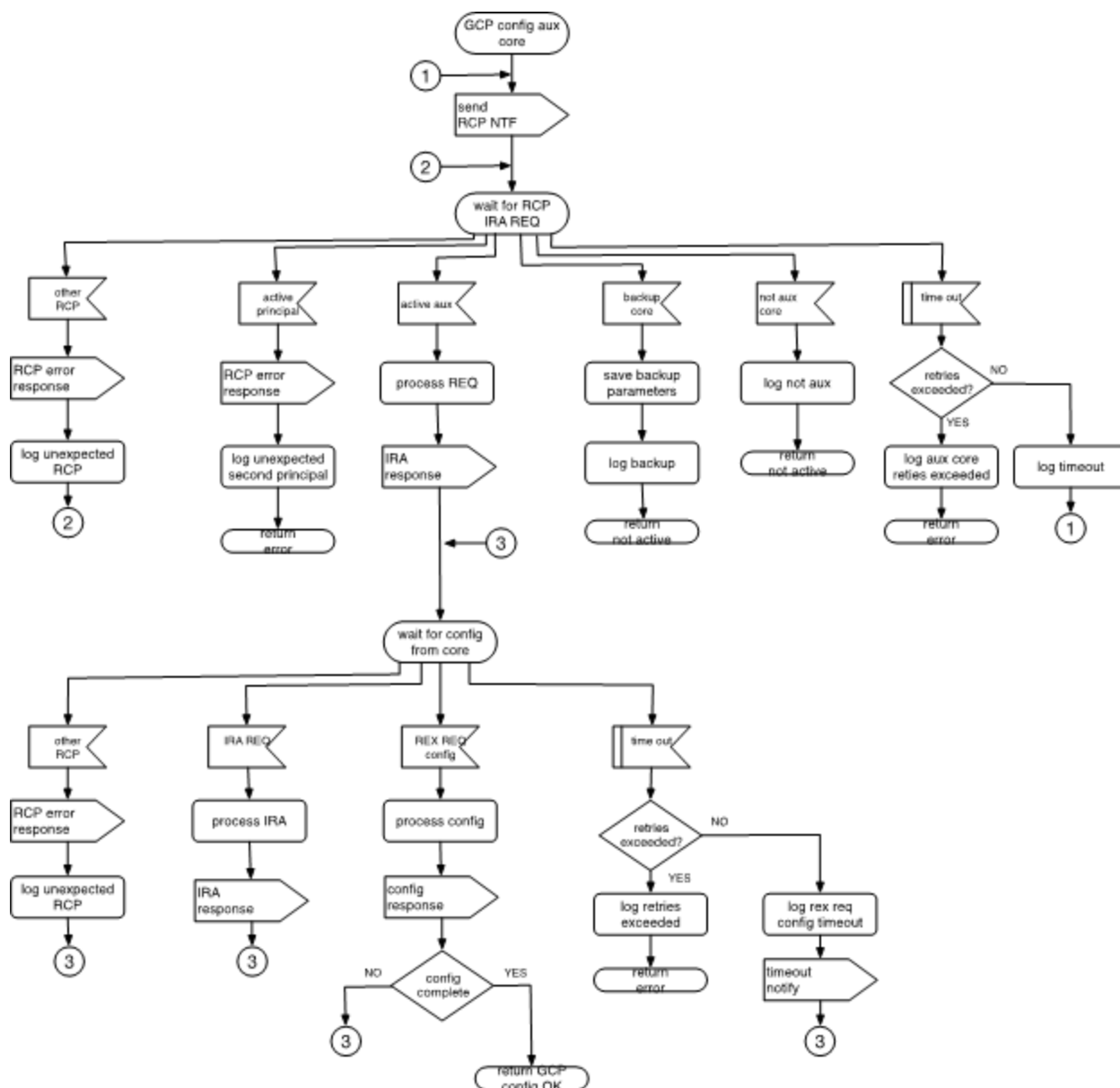
Figure 21 - Configuration by Auxiliary Core
