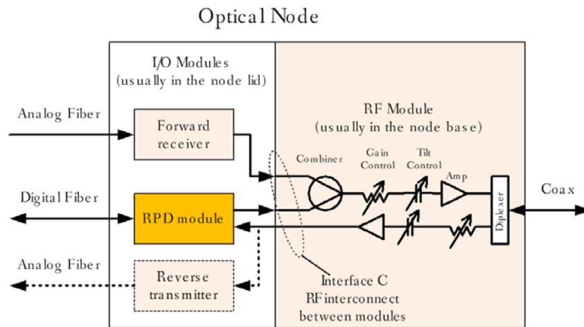
Figure 55 - R-PHY RF Interface Definition
