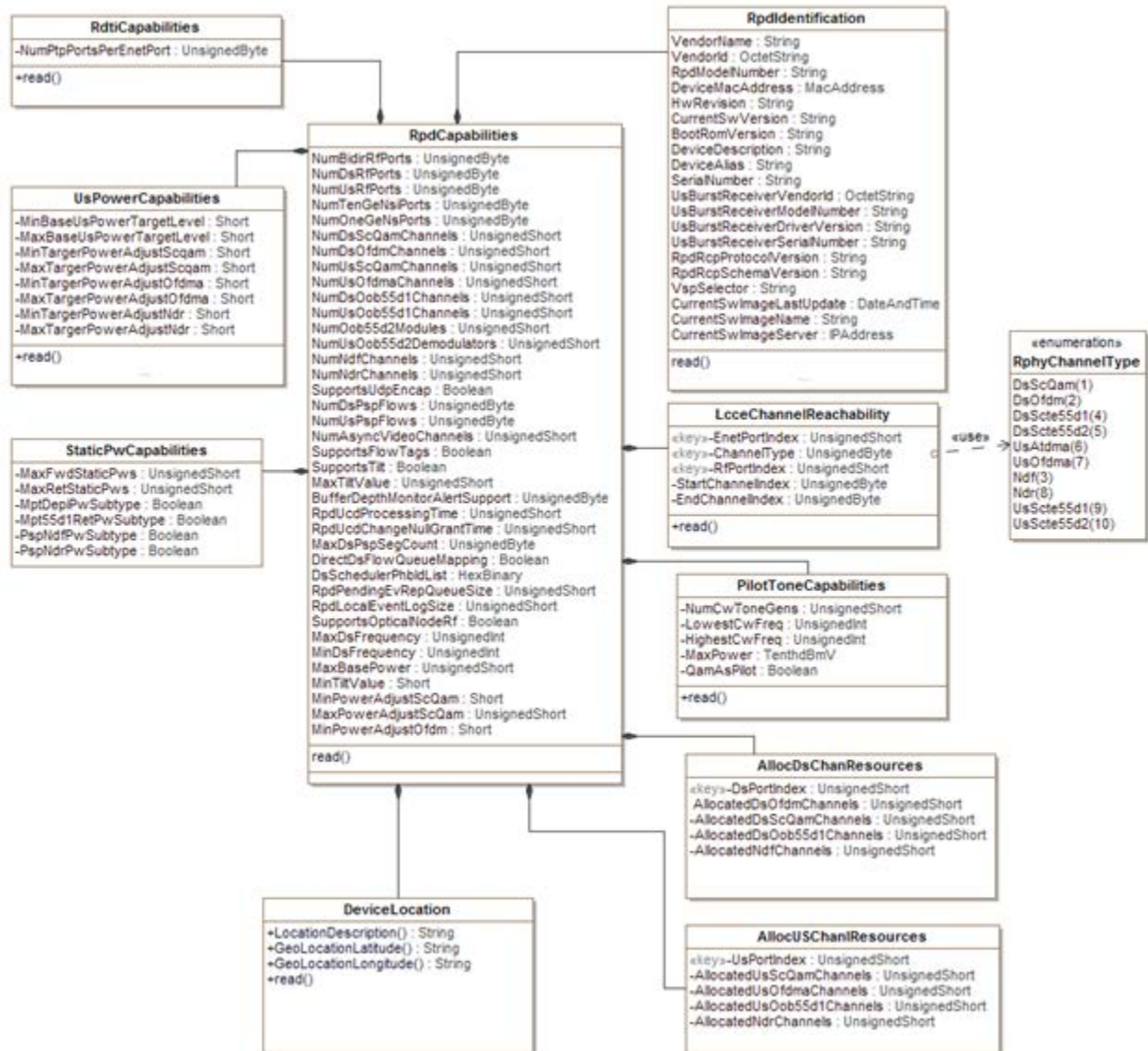
Figure 34 - RPD Capabilities Objects
