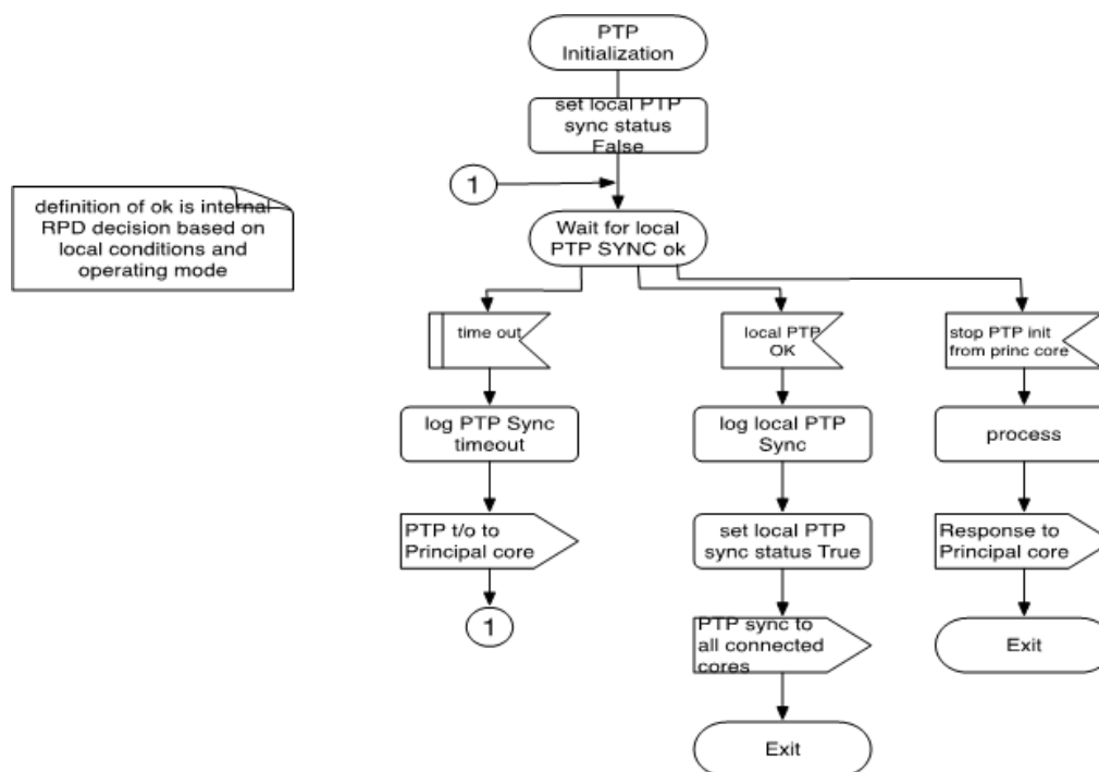
Figure 22 - PTP Synchronization
