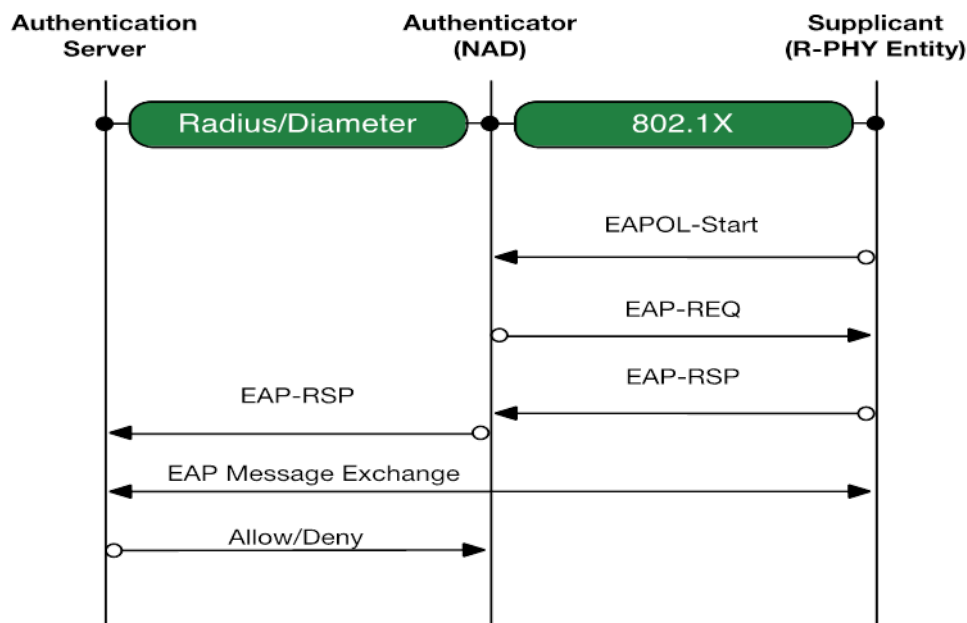
Figure 10 - Network Authentication Signaling
