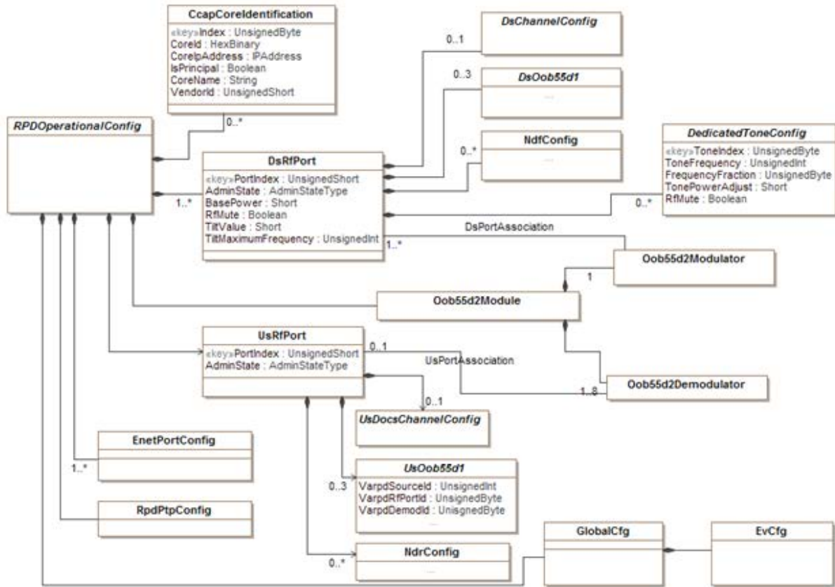
Figure 35 - RPD Operational Configuration Objects
