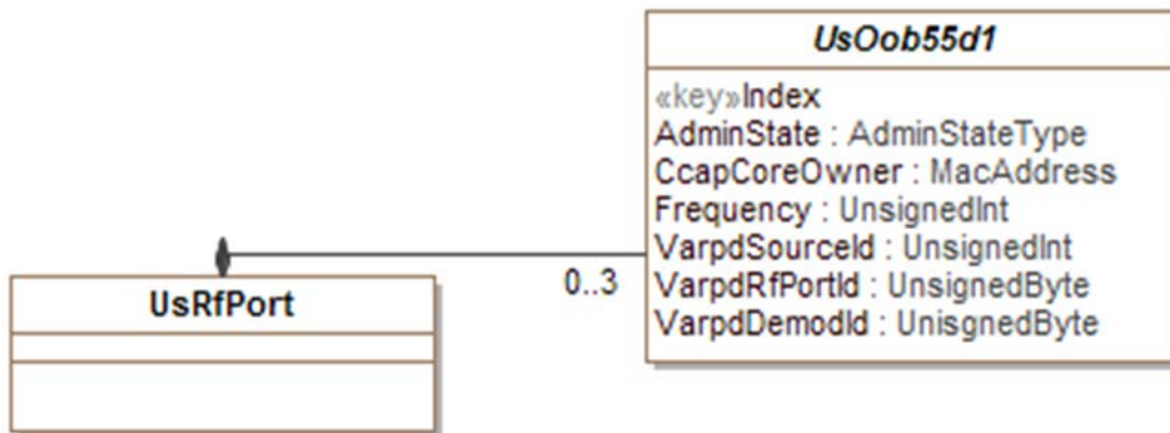
Figure 43 - SCTE 55-1 Upstream Channel Configuration
