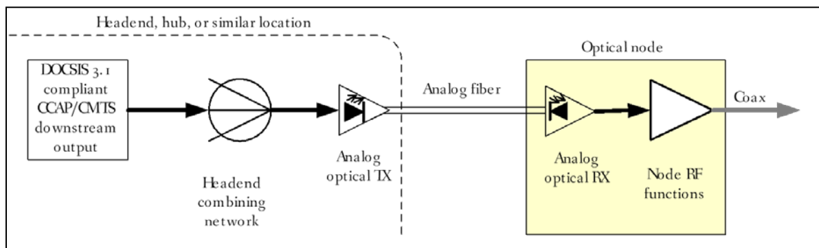
Figure 53 - Traditional Downstream RF Signal Path
