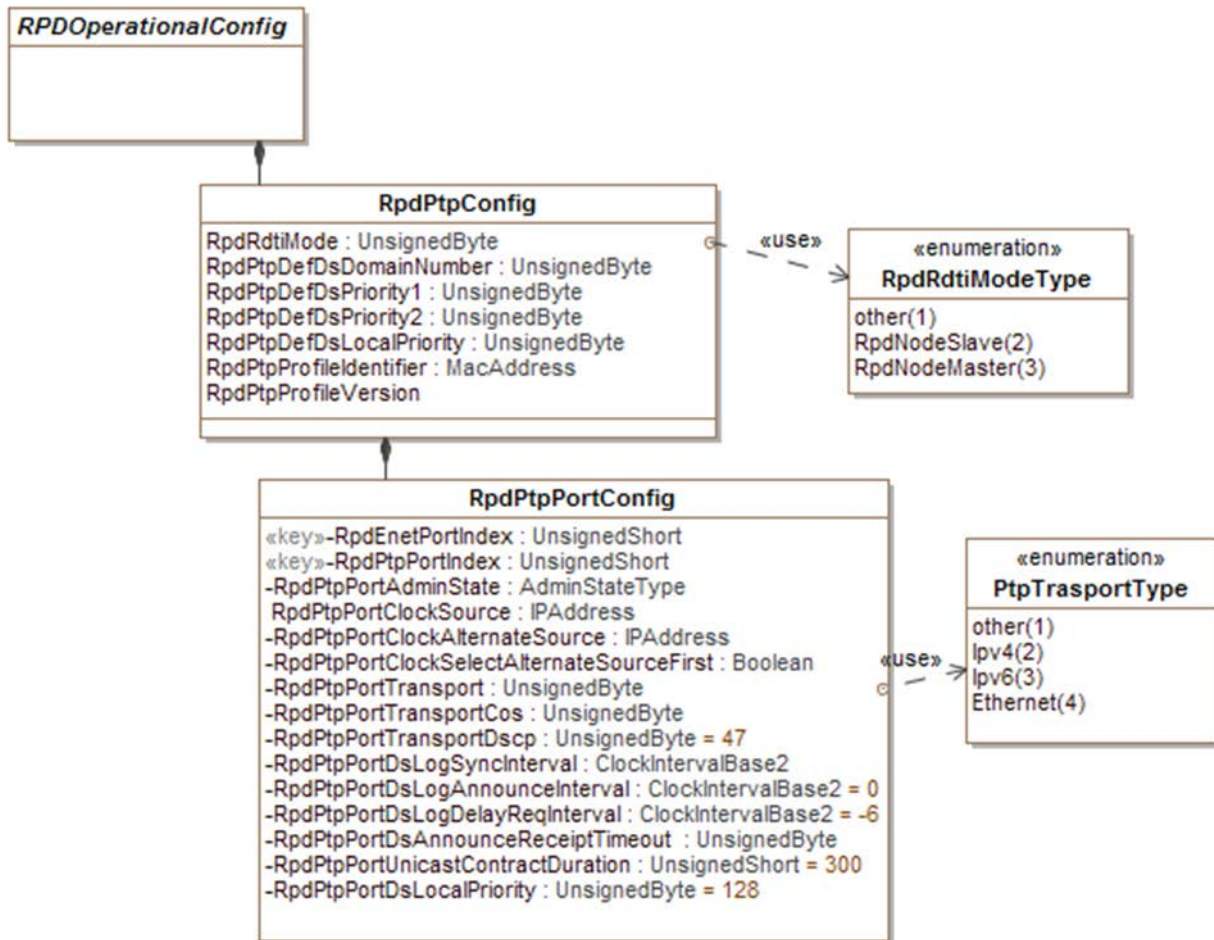
Figure 47 - RPD RDTI Configuration Attributes
