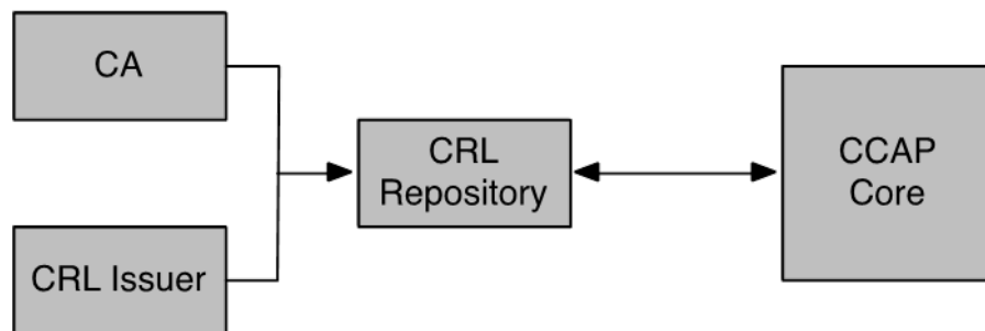
Figure 25 - CRL Framework
