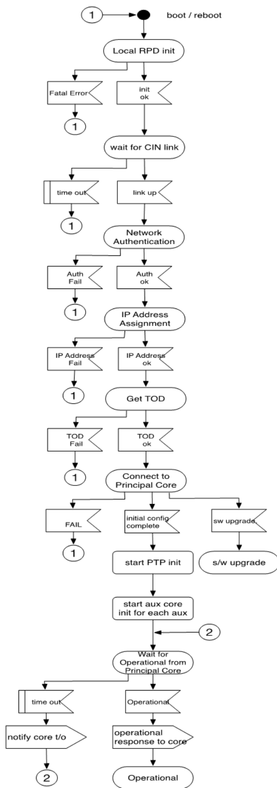
Figure 6 - RPD Initialization
