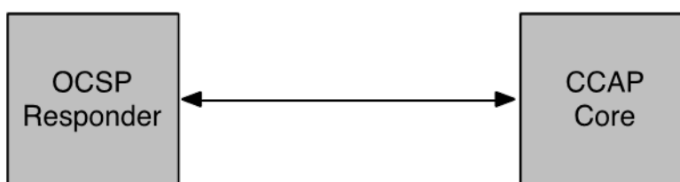
Figure 26 - OCSP Framework
