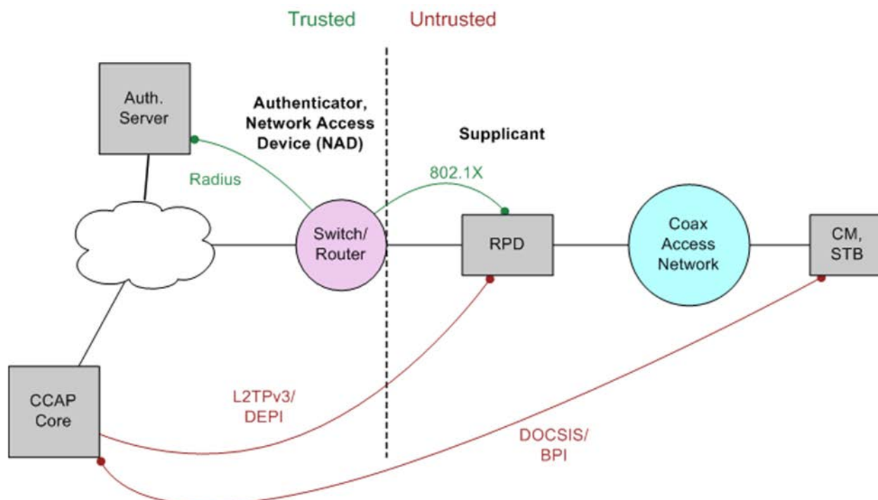
Figure 8 - Remote PHY: Trusted Domain and Untrusted Domain
