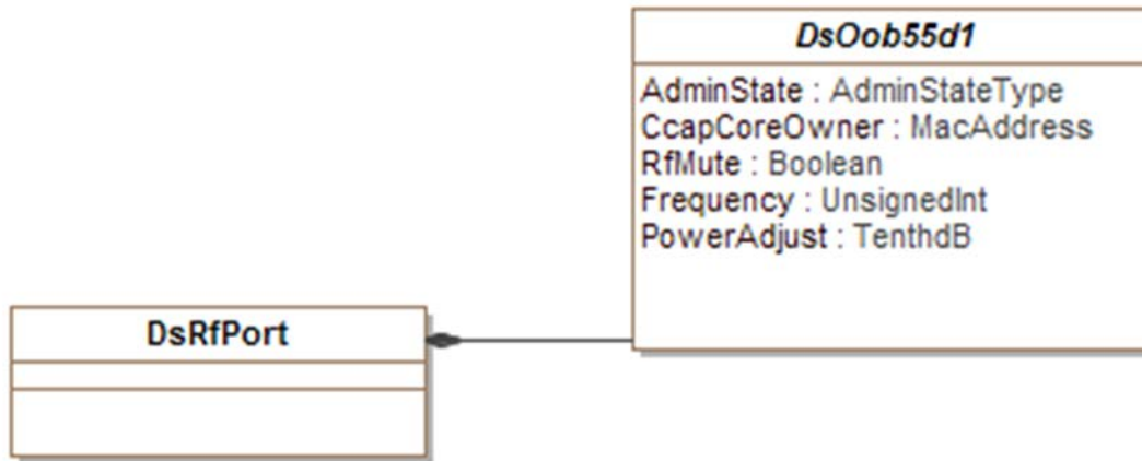
Figure 42 - SCTE 55-1 Downstream Channel Configuration
