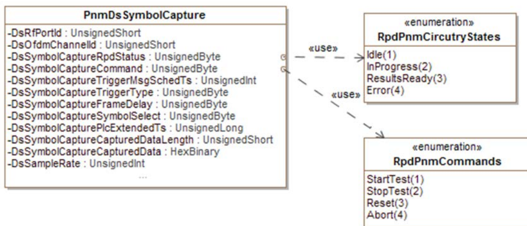
Figure 27 - GCP Objects used in DS Symbol Capture
