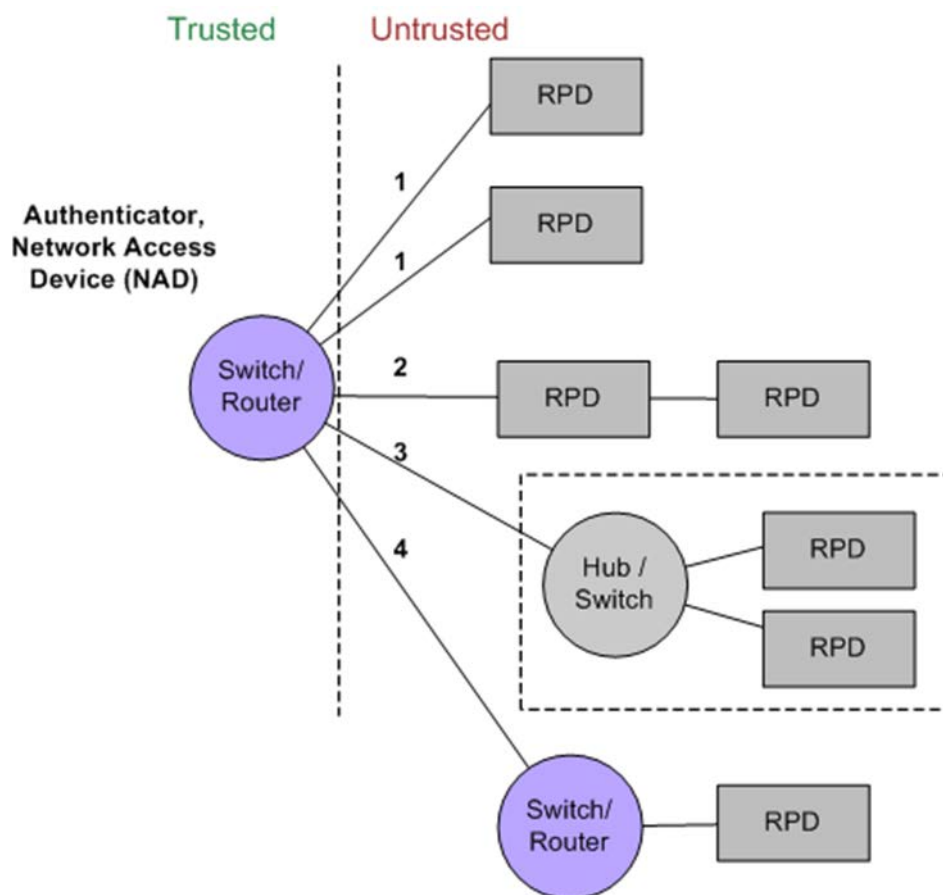
Figure 11 - RPD Topologies for 802.1x
