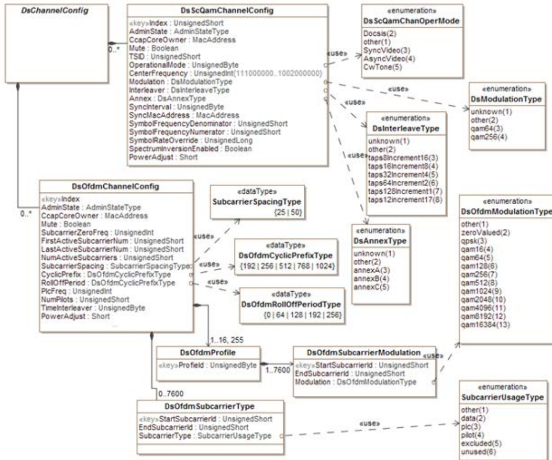
Figure 36 - RPD DOCSIS and MPEG Video Downstream Channel Configuration
