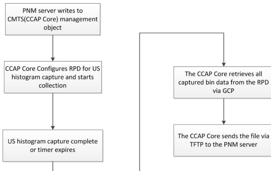
Figure 30 - US Histogram Capture Flow in R-PHY Architecture
