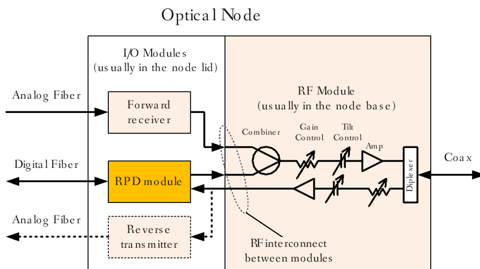
Figure 52 - R-PHY RF Interface Definition
