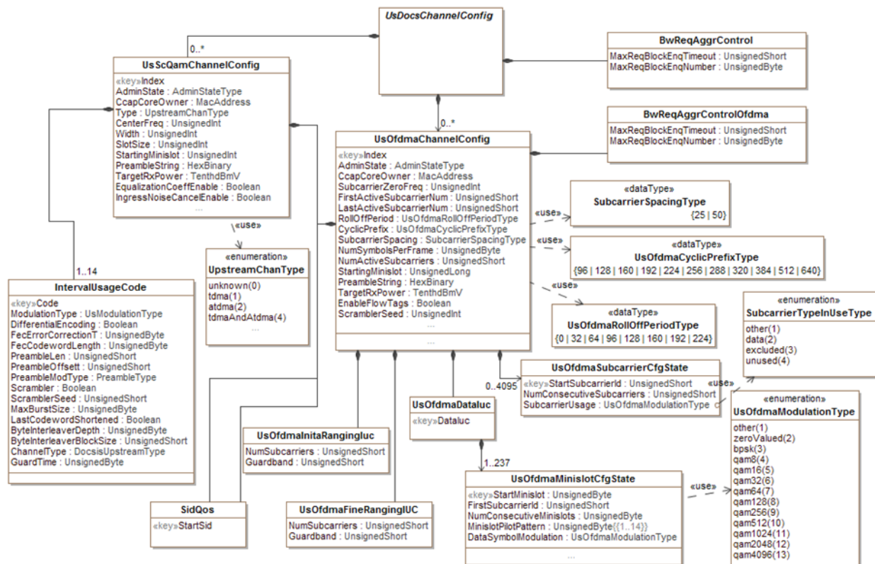
Figure 37 - DOCSIS Upstream Channel Configuration
