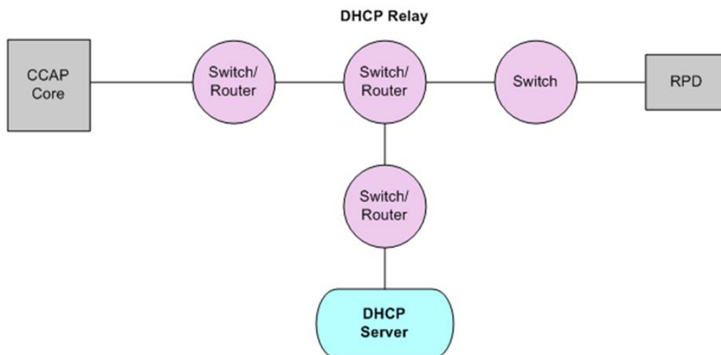
Figure 13 - DHCP Network Diagram
