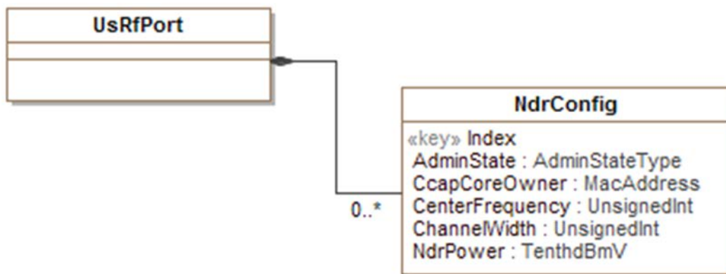
Figure 46 - NDR Configuration Objects.
