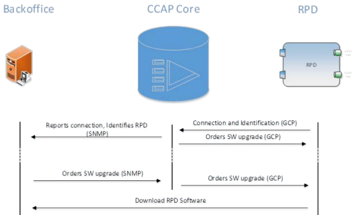
Figure 24 - RPD SW Upgrade Procedure
