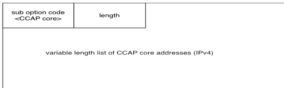
Figure 15 - CCAP Cores DHCP Suboption IPv4
