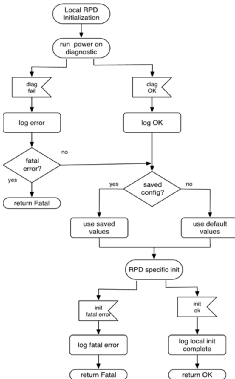
Figure 7 - Local RPD Initialization
