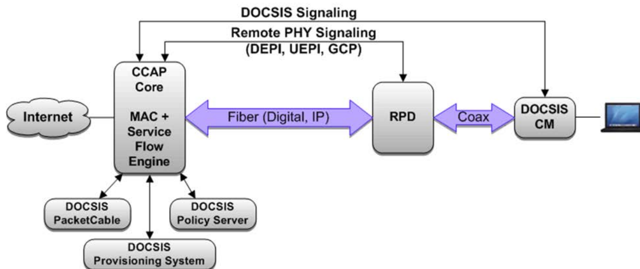
Figure 3 - MHA v2 Reference Architecture for DOCSIS Signaling and Provisioning
