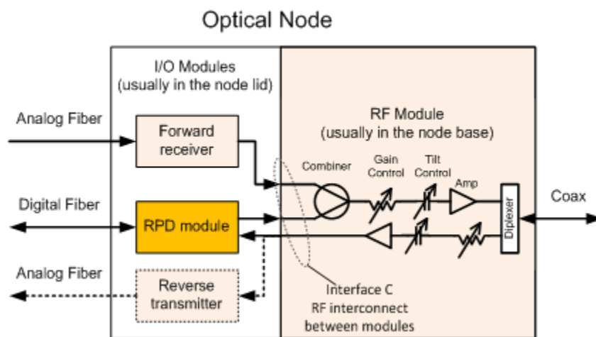
Figure 51 - R-PHY Upstream RF Signal Path
