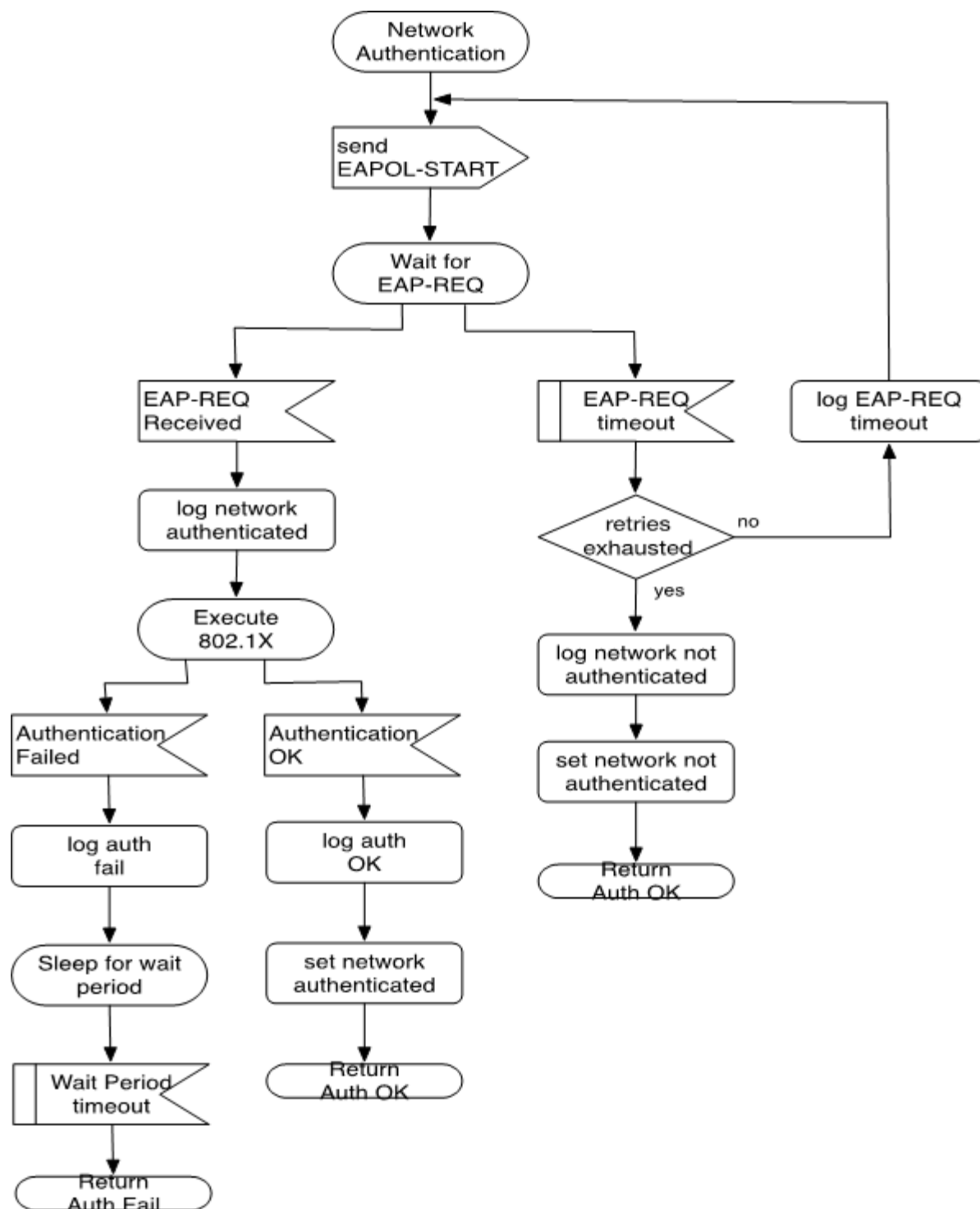
Figure 12 - RPD Authentication using 802.1x
