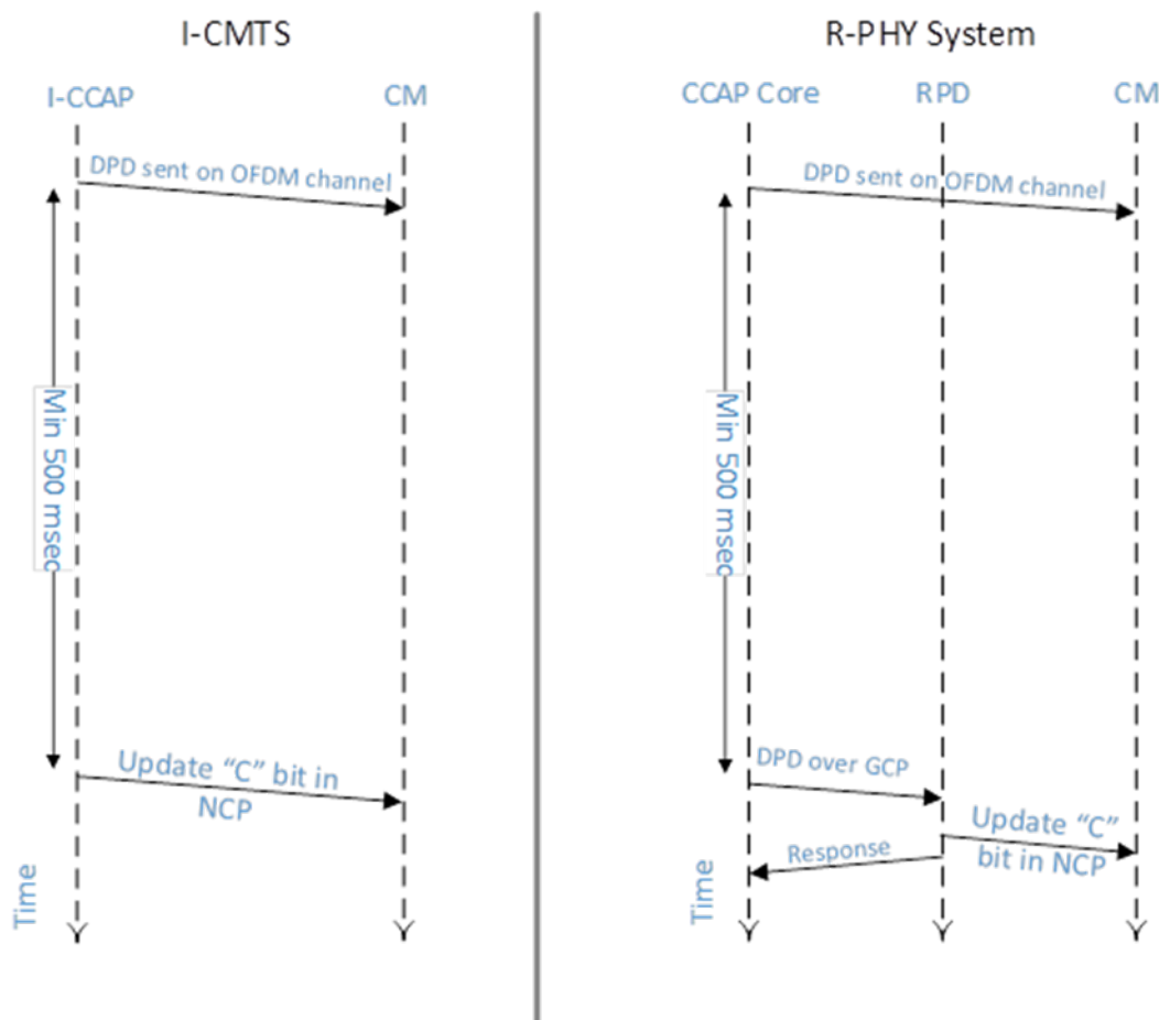
Figure 32 - Comparison of OFDM Profile Change Procedures between I-CCAP and R-PHY System
