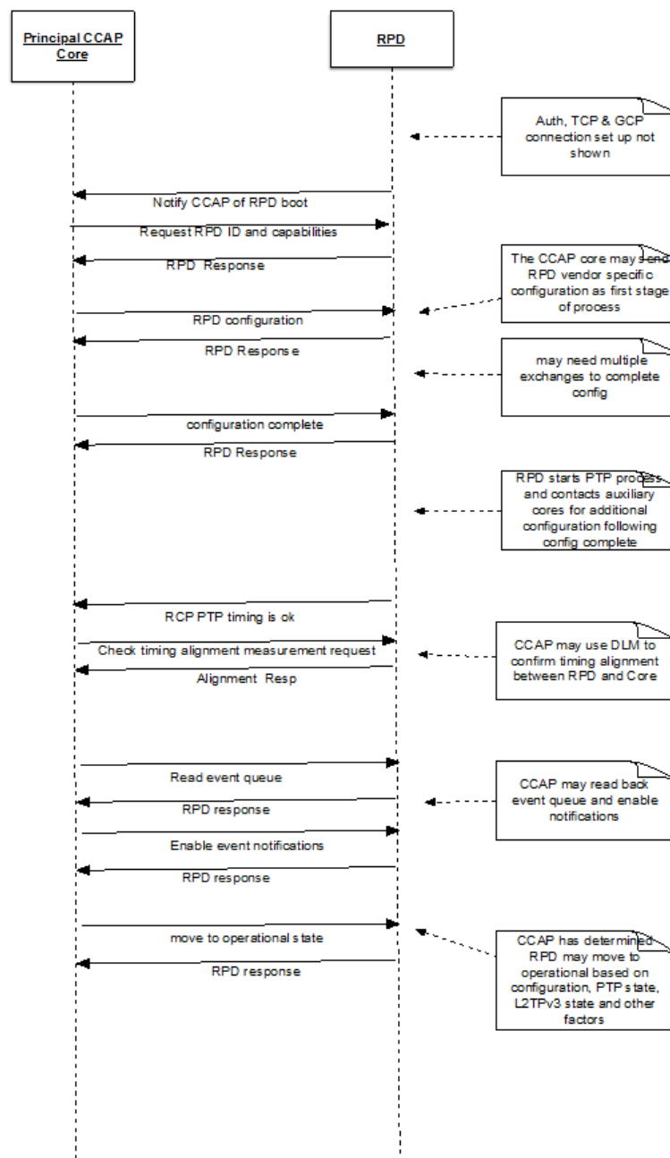
Figure 17 - Message Exchanges RPD and Principal Core
