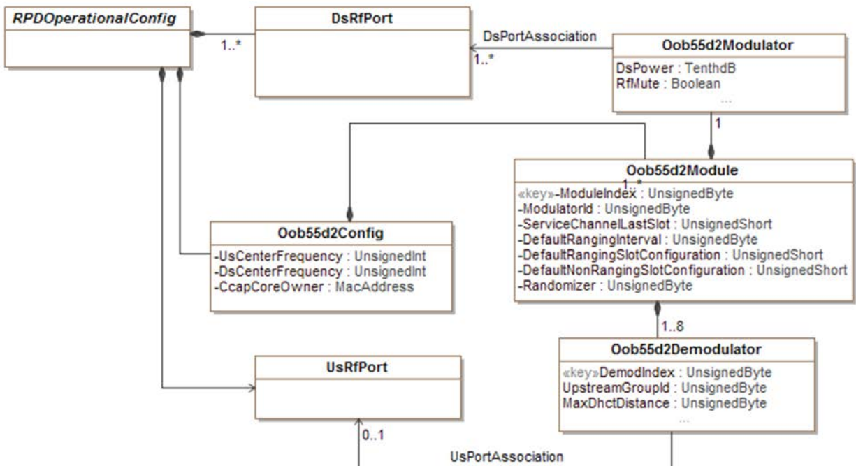
Figure 44 - SCTE 55-2 OOB Configuration Objects
