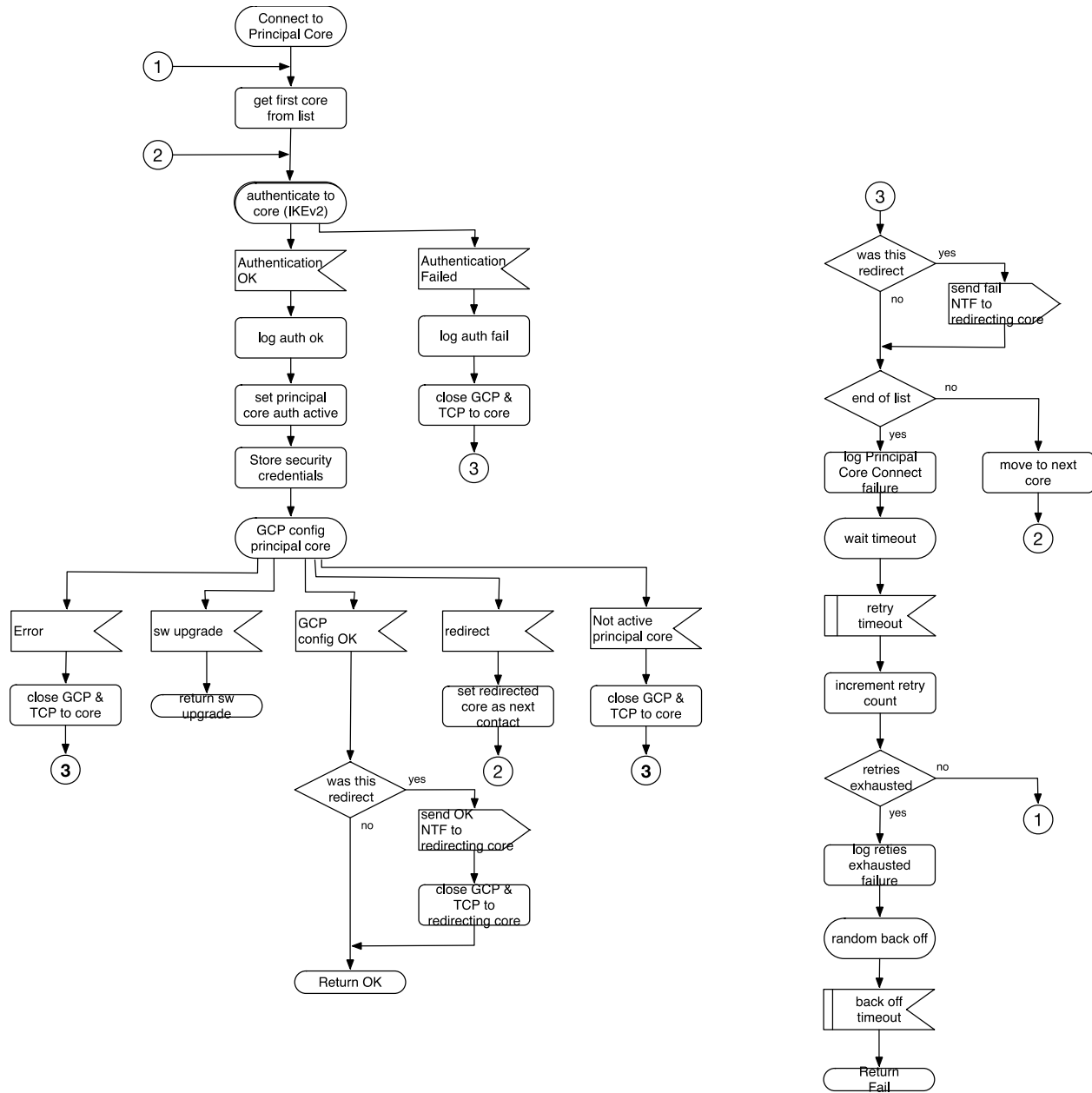
Figure 18 - Process for Connecting to the Principal Core
