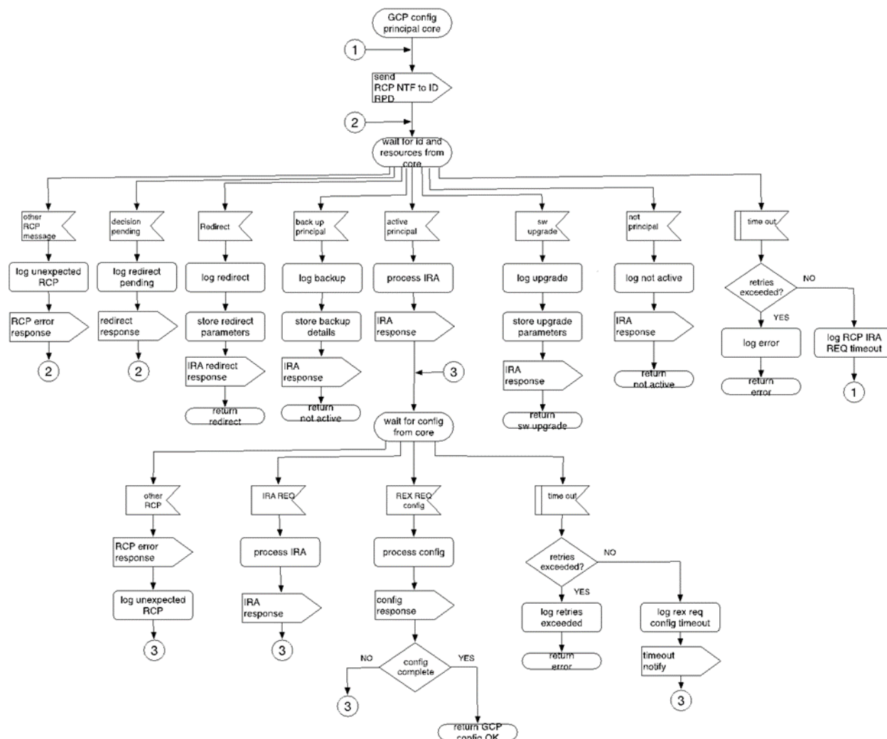
Figure 19 - Configuration by Principal Core
