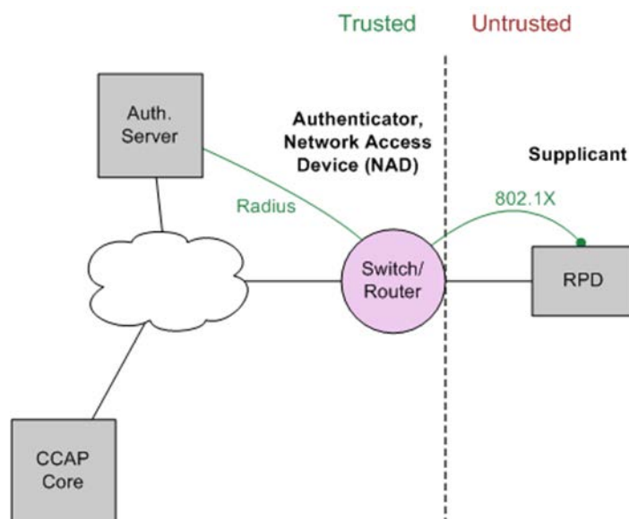
Figure 9 - Authentication Network Diagram
