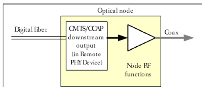
Figure 54 - R-PHY Downstream RF Signal Path
