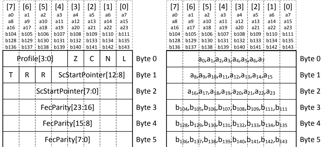
Figure 7-69 - Mapping FEC Encoded NCP Bytes into a Bitstream
