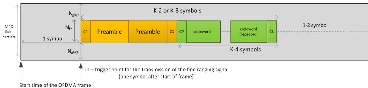
Figure 7-27 - Fine Ranging Signal Transmission
