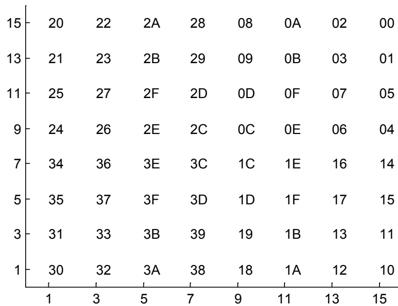
Figure A-10 - 256-QAM Constellation Mapping of \{y_2y_3y_4y_5y_6y_7\} on to Quadrant 1
