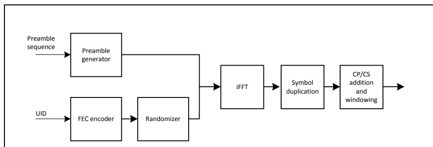
Figure 7-21 - Block Diagram of Initial Ranging Transmitter Processing
