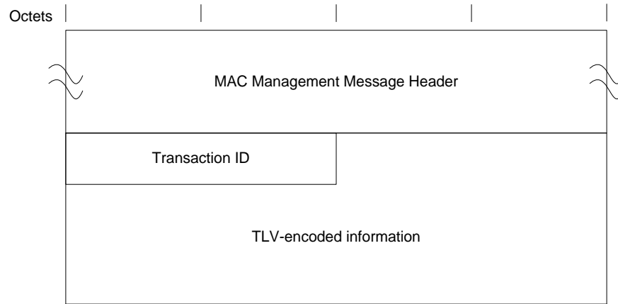
Figure 6–57 - CM-CTRL-RSP
