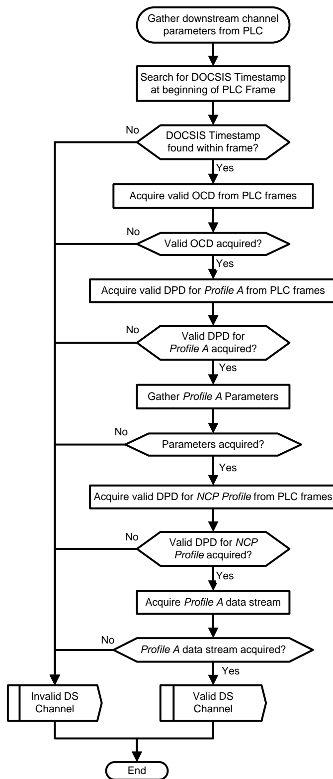
Figure 10-3 - Gather Downstream Channel Parameters from PLC
