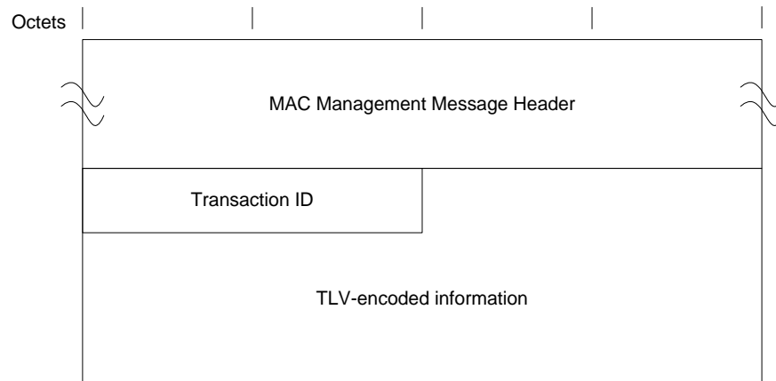
Figure 6–69 - DTP Request Message
