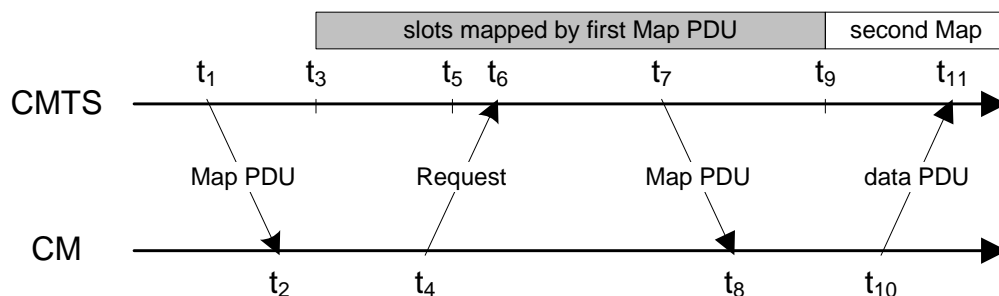
Figure 7–3 - Protocol Example
