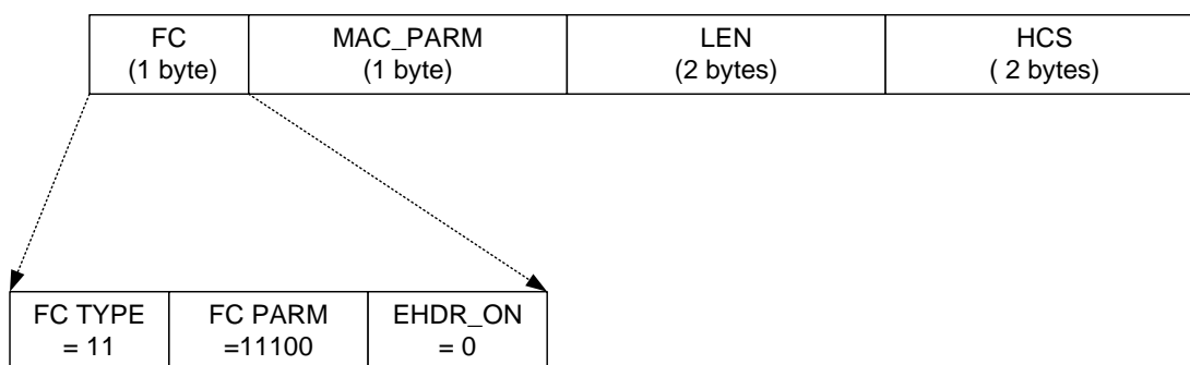
Figure 6–9 - Concatenation MAC Header Format
