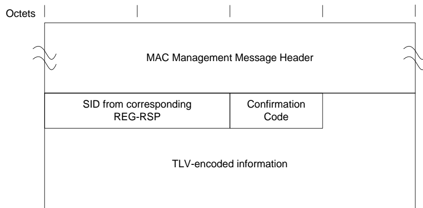
Figure 6–37 - Registration Acknowledgment
