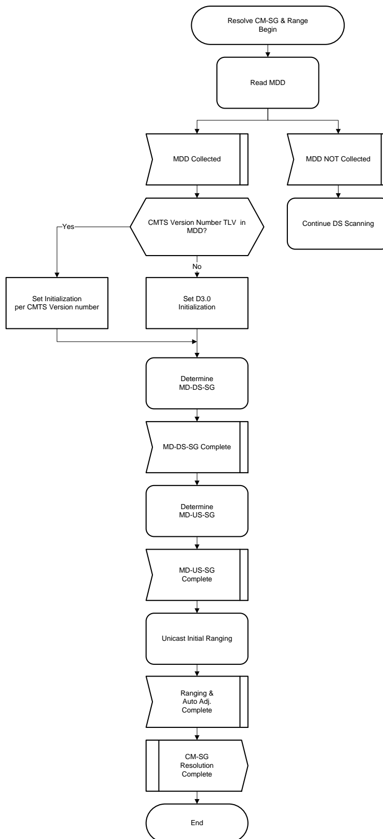
Figure 10-4 - Resolve Service Group (SG) and Range
