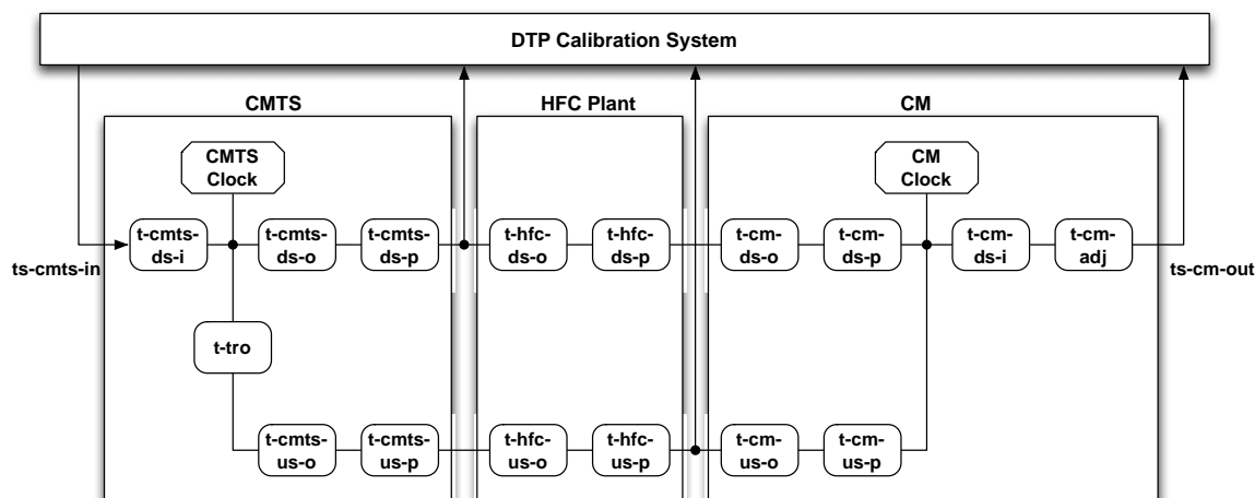
Figure 10–50 - DTP Math and Delays
