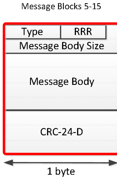
Figure 6–79- Generic Format for Message Blocks 5-15
