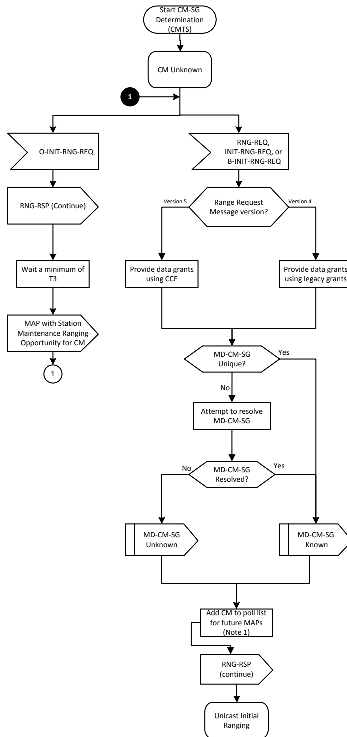
Figure 10–15 - CM-SG Determination - CMTS
