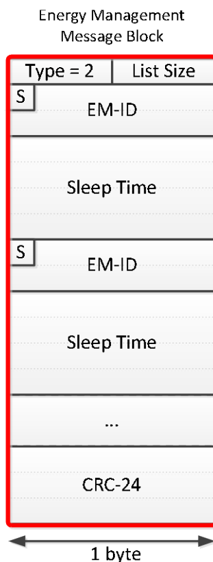
Figure 6–76 - Energy Management Message Block
