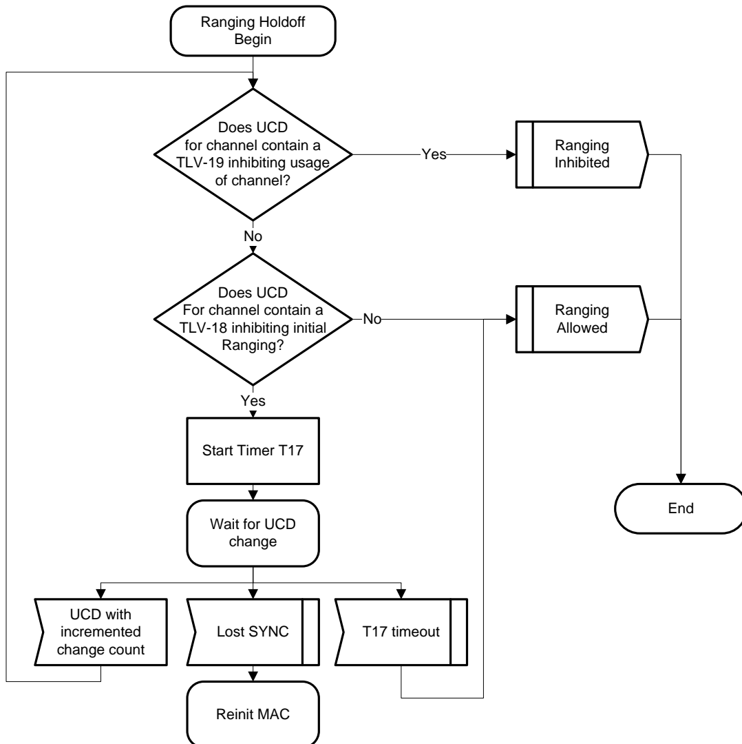
Figure 10–8 - Ranging Holdoff
