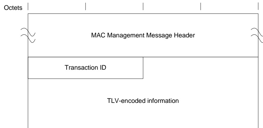
Figure 6–71 - DTP-INFO Message
