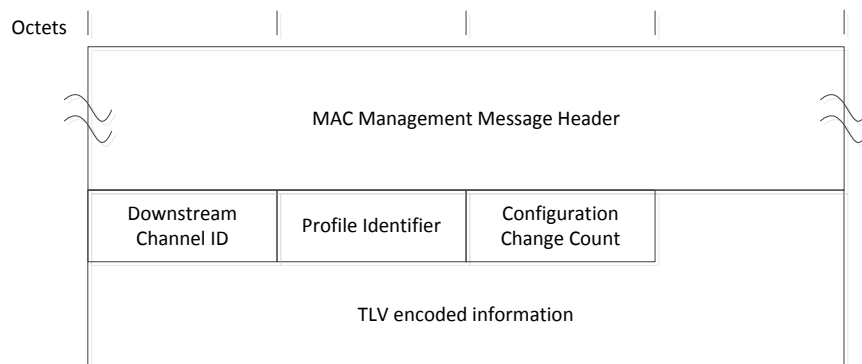
Figure 6–62 - Downstream Profile Descriptor
