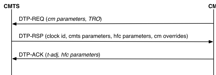
Figure 10–53 - CM is DTP Master
