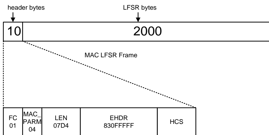
Figure 10-44 - MAC LFSR Frame
