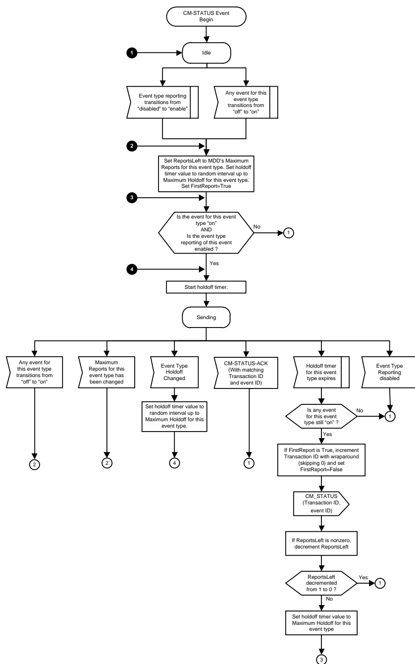
Figure 10–46 - CM-STATUS Event Type State Machine 96
