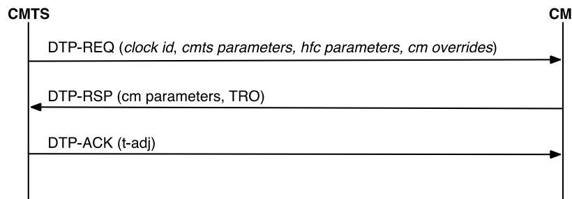
Figure 10–52 - CMTS is DTP Master
