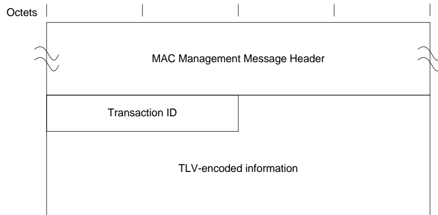
Figure 6–56 - CM-CTRL-REQ
