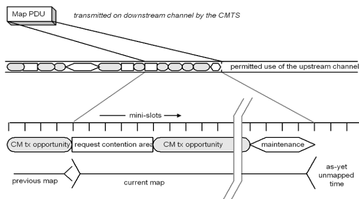
Figure 7-2 - Allocation Map
