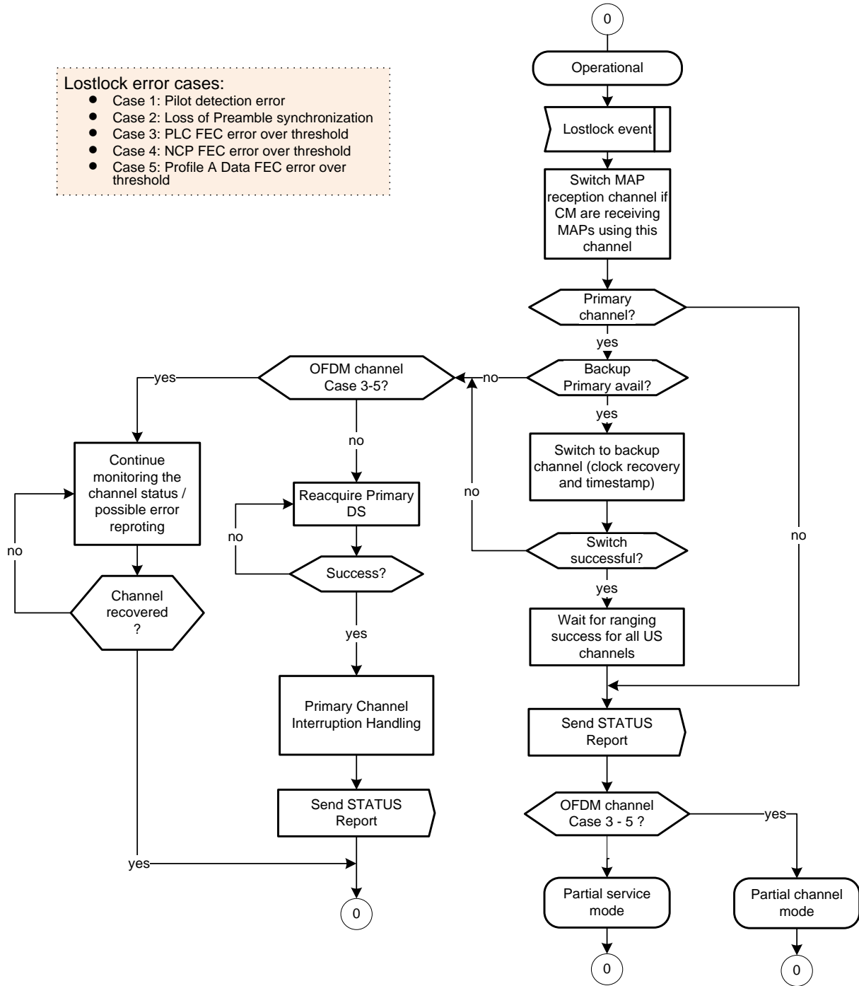
Figure 10–45 - Lost Lock Procedure
