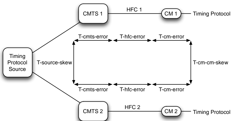
Figure 10-54 - DTP System Performance
