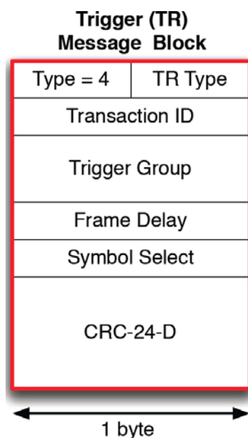
Figure 6–78 - Trigger Message Block
