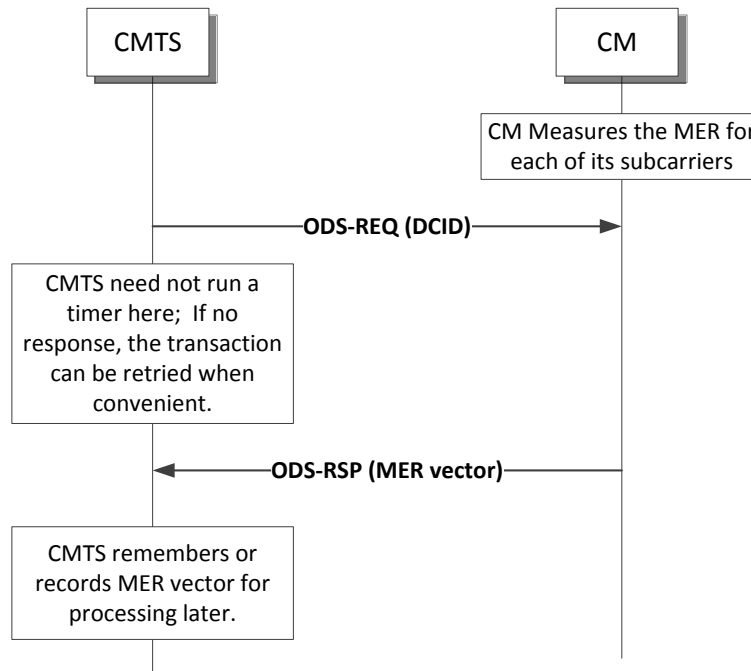
Figure 7–20 - OFDM-Downstream Spectrum Reporting Transaction
