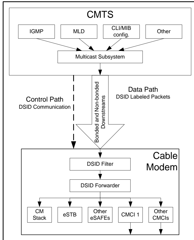
Figure 9-2 - Multicast Model
