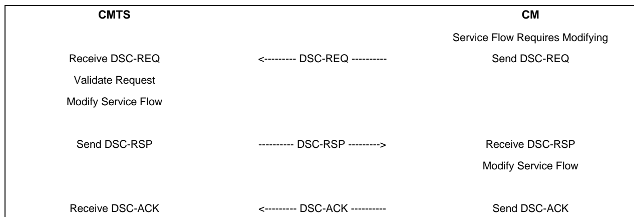
Figure 11–20 - CM-Initiated DSC
