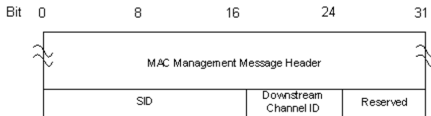
Figure 6–25 - RNG-REQ Format
