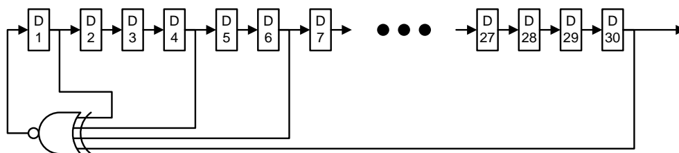
Figure 10-43 - Linear Feedback Shift Register for Synthetic Data Generation
