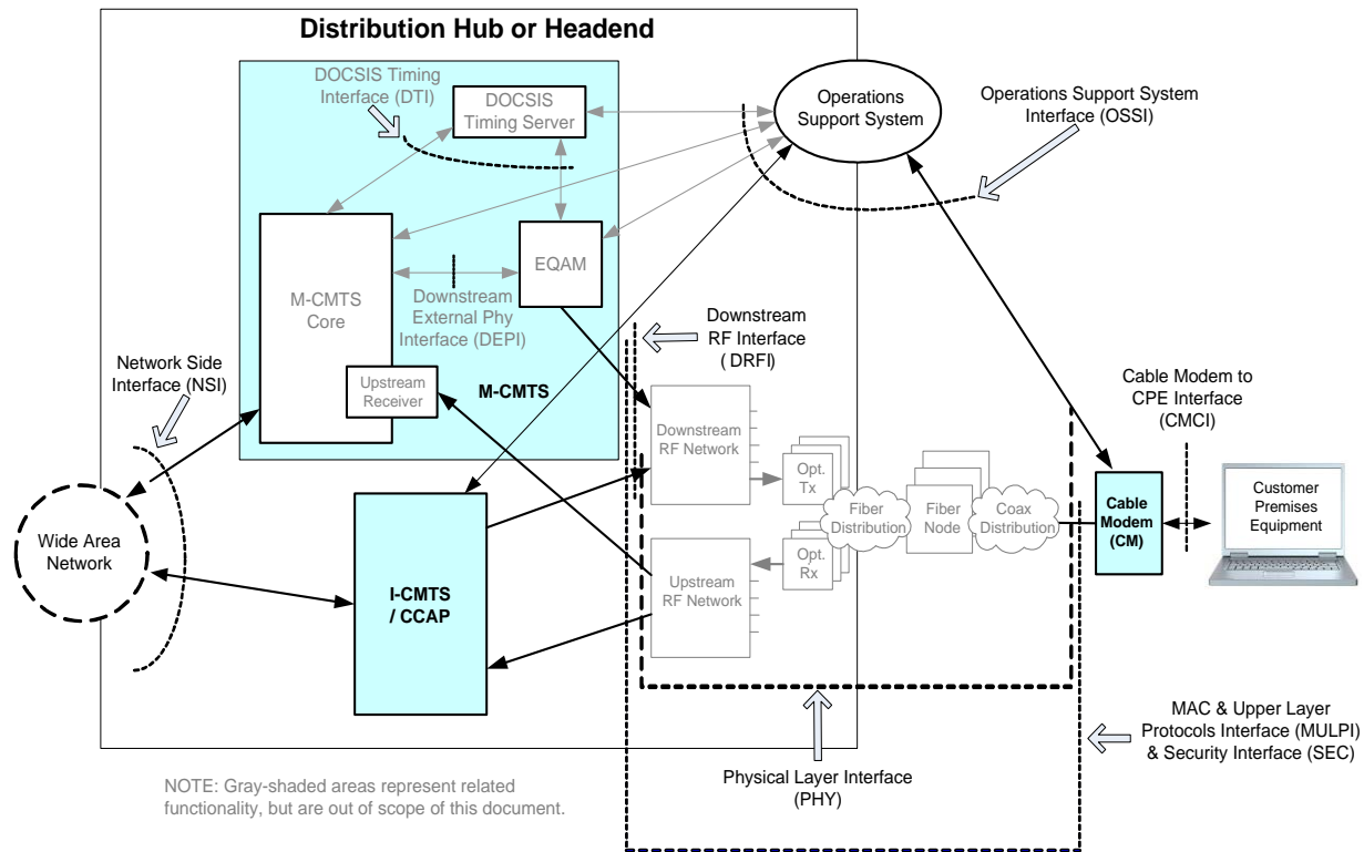
Figure 1-3 - Data-Over-Cable Reference Architecture
