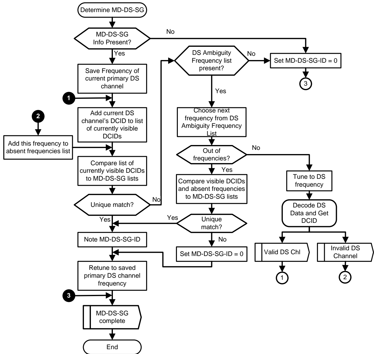
Figure 10–6 - Determine MD-DS-SG
