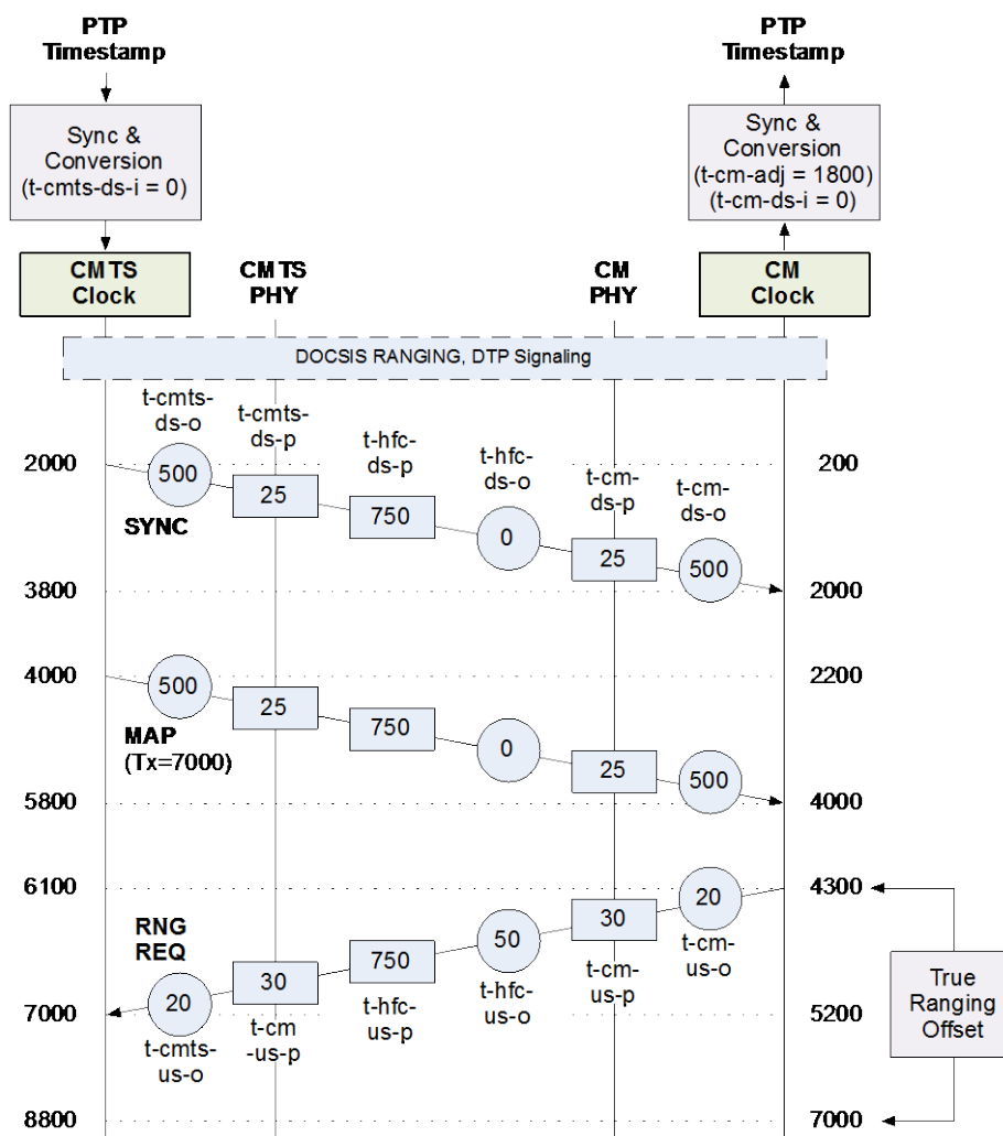
Figure 10-51 - True Ranging Offset Example
