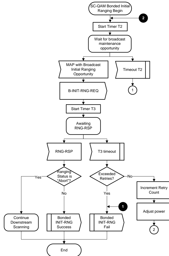
Figure 10–10 - SC-QAM Bonded Initial Ranging
