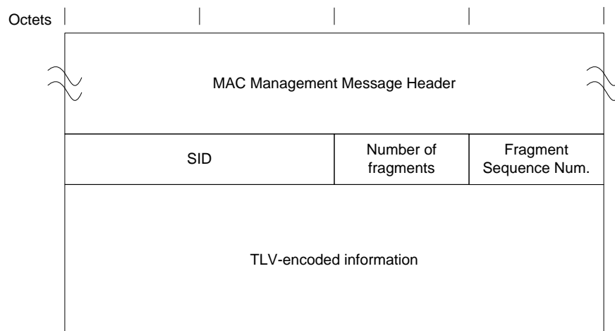
Figure 6–34 - Multipart Registration Request (REG-REQ-MP)
