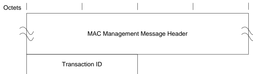
Figure 6–72 - DTP Acknowledge Message
