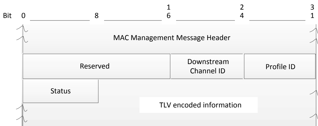
Figure 6–67 - The OFDM Profile Test Response (OPT-RSP) message
