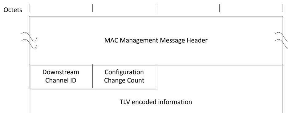
Figure 6–61 - OFDM Channel Descriptor
