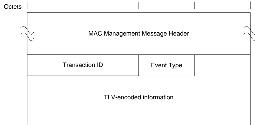
Figure 6–55 - CM-STATUS Report
