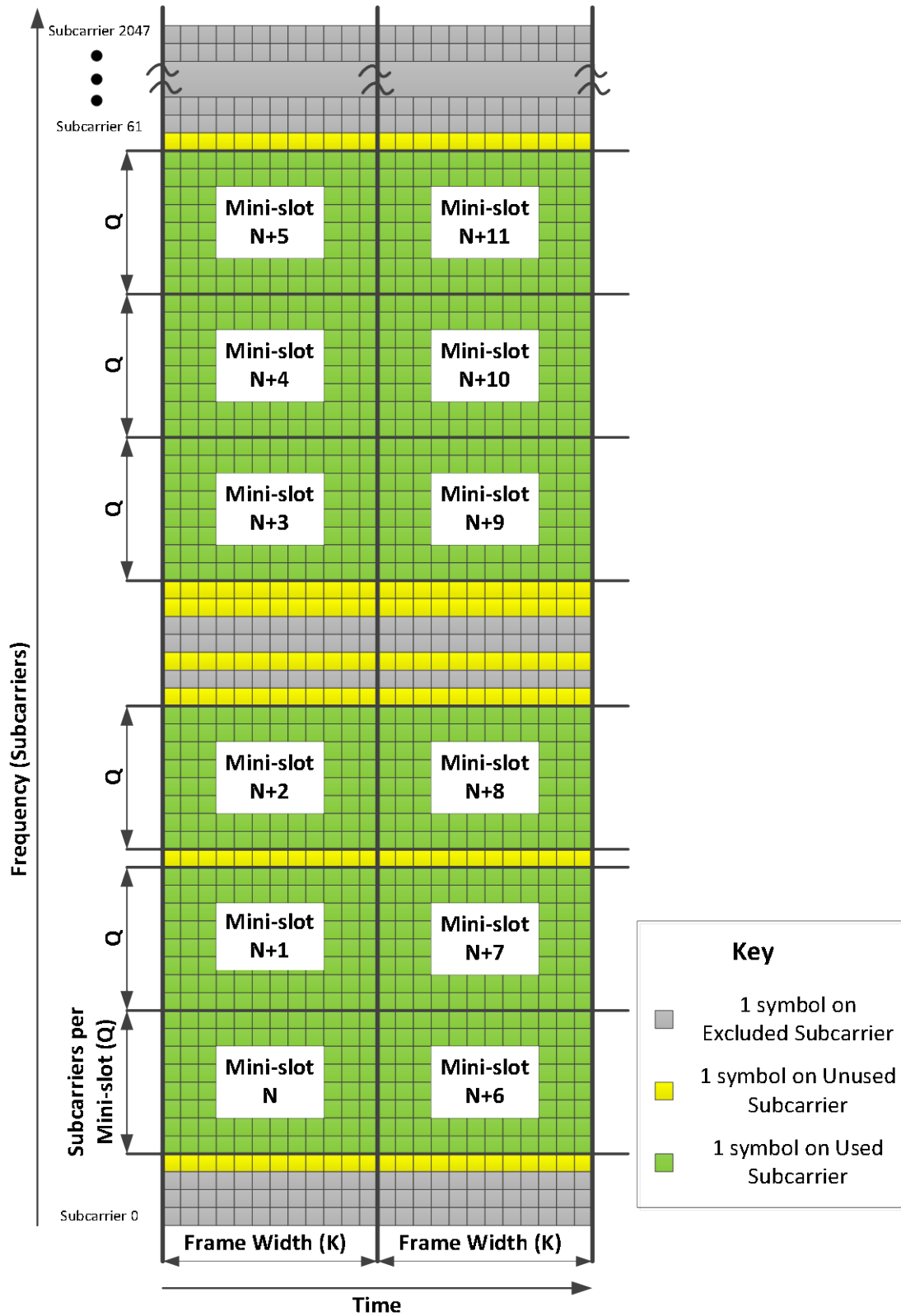
Figure 6-18 - Example Minislot Mapping for OFDMA
