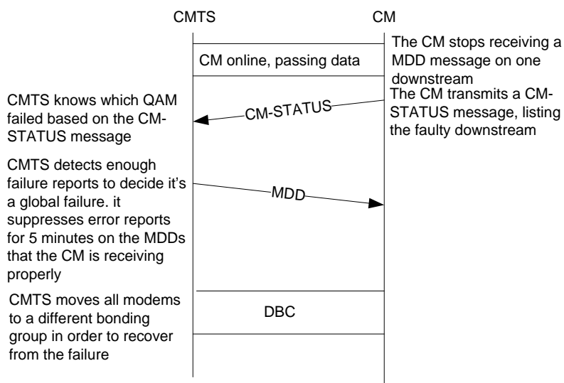
Figure V-2 - Example 2 - Option 4
