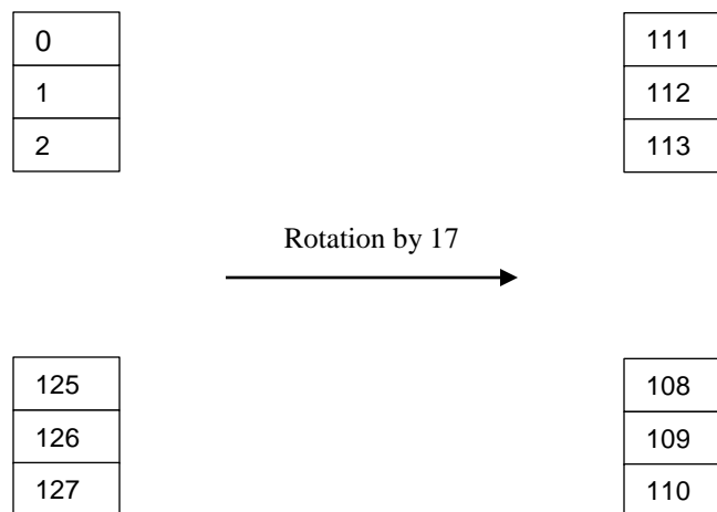
Figure 7-55 - Frequency Interleaver Rotation Definition
