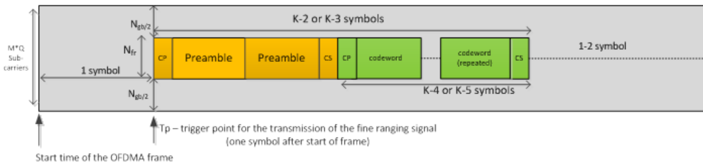
Figure 7-27 - Fine Ranging Signal Transmission 47
