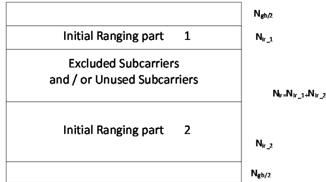
Figure 7-24 - Initial Ranging with Exclusions and Unused Subcarriers
