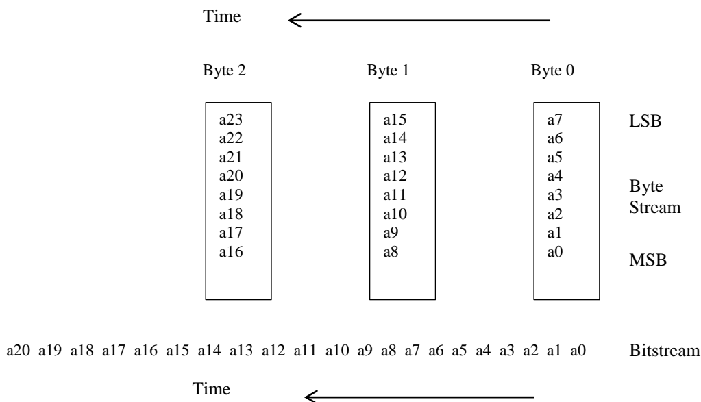
Figure 7-60 - Mapping Bytes into a Bitstream for FEC Encoding
