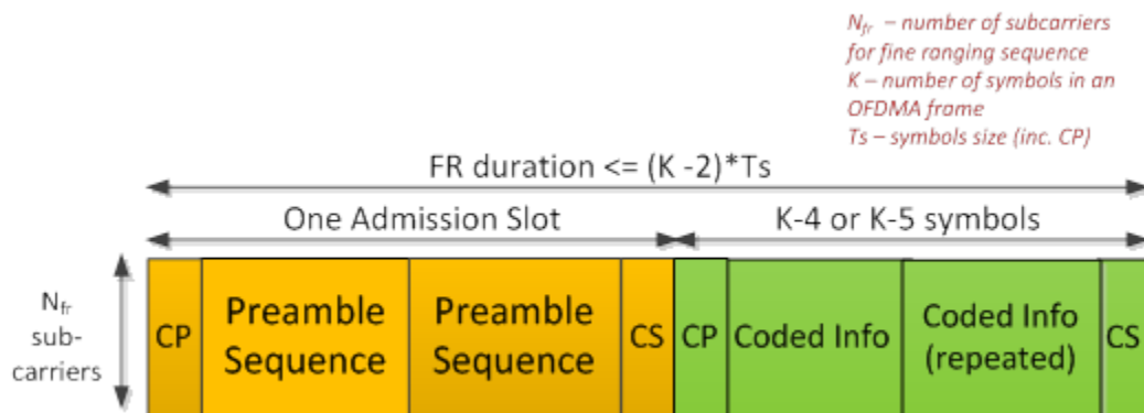
Figure 7-26 - Fine Ranging Signal 46
