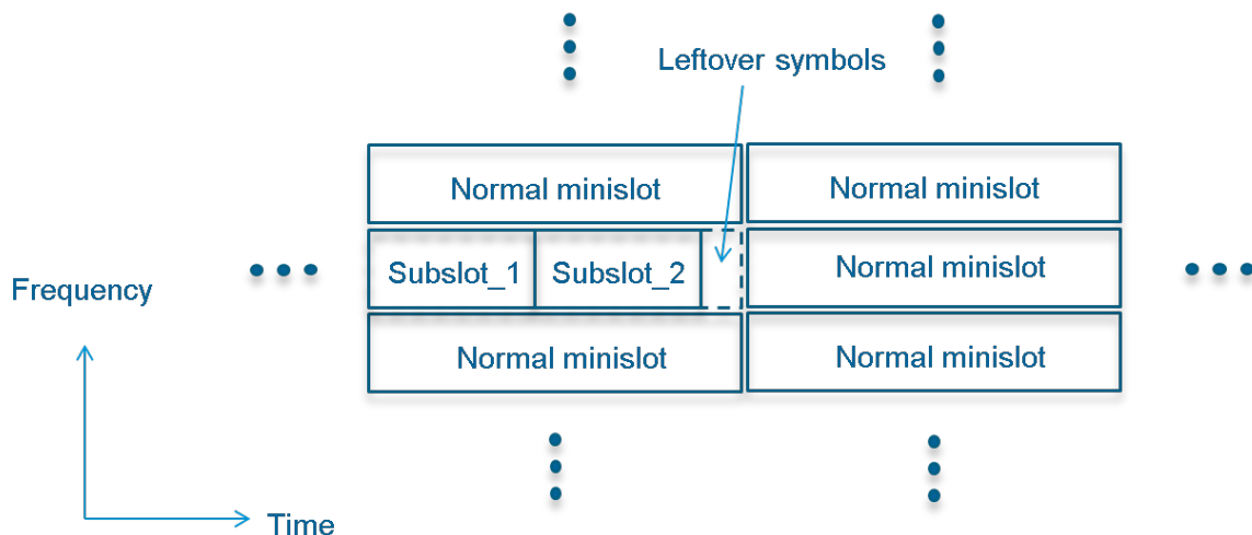
Figure 8-2 - Subslot Structure
