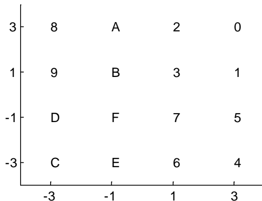
Figure 7-75 - 16QAM Constellation Mapping of \{y_{i,0} y_{i,1} y_{i,2} y_{i,3}\}
