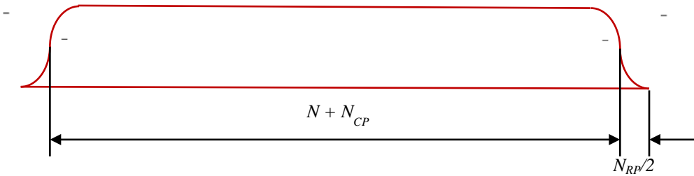
Figure 7-15 - Tapering Window
