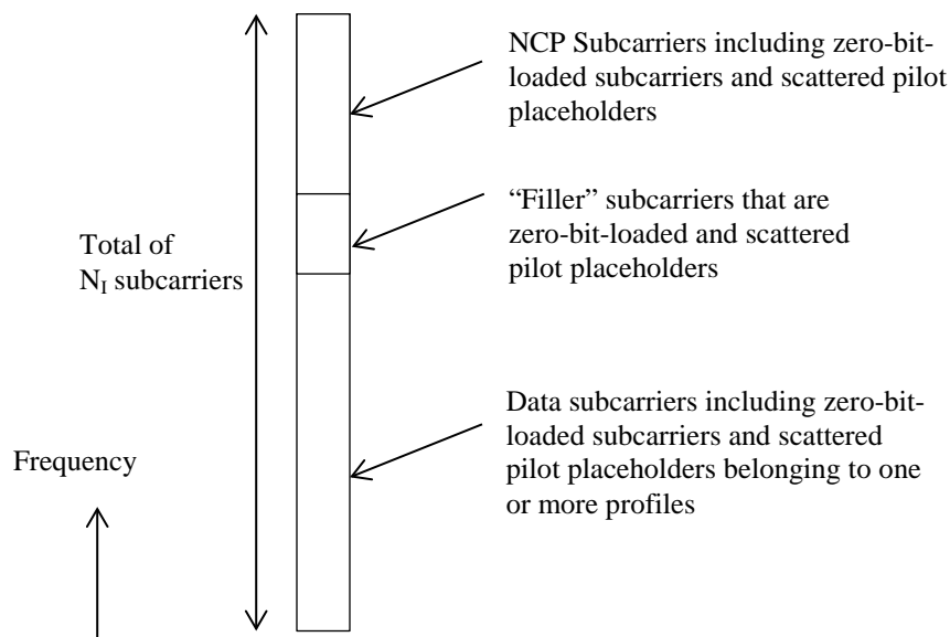
Figure 7-51 - NCP Insertion
