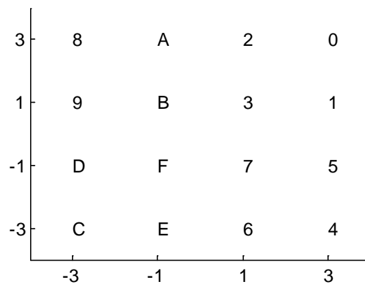
Figure A-4 - 16-QAM Constellation Mapping of \{y_0, y_1, y_2, y_3\}
