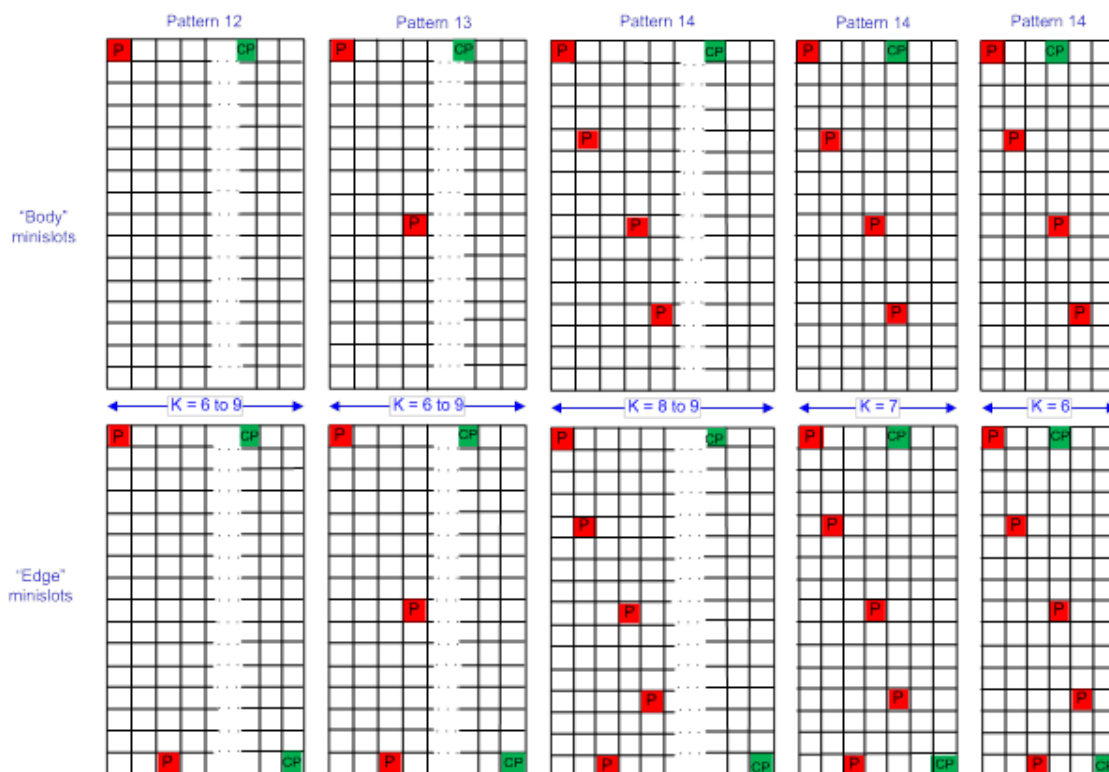
Figure 7-39 - Pilot Patterns 12-14 for Minislots with 16 Subcarriers 51
