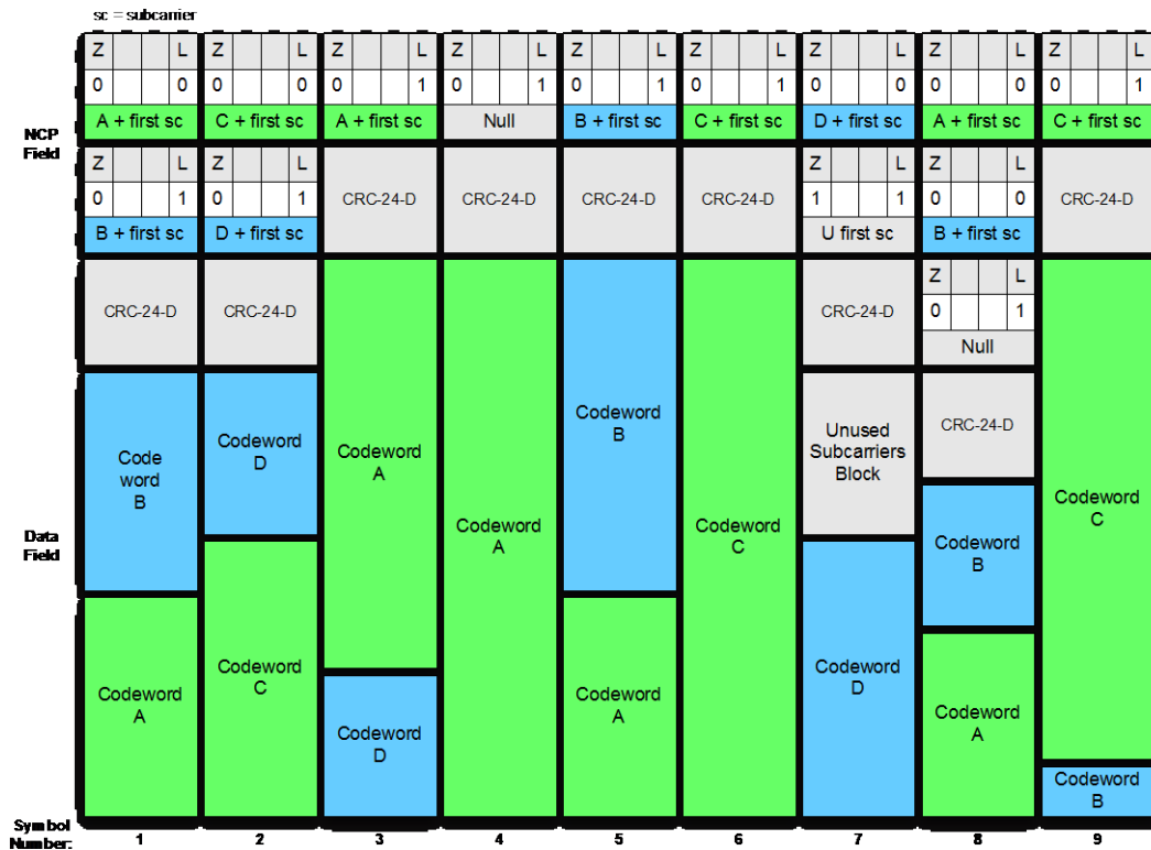
Figure 8-12 - NCP Examples
