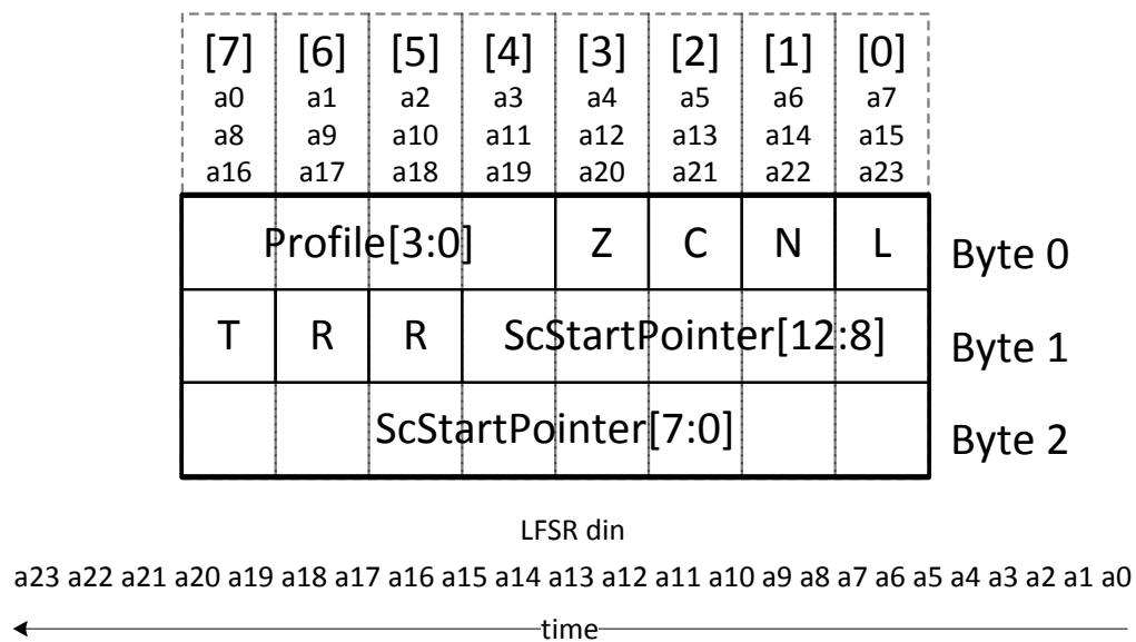
Figure 7-71 - Mapping NCP Data into the CRC-24-D Encoder
