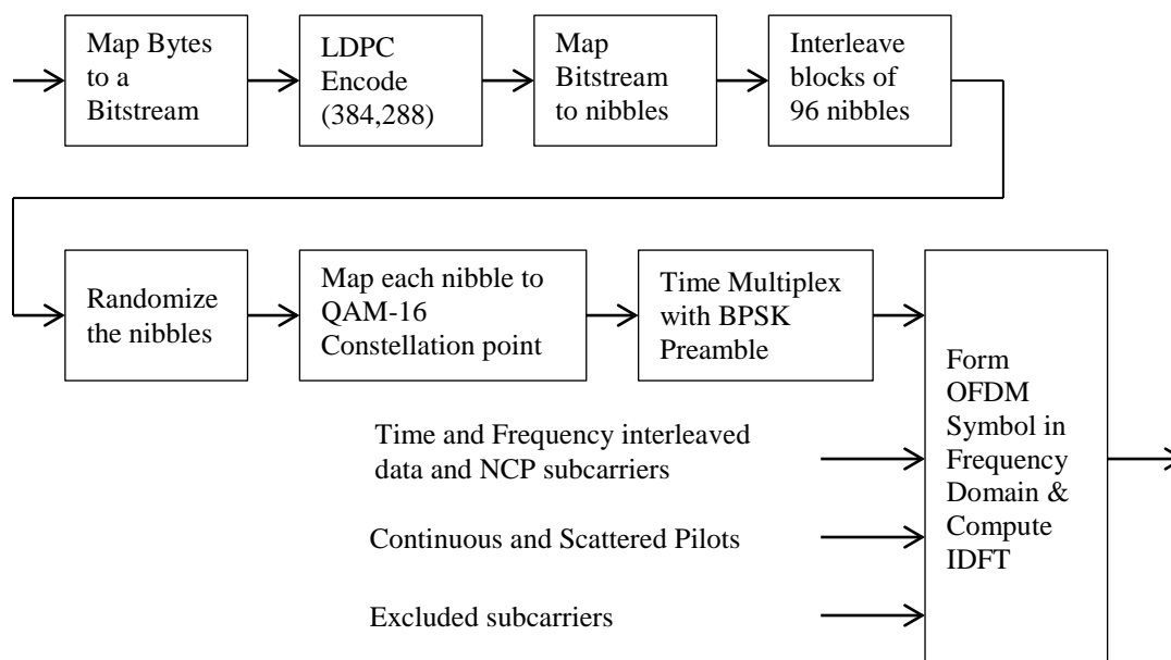
Figure 7-59 - Physical Layer Operations for Forming the PLC Subcarriers
