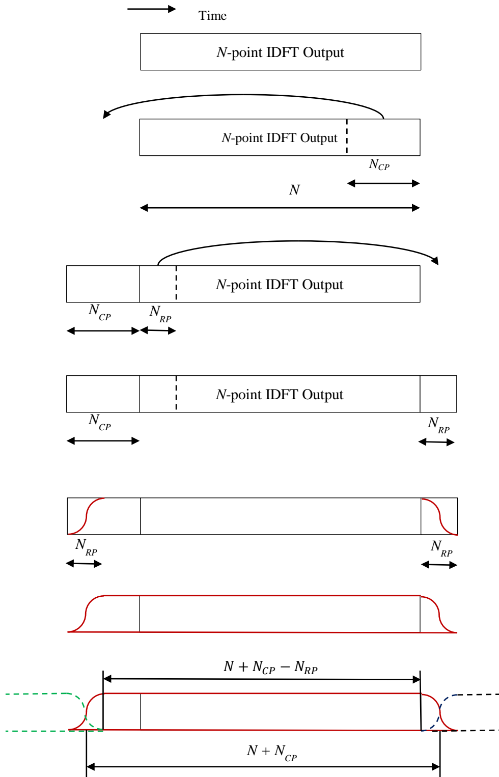
Figure 7-14 - Cyclic Prefix and Windowing Algorithm
