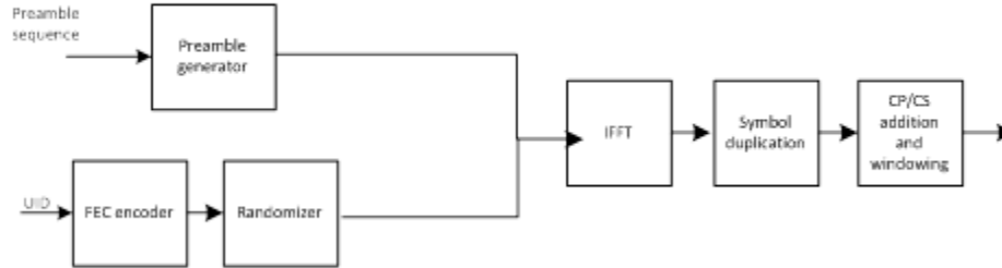
Figure 7-28 - Fine Ranging Transmitter Processing
