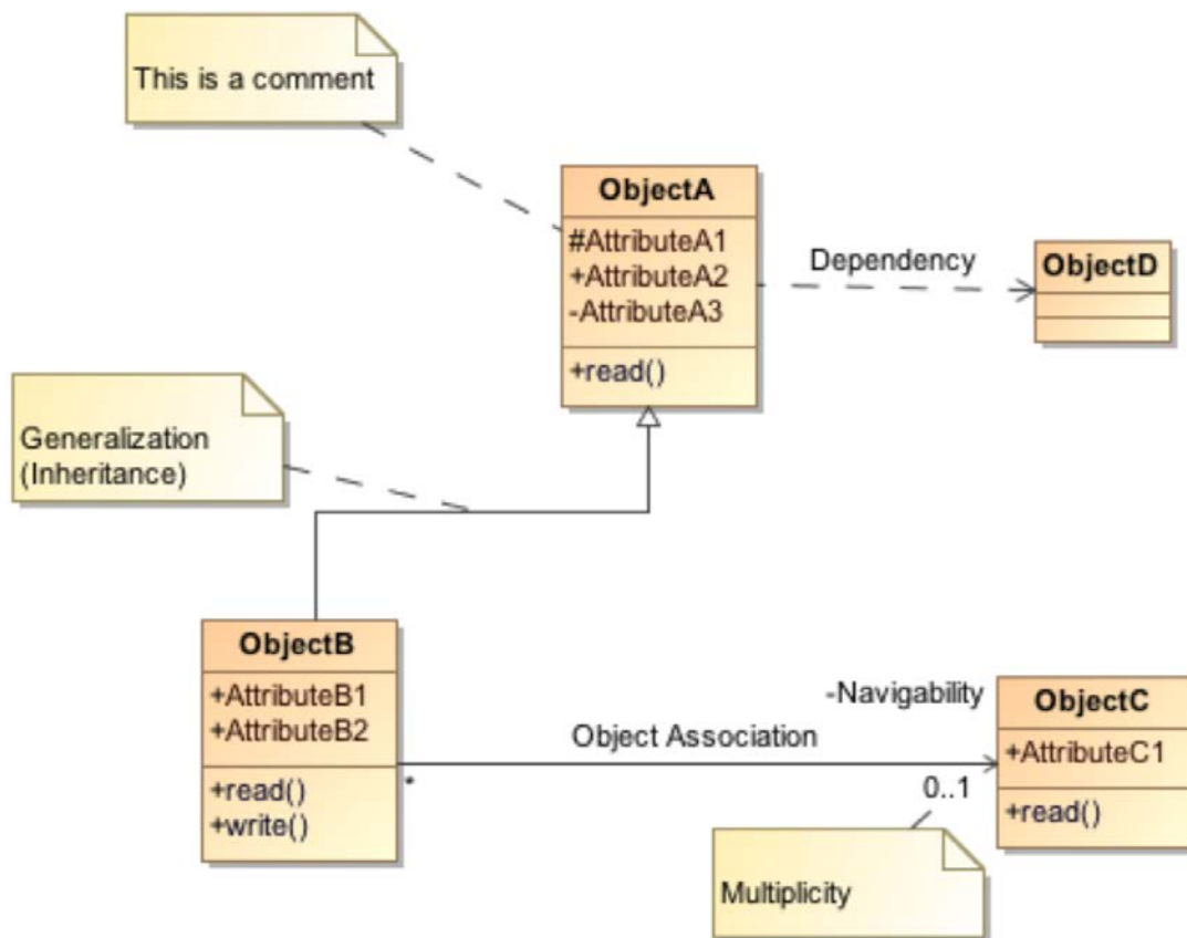
Figure 20 - Information Model UML Class Diagram Notation
