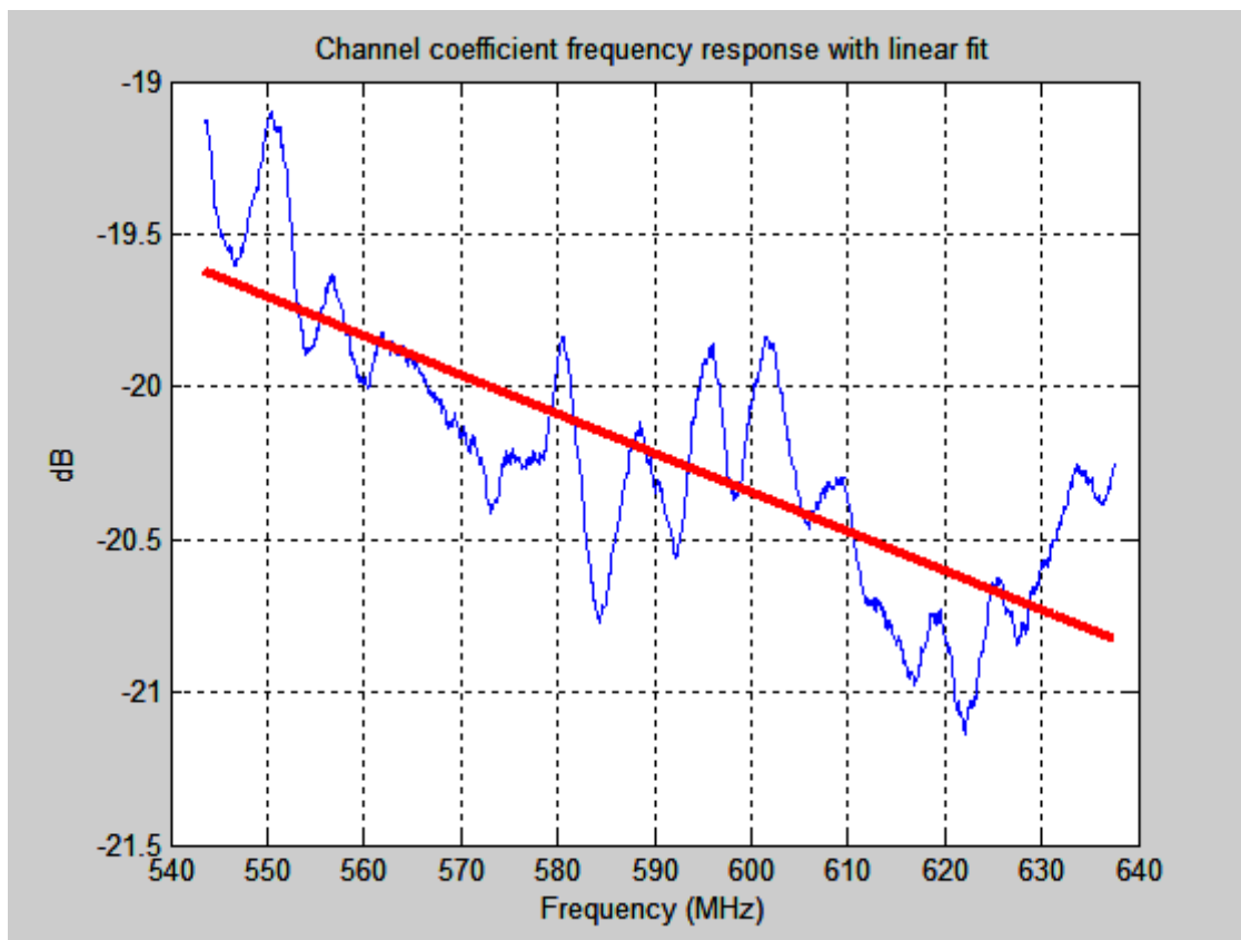
Figure 9 - Frequency Response of Channel Estimate Coefficient, with Best-Fit Line
