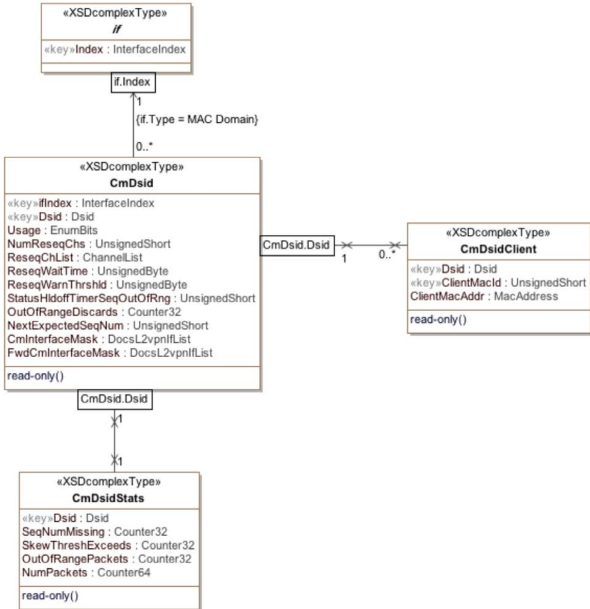
Figure 18 - DSID Information Model Diagram
