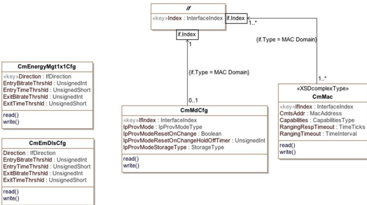
Figure 19 - CM MAC Domain Configuration Information Model Diagram
