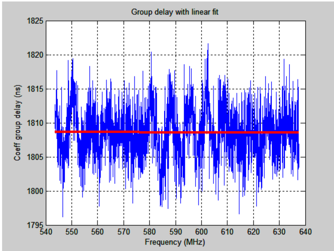
Figure 10 - Group Delay Response Of Channel Estimate Coefficients, With Best-Fit Line
