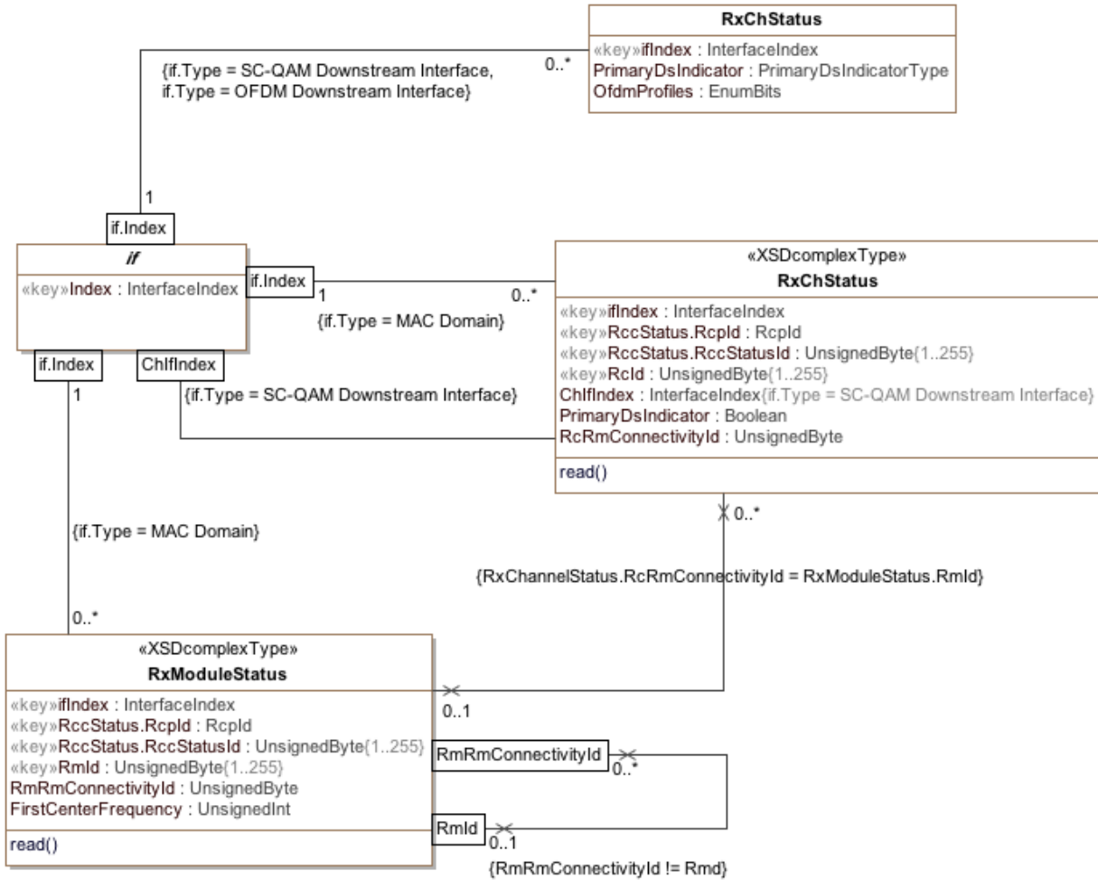
Figure 15 - RCC Status Information Model Diagram
