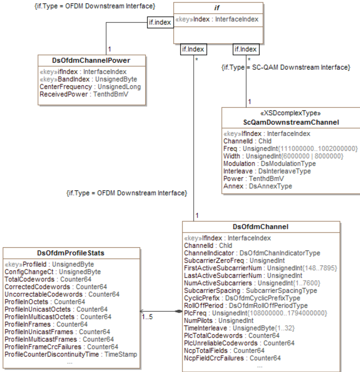
Figure 13 - CM Downstream Information Model Diagram
