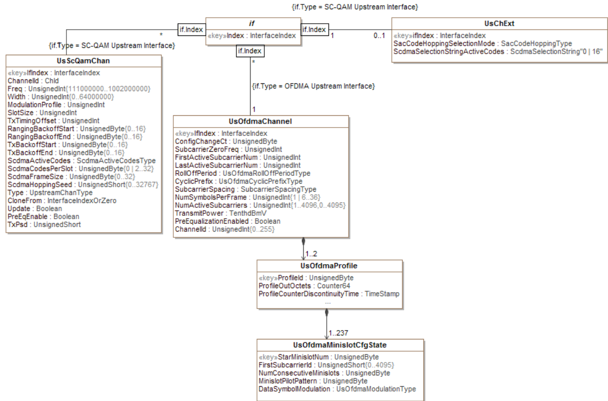
Figure 14 - CM Upstream Information Model Diagram
