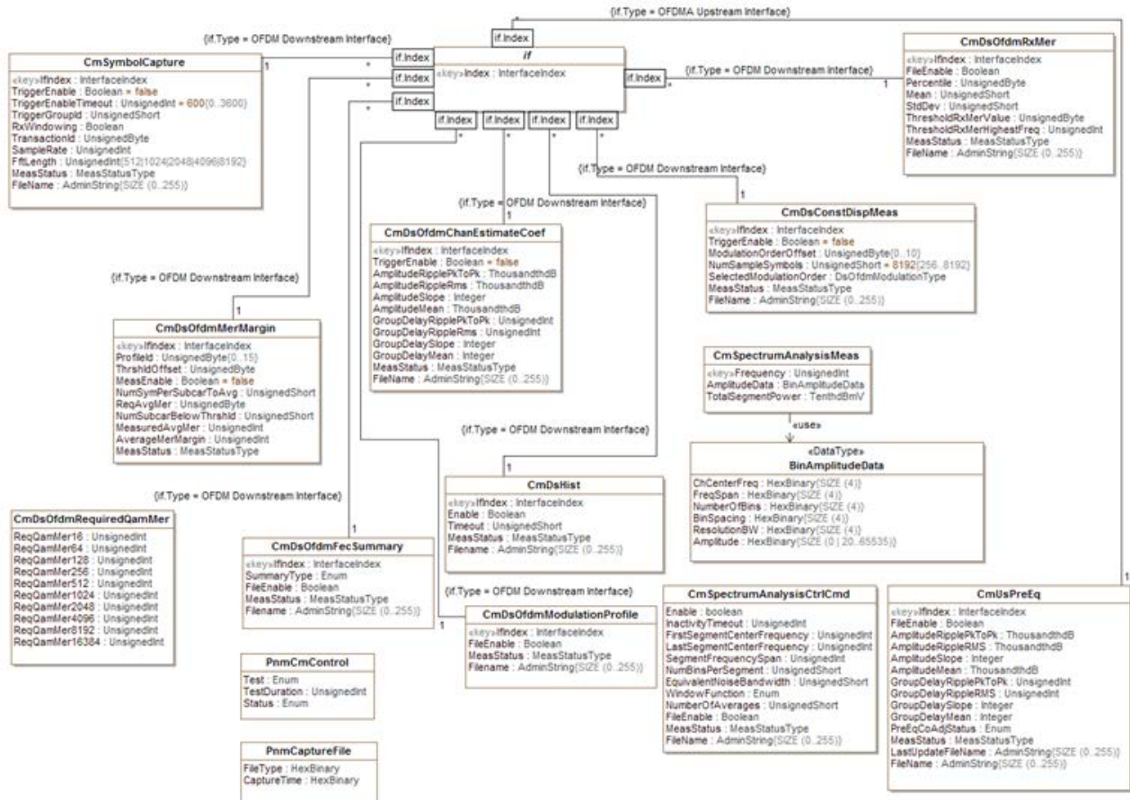
Figure 8 - Proactive Network Maintenance Information Model Diagram
