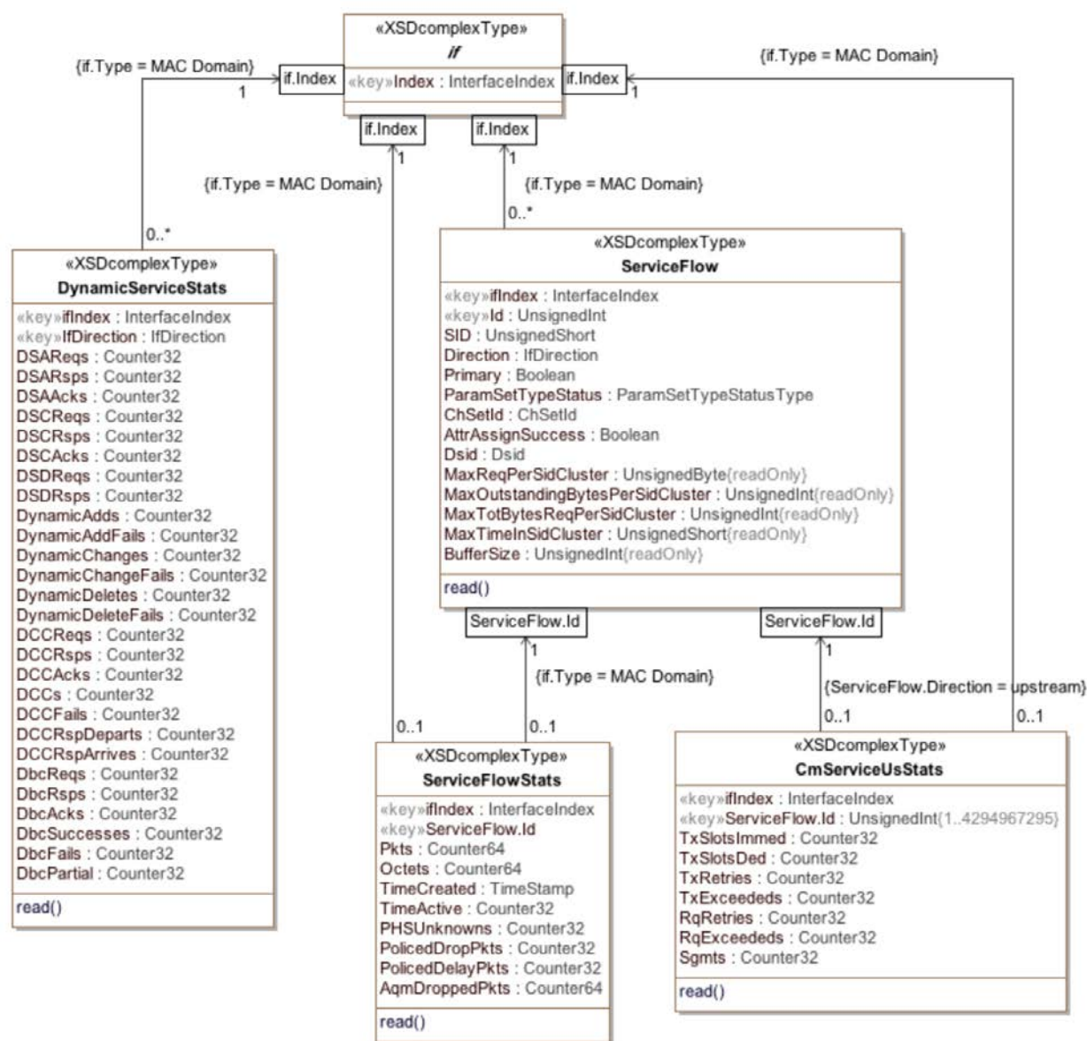
Figure 17 - QoS Statistics Information Model Diagram
