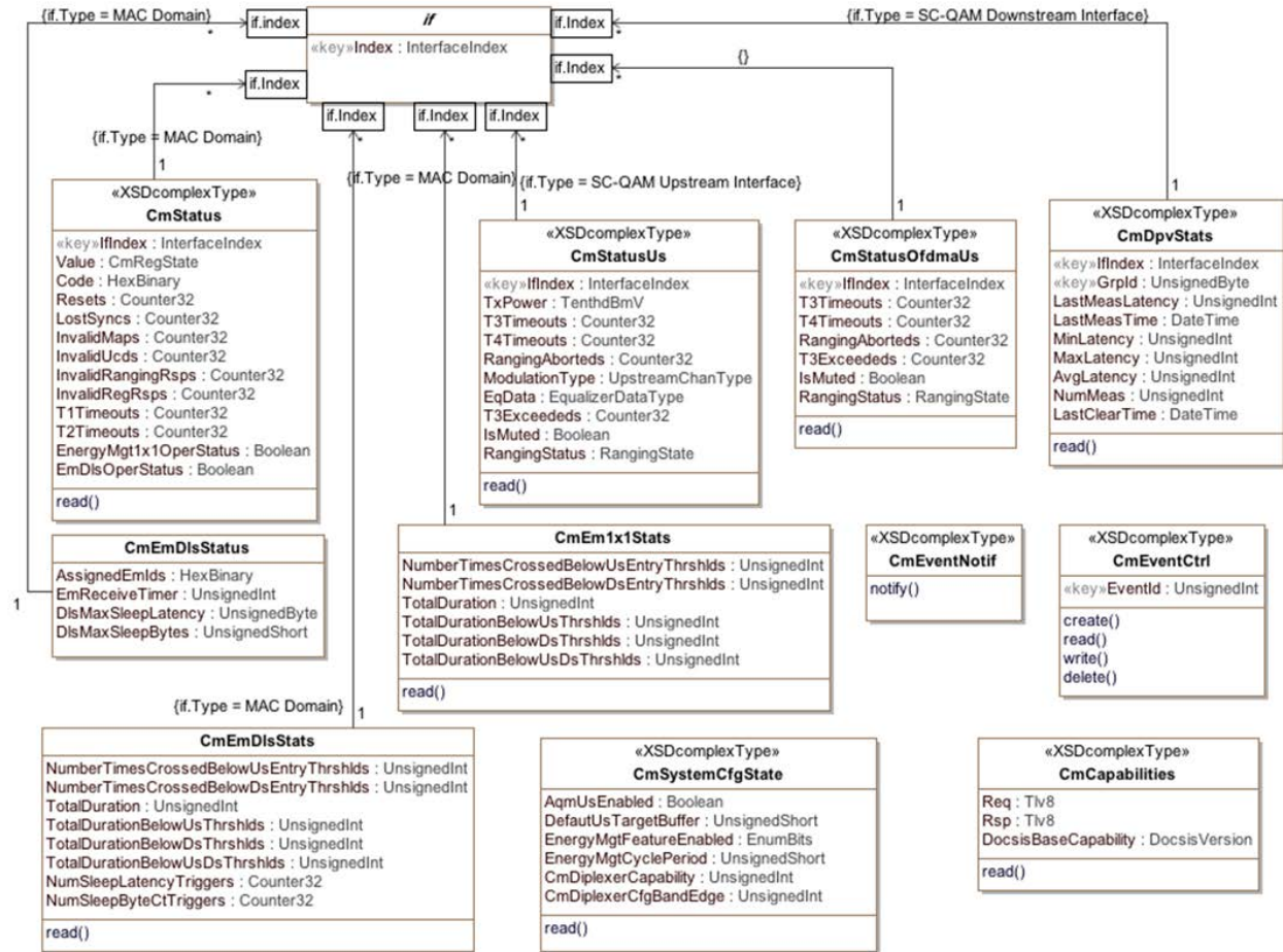
Figure 12 - CM Operational Status Information Model Diagram
