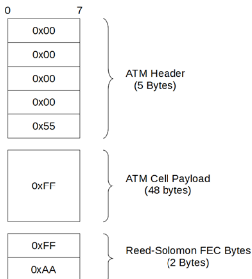
Figure 5 - ATM IDLE Cell Format
