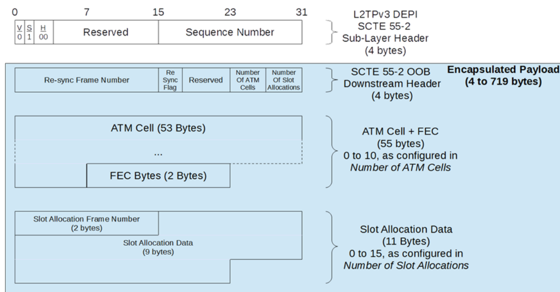
Figure 2 - SCTE 55-2 Downstream Packet Format 6
