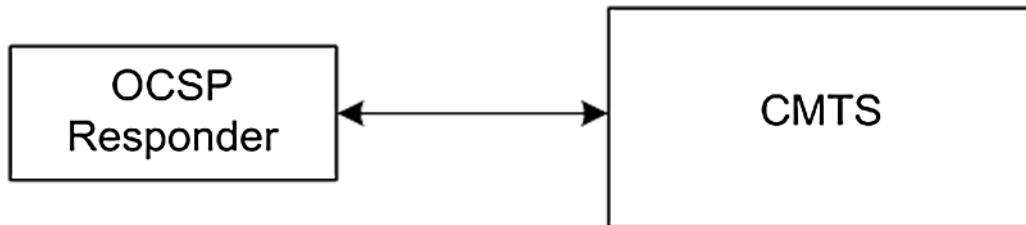
Figure 14 - OCSP Framework
